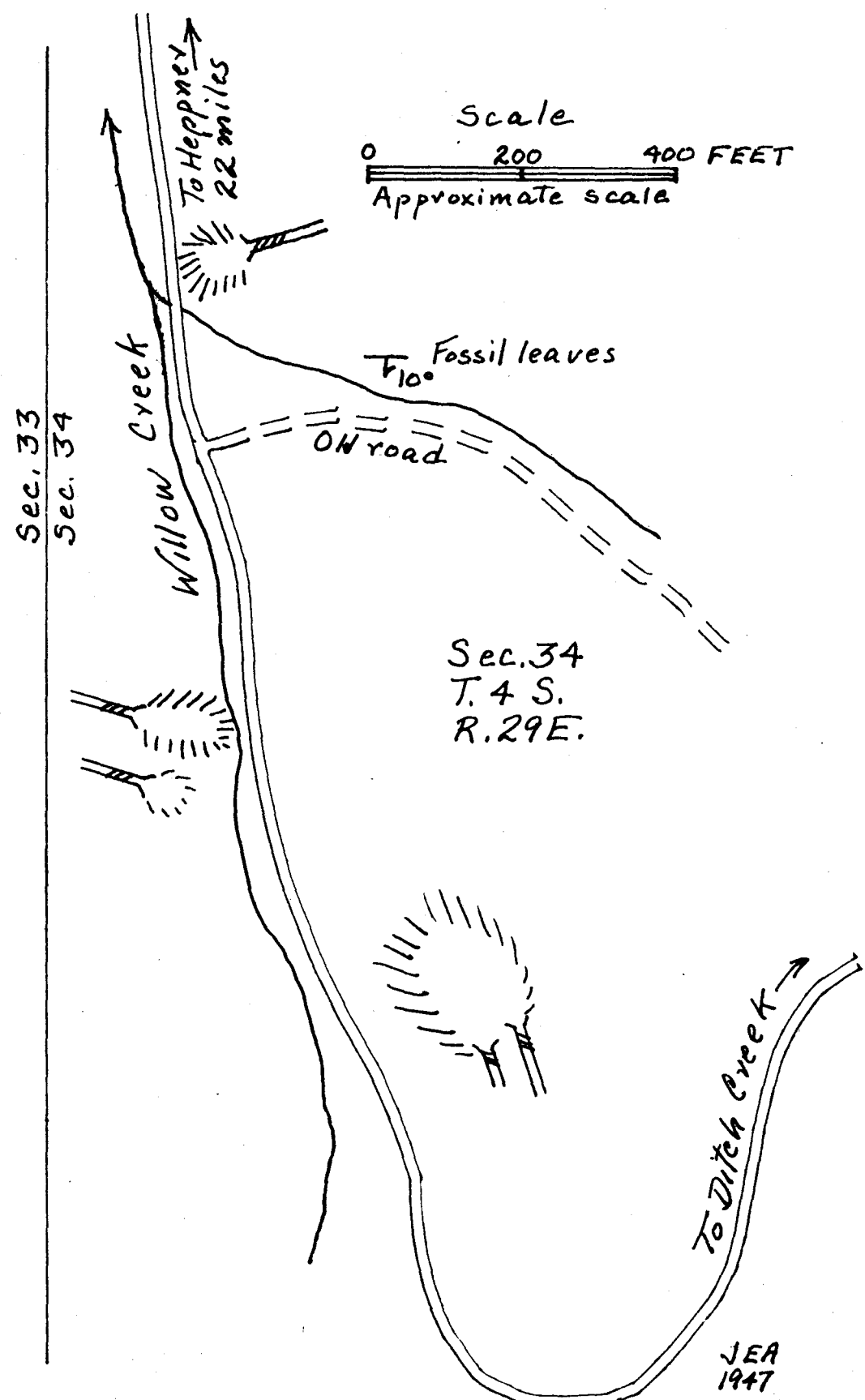
FIG. 3 Sketch map of Willow Creek coal prospects.
