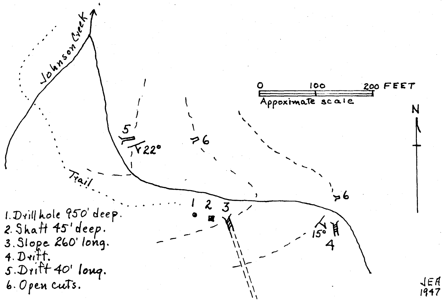
FIG. 2 Sketch map of Drill Camp coal prospects.
