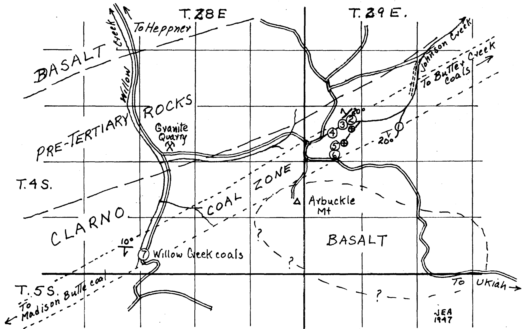
FIG. 1 Location and geological sketch of Heppner coal area.
