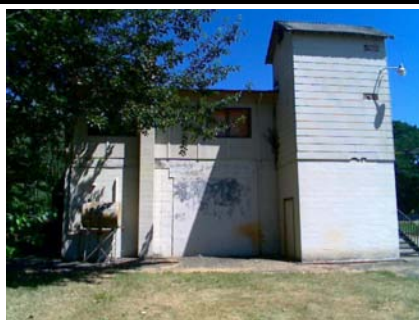
W Vertical Irregularity Primary also shows a plan irregularity, and a solid back wall indicating a possible torsion problem.
