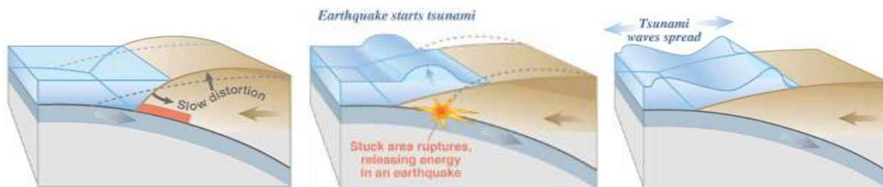
Figure 1. Illustration of a tsunami triggered by a subduction zone. The image on the left shows the subducting plate (grey) sliding under the continental plate (brown); the red area marks the zone where the two plates are stuck, and the dotted lines show how the continental plate would lie if it were not distorted by pressure. In the central image, the locked section breaks: the two plates move abruptly, displacing the water above the rupture. In the righthand image, the tsunami travels away from the rupture zone. (Image: USGS Circular 1187)
