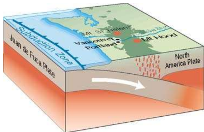
Figure 2. Cross section of the Cascadia subduction zone, an approximately 700-mile (1,130-km) long fault zone where the Juan de Fuca Plate, along with the Explorer Plate to the north and the Gorda Plate to the south, collide with and descend beneath the North America Plate. (Image: USGS)
