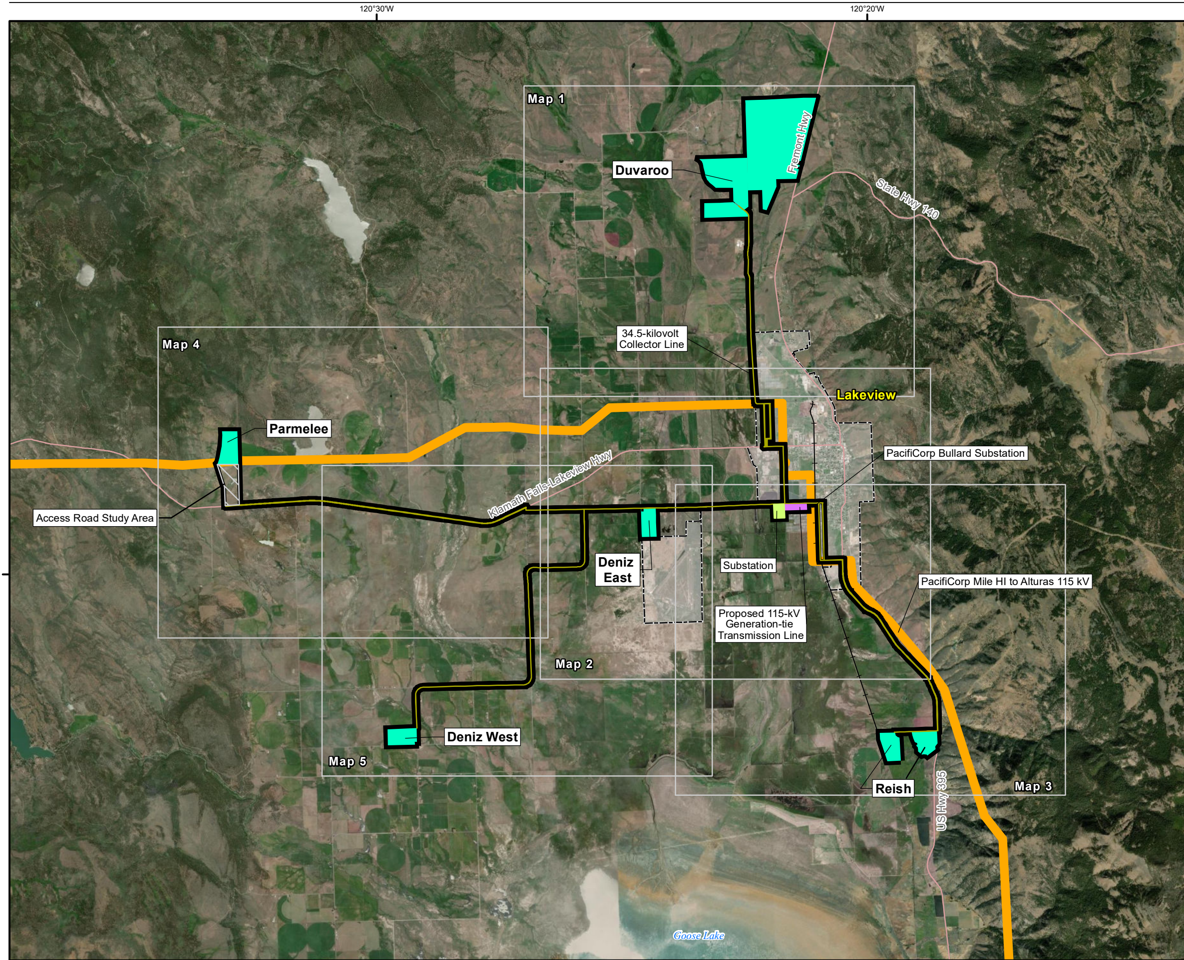
Figure G-2 Overview of Facility Layout Notice of Intent Blue Marmot Solar Energy Facility Lake County, OR
