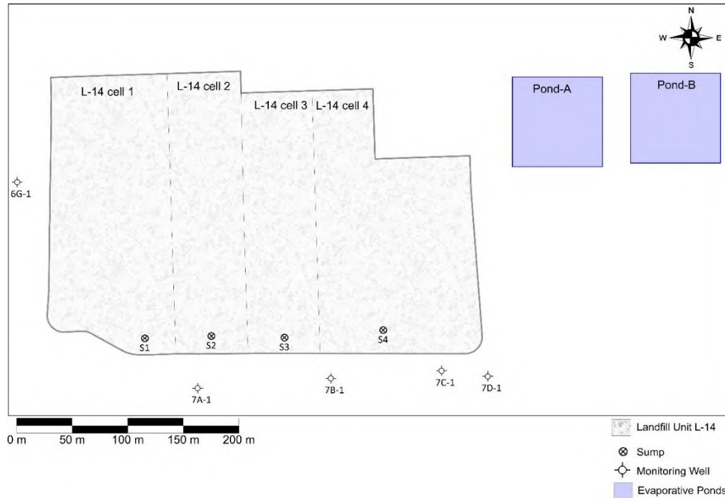
Figure 2-4. Landfill Unit L-14 showing the four cells (L-14 cell 1, L-14 cell 2, L-14 cell 3, and L-14 cell 4), the sumps (S1, S2, S3, and S4), evaporations ponds (Pond-A and Pond-B), and nearby monitoring wells.
