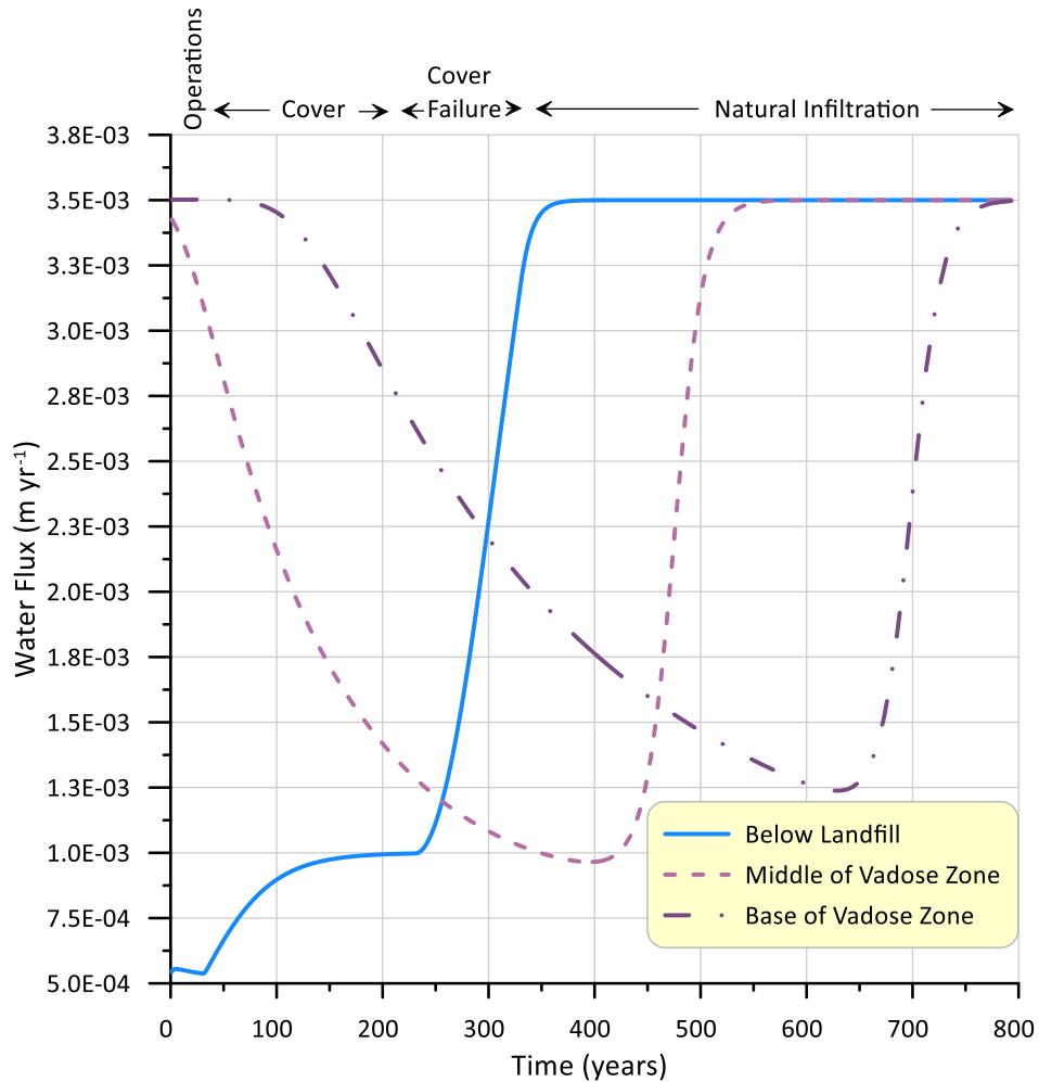
Figure 5-6. Vadoso zone water fluxes as a function of time starting at the time when the Bakken oilfield waste was disposed.
