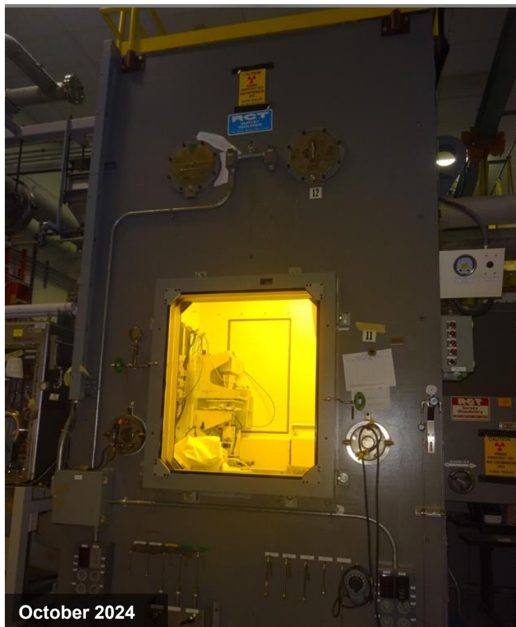
Newly installed hot-cell window
