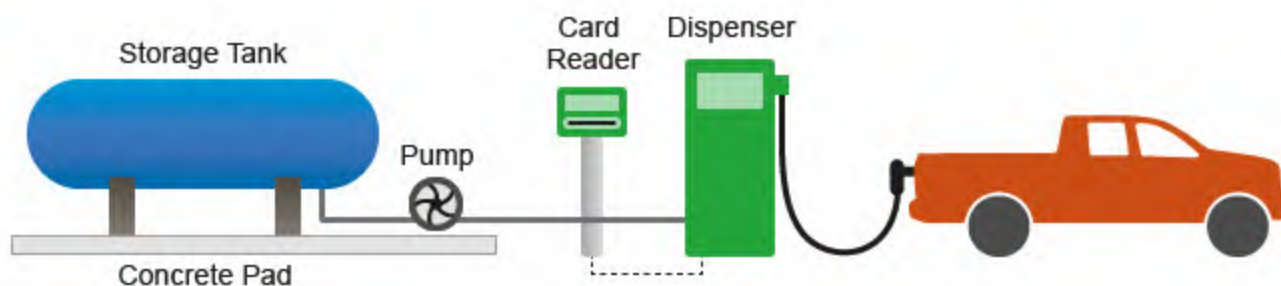
Figure 49: Propane Distribution 69
