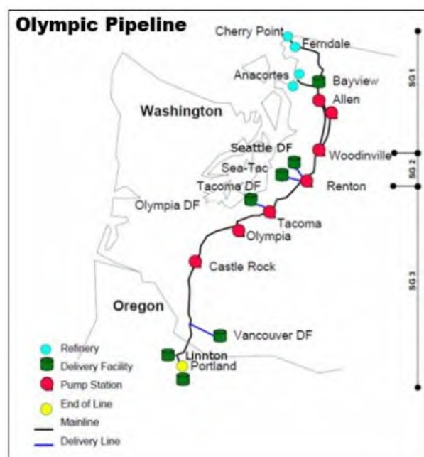
Figure 26: Olympic Pipeline Map 32
