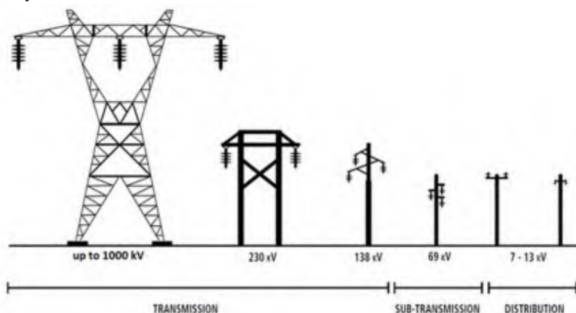
Figure 13: Typical Sizes of Transmission and Distribution Systems
