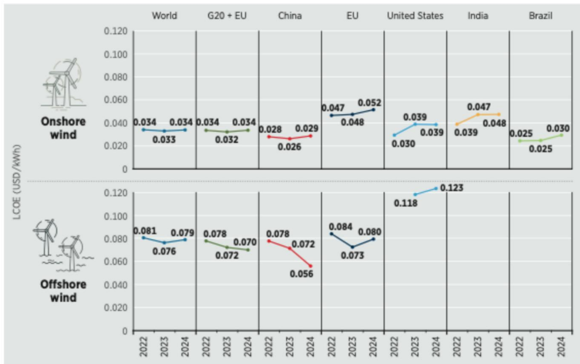
Figure 2. Wind power weighted average LCOE: Global, G20, EU and selected countries, 2022-2024.
