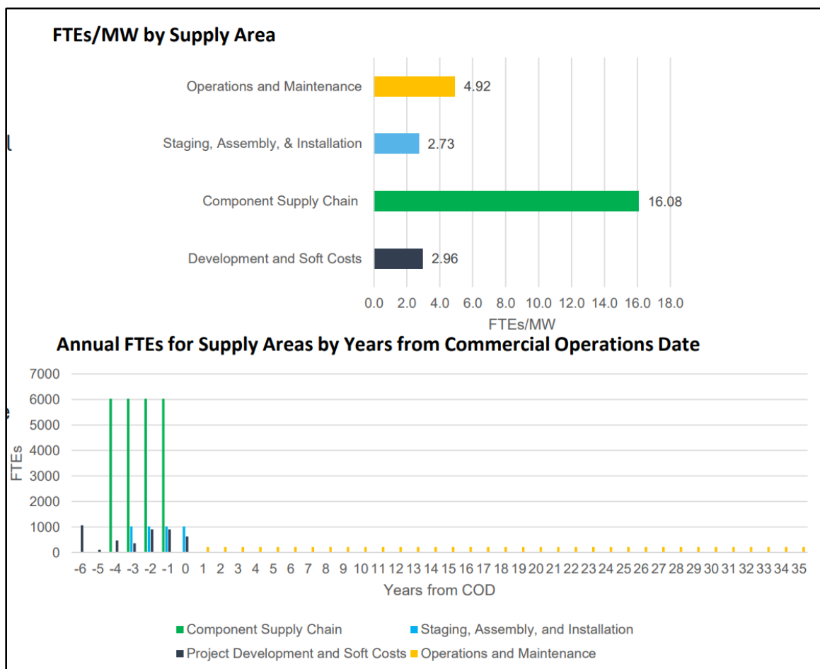
Figure 2-5. Summary Data of Job Duration and Supply Area Over the Course of an Offshore Wind Energy Project Lifecycle
