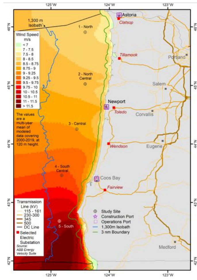
Figure 4-6. Annual average wind speeds offshore Oregon along with electrical transmission lines and substations
