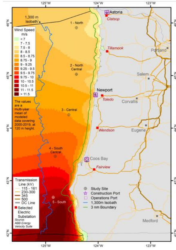
Figure 2-2. Annual average wind speeds off Oregon's coast along with electrical transmission lines and substations.
