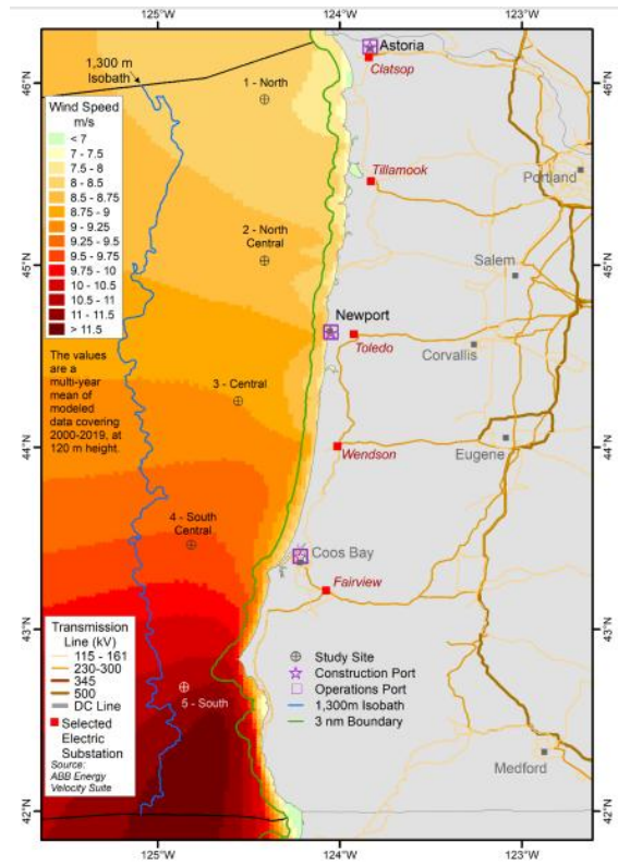
Figure 4-7. Annual average wind speeds offshore Oregon along with electrical transmission lines and substations (Source: PNNL 2021 144 )
