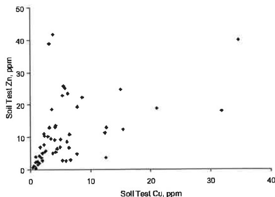
Figure 7.—The relationship between soil test Zn and Cu from the surface 6 inches of 56 fields on dairy farms.
