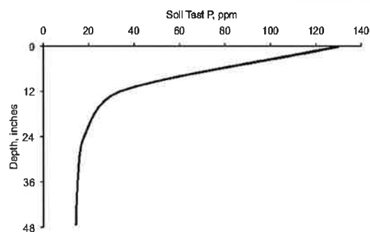
Figure 1.—Soil test phosphorus (Bray P1 extractant) with depth from a field of Woodburn soil regularly receiving manure. Created from data in Marx, E.S., 1995.
