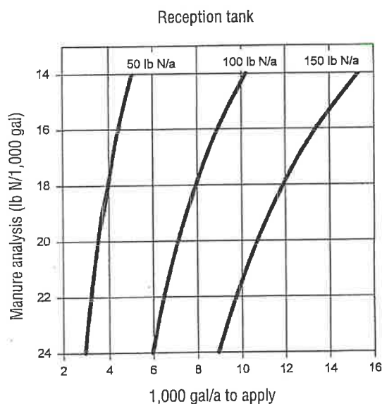
Figure 1.—Determining application rate for reception tank manure.
