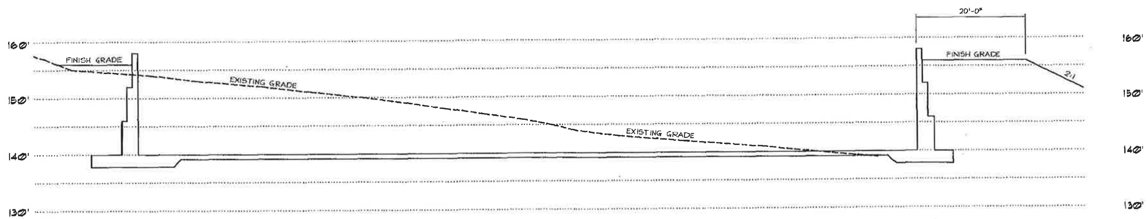
B LAGOON SECTION 1/8" = 1'-0"
