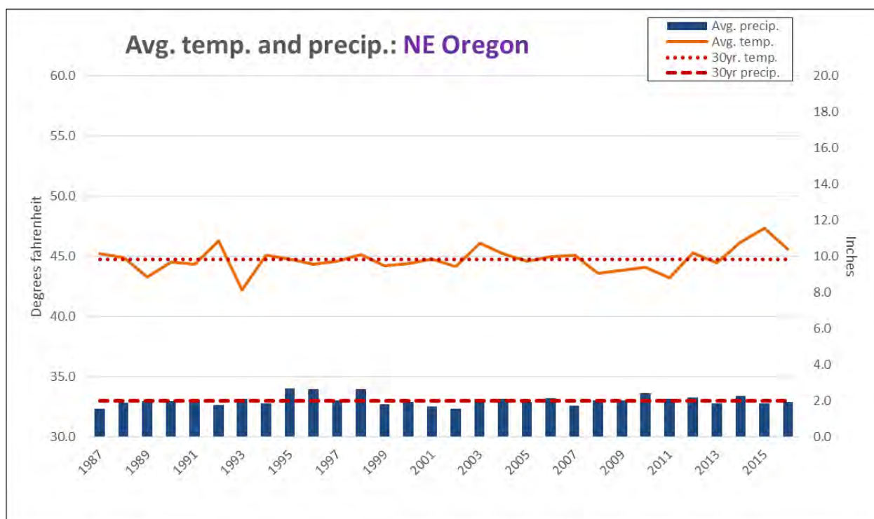
Figure 3. Raw annual average temperature and precipitation over the last 30 years in the Willamette Valley and northeastern Oregon ecoregions. Data from National Oceanic and Atmospheric Administration.
