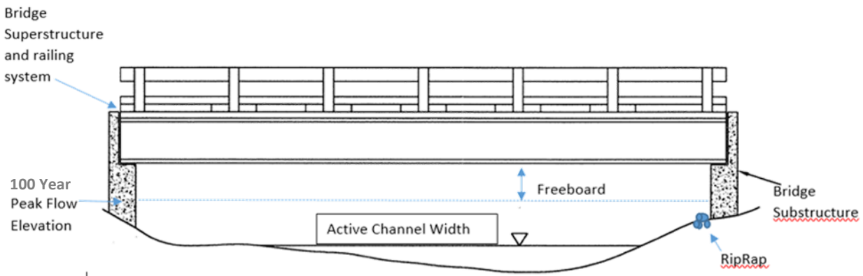
Figure 8. Freeboard illustration.
