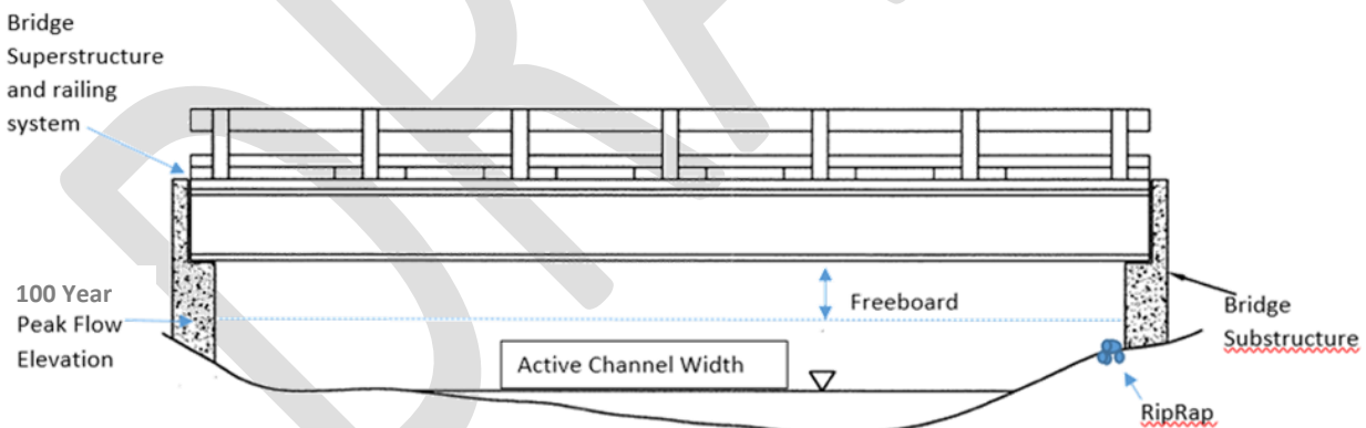
Figure 8. Freeboard illustration.
