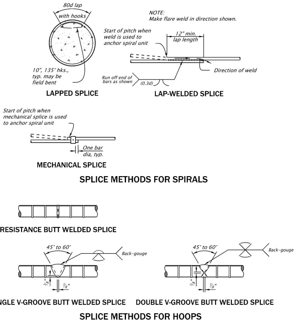
Figure 1.11.3.6-1 Transverse Reinforcement Splice Methods and Termination Details
