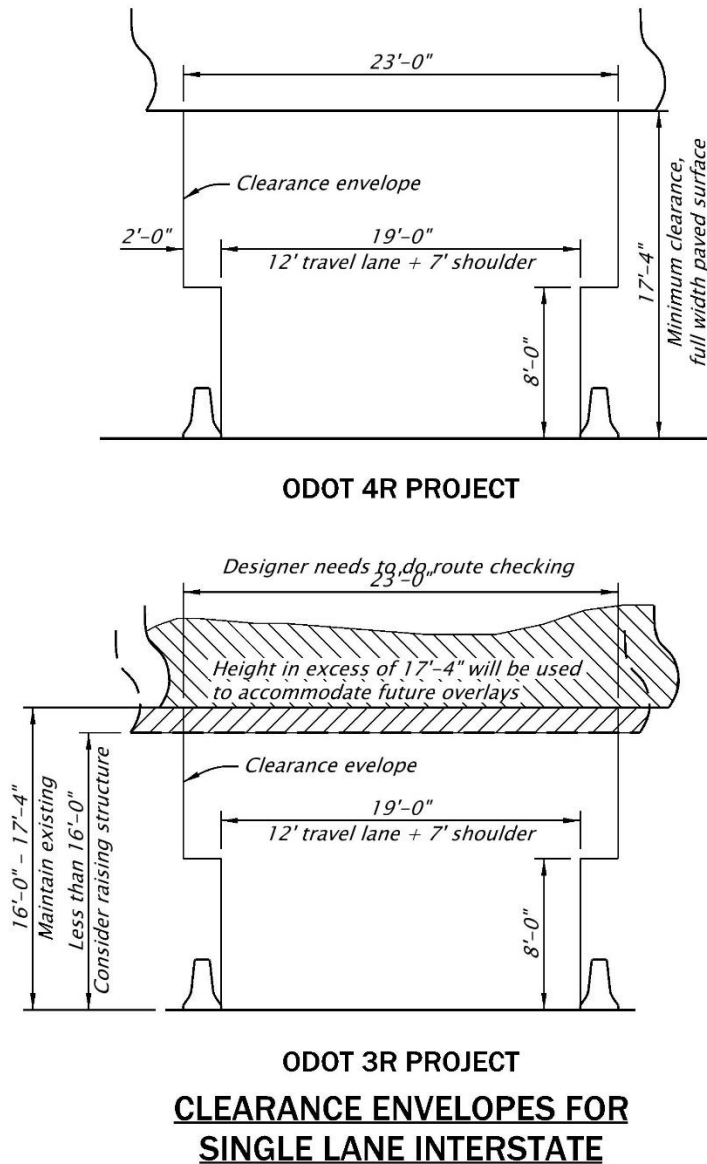
Figure 0-2 Clearance Envelopes
