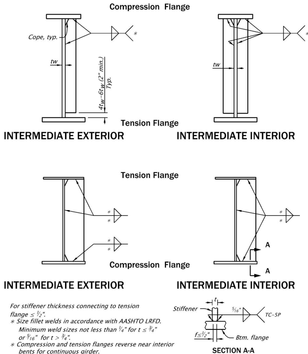
Figure 1.6.2.8.4-1 Intermediate Web Stiffeners
