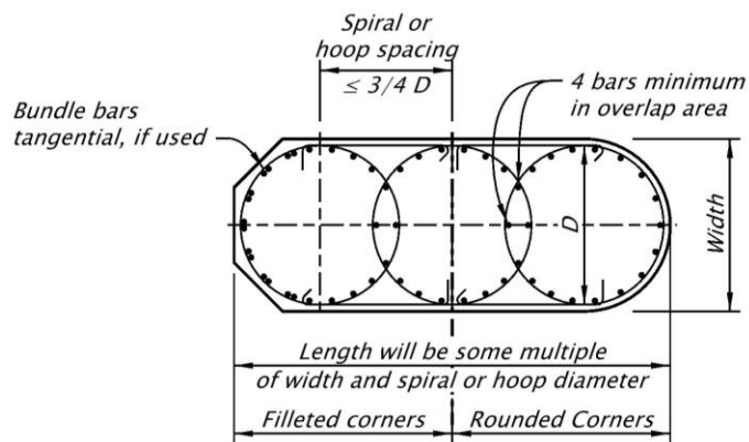
Figure 1.11.3.5-1 Multiple Interlocking Transverse Reinforcing Details
