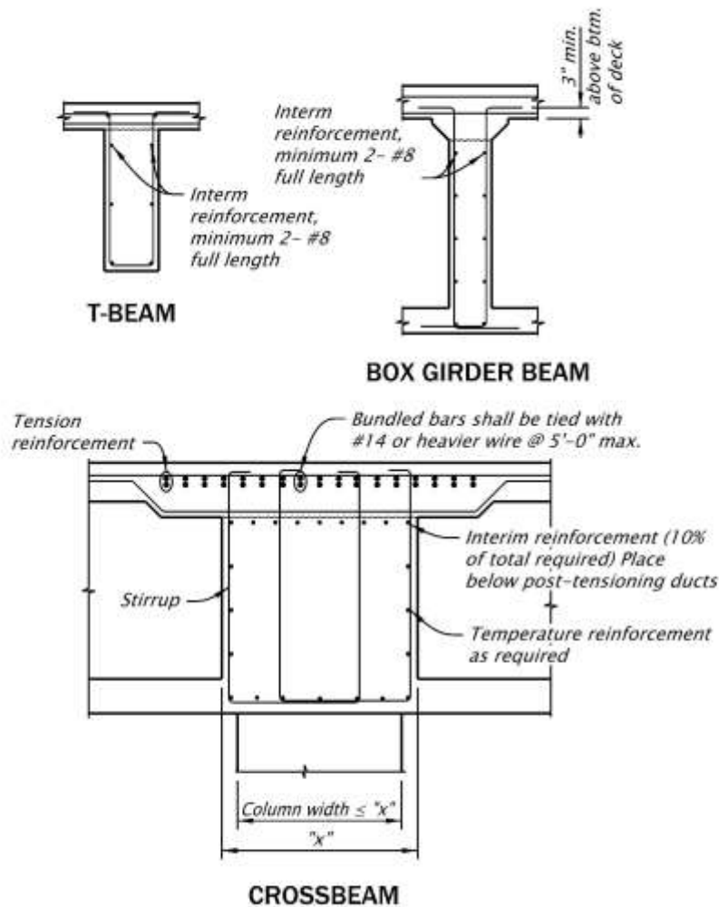
Figure 1.5.5.19-1 Interim Reinforcement
