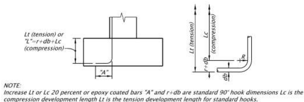
Figure 1.5.5.8-1 Minimum Column Bar Lengths in Footings
