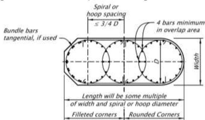
Figure 1.11.3.5.2-1 Multiple Interlocking Transverse Reinforcing Details
