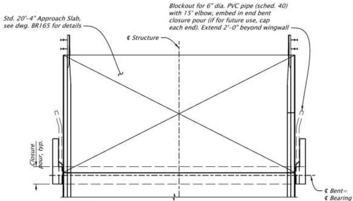
PLAN- END BENT
