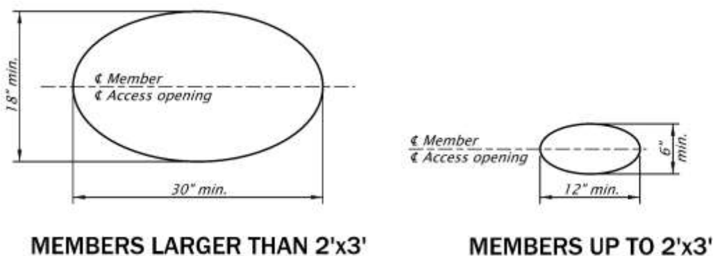
Figure 1.6.4.4.1-1 Access Openings for Closed Members
