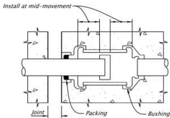
Figure 1.14.2.4.2-1 Electrical Conduit Expansion Joint
