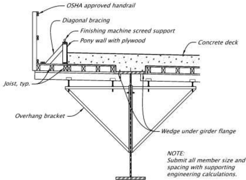
Figure 1.16.3.3.2-2 Typical Deck Forming Detail
