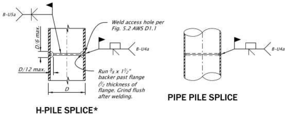
Figure 1.10.5.4.2-3 Steel Pile Splices
