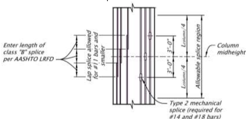
Figure 1.11.3.5.3-1 Vertical Bar Splices
