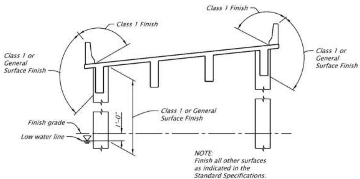
Figure 1.5.2.1-3 Concrete Finish Detail for Reinforced Concrete Deck Girder Bridges
