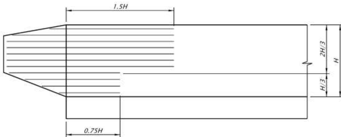
Figure 1.11.2.3-1 Wingwall Reinforcement
