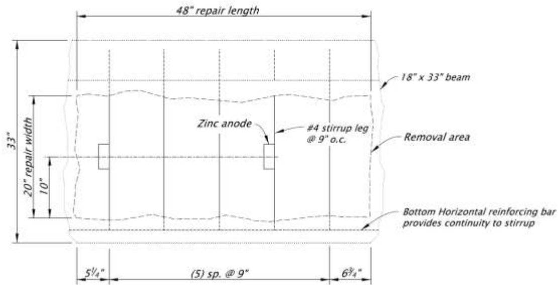
Figure 1.15.2.1.3-2 Anode Puck Placement for Beam Repair with Stirrups (one -directional reinforcing) Elevation View
