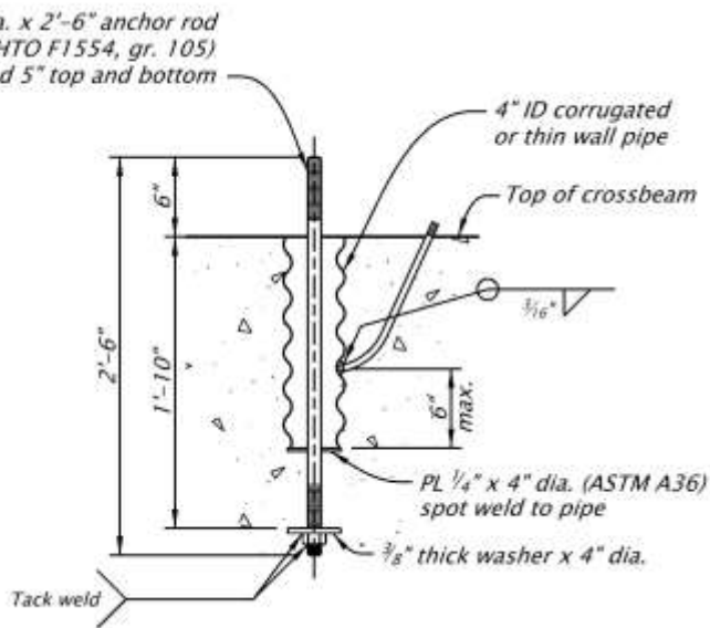
Figure 1.5.11.2-1 Anchor Rod Detail
