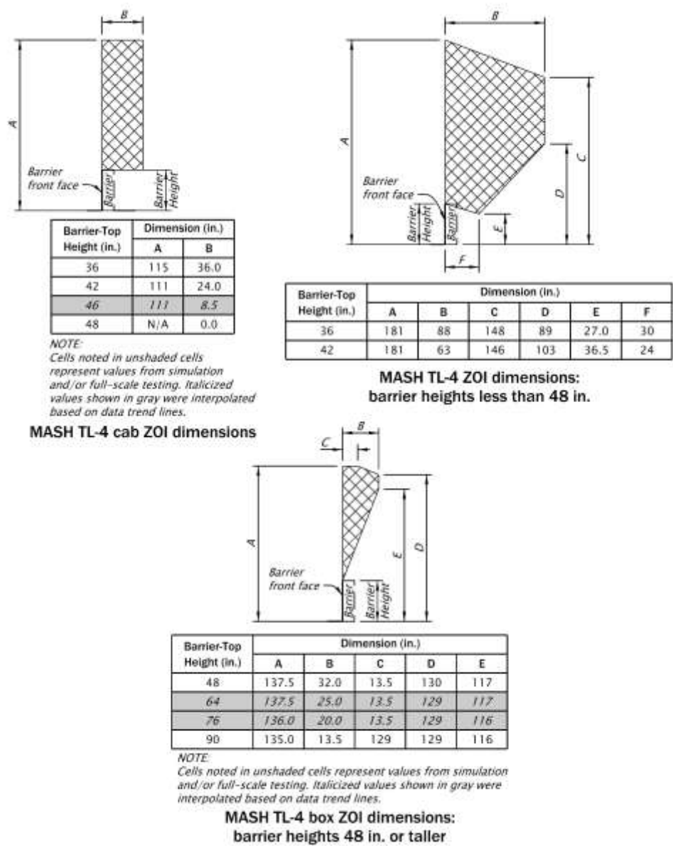
Figure 1.3.6-2 MASH TL-4 Zones of Intrusion
