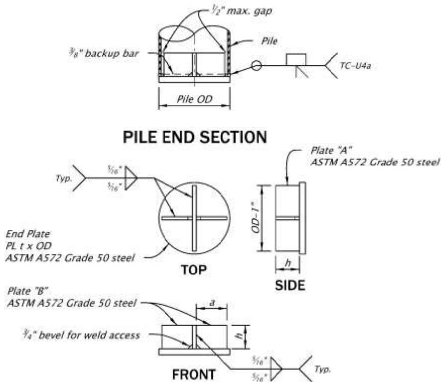
Figure 1.10.5.4.1-2 Welded End Plate with Stiffeners
