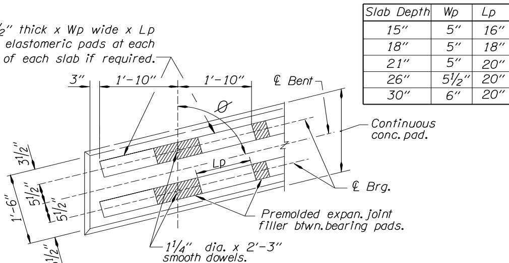
BEARING DETAIL (PRESTRESSED SLABS)
