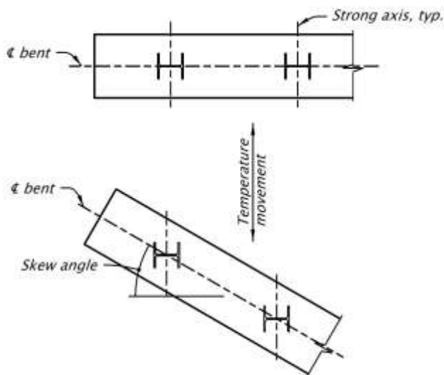
Figure 1.11.2.5-1 H-Pile Orientation
