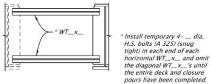
Figure 1.6.2.18-2 Diaphragm Connection Detail
