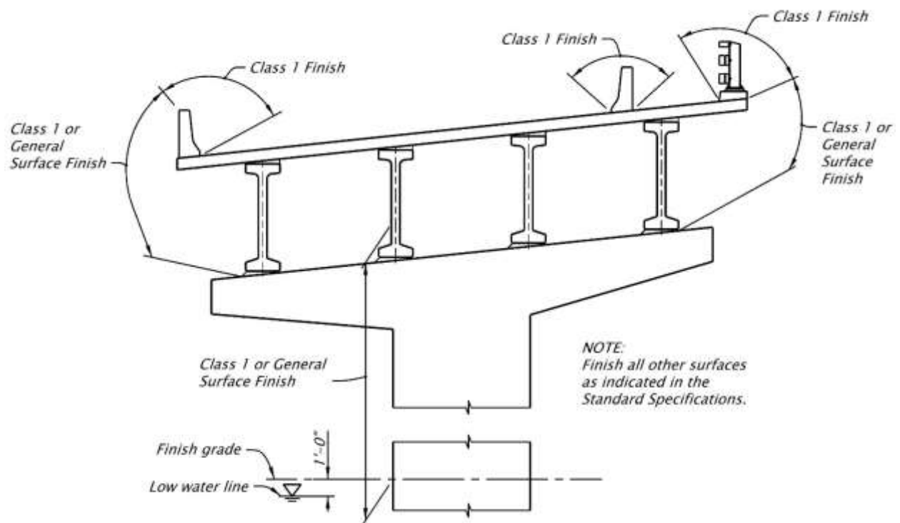
Figure 1.5.2.1-2 Concrete Surface Finish Detail for Precast/Prestressed Concrete Girder Bridges
