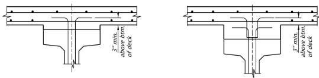
Figure 1.5.6.2.5-1 Beam Stirrup Details
