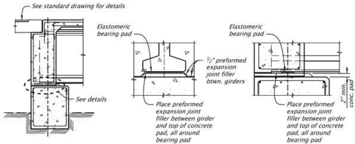
Figure 1.11.2.8-3 Bearing Detail
