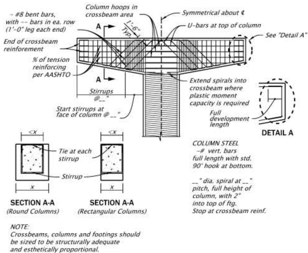
Figure 1.11.3.1-3 Structure Detailing Requirements
