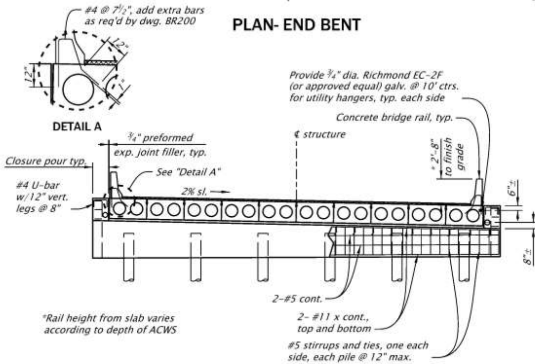
ELEVATION- END BENT
