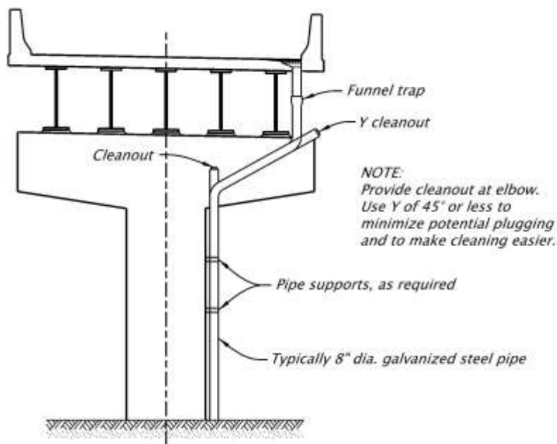
Figure 1.9.5.2-1 Drainpipe Detail
