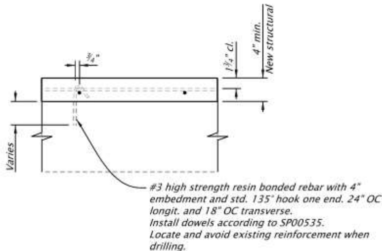
Figure 1.9.3.1.4-1 Shear Dowel Detail
