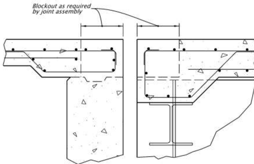
Figure 1.14.2.4.1-1 Expansion Joint Blockout
