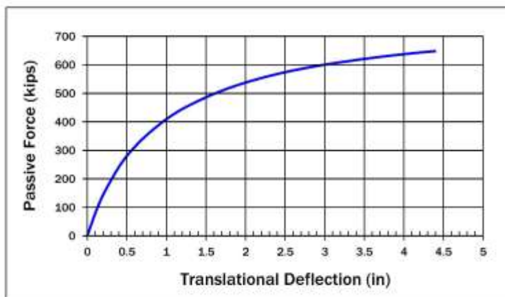
Figure 1.10.4.2.3-4 Pile Cap Stiffness
