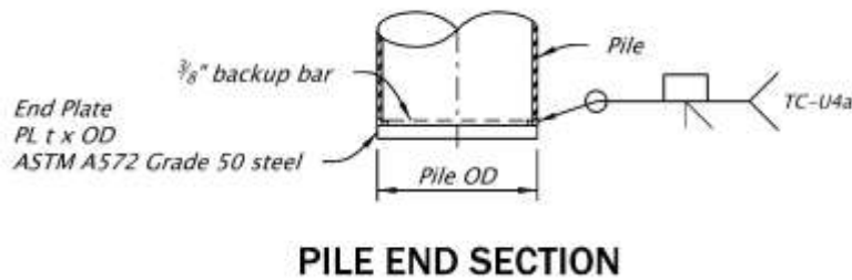
Figure 1.10.5.4.1-1 Welded End Plate
