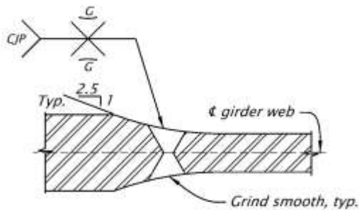
Figure 1.6.3.4-1 Unequal Thickness Web Splice
