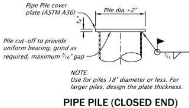
Figure 1.10.5.4.2-2 Pipe Pile Cover Plate
