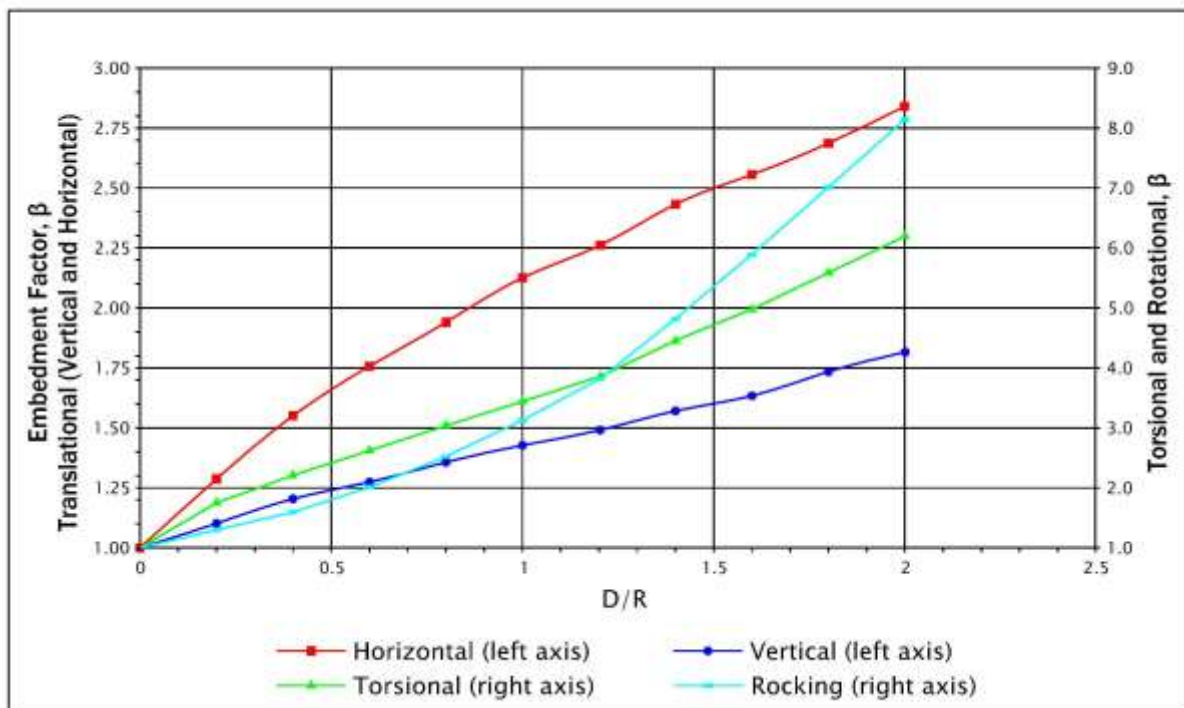
Figure 1.10.4.2.3-3 Embedment Factors for Footings, \beta
