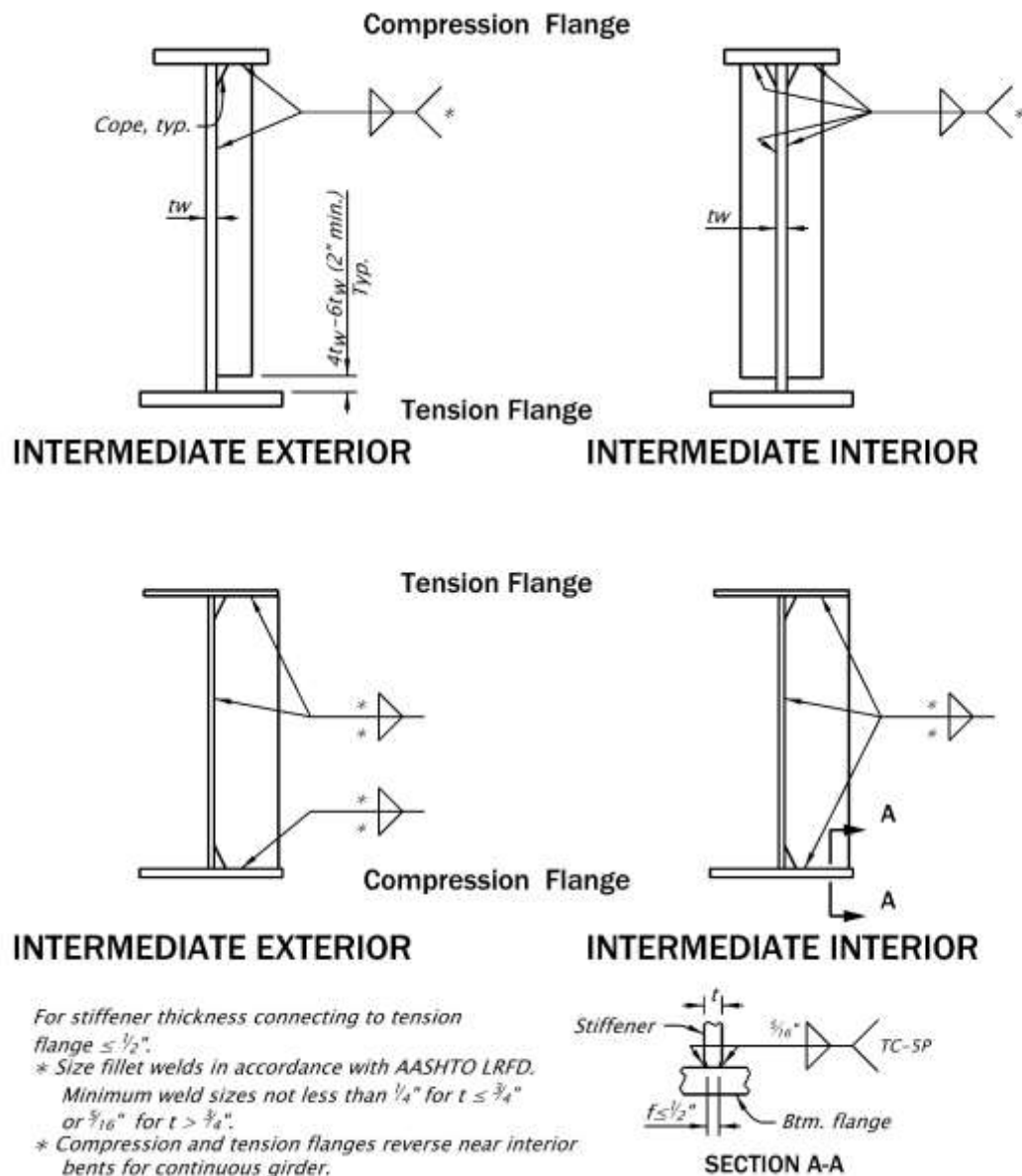
Figure 1.6.2.8.4-1 Intermediate Web Stiffeners
