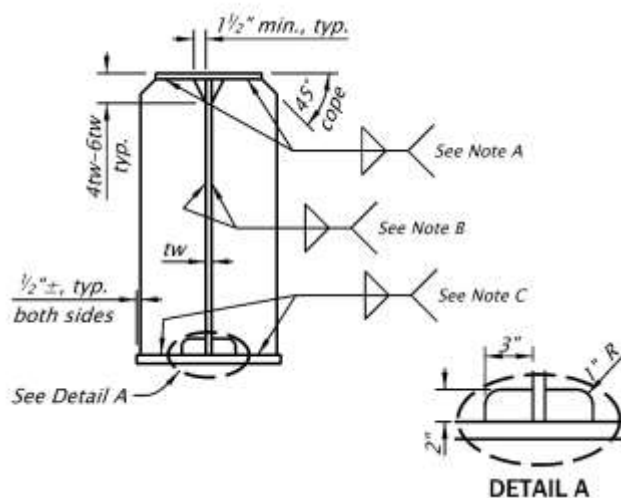
Figure 1.6.2.8.5-1 Bearing Stiffener Detail
