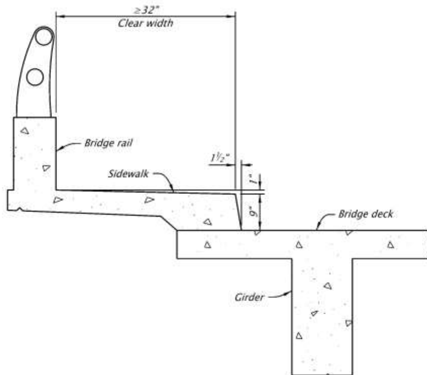
Figure 1.2.10.2.2-3 Existing Bridge, Clear Width Examples
