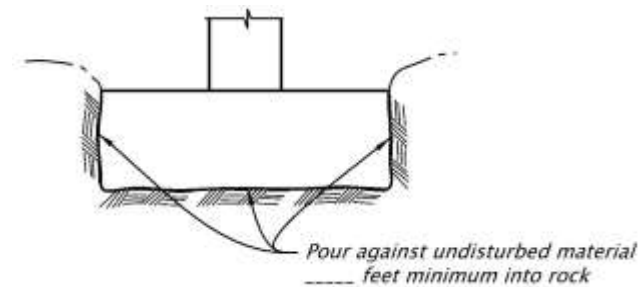
Figure 1.10.3.2-1 Footing Note Callouts at Streams
