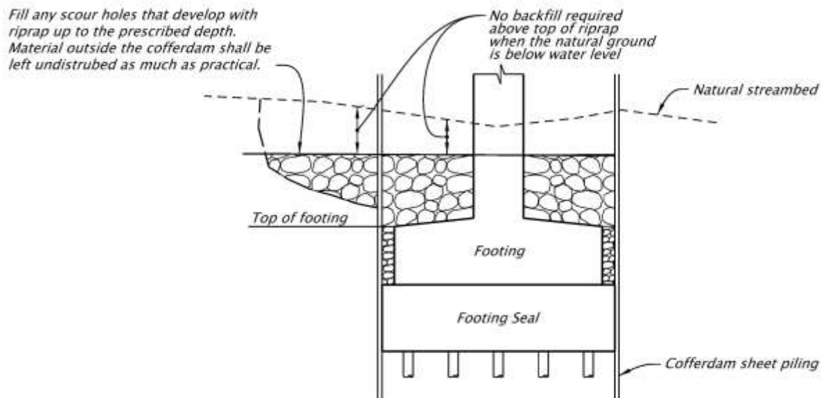
Figure 1.16.3.5.1-1 – Typical Cofferdam Detail
