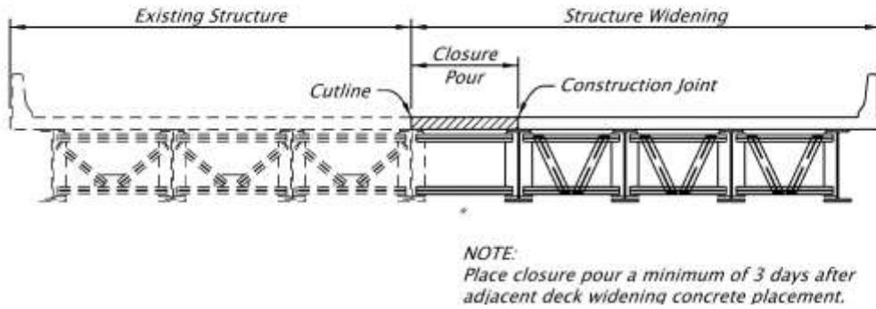
Figure 1.6.2.18-2 Diaphragm Connection Detail
