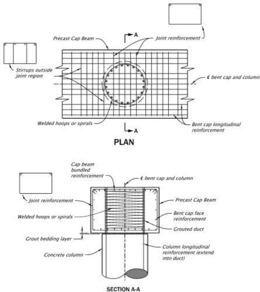
Figure 1.16.2.8-1 Grouted Duct Connection to Achieve Full Ductility.
