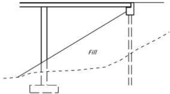
Figure 1.11.3.4-1 Additional Column Loading Situations
