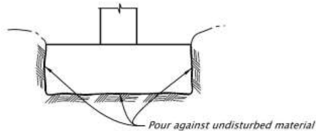
Figure 1.10.2-1 Lateral Earth Restraints
