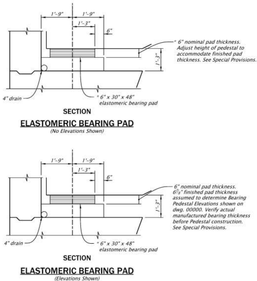
Figure 1.14.1.2-2 Elastomeric Bearing Pad Examples
