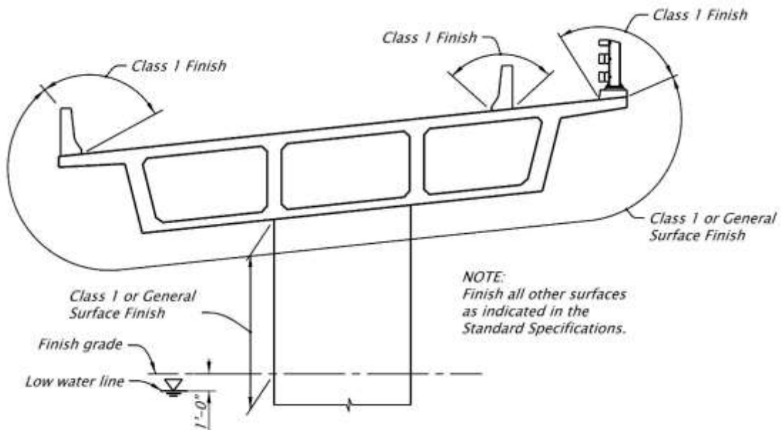
Figure 1.5.2.1-1 Concrete Surface Finish Detail for Box Girder Bridges
