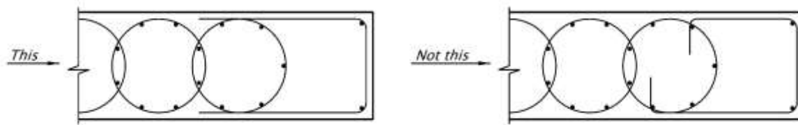
Figure 1.11.3.8-1 Supplemental Transverse Reinforcement Details
