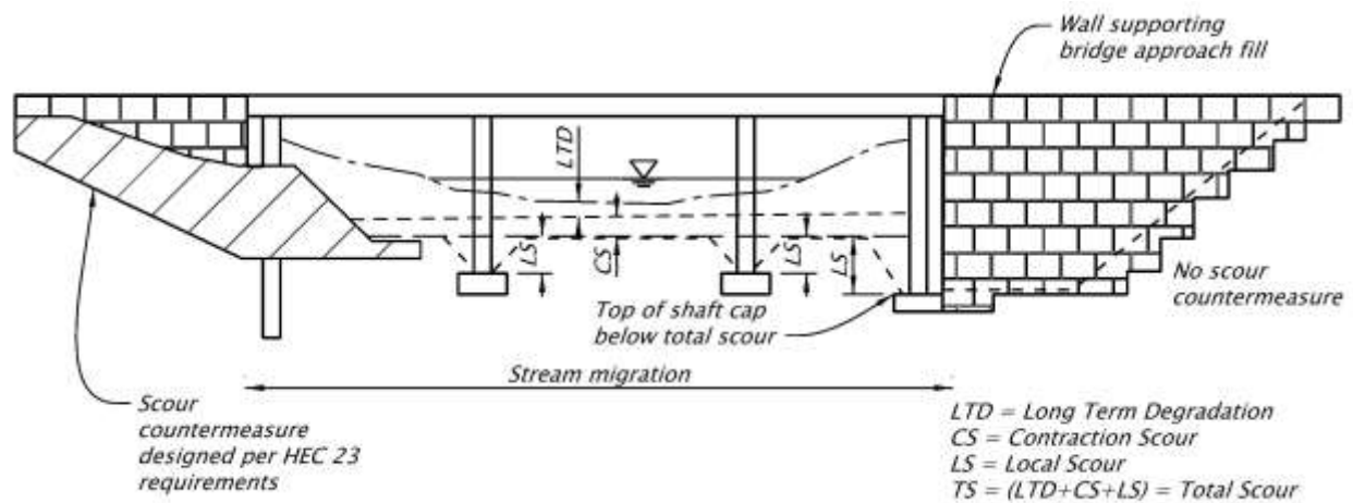
Figure 1.10.5.8-1 Scour Components
