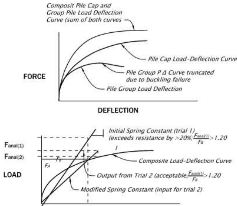
Figure 1.10.4.2.4-3 Modified Springs: (A) Development of Composite Load, Deflection Curve (B) Spring Iteration Process and Resistance Check
