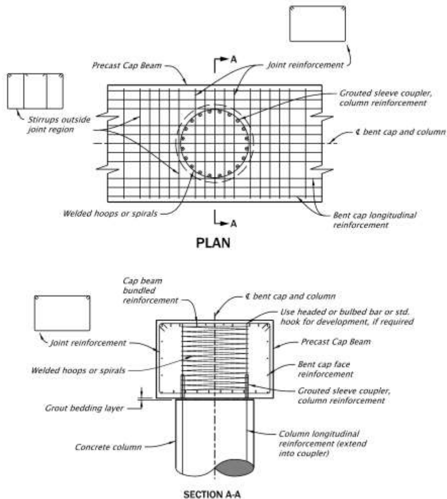
Figure 1.16.2.8-2 Grouted Sleeve Coupler Connection to Achieve Full Ductility
