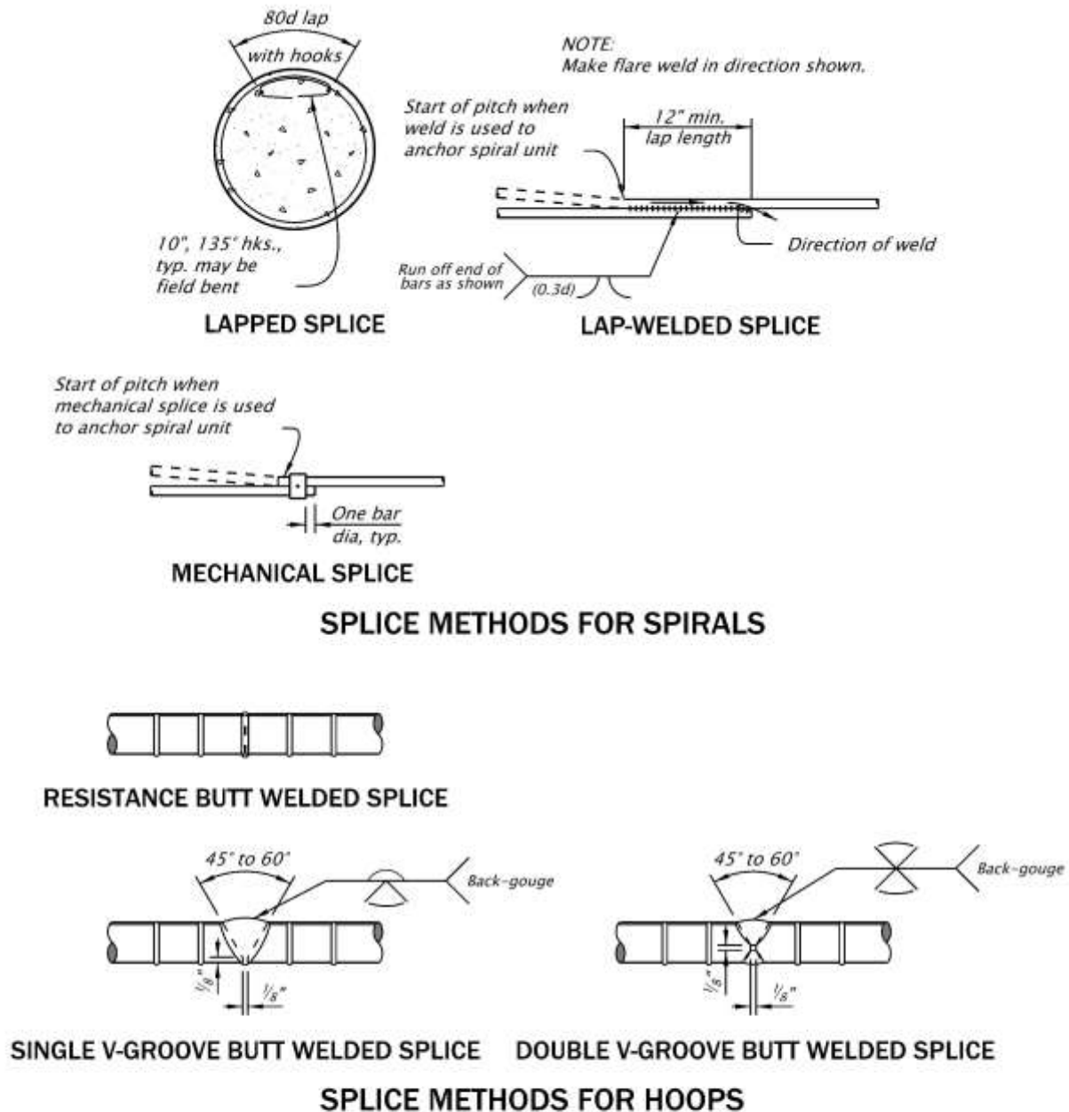
Figure 1.11.3.6-1 Transverse Reinforcement Splice Methods and Termination Details
