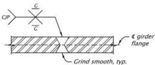
Figure 1.6.3.3-2 Equal Thickness Flange Splice
