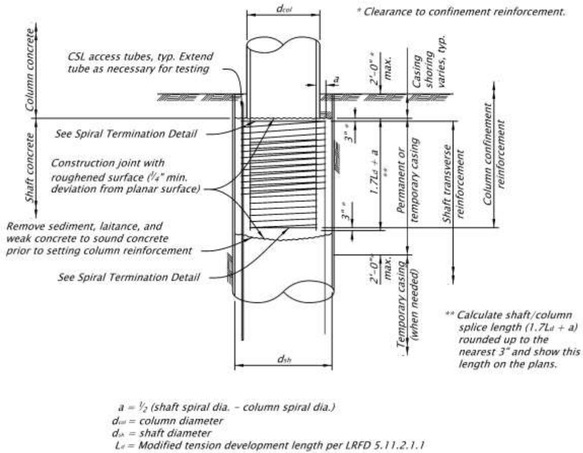
Figure 1.10.5.5.1-1 In-Ground Non-Contact Drilled Shaft Splice
