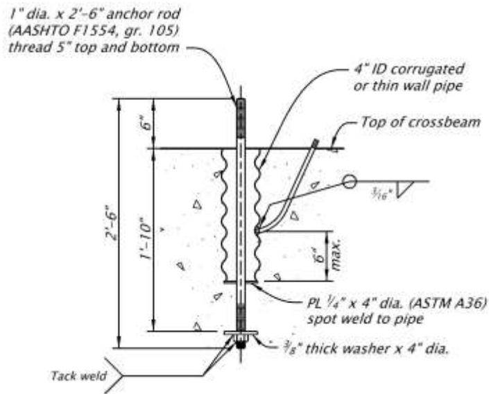
Figure 1.5.11.2-1 Anchor Rod Detail
