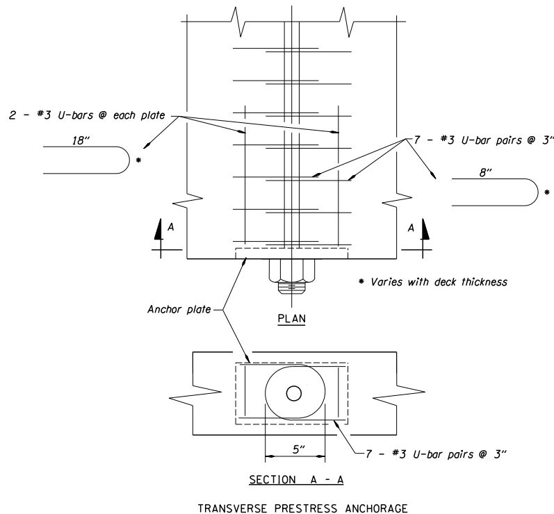
Figure 1.9.2.2.3-1 Transverse Prestress Anchorage
