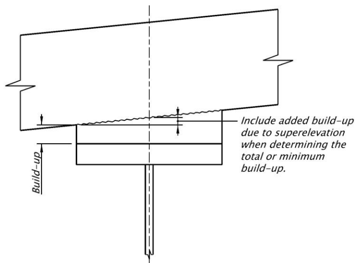
Figure 1.6.2.13-1 Superelevation Deck Build-Up
