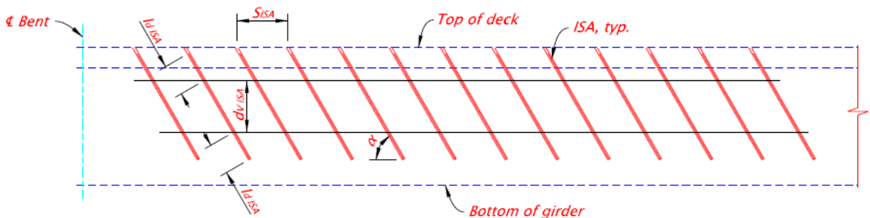
Figure 1.15.1.1.3-1 Internal Shear Anchors
