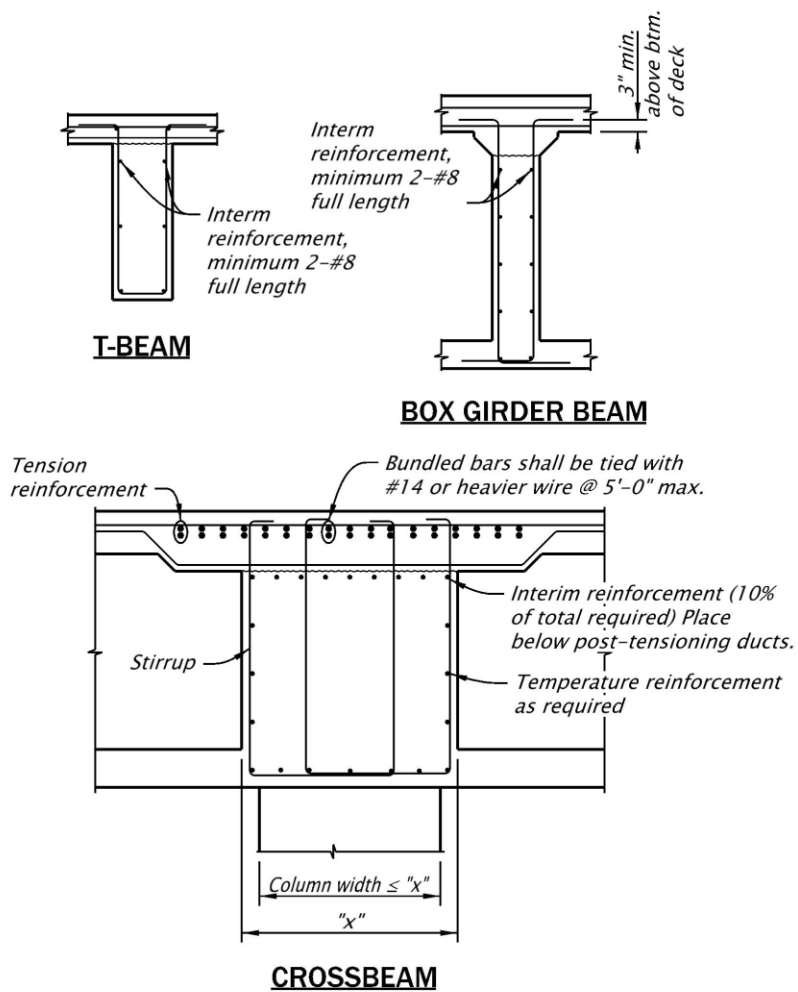
Figure 1.5.5.19-1 Interim Reinforcement
