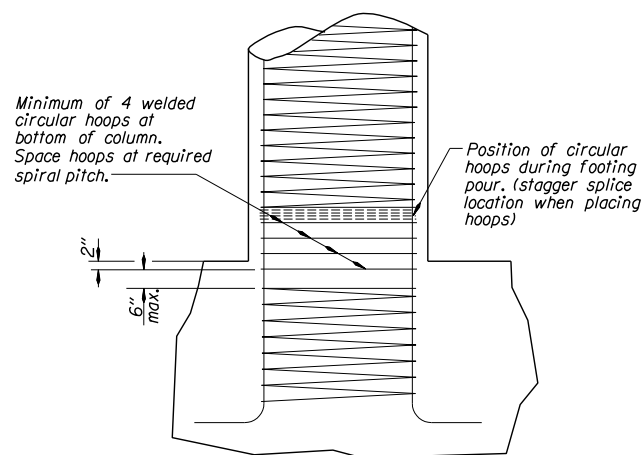
Figure 1.11.3.10-1 Optional Hoop Detail at Bottom of Column
