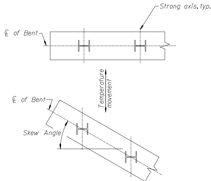
Figure 1.11.2.5-1 H-Pile Orientation
