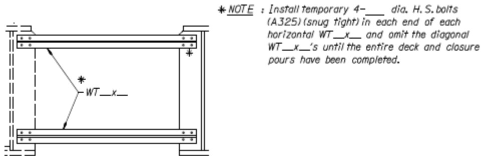
Figure 1.6.2.18-2 Temporary Diaphragm Connection Detail
