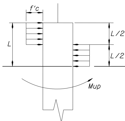
Figure 1.10.5.4.2-3 Method to Determine Steel Pile Embedment to Develop Fixity
