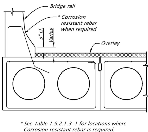
Figure 1.9.2.1.3-2 Reinforcement Protection for Non-Coastal Precast Slabs and Boxes
