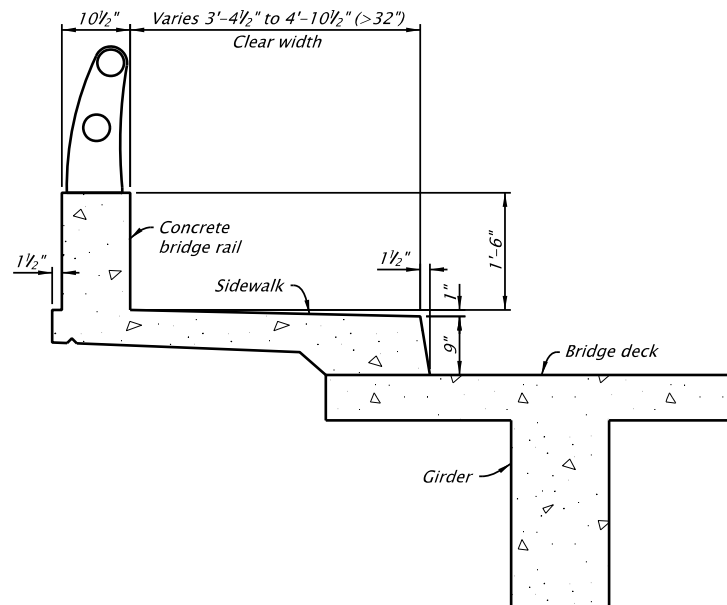
Figure 1.2.10.2.2-2 Existing Bridge, Section with Sidewalk
