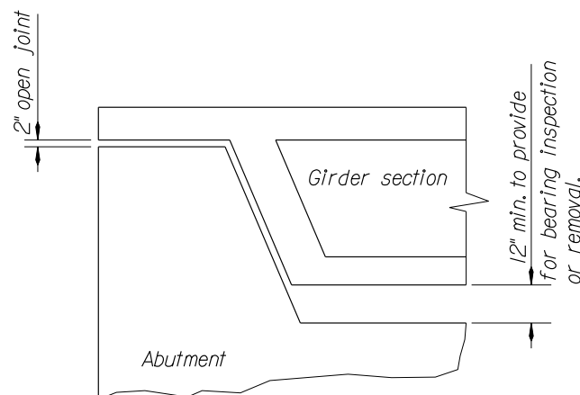
Figure 1.11.2.11-1 Bent Joint Detail
