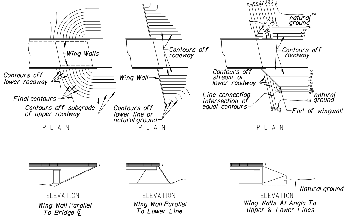
Figure 1.11.2.2-1 Wingwalls at End Bents
