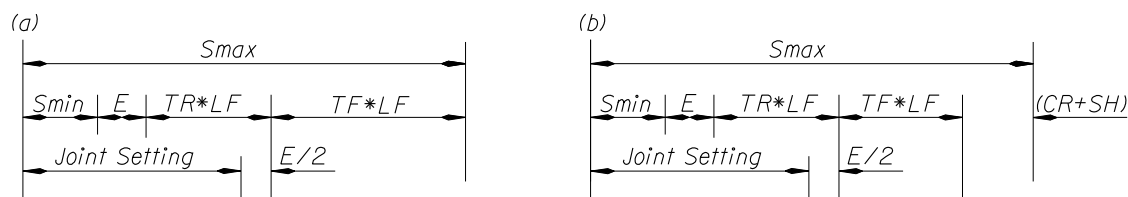
Figure 1.14.2.3-2 Joint Setting Schematic
