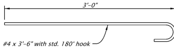
Figure 1.5.5.18-1 Specified Length of Bar with Hook
