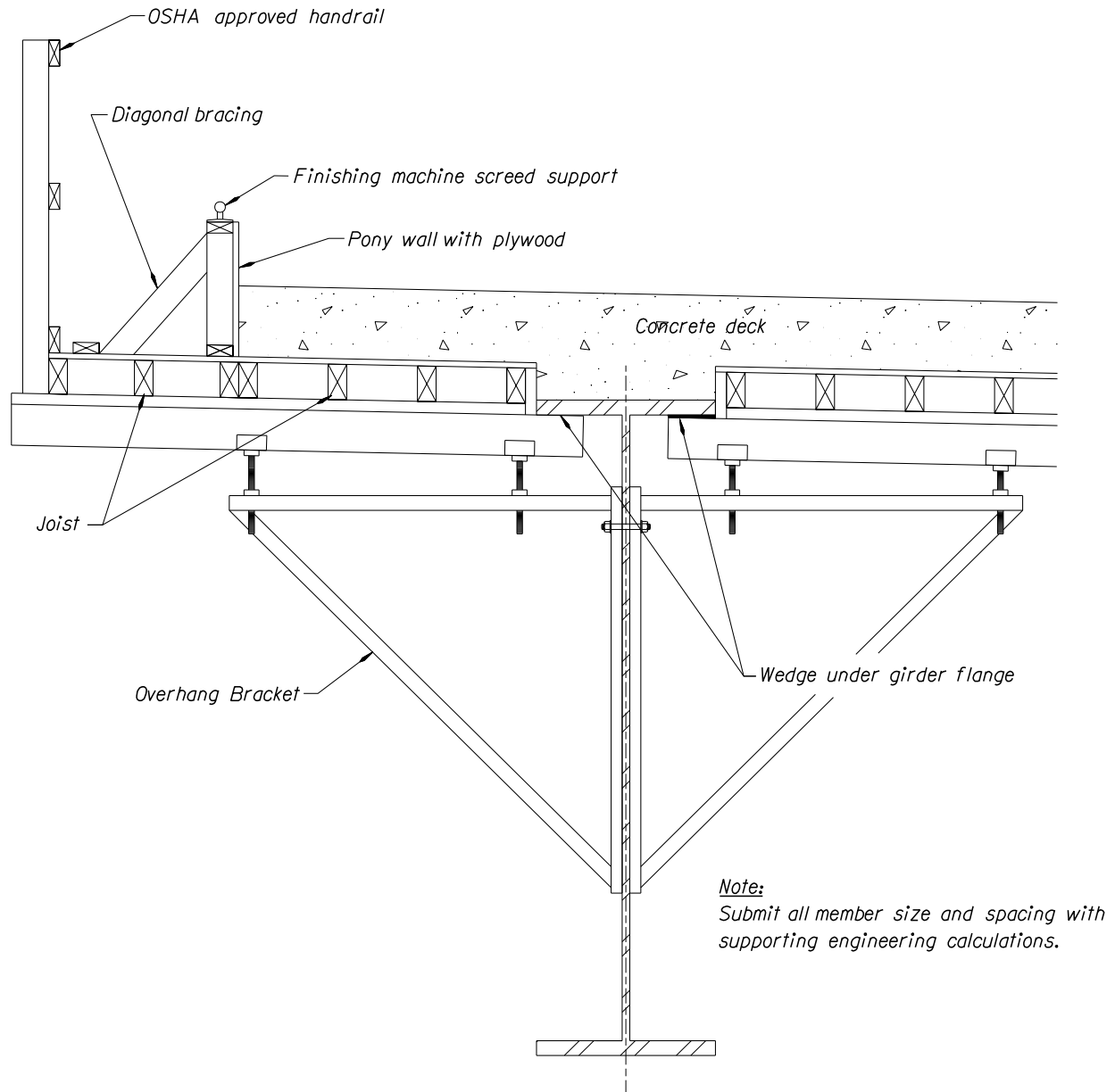
Figure 1.16.3.3.2-2 – Typical Deck Forming Detail
