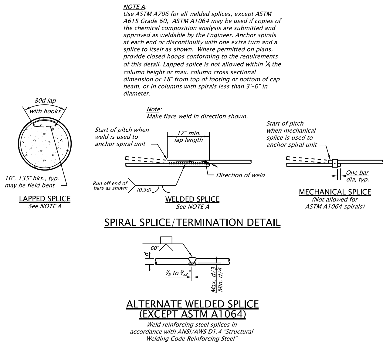
Figure 1.11.3.6-2 Spiral Splice and Termination Detail
