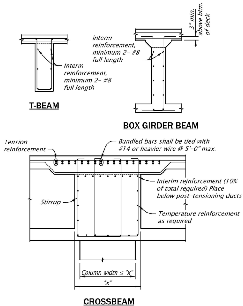
Figure 1.5.5.19-1 Interim Reinforcement
