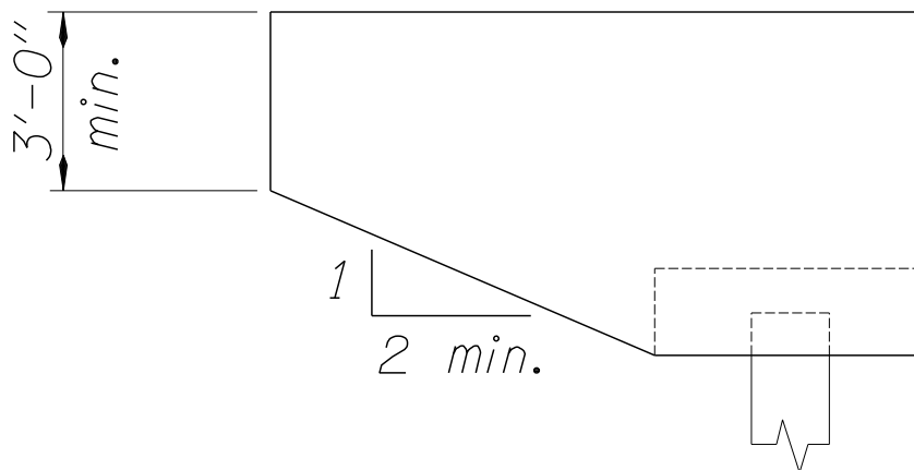
Figure 1.11.2.3-2 Wingwall Slopes
