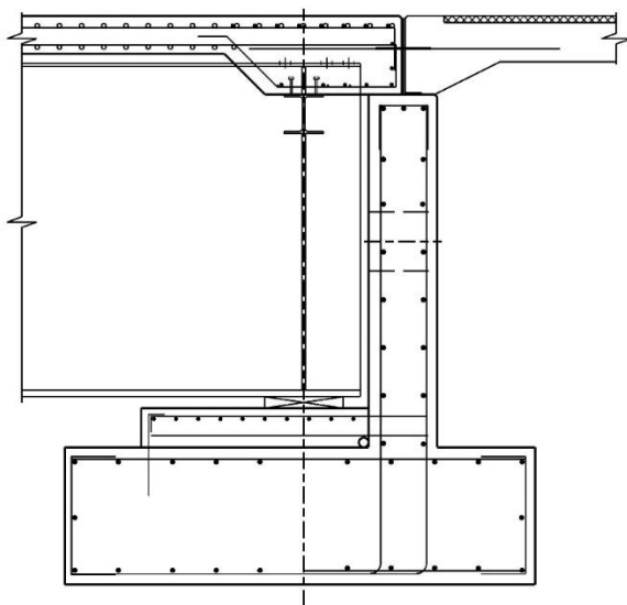
Figure 1.6.2.15-1 Extended Deck Details at End Bents
