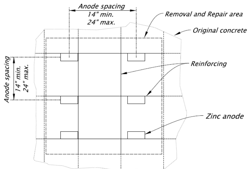
Figure 1.15.2.1.3-1 Anode Puck General Placement
