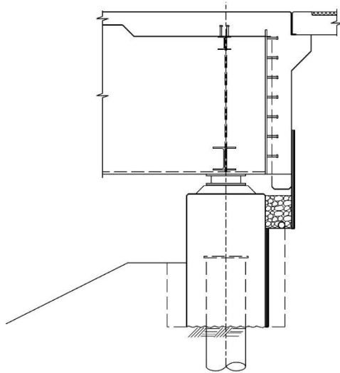
Figure 1.6.2.15-2 Semi Integral Bent Detail
