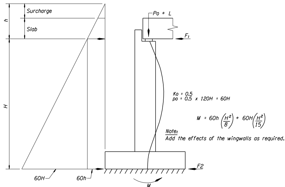
Figure 1.11.2.7-1 Strutted Abutment Loading
