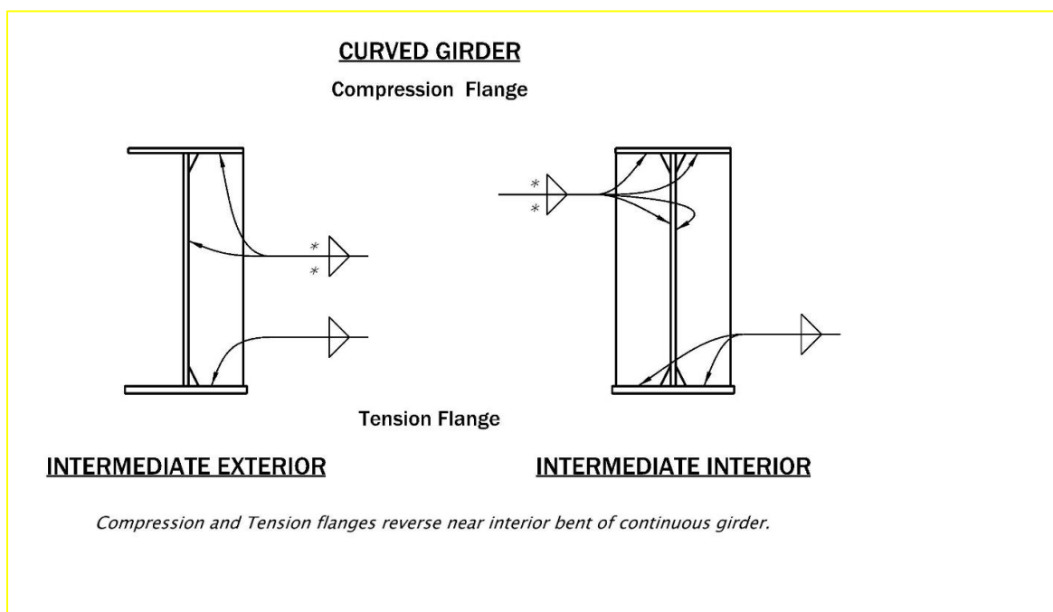
Figure 1.6.2.10-3 Transverse Connection Plates on Curved Girders
