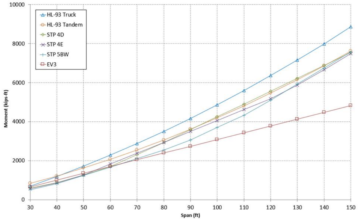
Figure 1.3.3.1-1 Live Load Plus Impact for Single Span Prismatic Members – Bending Moment at Mid-Span, (span lengths 30 – 150 feet)
