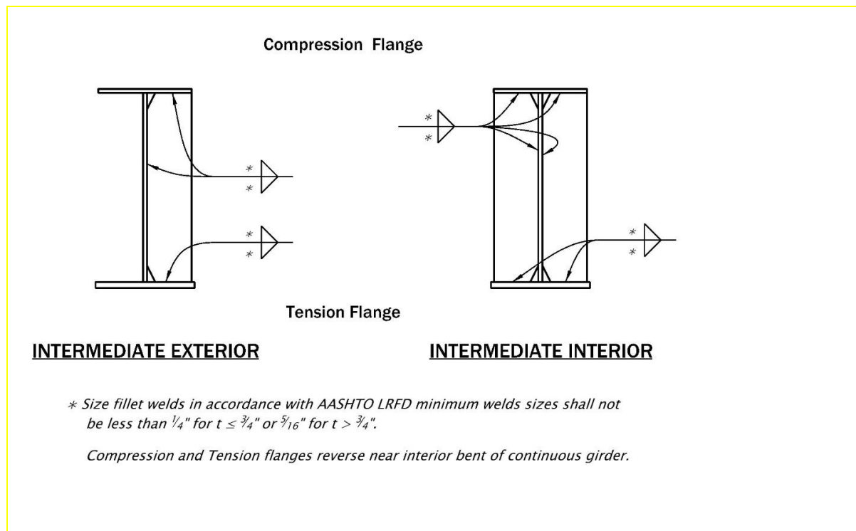
Figure 1.6.2.10-3 Transverse Connection Plates on Curved Girders
