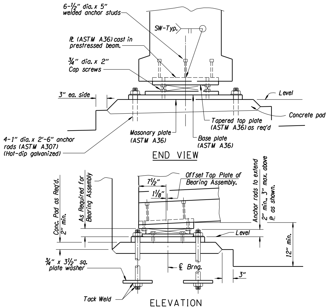
Figure 1.14.1.3-2 Schematic of Bearing Showing Attachment
