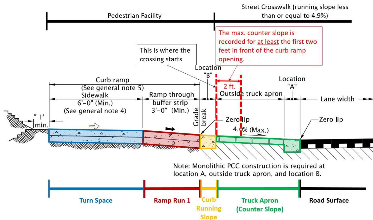
Truck Apron Detail from RD170, Roundabout and Truck Apron Curb Placement. Note Design Counter Slope is 4% Max. but Finished Counter Slope has a Maximum of 4.9%
