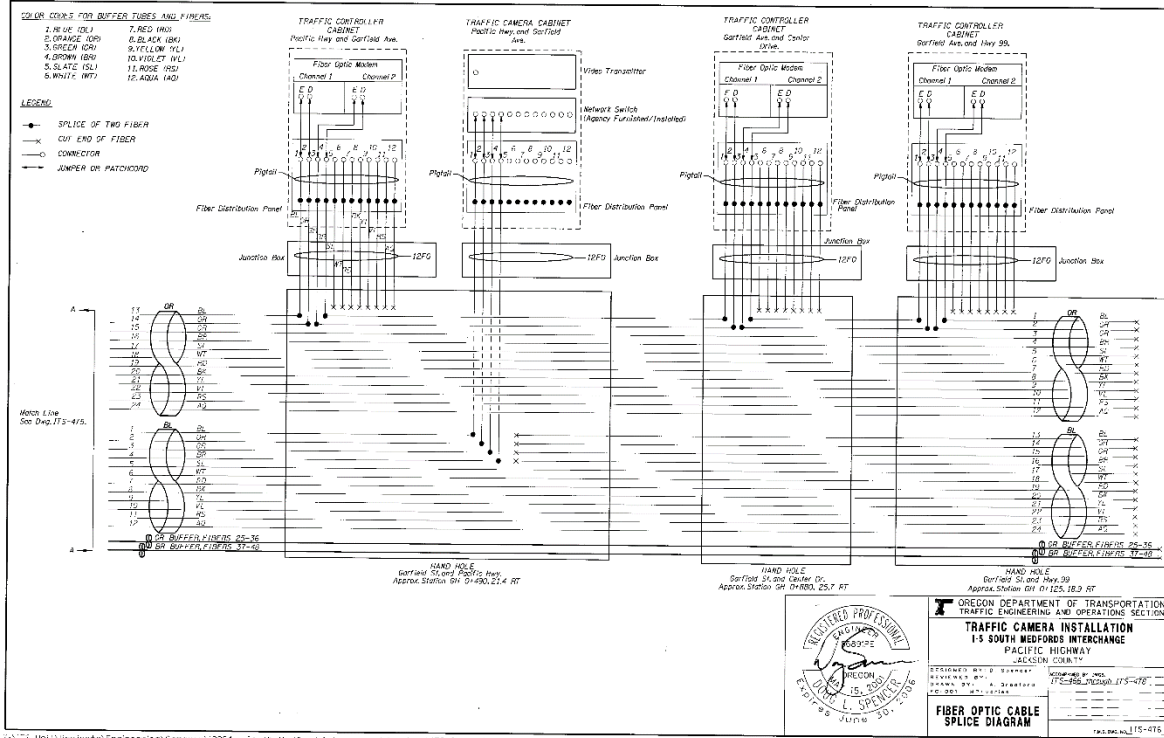
Figure 7-2 | Fiber Optic Installation – Example of Fiber Optic Cable Splice Diagram created by the ITS Unit
