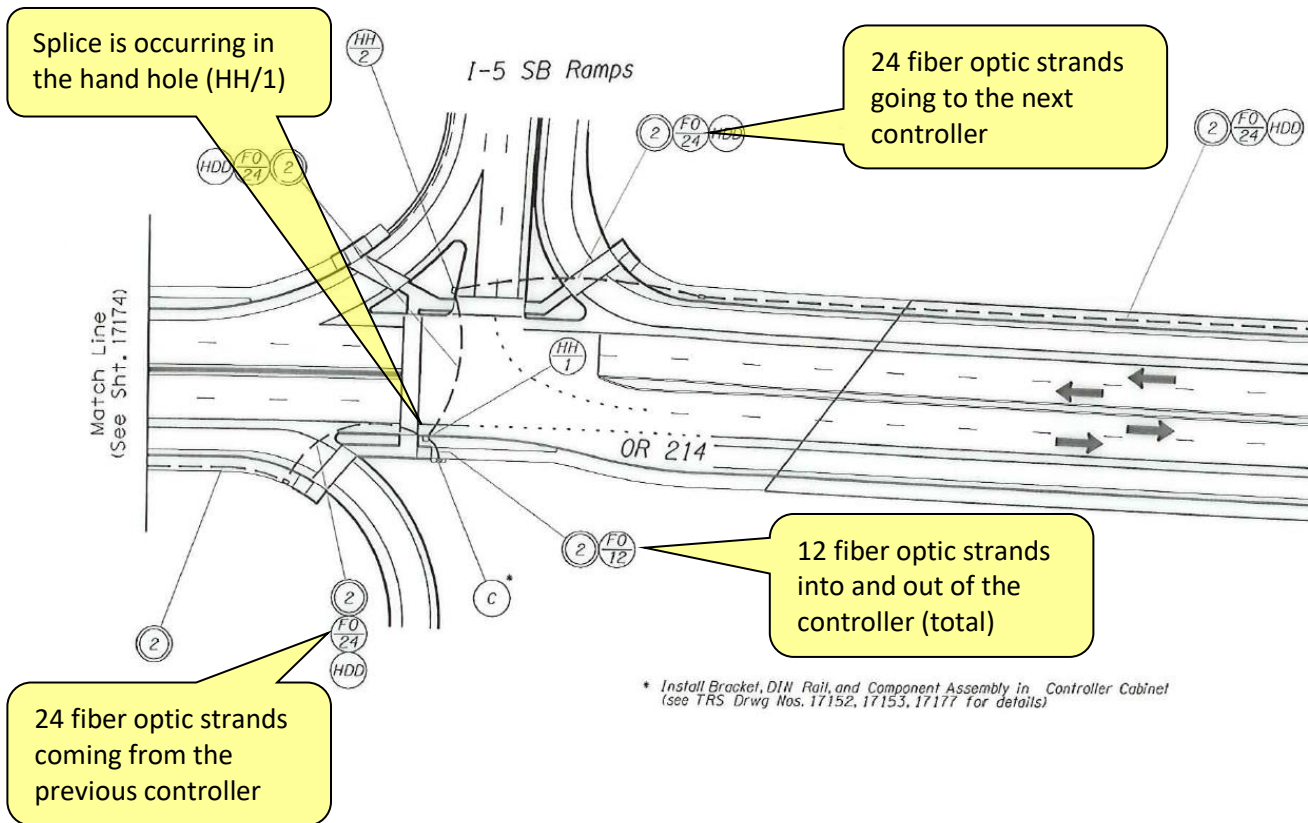
Figure 7-1 | Fiber Optic Installation – Example of Interconnect Plan created by the Signal Designer
