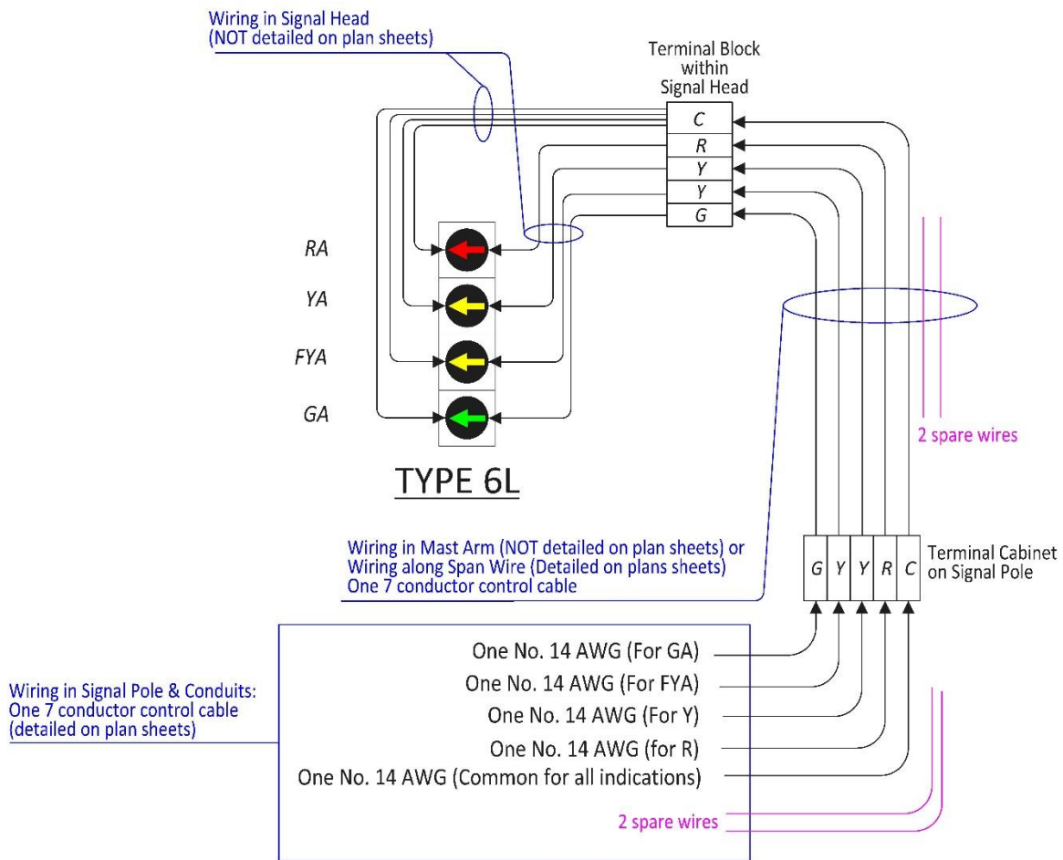
Figure 5-125 | Wiring for Type 6L Signal Head
