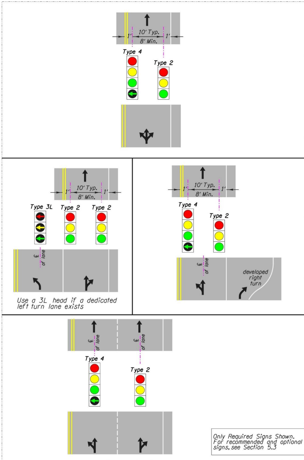
Figure 5-39 | Signal Head Placement for Split Phasing
