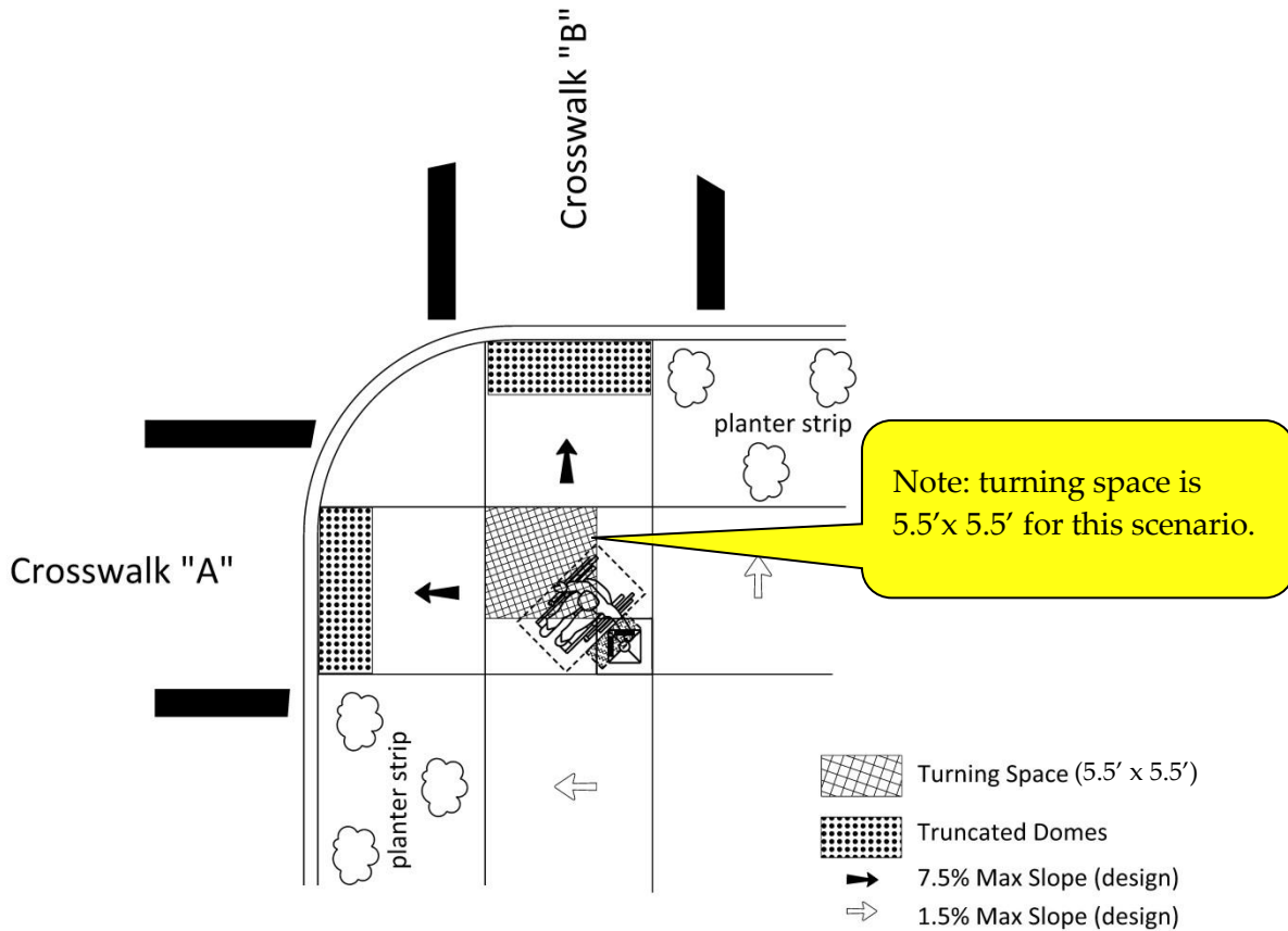
Figure 5-83 | Preferred Pushbutton Placement for Two Curb Ramps That Share a Turning Space (Two Buttons on Pedestal)
