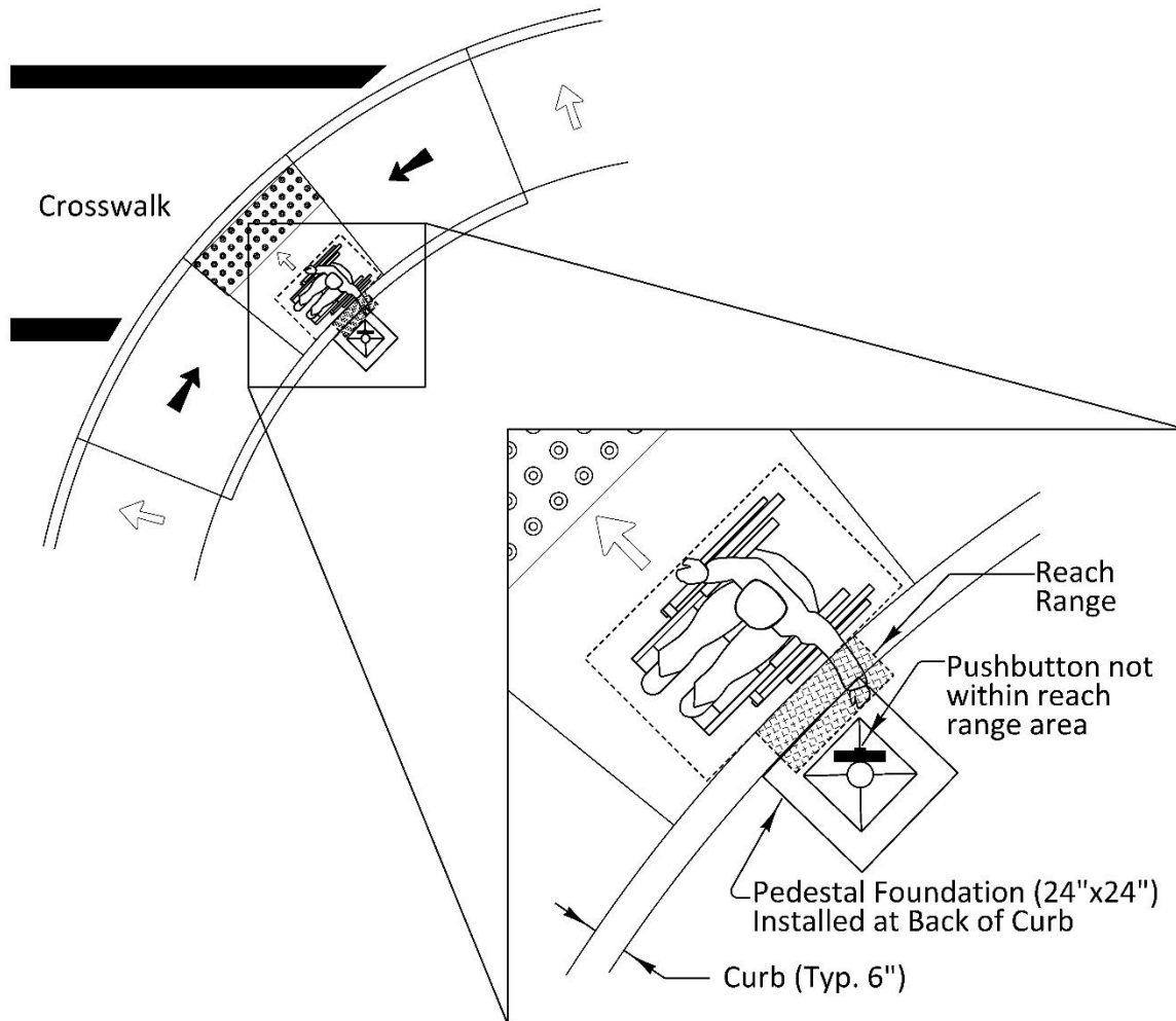
Figure 5-56 | Pedestals Located Behind Curbs Do NOT Meet 10 Inch Horizontal Reach Requirement
