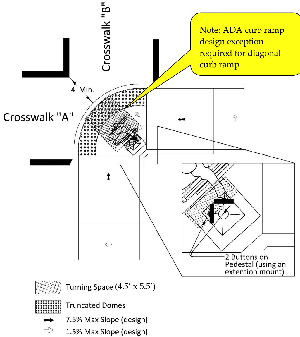
Figure 5-86 | Preferred Pushbutton Placement for Diagonal Parallel Style Curb Ramp (Two Buttons on Pedestal) – Example 2
