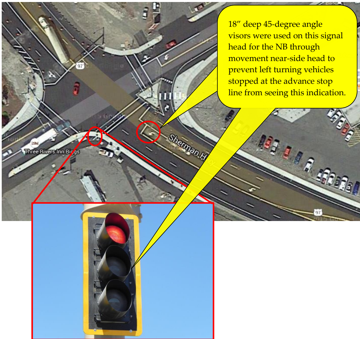
Figure 5-50 | Cut-Off Visor Example
