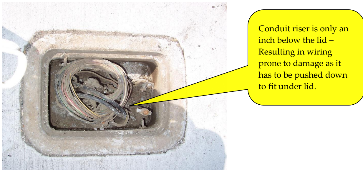
Figure 5-111 | Impacts from Raising Elevation Without Adjusting Junction Box
