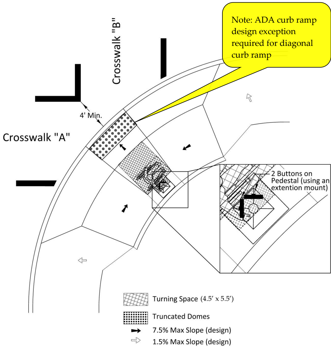
Figure 5-87 | Preferred Pushbutton Placement for Diagonal Combo Style Curb Ramp (Two Buttons on Pedestal)
