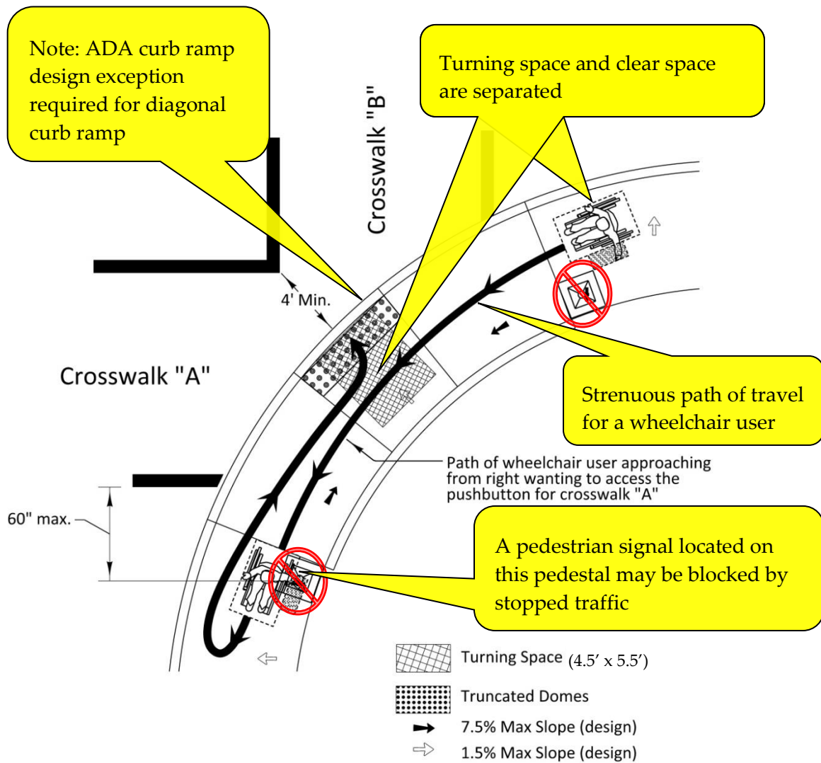
Figure 5-81 | Drawbacks to the 10-foot Separation of Pushbuttons at Diagonal Curb Ramps
