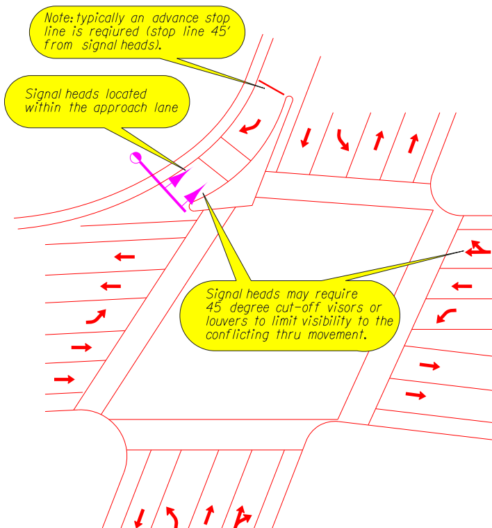
Figure 5-34 | Signal Head Placement for Right Turn Phases –Right Turn Slip Lanes
