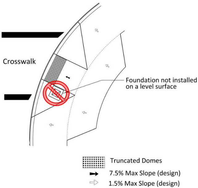
Figure 5-61 | Pedestal Foundation Placement – Example 1
