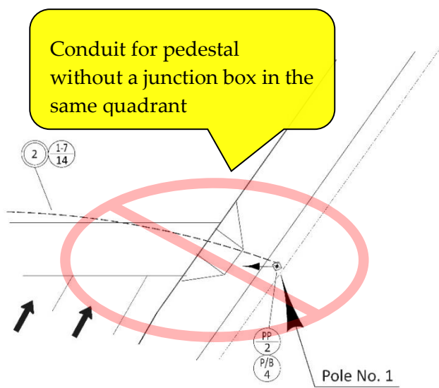
Figure 5-119 | Conduit Routing to Pedestal Not Located in Same Quadrant as Large Pole – Avoid This Method
