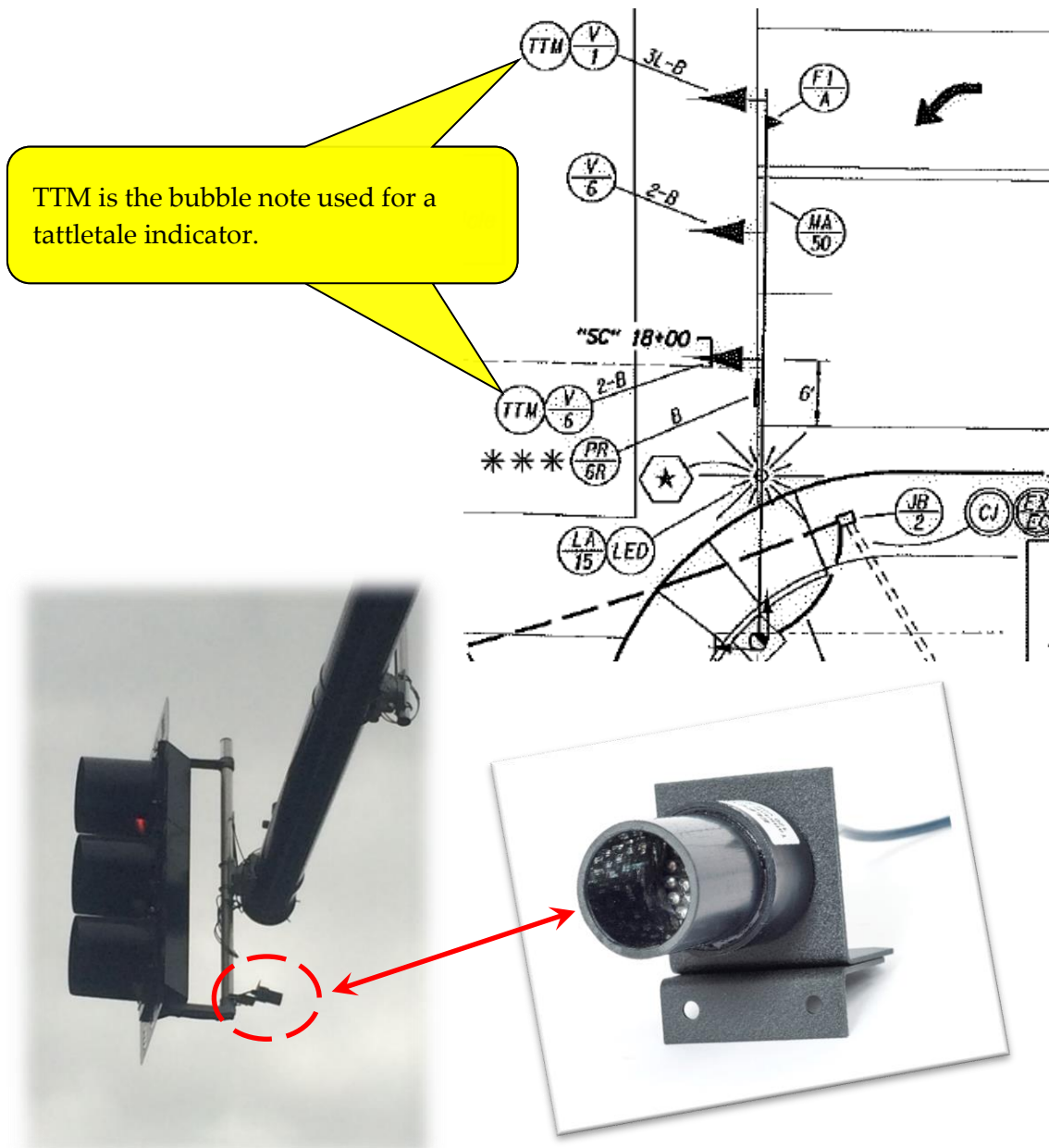
Figure 5-51 | Tattletale Indicator Example
