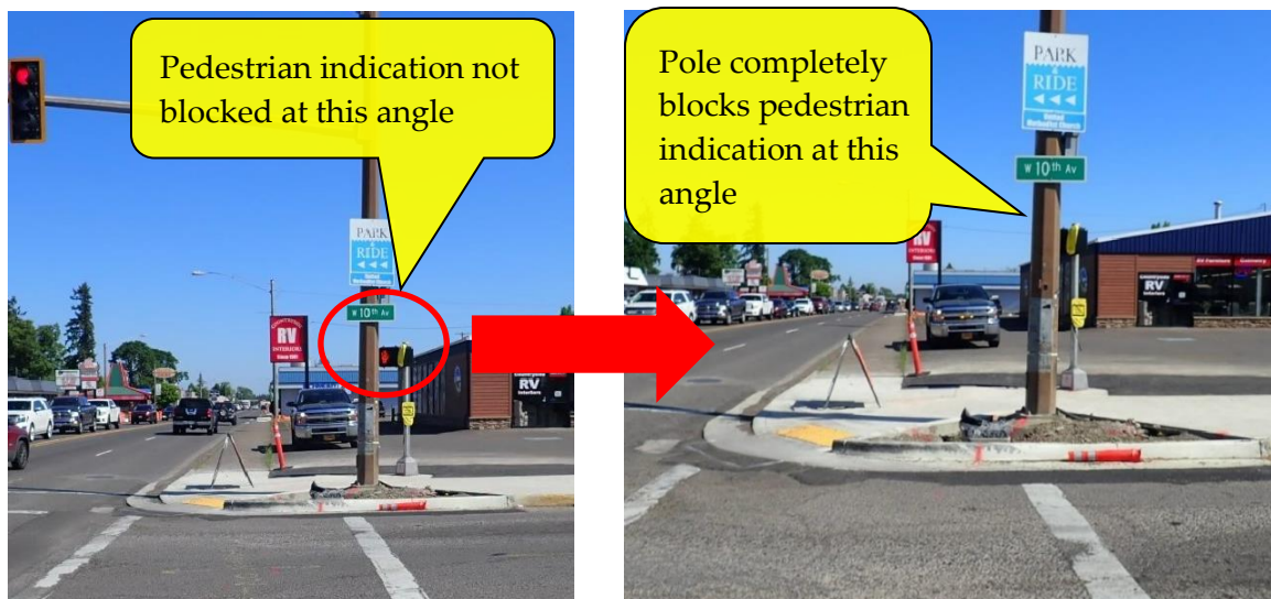
Figure 5-98 | Poor Pedestrian Signal Visibility
