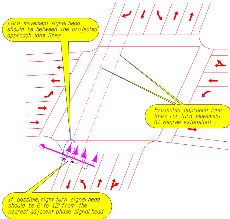
Figure 5-34 | Signal Head Placement for Right Turn Phases –Right Turn Slip Lanes
