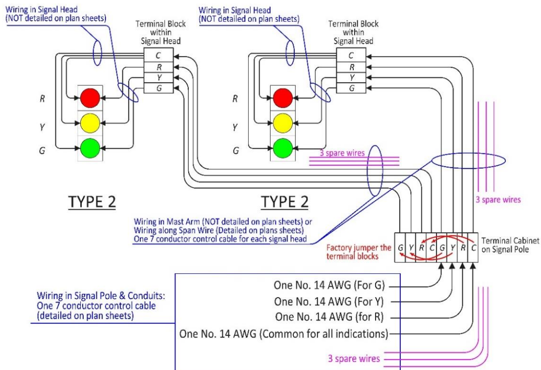
Figure 5-130 | Wiring Multiple Signal Heads for the Same Phase on the Same Pole
