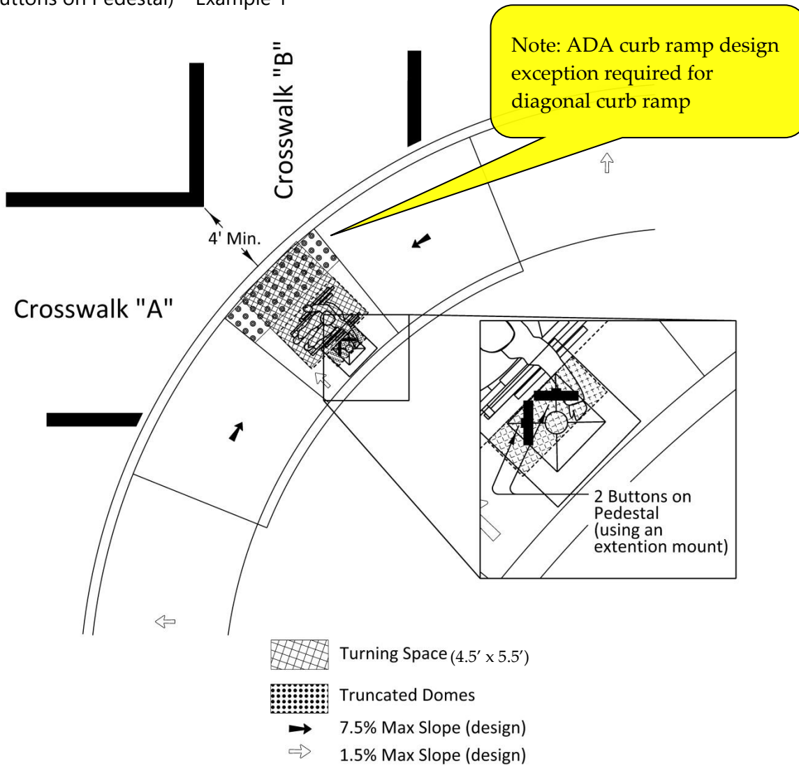
Figure 5-85 | Preferred Pushbutton Placement for Diagonal Parallel Style Curb Ramp (Two Buttons on Pedestal) – Example 1
