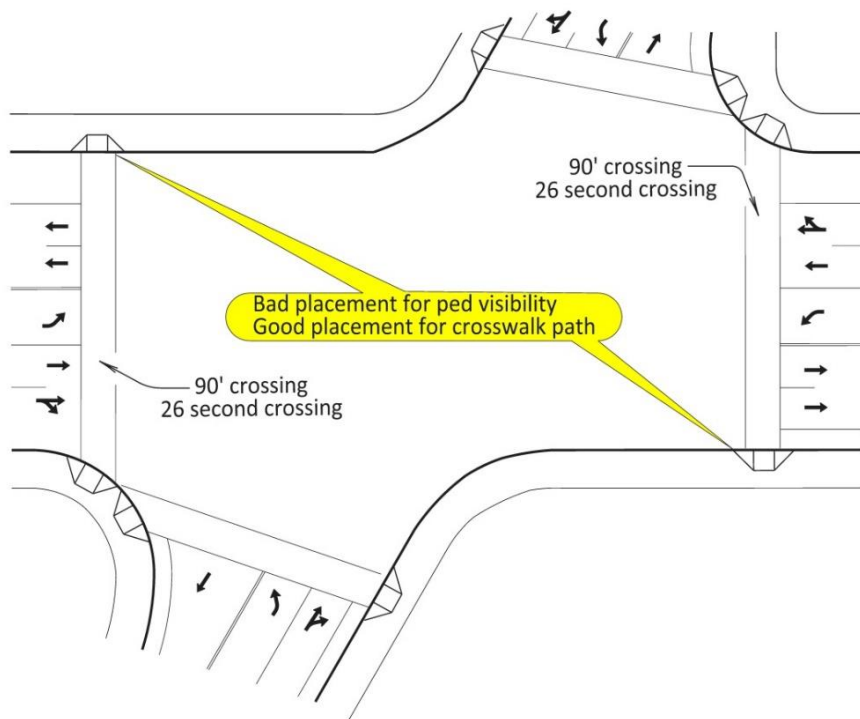
Figure 5-7 | Crosswalk Example 2
