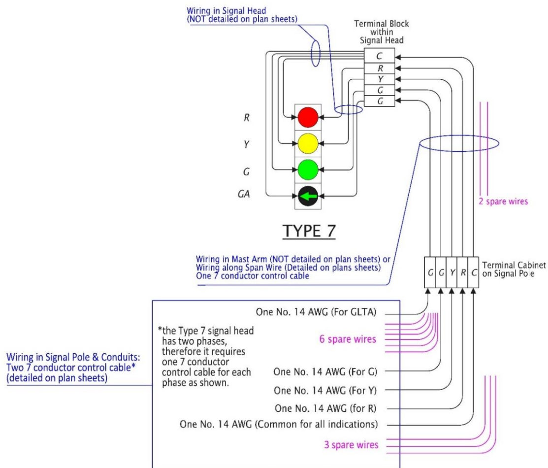
Figure 5-126 | Wiring for Type 7 Signal Head
