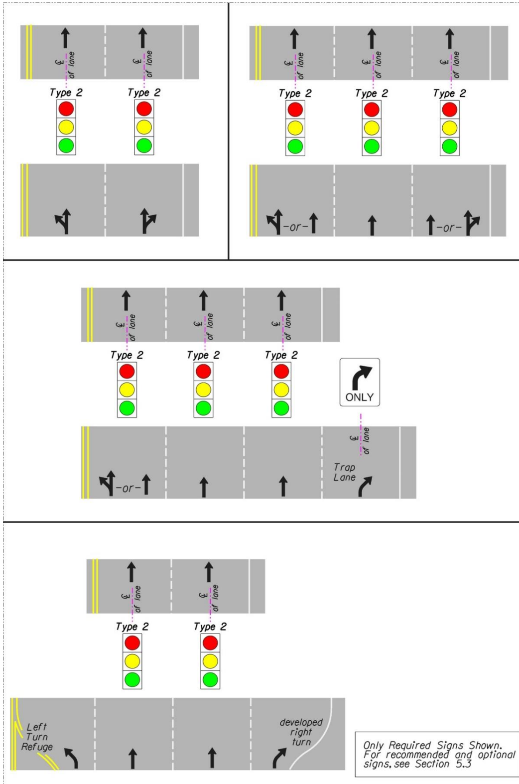
Figure 5-36 | Signal Head Placement for Lanes Sharing the Same Phase (cont.)
