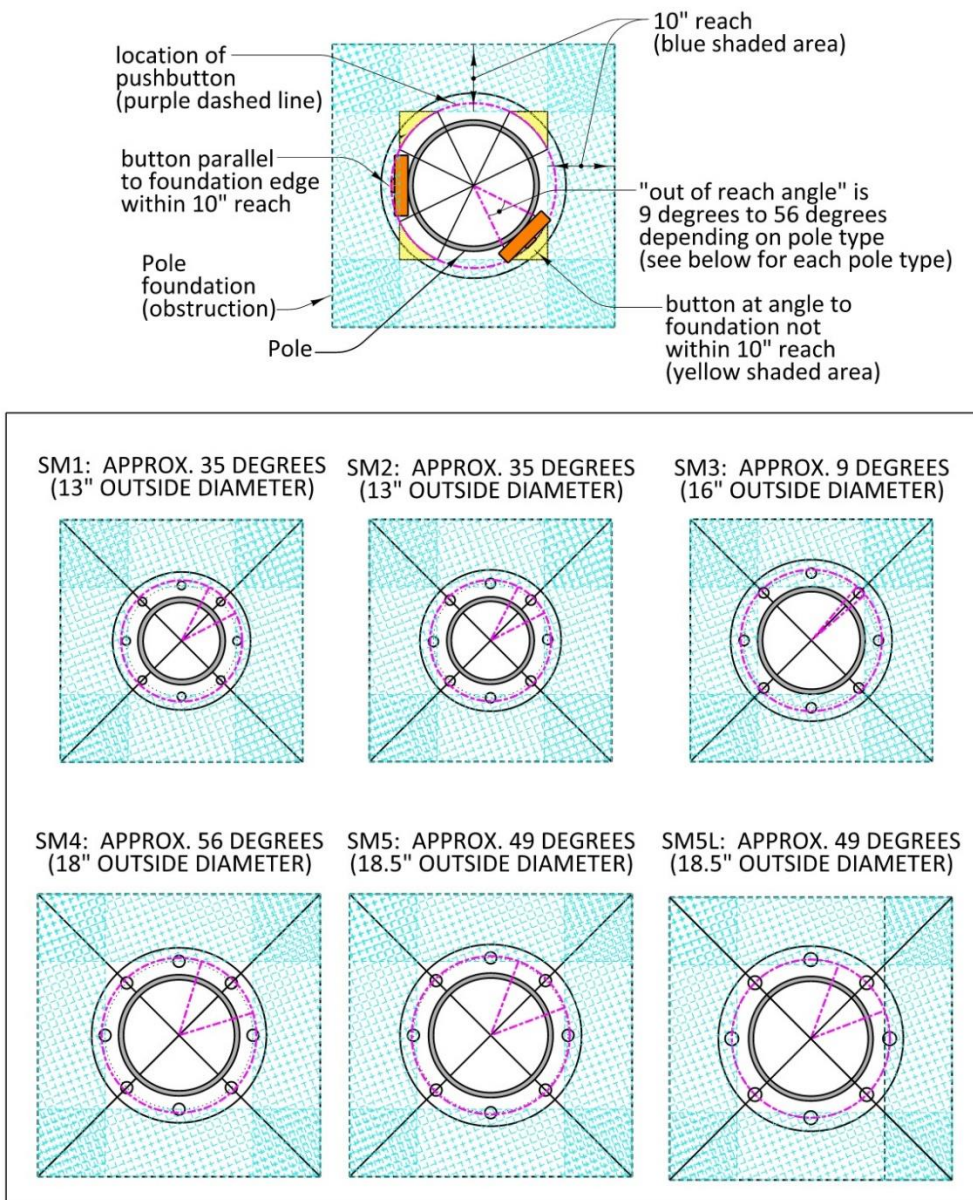
Figure 5-80 | Out-of-Reach Angle for Pushbuttons Located on Large Poles (POLES CONSTRUCTED BEFORE JANUARY 2020)
