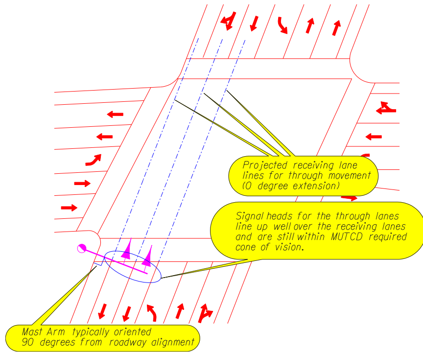
Figure 5-29 | Signal Head Placement For Through Movement Using Projected Lane Lines (INCORRECT METHOD)
