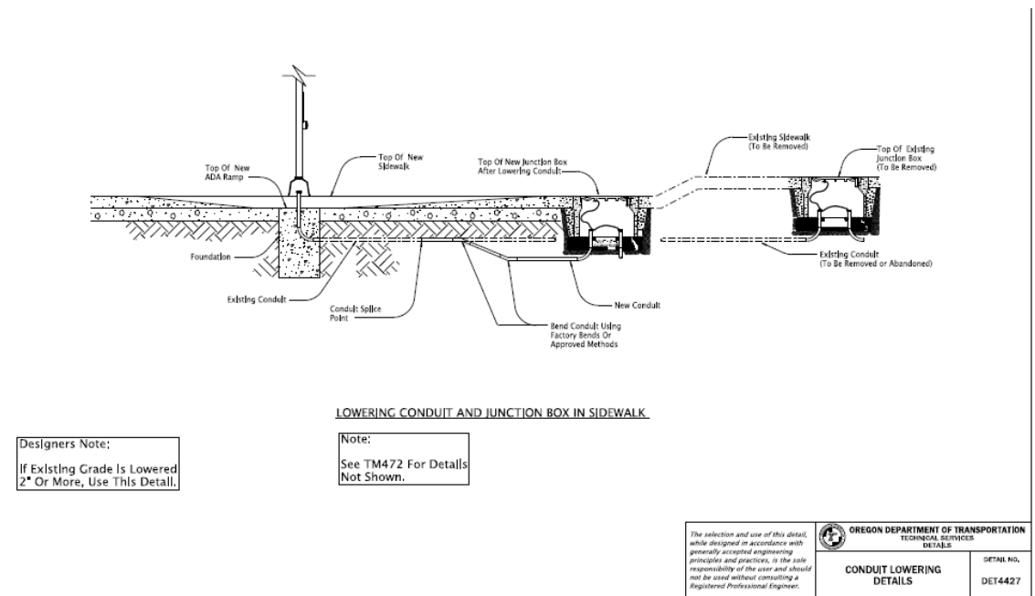
Figure 5-112 | DET4427 – Conduit Lowering Details
