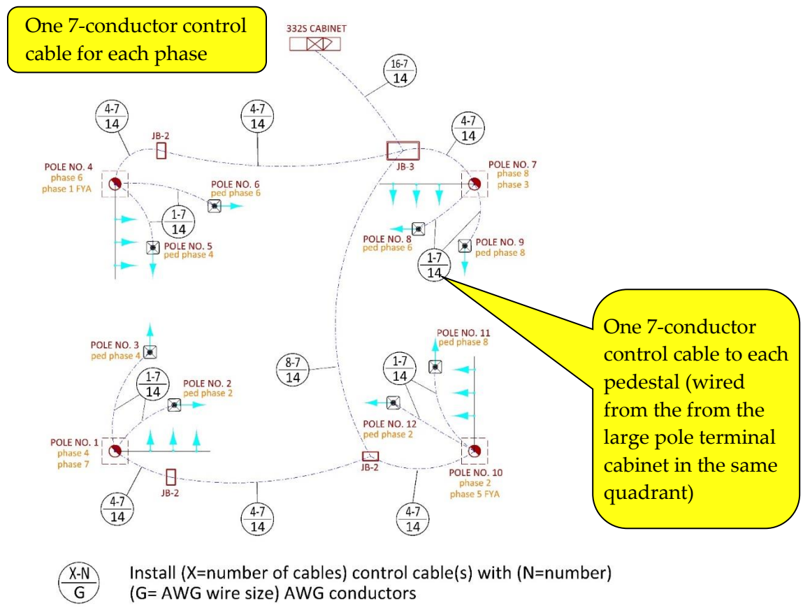
Figure 5-132 | Wiring Phases with Control Cables
