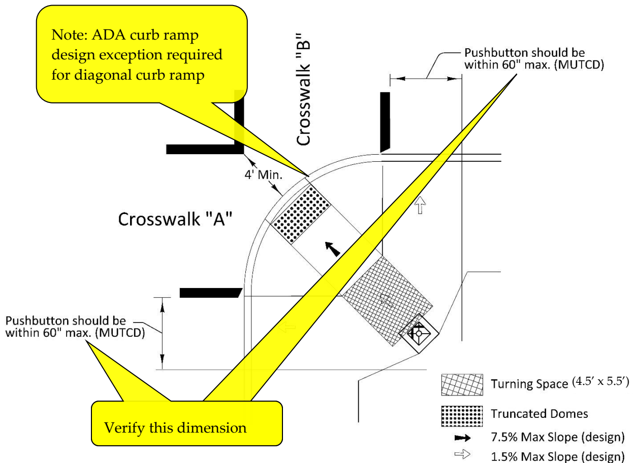
Figure 5-88 | Pushbutton 60” From Outside Edge of Crosswalk Striping at Diagonal Curb Ramp
