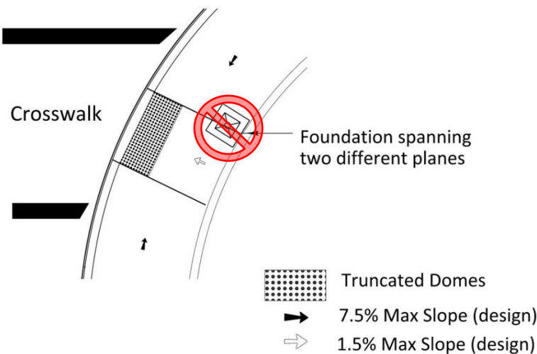
Figure 5-62 | Pedestal Foundation Placement – Example 2
