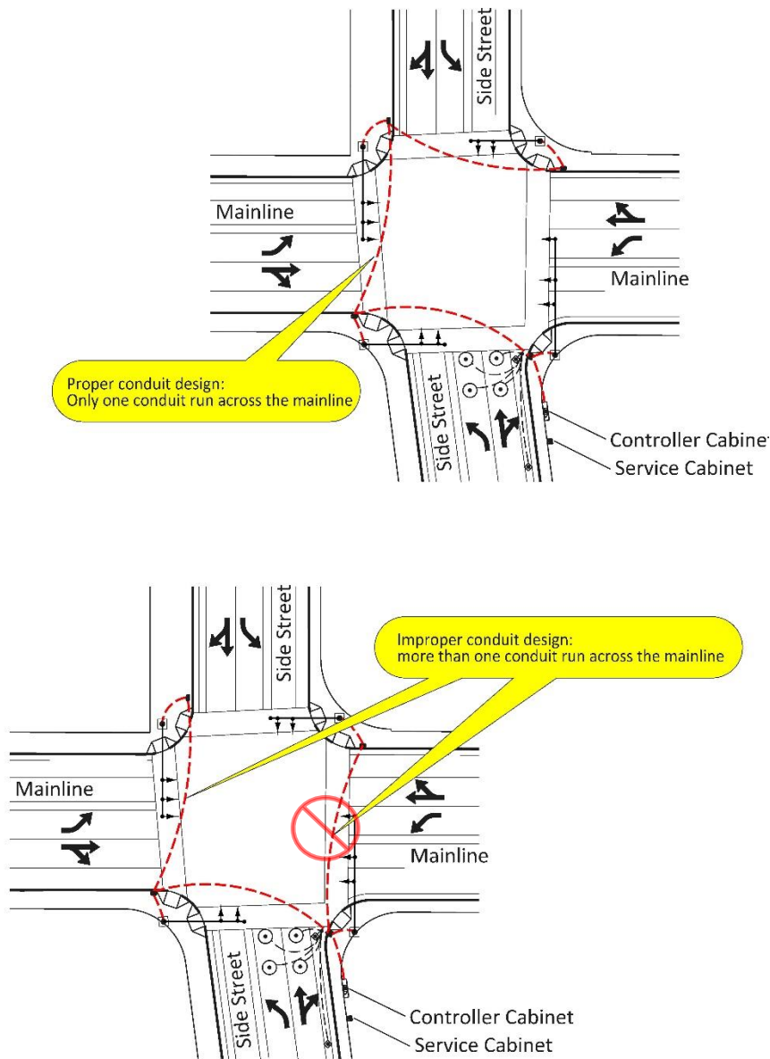
Figure 5-113 | General Conduit Layout
