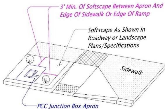
Figure 5-109 | ADA Softscaping Requirements for Junction Box PCC Apron
