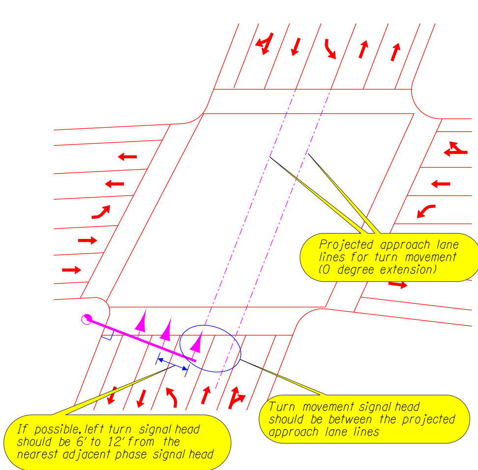
Figure 5-32 | Signal Head Placement for Left Turn Phases Using Projected Lane Lines
