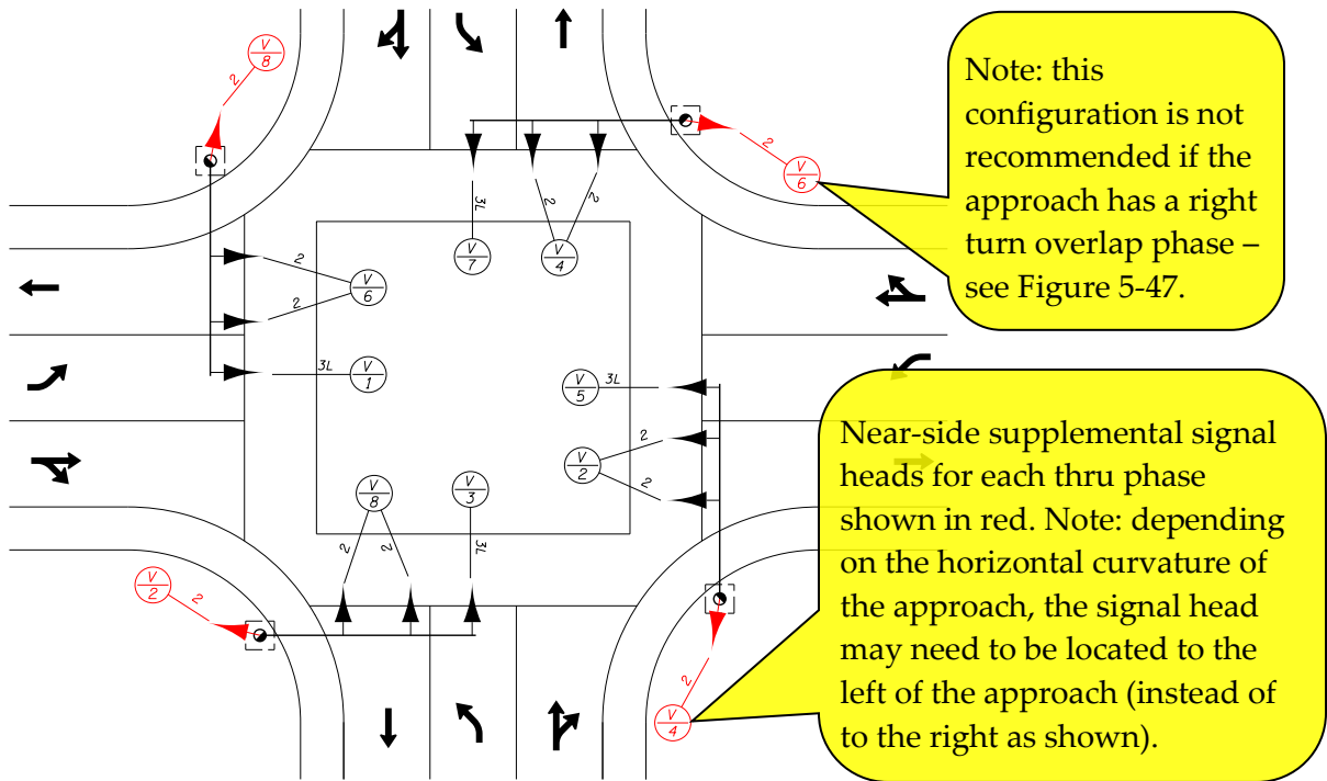
Figure 5-43 | Supplemental Near-Side Signal Heads – Typical Placement for Left Turn Phase
