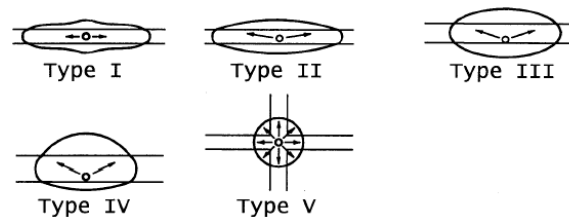
Figure 5-103 | Illumination Engineering Society (IES) Light Distribution Patterns
