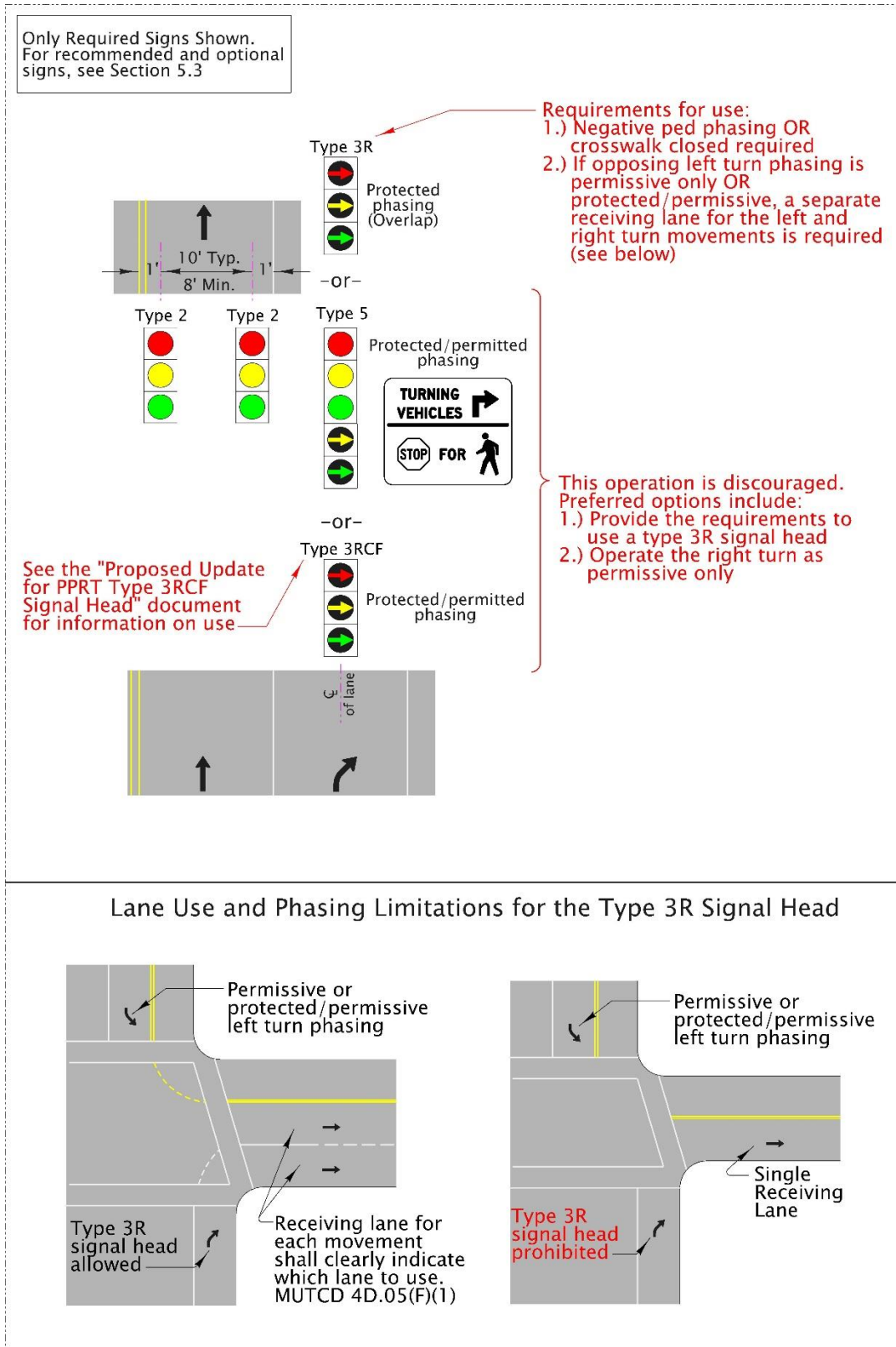
Figure 5-38 | Signal Head Placement for Right Turn Phasing
