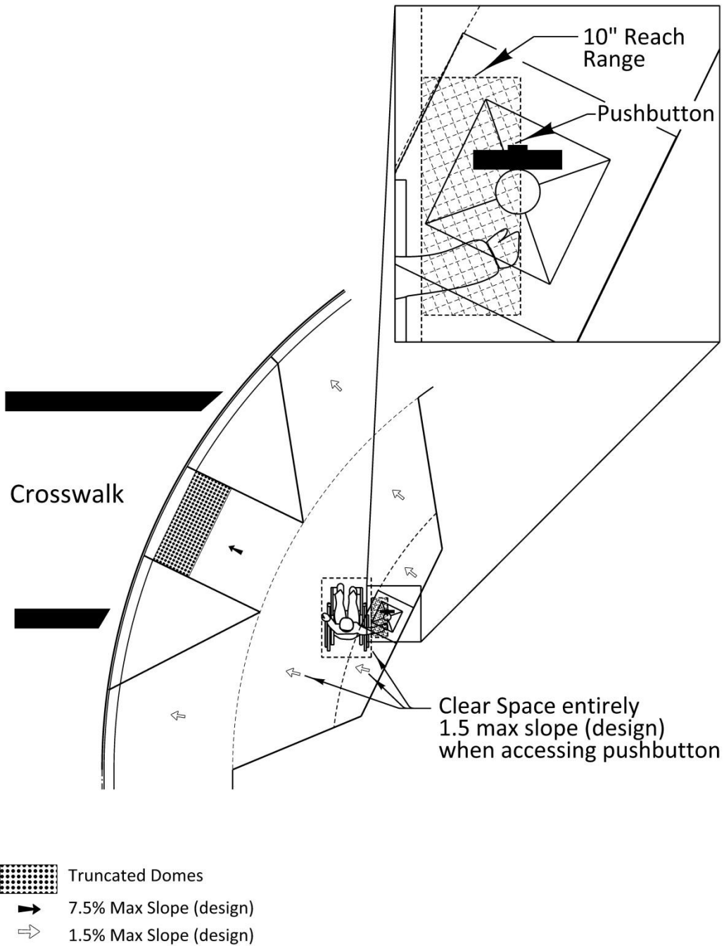
Figure 5-68 | Accessing the Pushbutton – Clear Space within 1.5% Slope (design), Example 2
