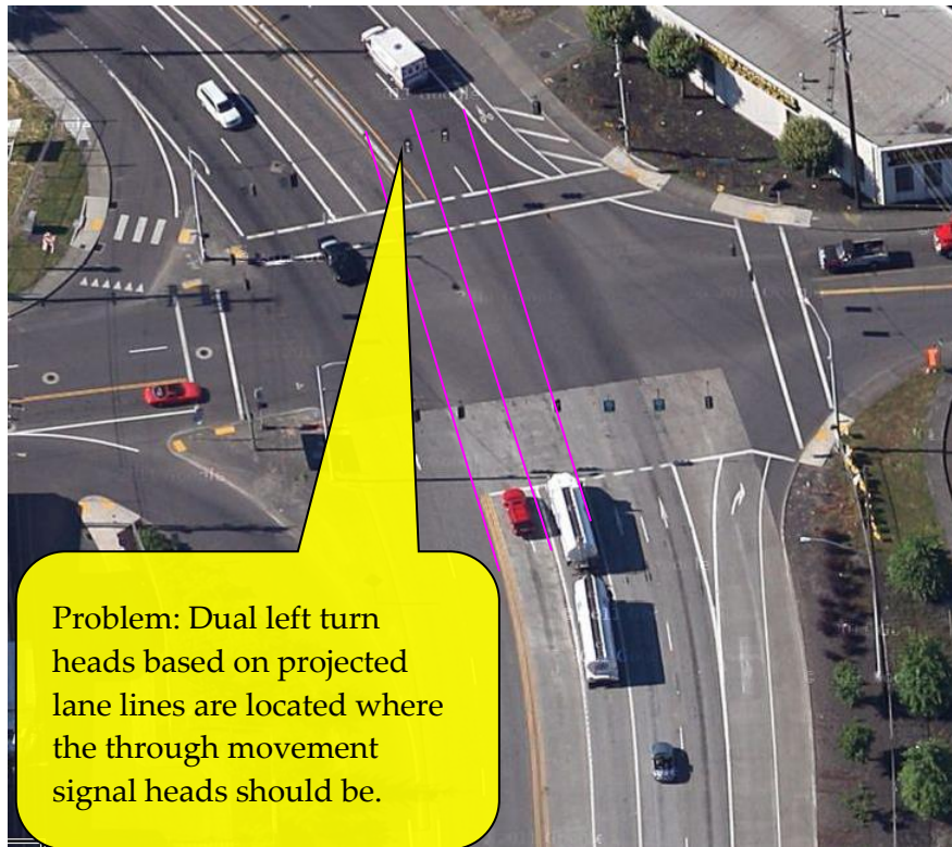
Figure 5-30 | Horizontal Curves and Signal Head Alignment, Example 1
