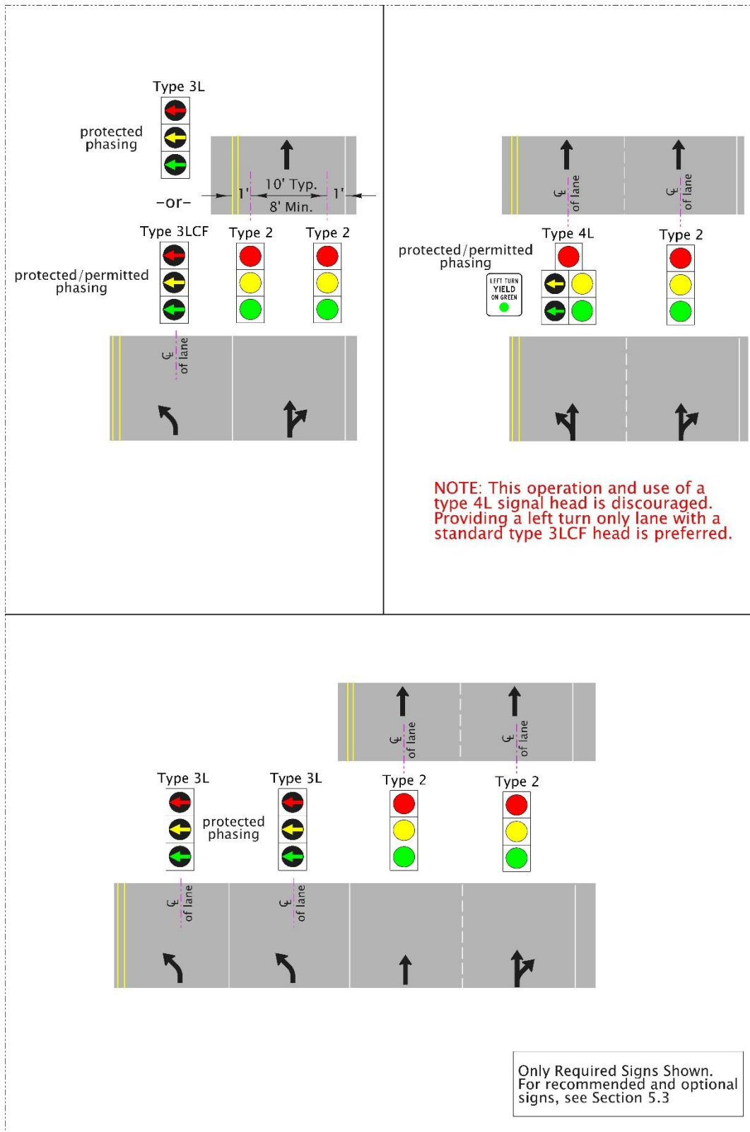
Figure 5-37 | Signal Head Placement for Left Turn Phasing
