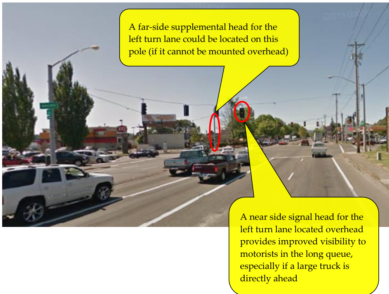
Figure 5-48 | Supplemental near-side signal head placement: Example 3
