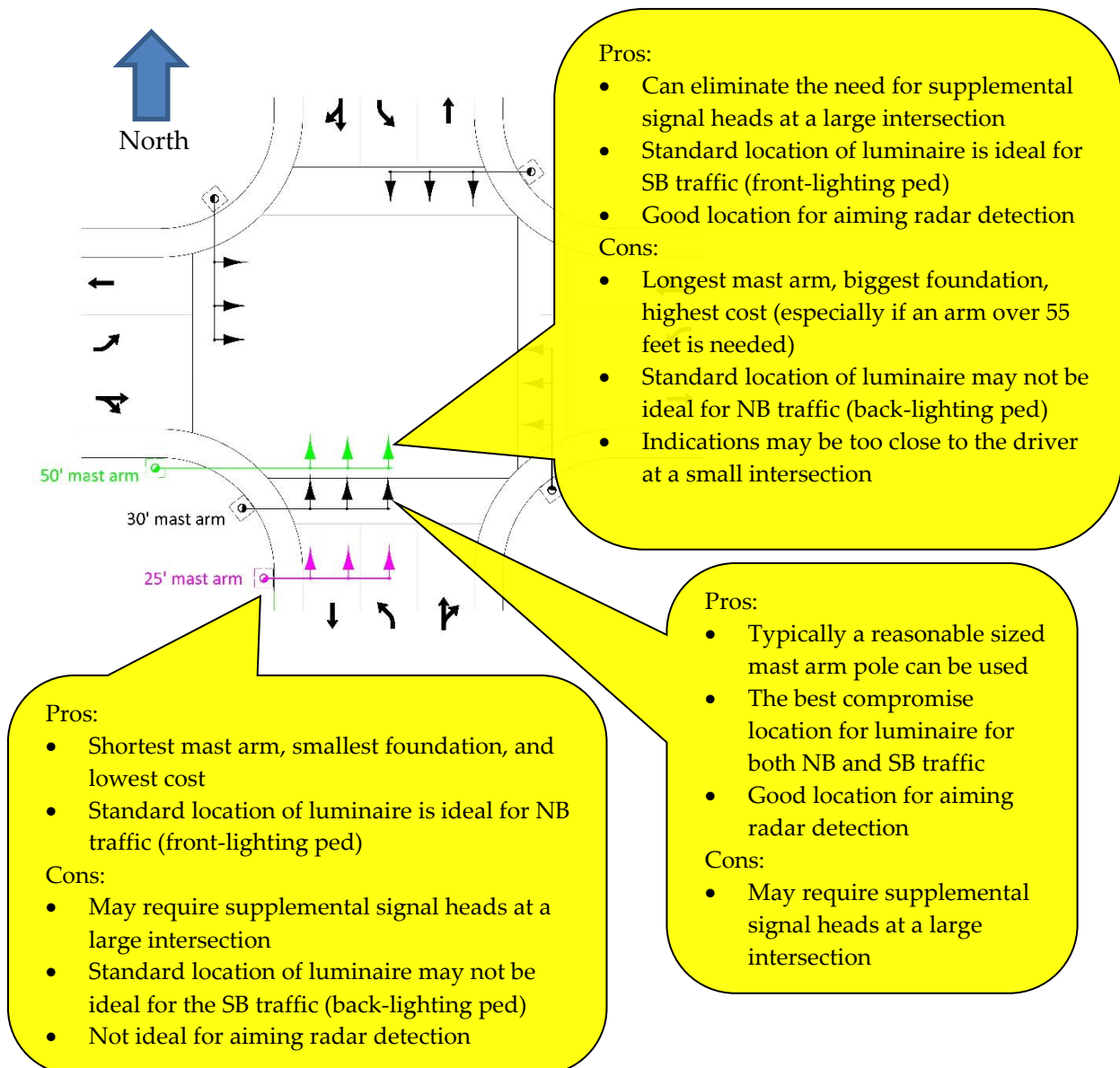
Figure 5-102 | Typical Mast Arm Pole Locations (Pros and Cons)
