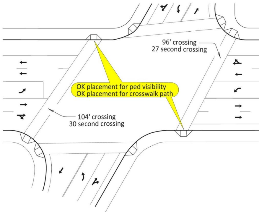
Figure 5-8 | Crosswalk Example 3
