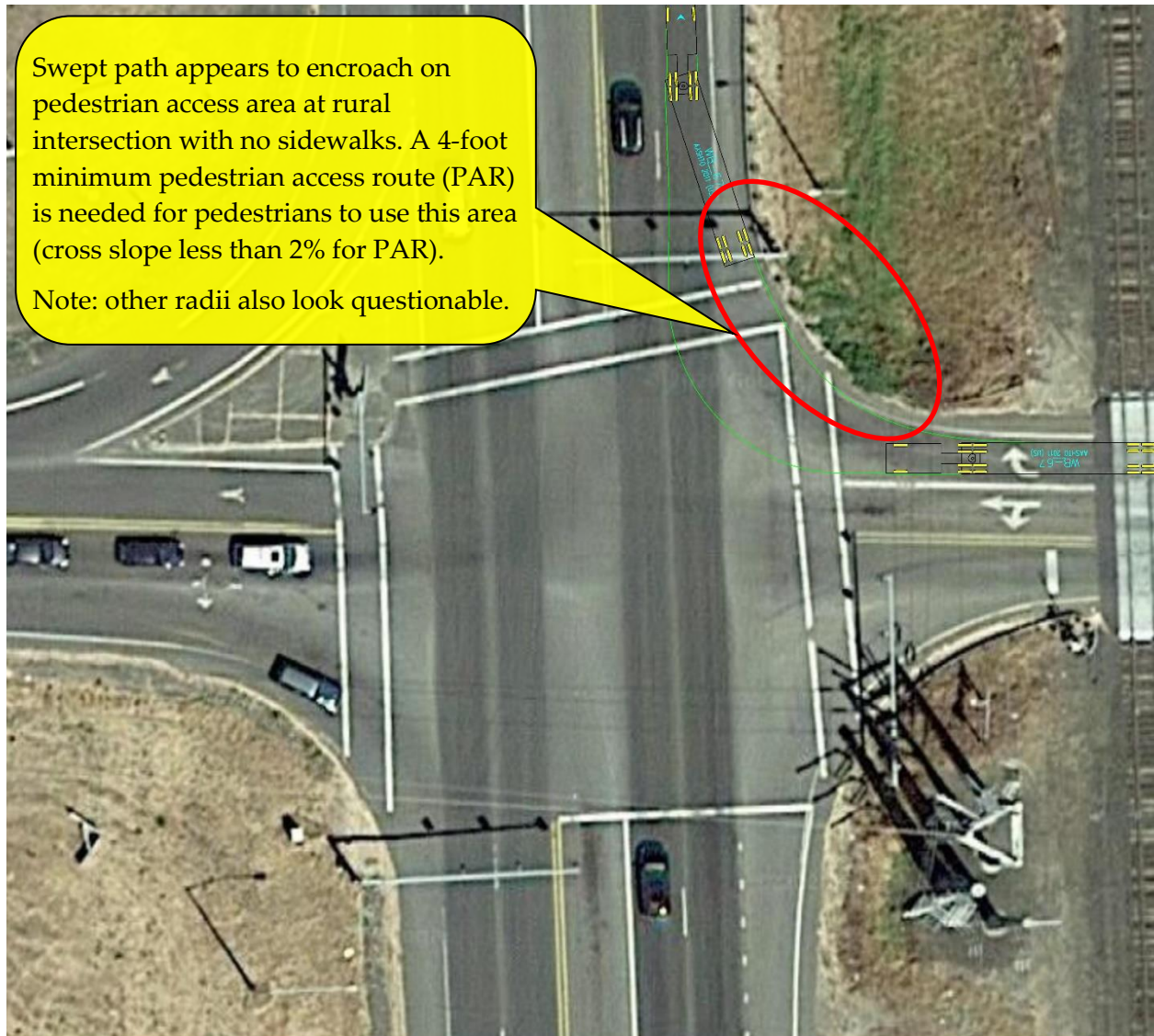
Figure 5-21 | Truck Turning Templates – Verifying Right Turns
