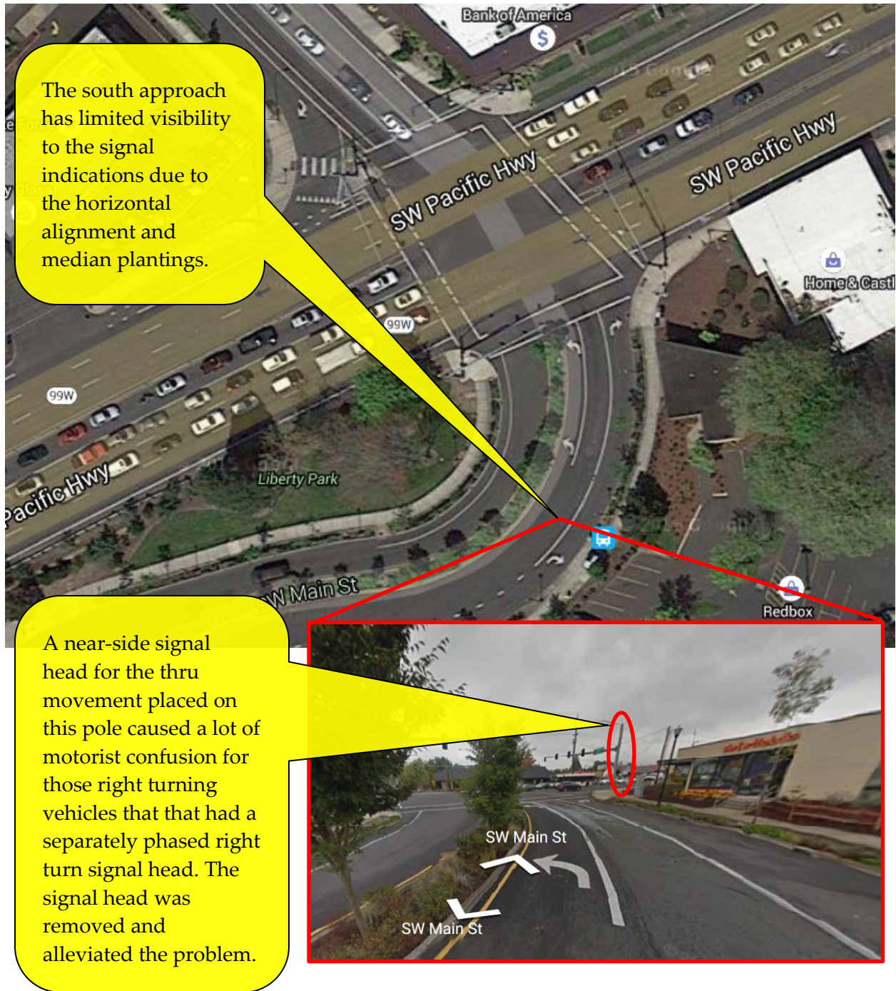
Figure 5-47 | Supplemental near-side signal head placement: Example 2
