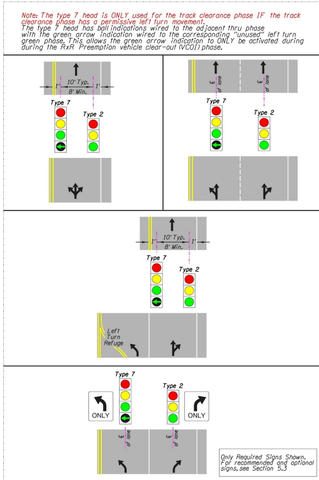
Figure 5-41 | Signal head Placement for Railroad Preemption
