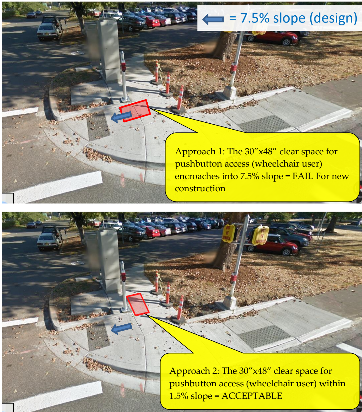
Figure 5-71 | Multiple Ways to Parallel Approach the Pushbutton
