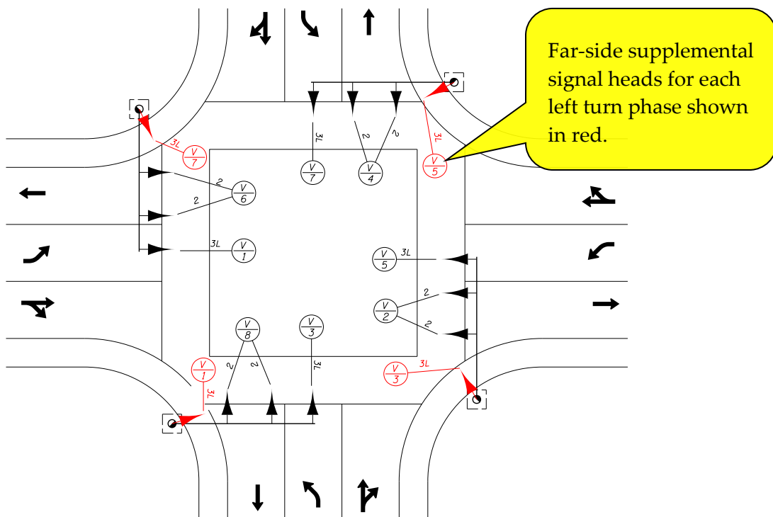
Figure 5-45 | Supplemental Far-Side Signal Heads – Typical Placement for Left Turn Phase
