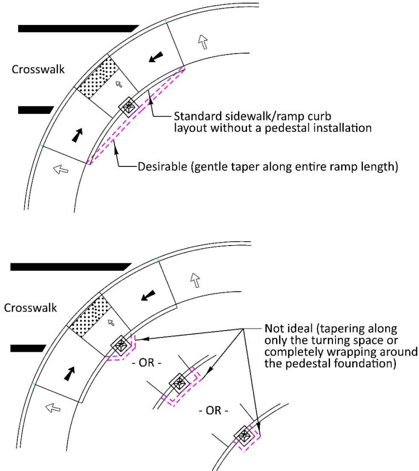
Figure 5-60 | Pedestal with Curb Around Foundation – Examples of Desirable and Not Ideal Curb Layouts
