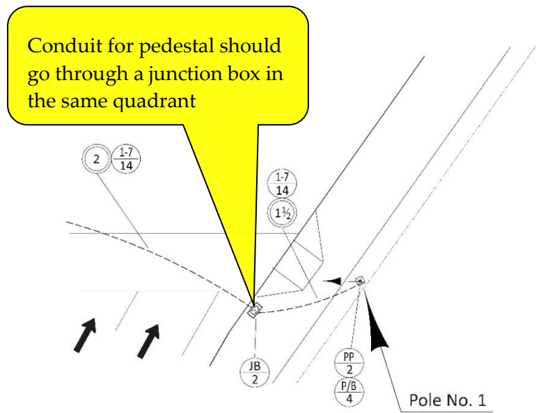
Figure 5-118 | Conduit Routing to Pedestal Not Located in Same Quadrant as Large Pole – Preferred Method
