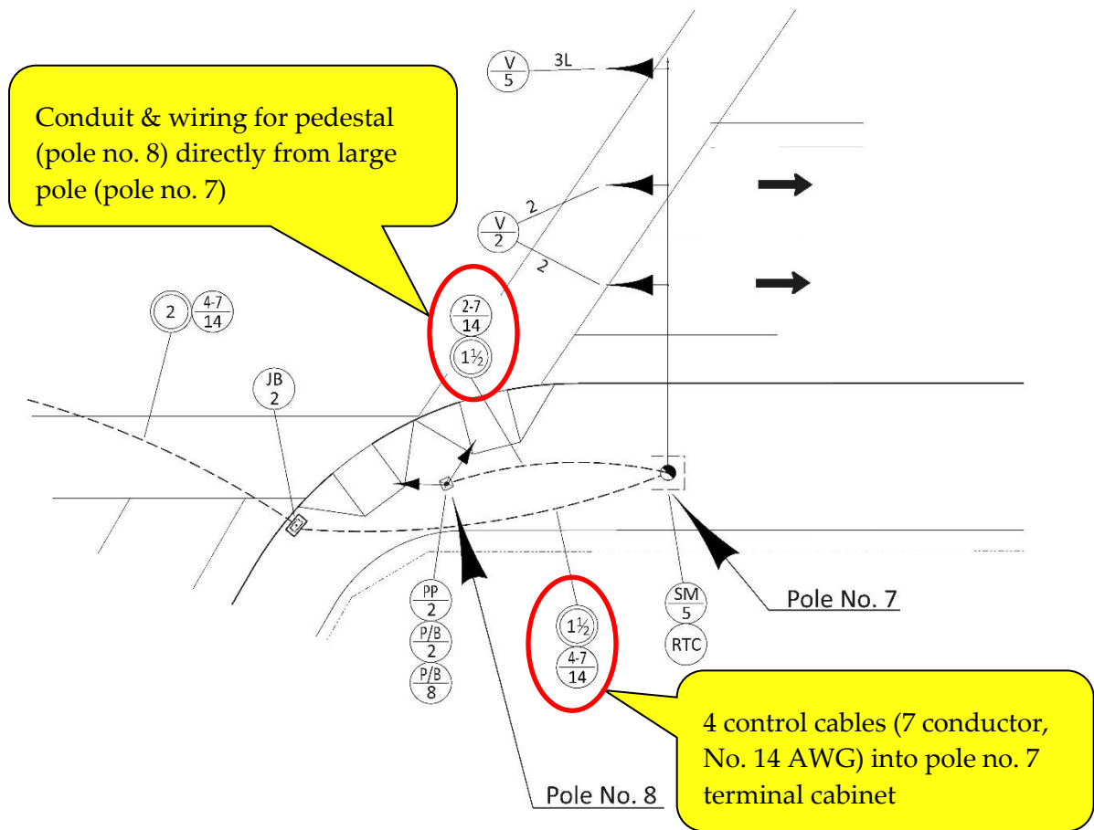
Figure 5-116 | Conduit Routing to Pedestal with Large Pole in Same Quadrant – Preferred Method
