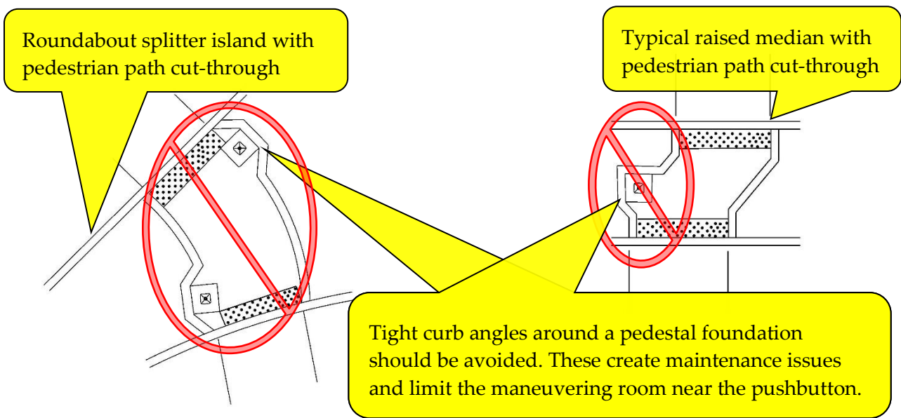
Figure 5-59 | Pedestal with Curb Around Foundation – Use Gentle Tapers
