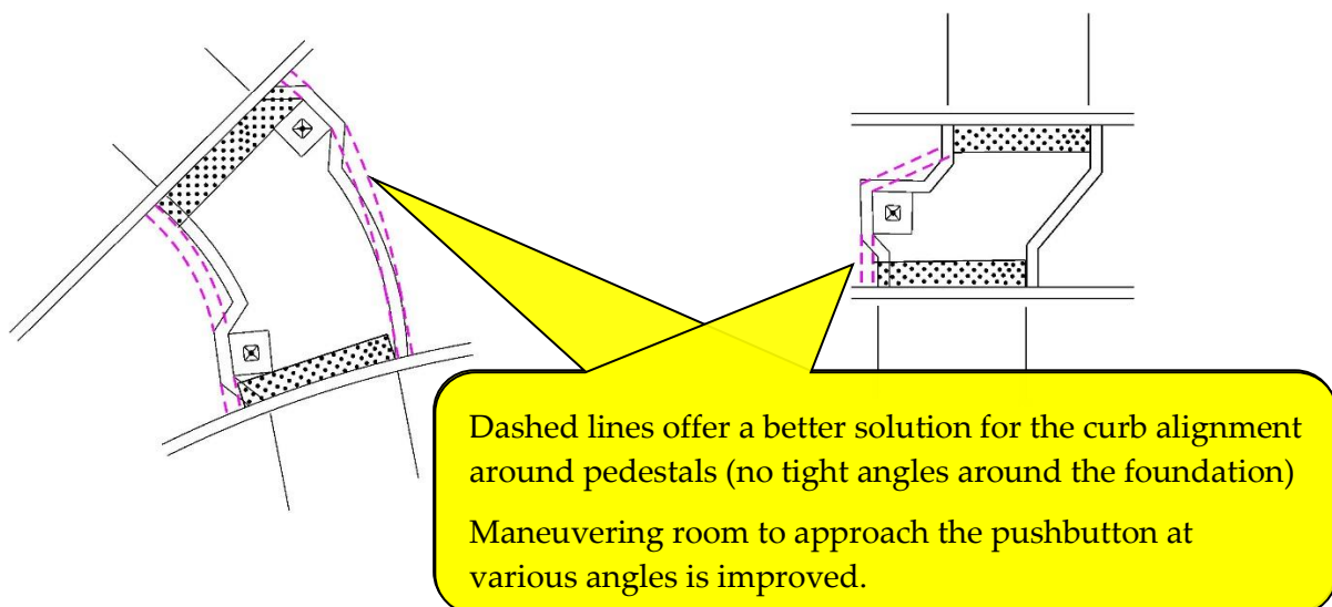
Figure 5-59 | Pedestal with Curb Around Foundation – Use Gentle Tapers
