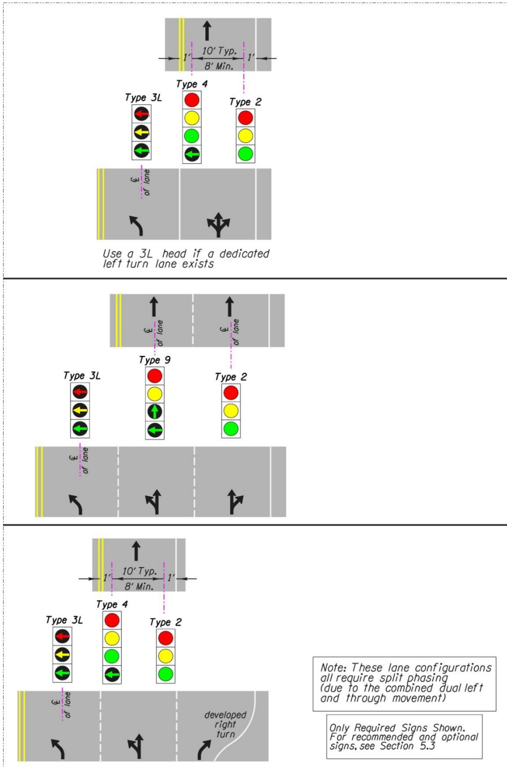
Figure 5-40 | Signal Head Placement for Split Phasing (cont.)
