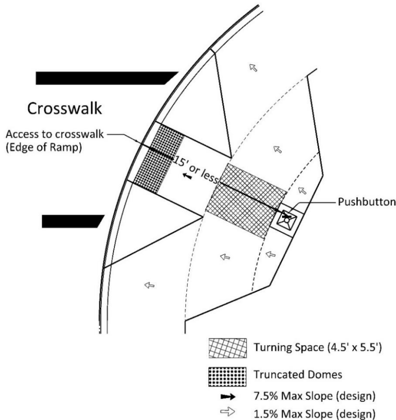
Figure 5-75 | Distance from Pushbutton to Crosswalk (Edge of Curb Ramp)
