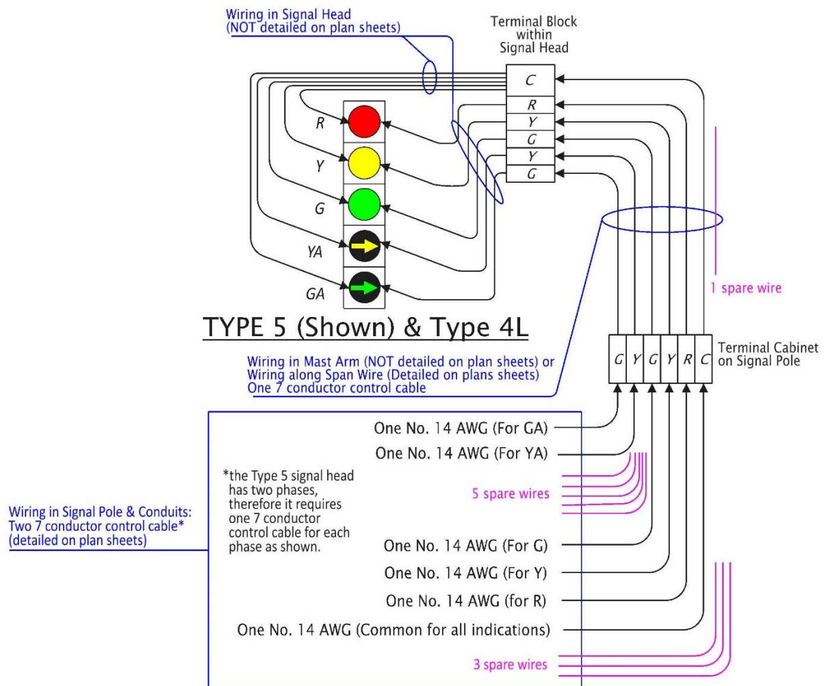
Figure 5-124 | Wiring for Type 4L & 5 Signal Heads
