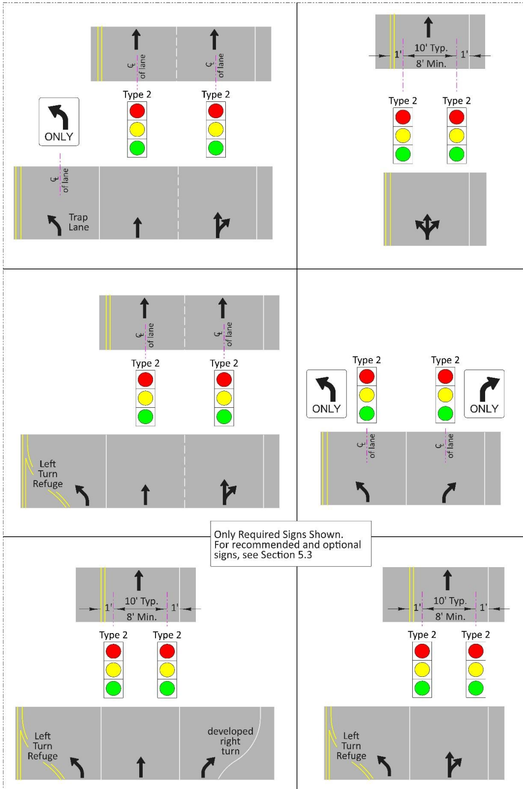
Figure 5-35 | Signal Head Placement for Lanes Sharing the Same Phase
