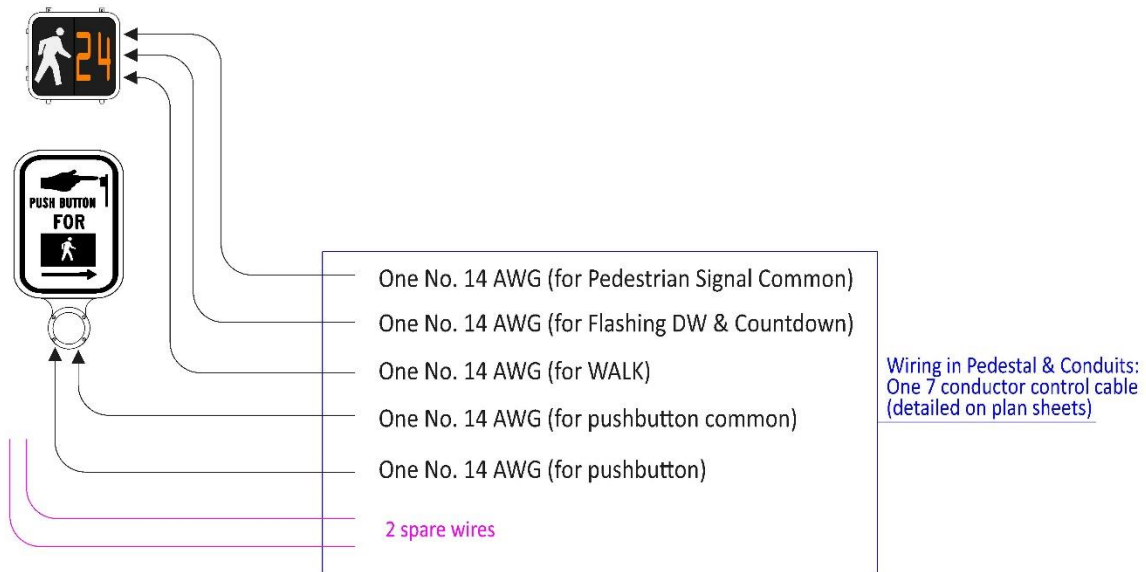
Figure 5-129 | Pedestrian Indication and Pushbutton Wiring
