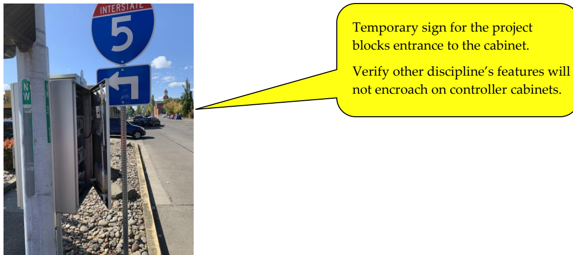
Figure 5-107 | Controller Cabinet Without the 3 Foot Minimum Working Space Due to Other Features Installed on the Project
