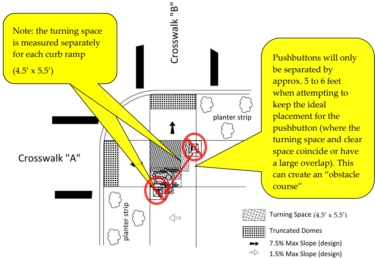
Figure 5-82 | Drawbacks to the 10-foot Separation of Pushbuttons at Two Curb Ramps That Share a Turning Space
