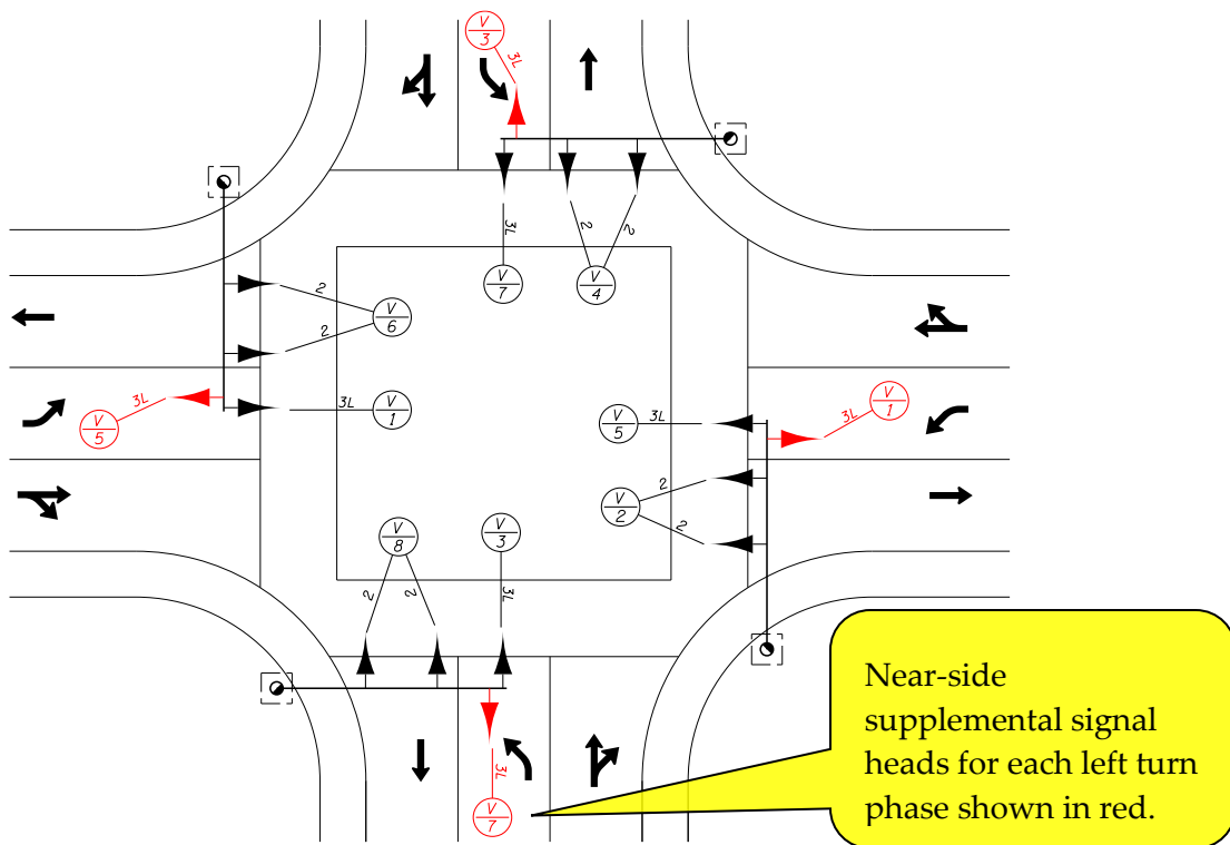
Figure 5-43 | Supplemental Near-Side Signal Heads – Typical Placement for Left Turn Phase
