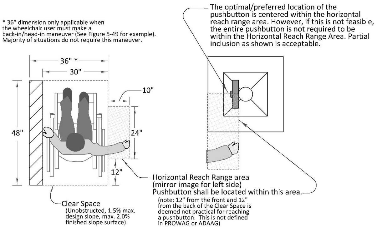
Figure 5-54 | Design Vehicle (Clear Space with 10" Max Horizontal Reach)
