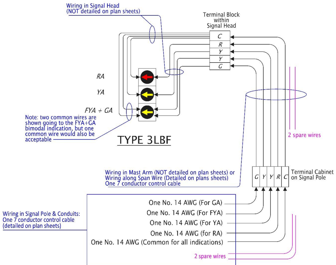
Figure 5-122 | Wiring for Type 3LBF Signal Head
