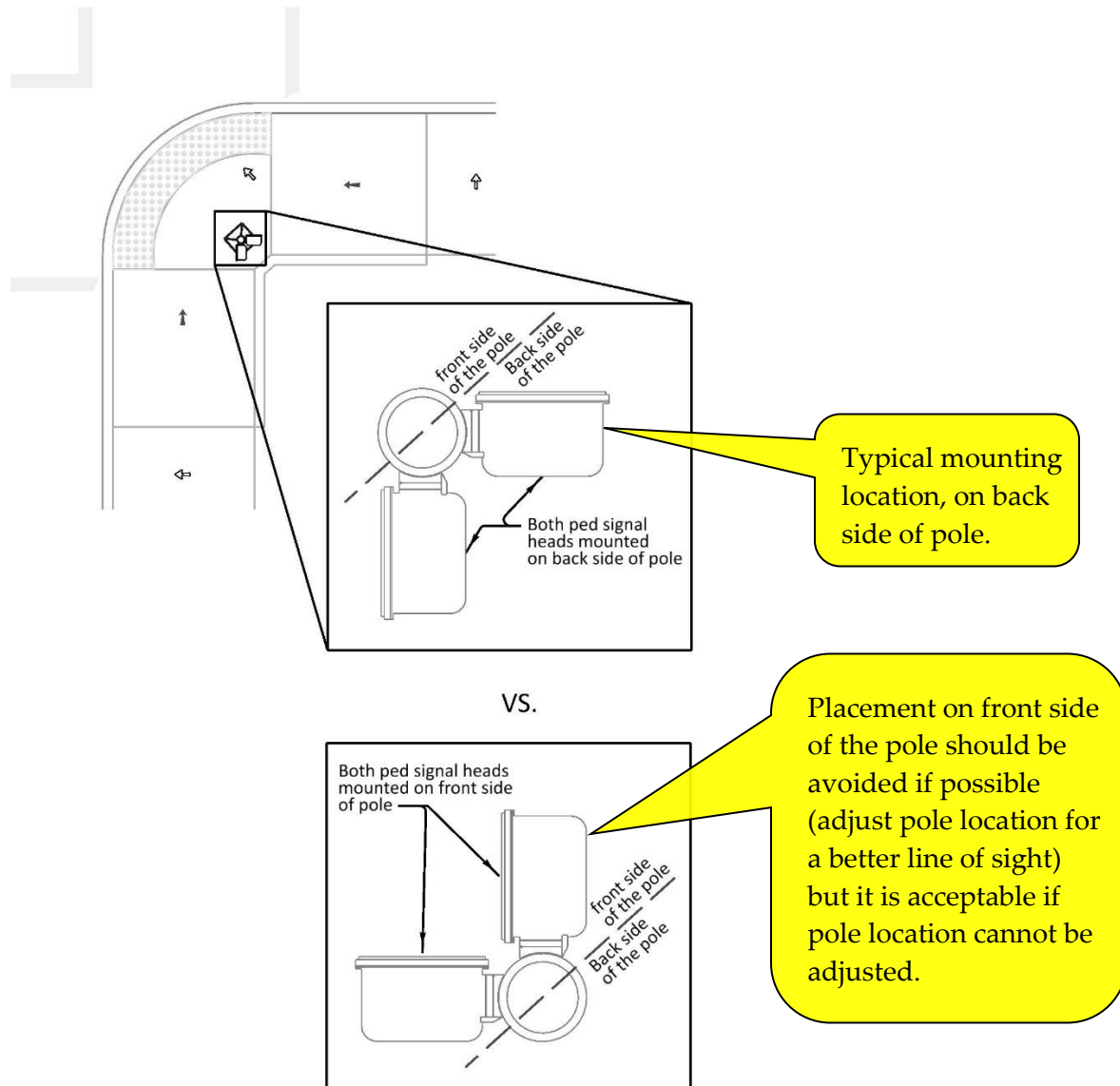
Figure 5-99 | Pedestrian signal orientation (back side vs. front side)
