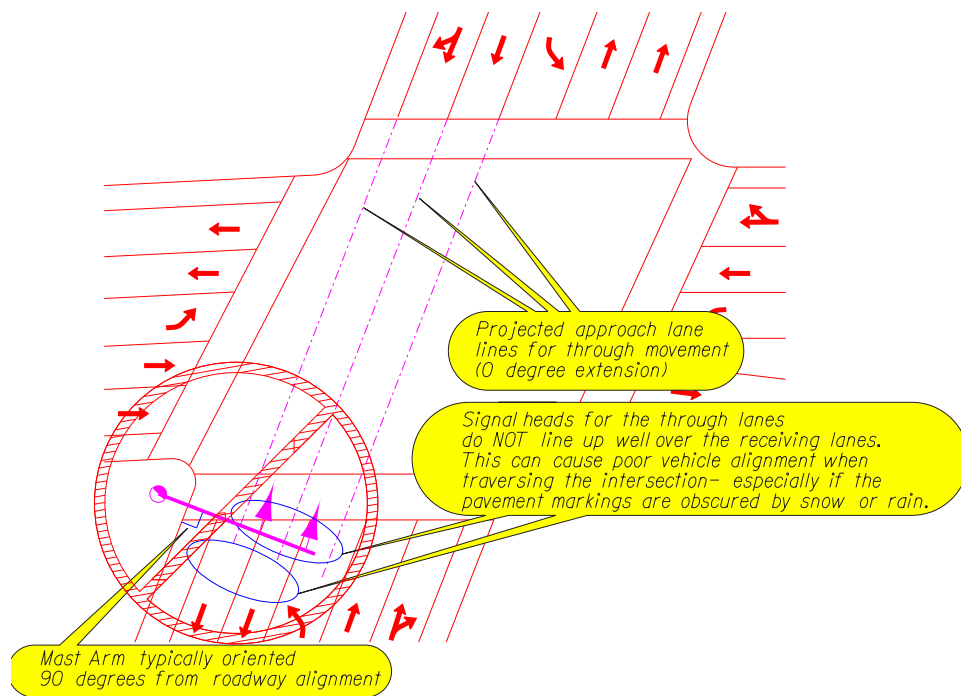
Figure 5-29 | Signal Head Placement For Through Movement Using Projected Lane Lines (INCORRECT METHOD)
