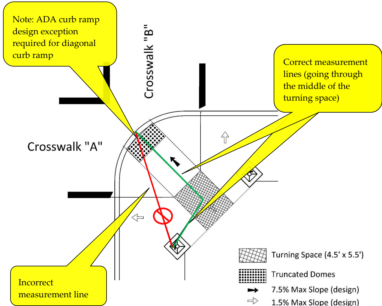
Figure 5-76 | Measuring Distance from Pushbutton to Crosswalk (Edge of Curb Ramp) Example
