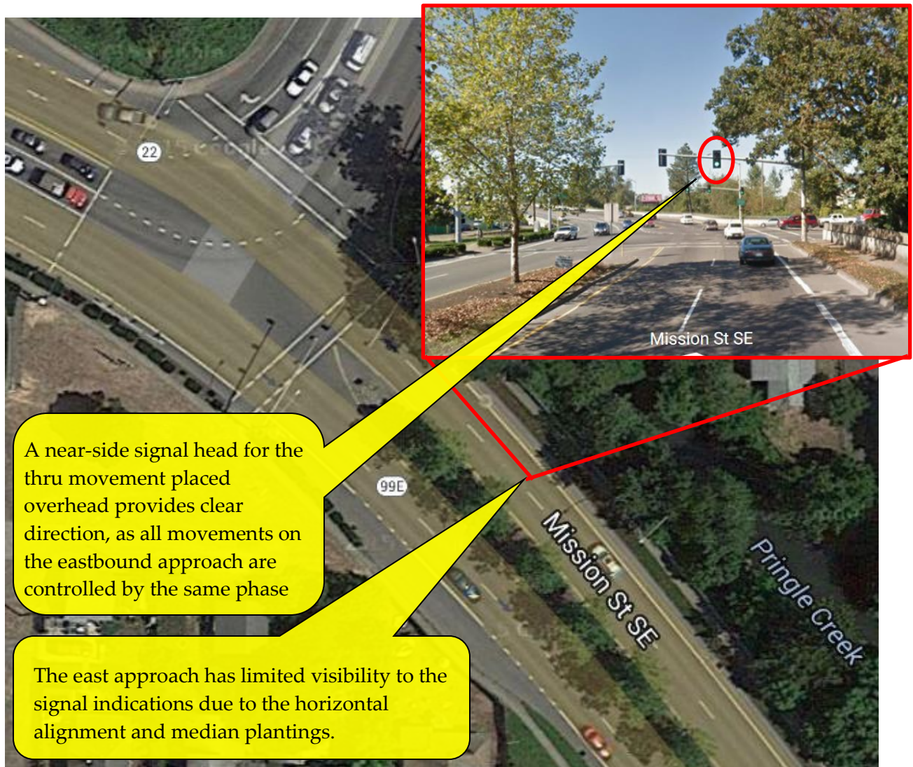
Figure 5-46 | Supplemental near-side signal head placement: Example 1
