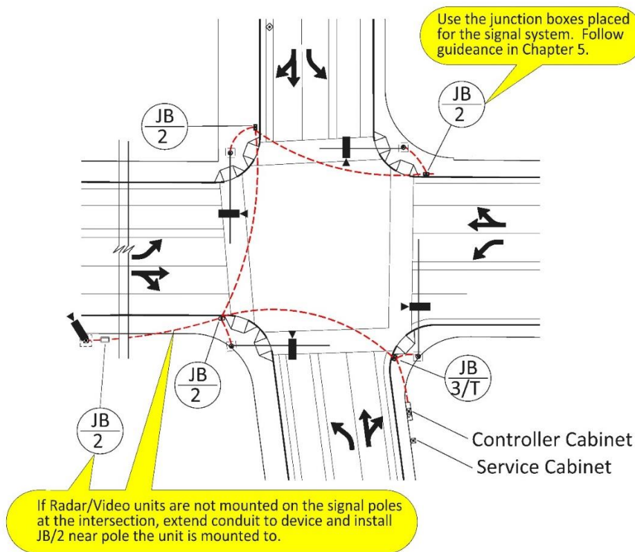
Figure 6-10 | Radar/Video Detection Conduit and Junction Box System
