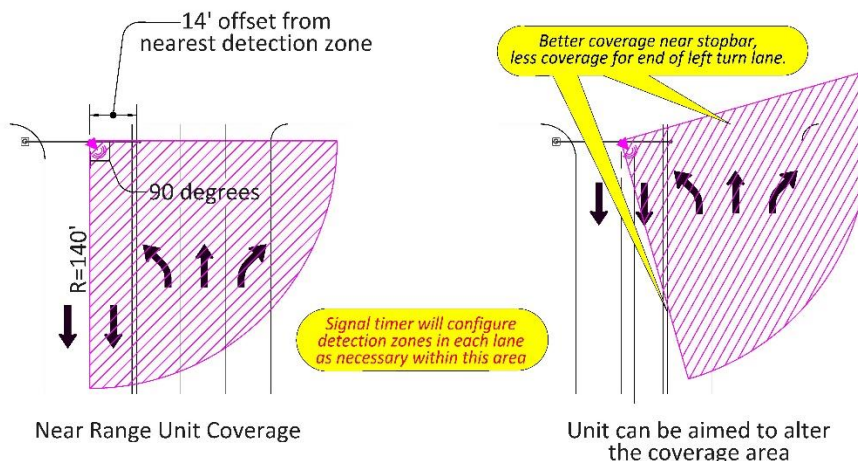
Figure 6-13 | Near Range Unit Coverage Area
