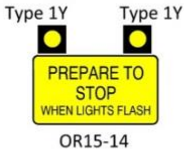
Figure 12-12 | Actuated Warning Beacon – Overhead Application
