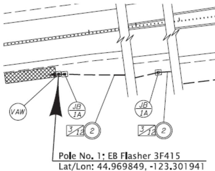
Figure 12-19 | TRAWS Wiring Example
