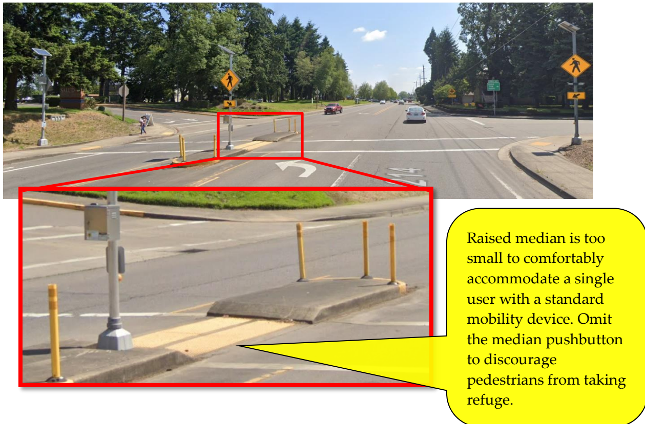
Figure 12-27 | Omit Pushbutton in Small Raised Medians
