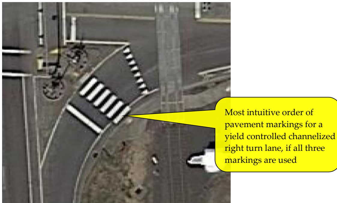
Figure 16-12 | Yield Controlled Channelized Right Turn Lane Pavement Marking Example
