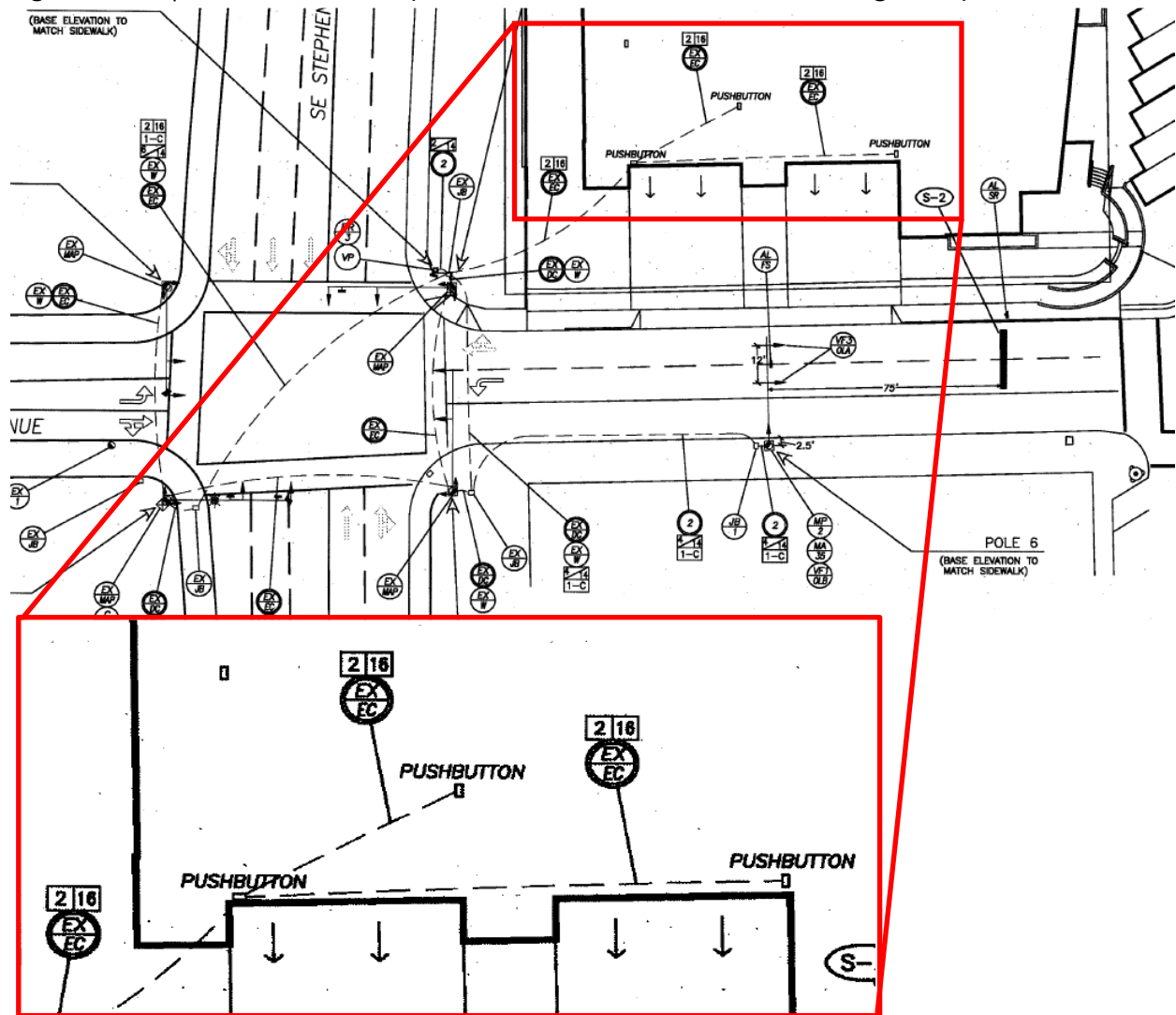
Figure 17-10 | Pushbutton Preemption – Placement and Conduit Routing Example
