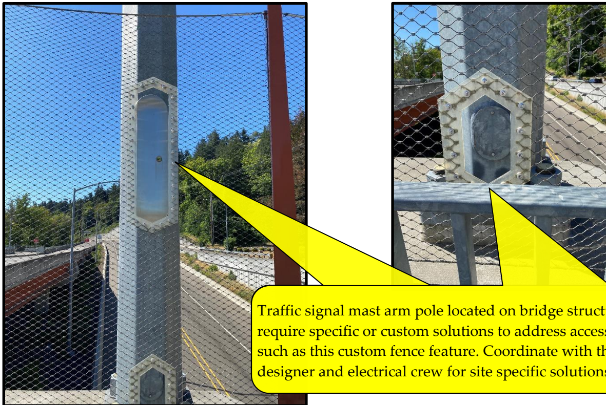
Figure 9-10 | Terminal Cabinet Degrees: Examples of Solutions to Access Issues
