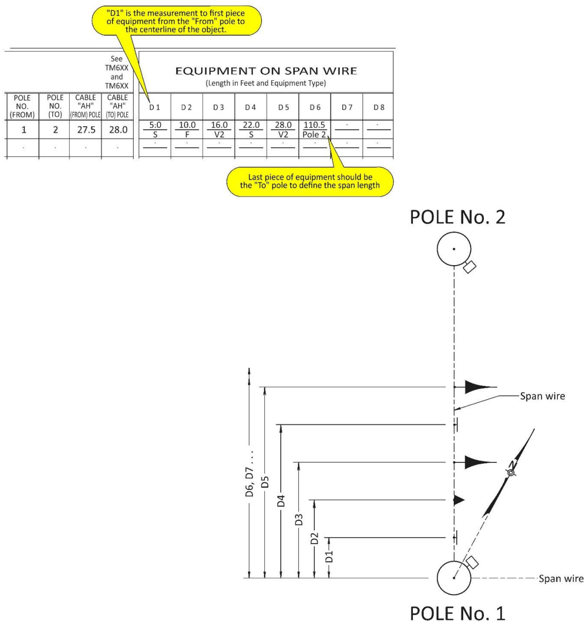
Figure 9-34 | Equipment on Span Wire
