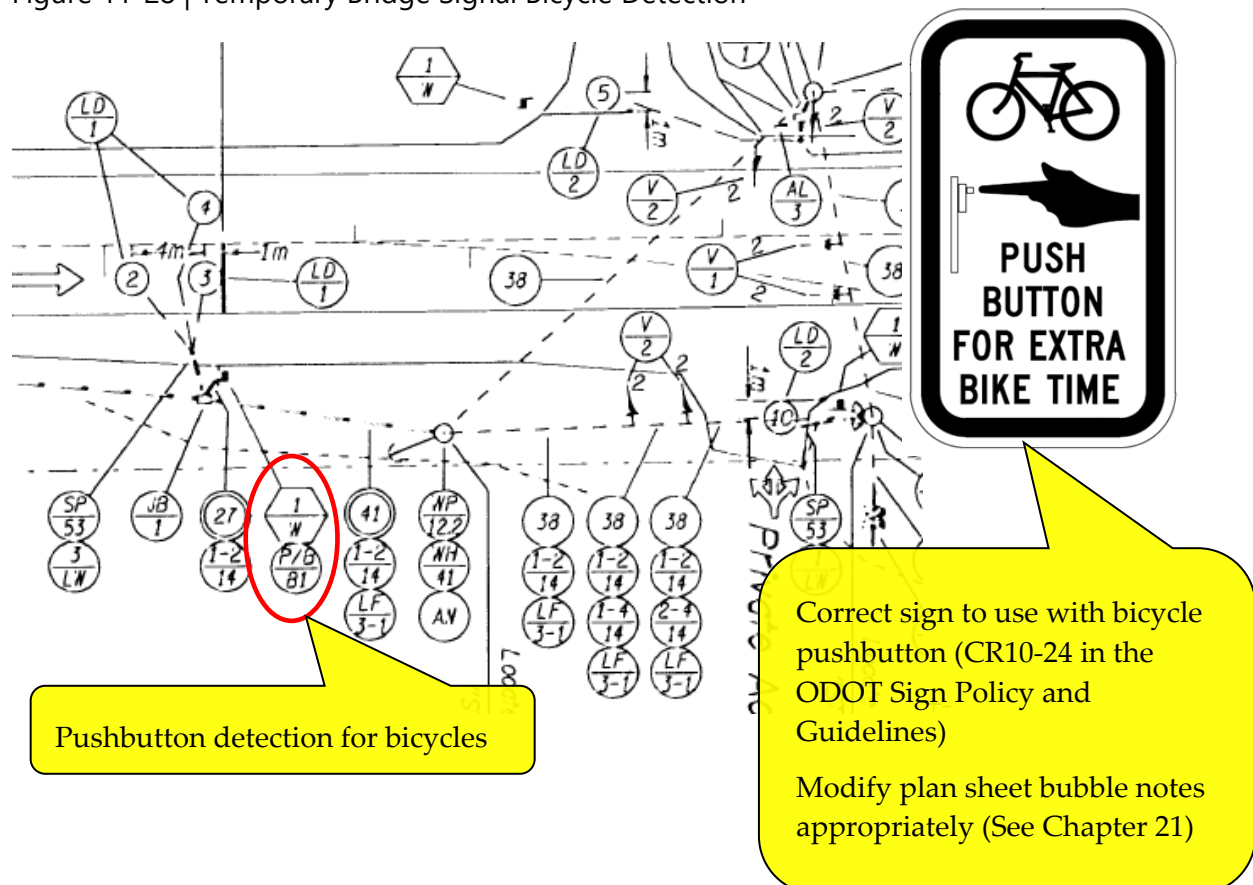
Figure 11-28 | Temporary Bridge Signal Bicycle Detection
