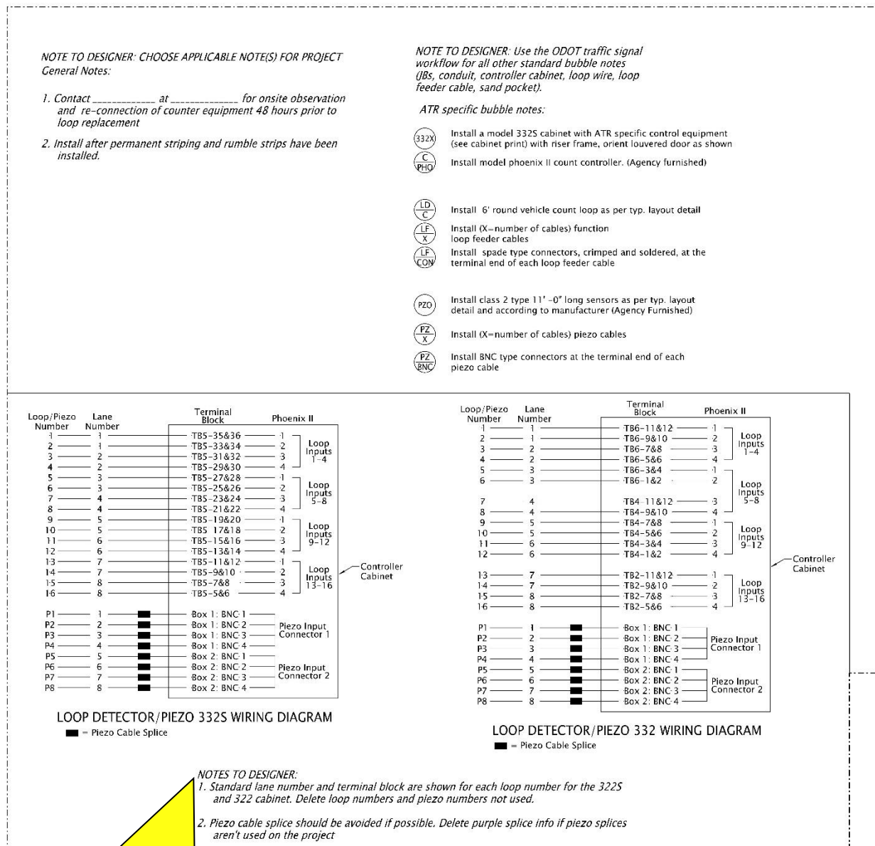
Figure 25-25 | DET4480 Drafting Content Example
