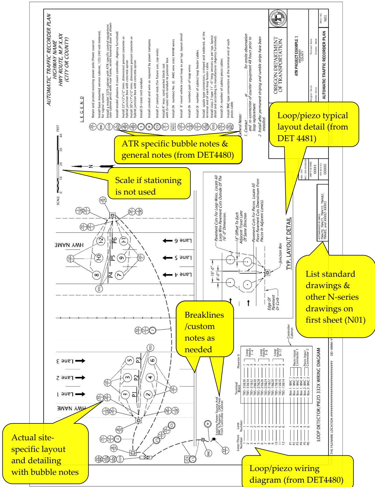
Figure 25-30 | ATR Project Example 1, Sheet N01
