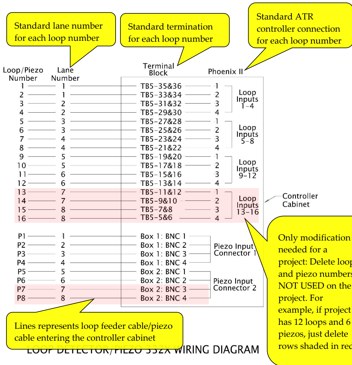
Figure 25-4 | Standard 332X Loop/Piezo Wiring Diagram
