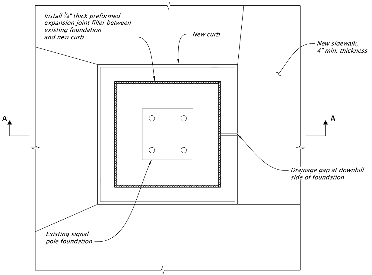
PLAN - TOP OF FOOTING
