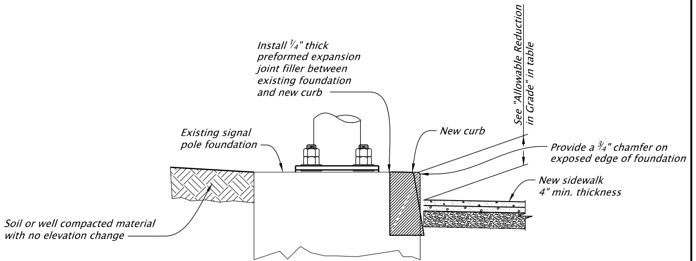
ELEVATION - TOP OF FOOTING
