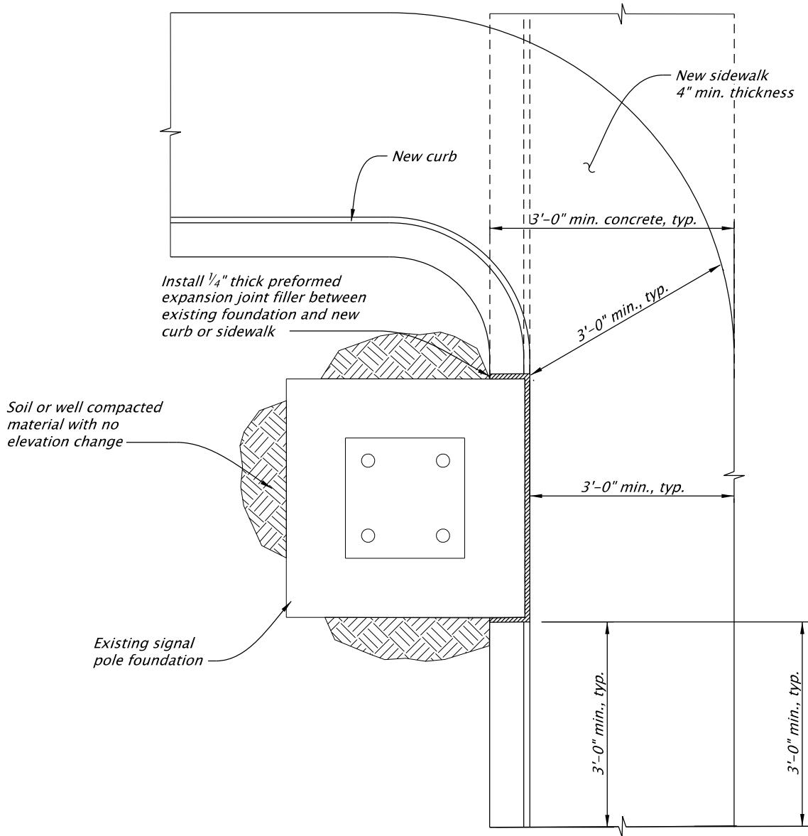
PLAN - TOP OF FOOTING
