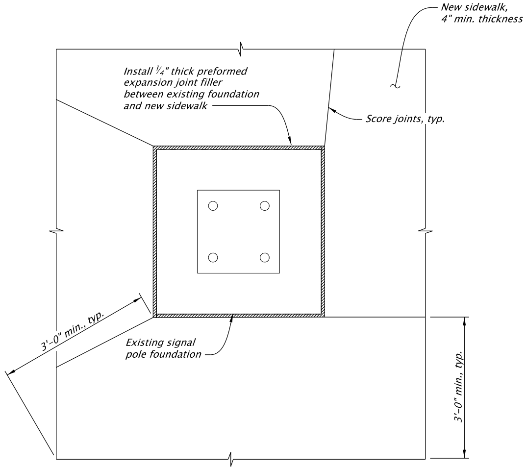
PLAN - TOP OF FOOTING
