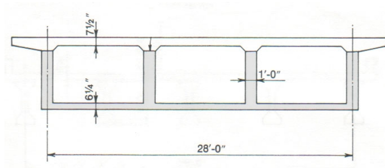
Figure 1.20. Typical Box Girder Bridge Section Source: Libby & Perkins (1976)
