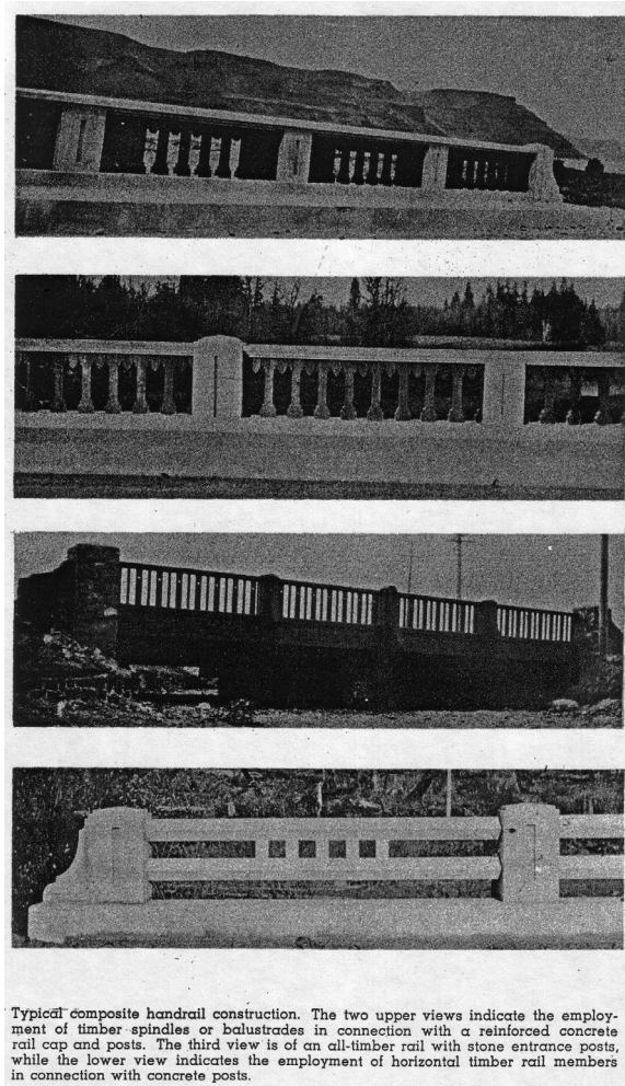
Figure 2.2. Typical Oregon Bridge Rails of the late 1930s
