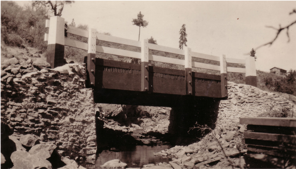
Figure 1.4. Bridge 1084, Timber Stringer Construction (undated), Photo circa 1930 Source: ODOT Archive
