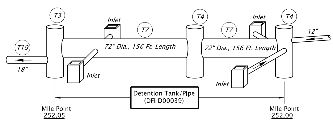
SCHEMATIC OF PIPE DRAINAGE SYSTEM N.T.S.
