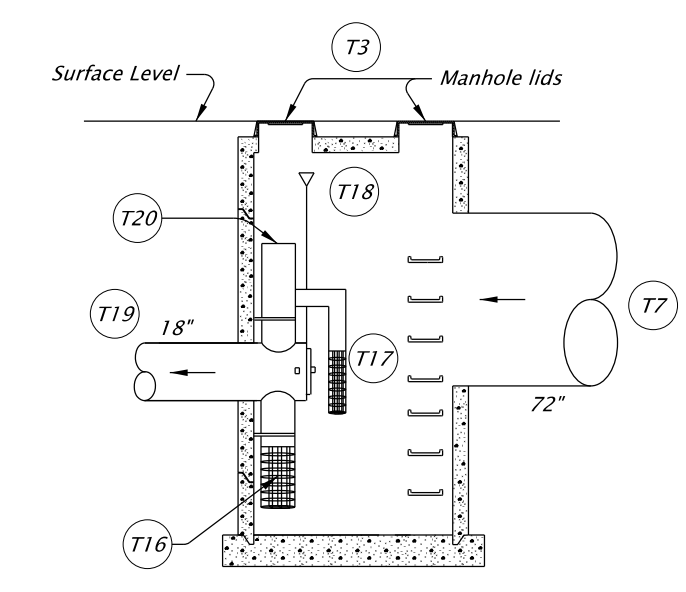
Flow Control Structure for Detention Tank / Pipe (DFI D00039)
