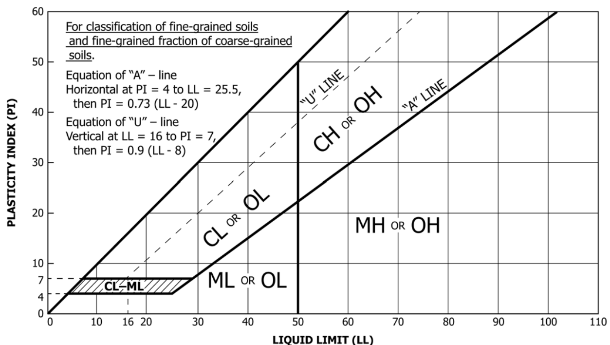
Figure 5-1 Plasticity Chart
