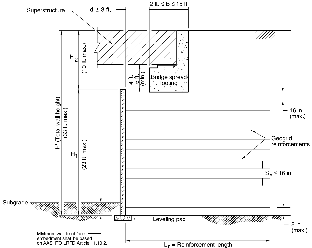
Figure 16-5 MSE Wall Supporting Bridge Abutment Spread Footing (Geogrid Reinforcements)
