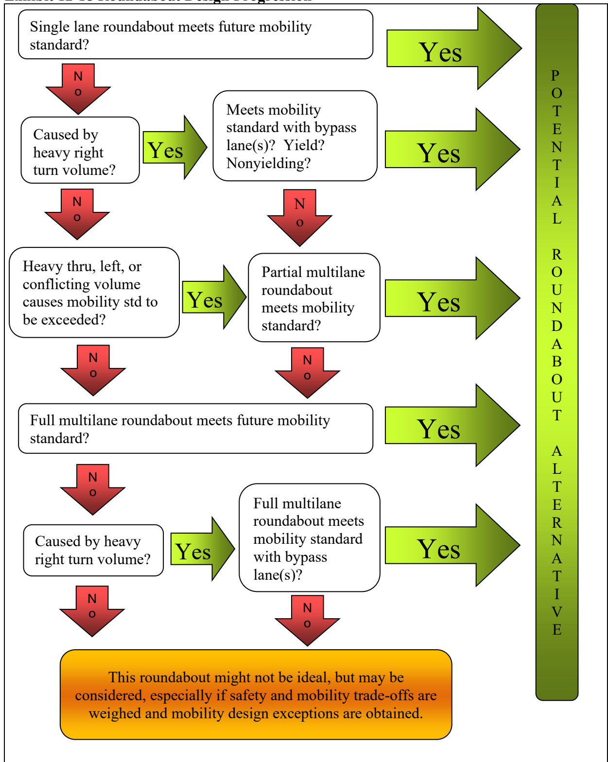
Exhibit 12-18 Roundabout Design Progression
