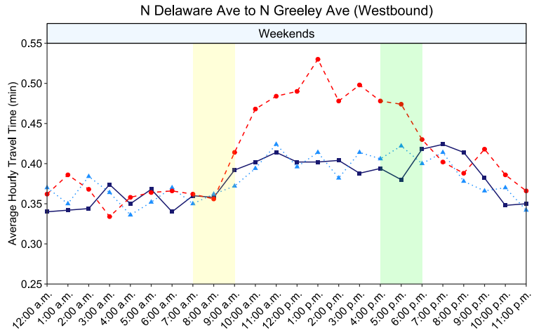
Figure 3.12: Average Hourly Travel Time Trends on N Greeley Ave ↔ N Delaware Ave
