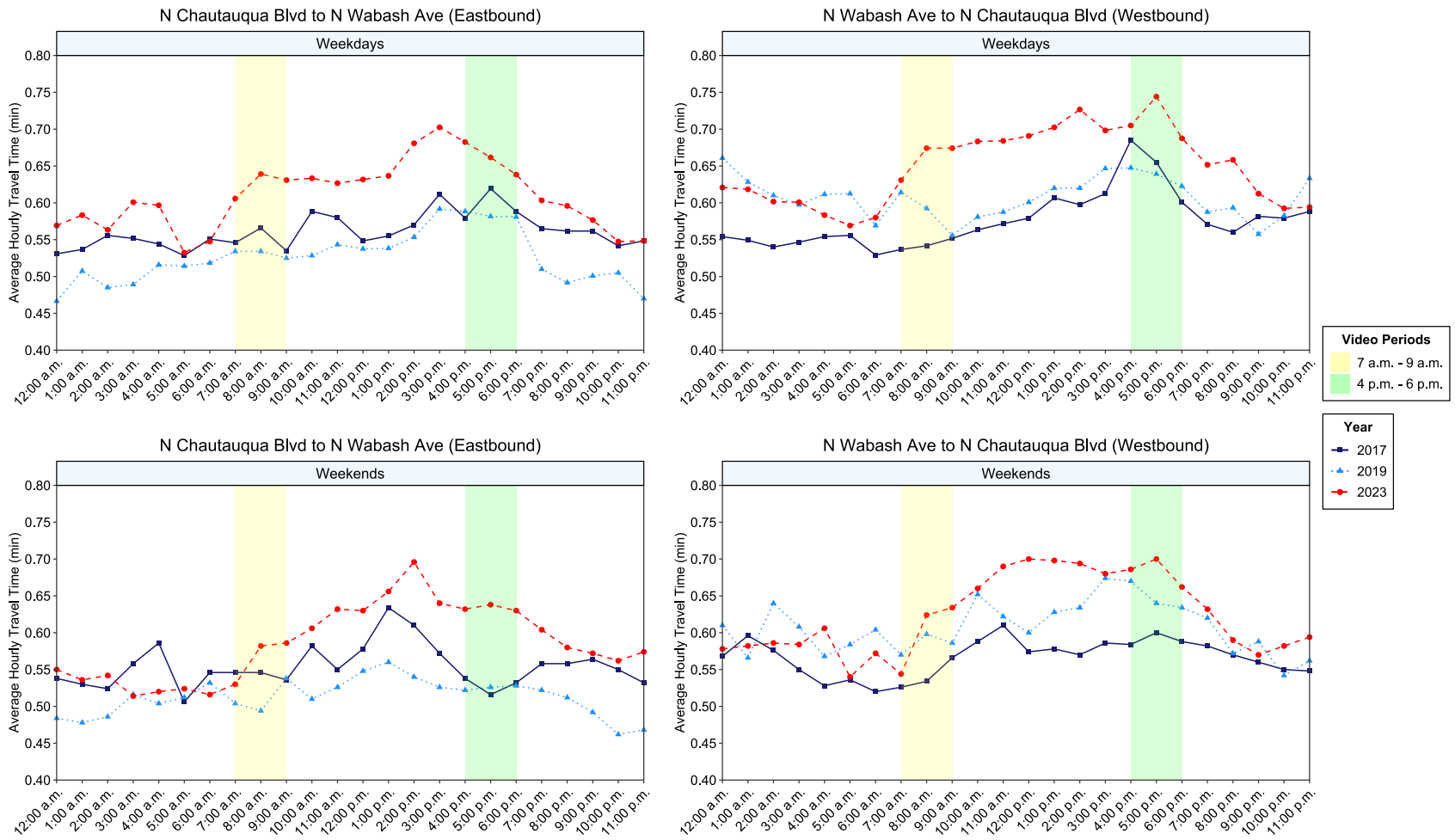
Figure 3.8: Average Hourly Travel Time Trends on N Chautauqua Blvd ↔ N Wabash Ave
