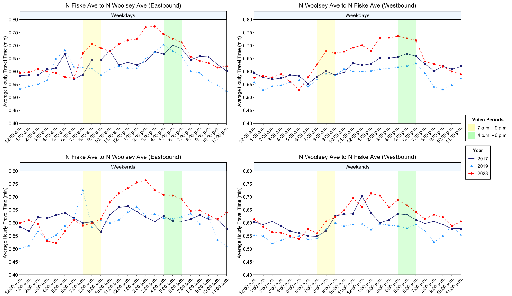
Figure 3.6: Average Hourly Travel Time Trends on N Fiske Ave ↔ N Woolsey Ave
