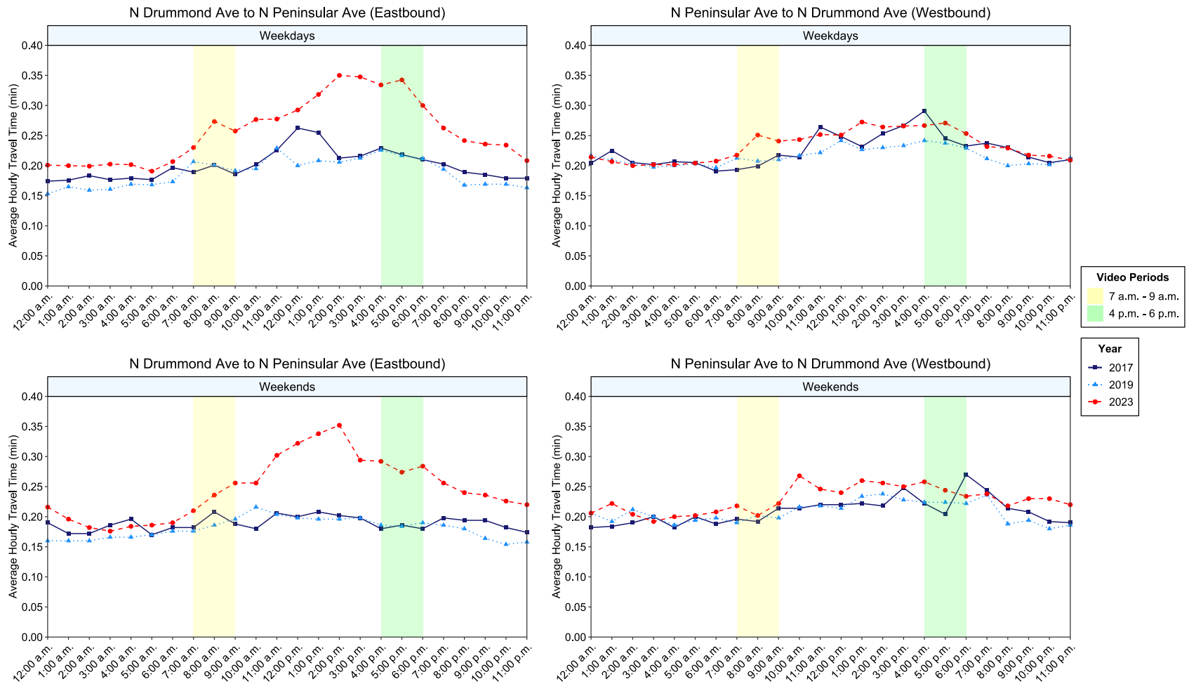
Figure 3.10: Average Hourly Travel Time Trends on N Drummond Ave ↔ N Peninsular Ave
