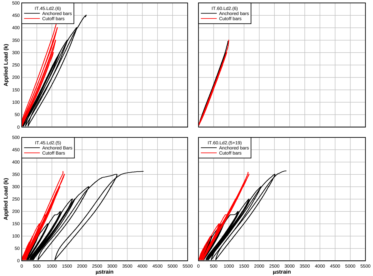
Figure 5.2: Average strain in flexural bars at the preformed diagonal crack for IT-beam specimens
