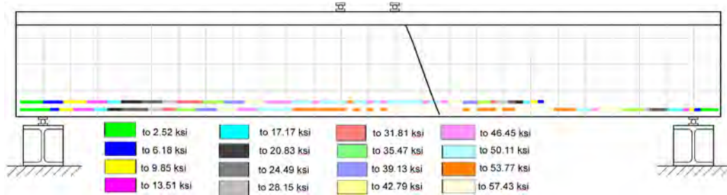
Figure 5.36: Specimen T.60.Ld3.(5) predicted steel reinforcement stresses at 274 kips
