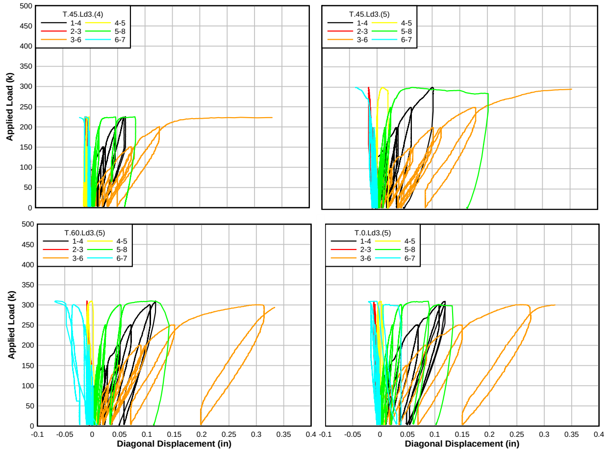
Figure A.10: Load – diagonal displacement plots for T-beam specimens
