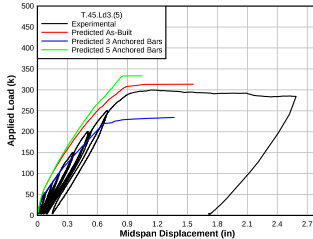
Figure 5.42 Predicted bounds of T-beam specimen with more and less flexural reinforcement than as-built
