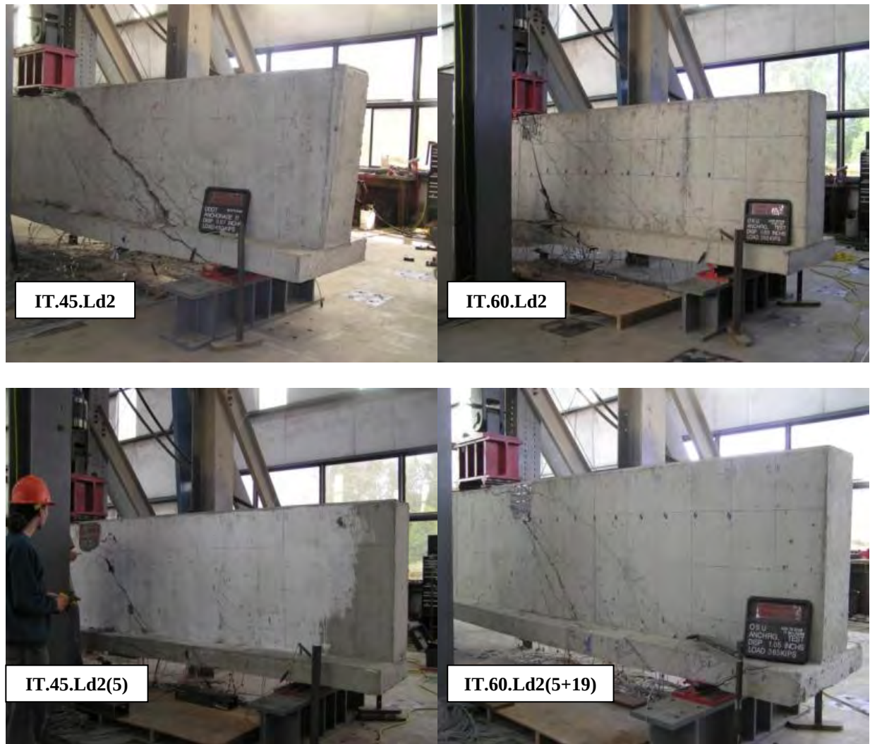
Figure 4.6: Digital photographs at failure of IT-beam specimens
