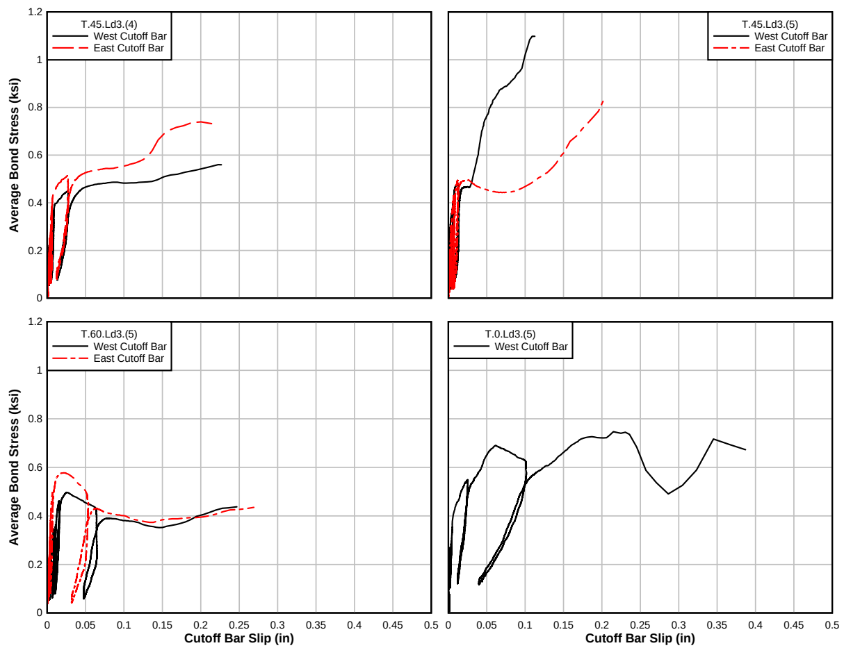
Figure 4.13: Bond stress – cutoff bar slip comparison for T-beams
