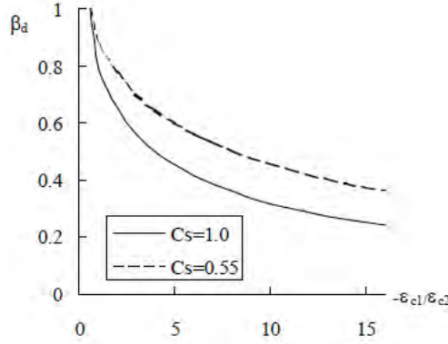
Figure D.3: Vecchio 1992-A compression softening model (Vecchio and Wong, 2002)
