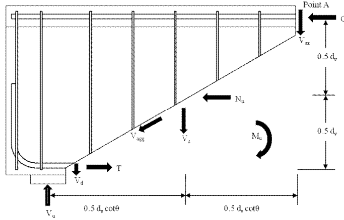
Figure 2.4: Internal forces in a diagonal cracked reinforced concrete section
