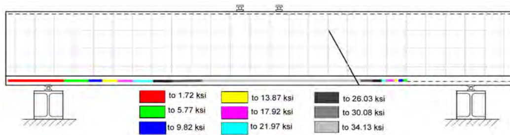
Figure 5.41: Specimen T.60.Ld2.(5+19) predicted steel reinforcement stresses at failure
