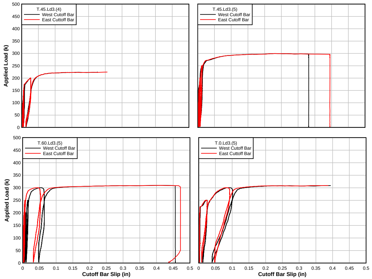
Figure A.6: Load – cutoff bar slippage plots for T-beam specimens
