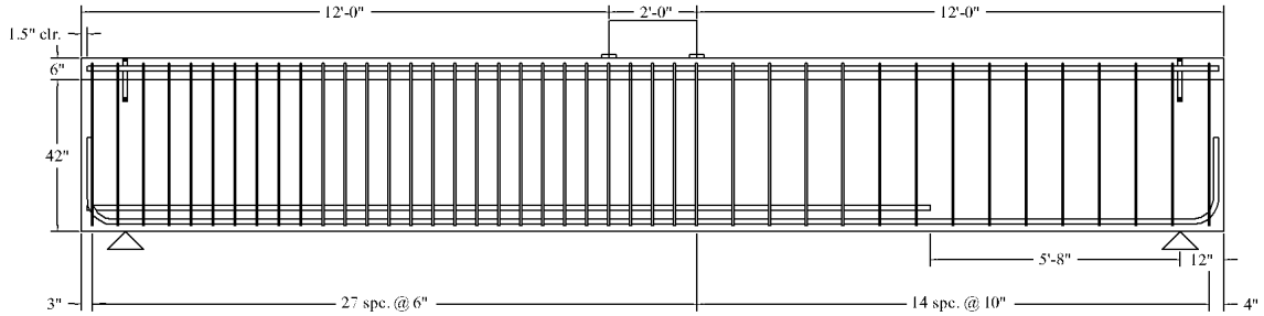
Figure 3.4: Elevation of specimen T.0.Ld3.(5)
