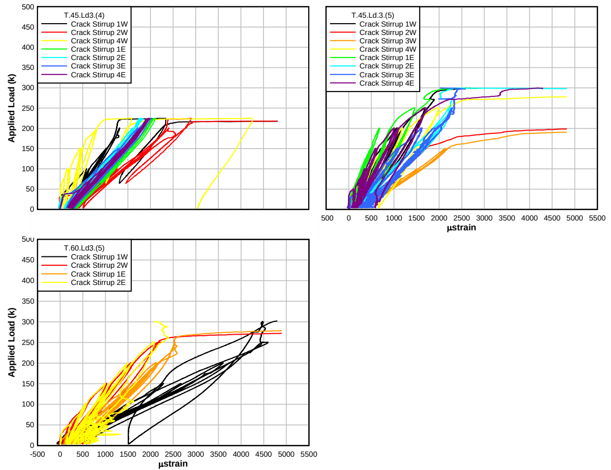
Figure A.25: Load – preformed crack stirrup stain plots for T-beam specimens
