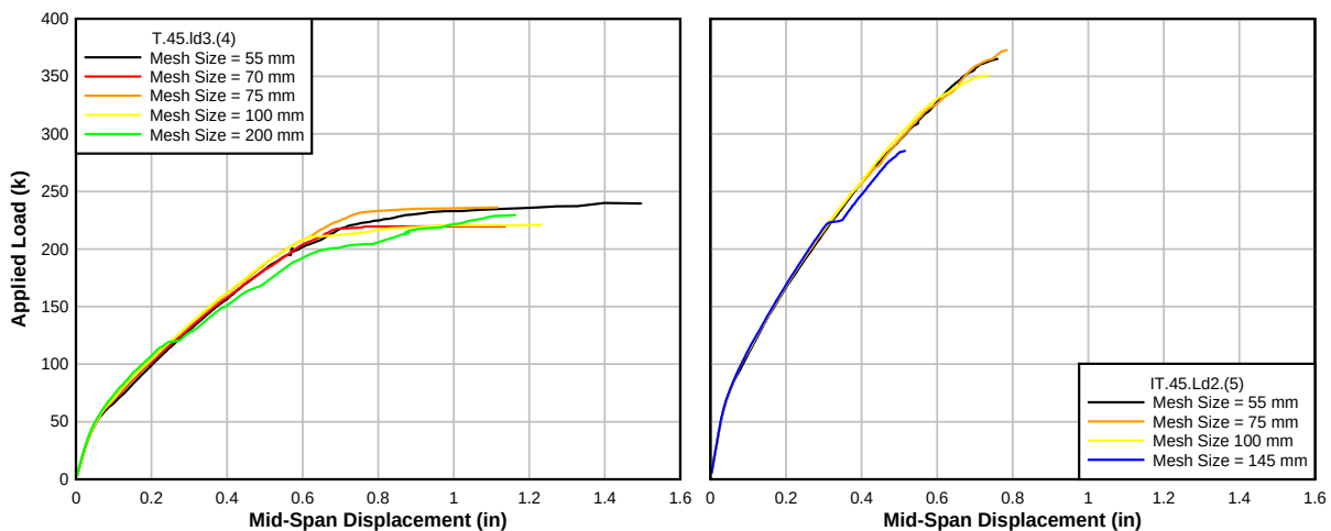
Figure 5.23: Predicted load-deformation response for different finite element mesh sizes (specimen T.45.Ld3(4))
