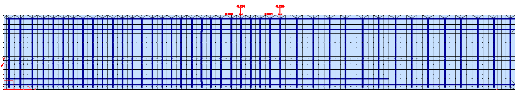
Figure 5.17: Specimen T.0.Ld3.(5) finite element model
