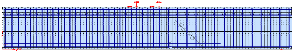
Figure 5.14: Specimen T.45.Ld3.(4) finite element model
