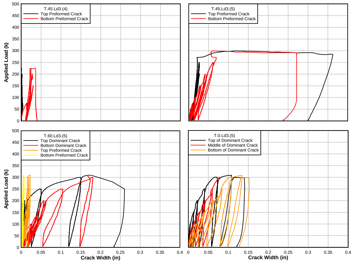
Figure A.8: Load – preformed crack width plots for T-beam specimens
