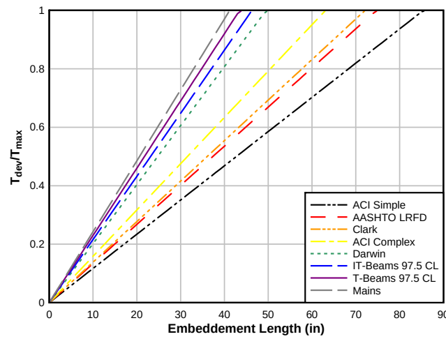
Figure 5.4: Comparison of literature, design specification, and experimental development lengths
