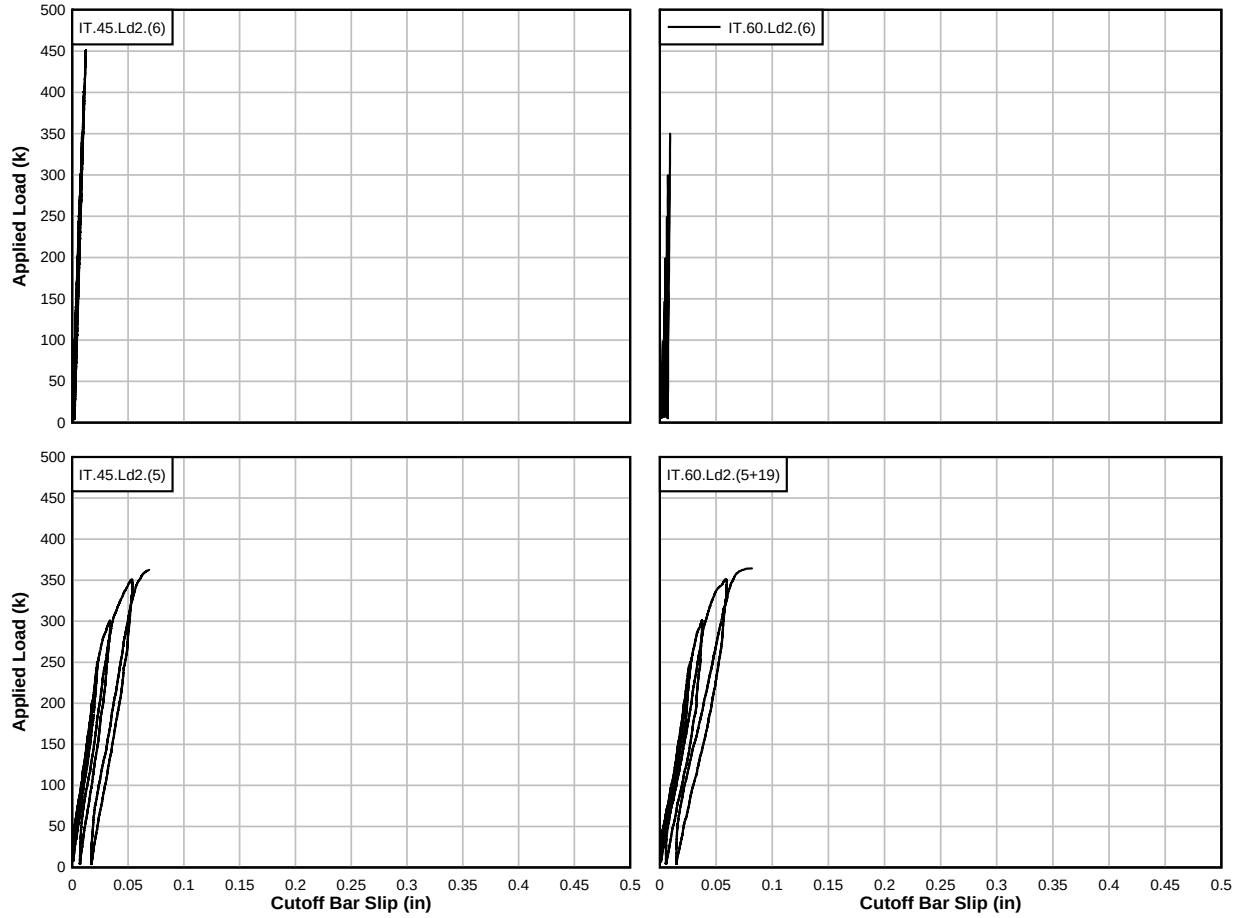
Figure 4.10: Load-cutoff bar slippage plots for IT-beam specimens
