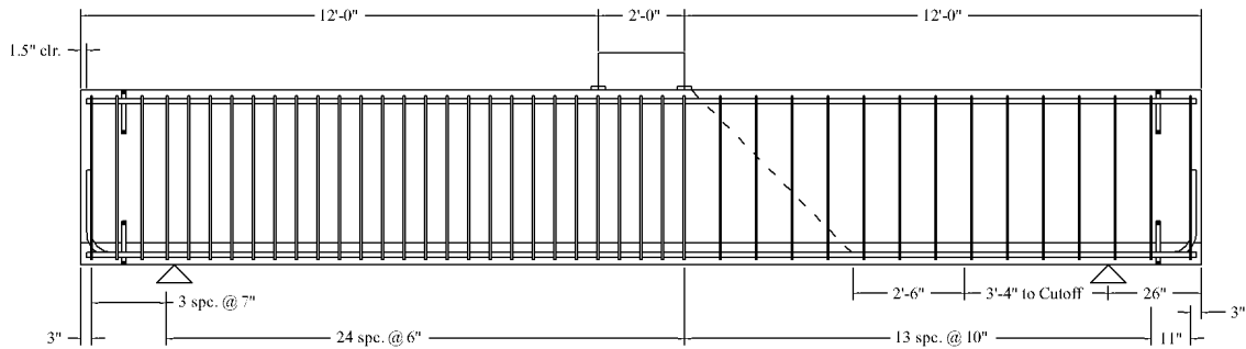
Figure 3.8: Elevation of specimen IT.45.Ld2(5)
