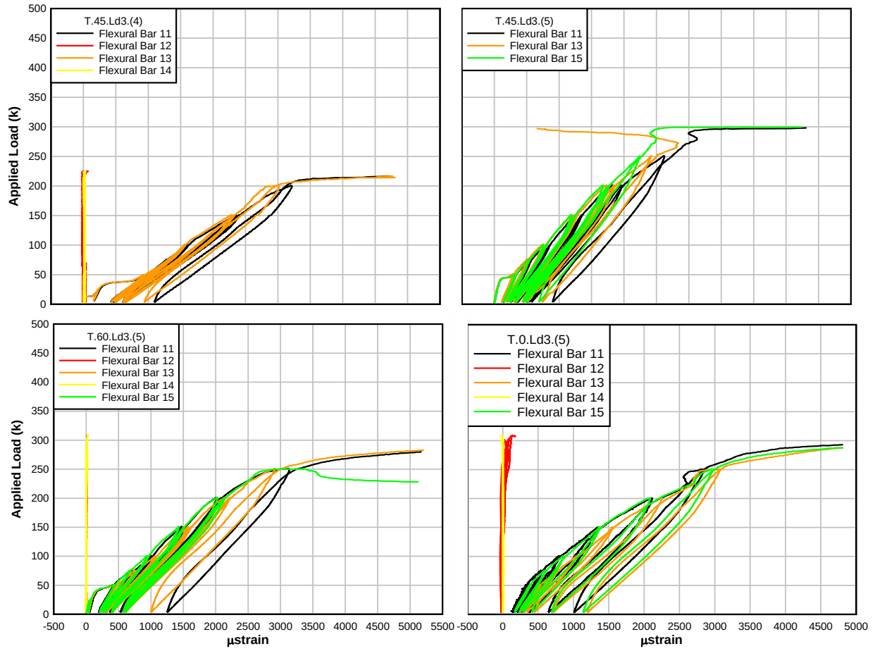
Figure A.12: Load – flexural bar location 1 strain plots for T-beam specimens
