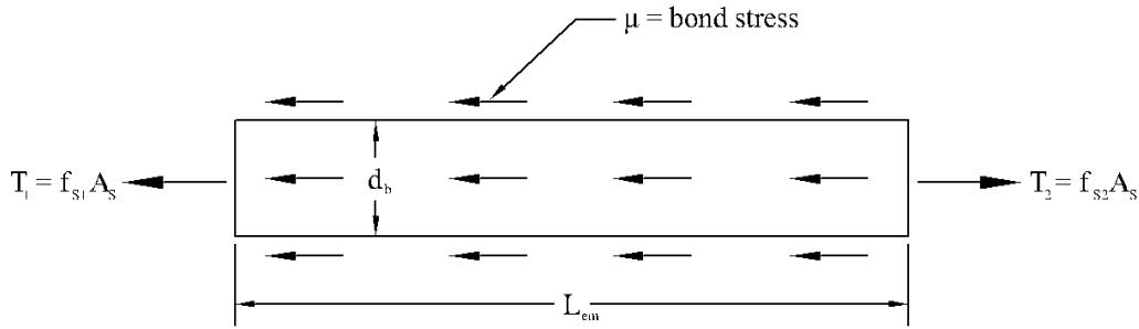
Figure 2.2: Forces acting on a segment of reinforcing steel
