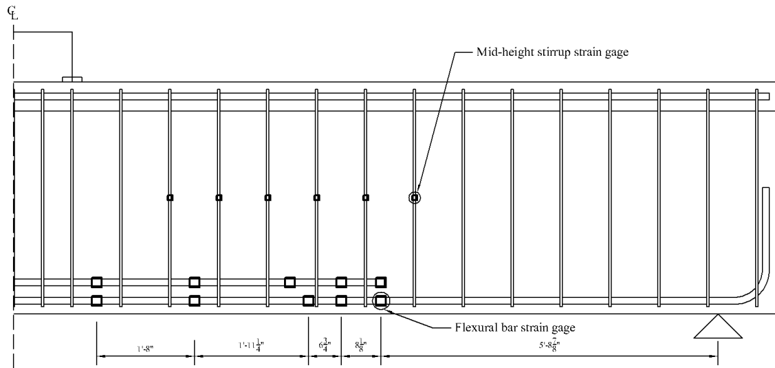
Figure 3.14: Specimen T.0.Ld3(5) internal sensor array
