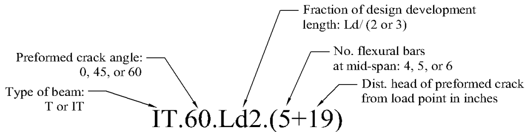
Figure 3.1: Specimen naming convention
