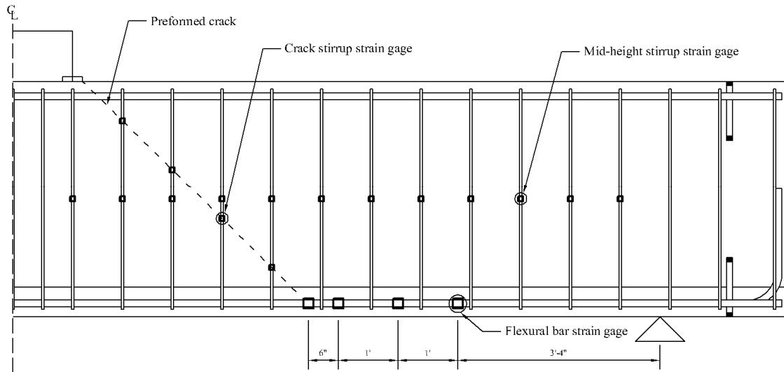
Figure 3.17: Specimen IT.45.Ld2(5) internal sensor array
