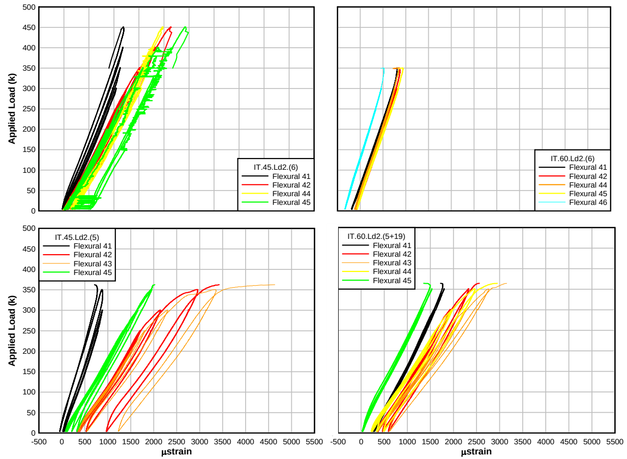
Figure A.19: Load – flexural bar location 4 strain plots for IT-beam specimens
