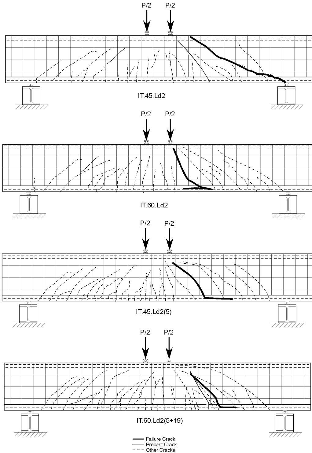
Figure 4.4: Failure crack maps for IT-beam specimens
