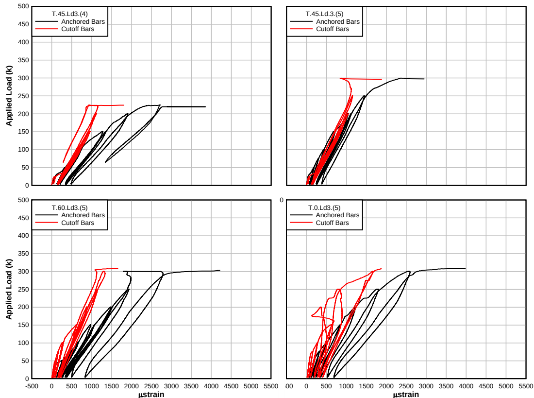
Figure 5.1: Average strain in flexural bars at the performed diagonal crack for T-beam specimens
