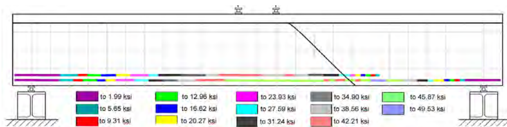
Figure 5.34: Specimen T.45.Ld3.(4) predicted steel reinforcement stresses at 182 kips
