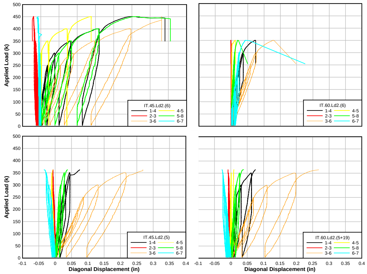
Figure A.11: Load – diagonal displacement plots for IT-beam specimens
