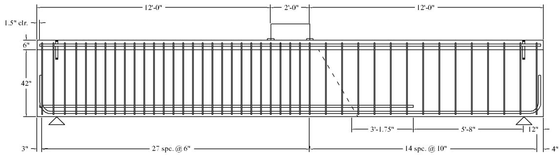
Figure 3.3: Elevation of specimen T.60.Ld3.(5)
