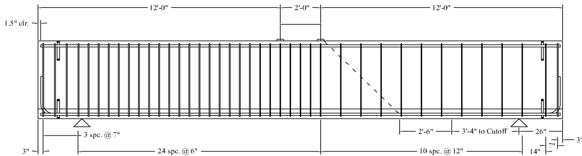
Figure 3.6: Elevation of specimen IT.45.Ld2
