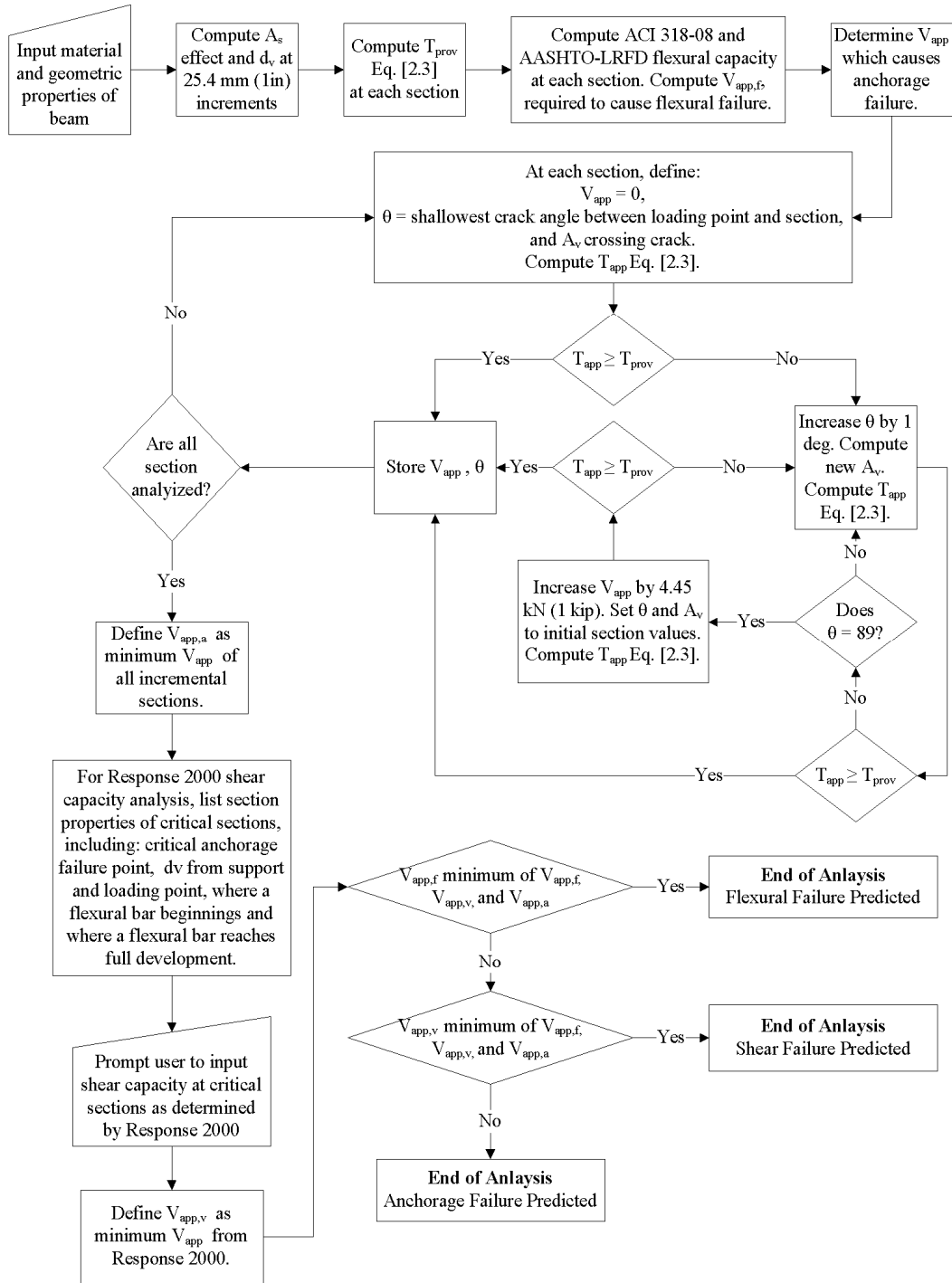
Figure 5.5: Failure load and mode solution procedure using Excel Macro
