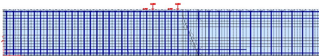
Figure 5.16: Specimen T.60.Ld3.(5) finite element model
