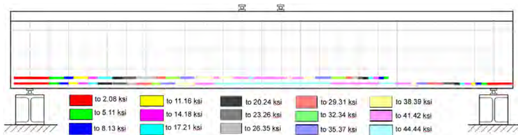
Figure 5.37: Specimen T.0.Ld3.(5) predicted steel reinforcement stresses at 228 kips
