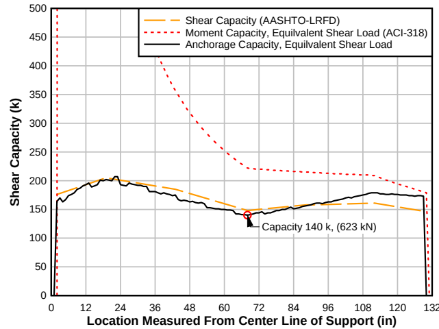
Figure 5.7: Example evaluation method one capacity and failure mode prediction for Specimen T.45.Ld3.(4)
