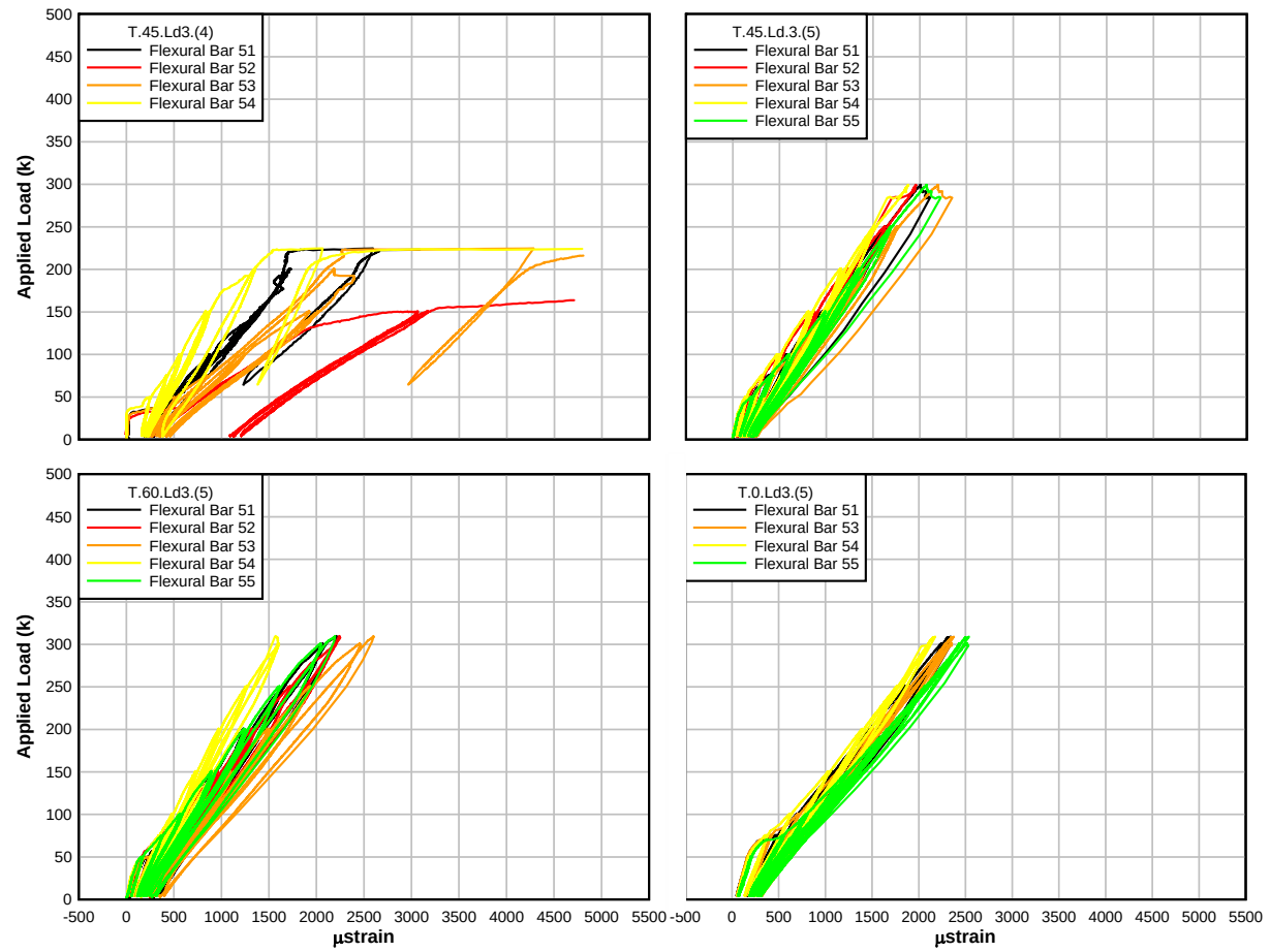
Figure A.20: Load – flexural bar location 5 strain plots for T-beam specimens
