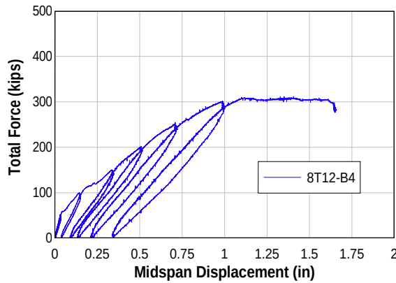
Figure 5.9: Specimen 8T12-B4 load-deflection plot and failure photo (Higgins, et al. 2004)
