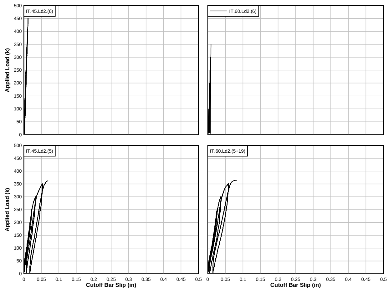
Figure A.7: Load – cutoff bar slippage plots for IT-beam specimens
