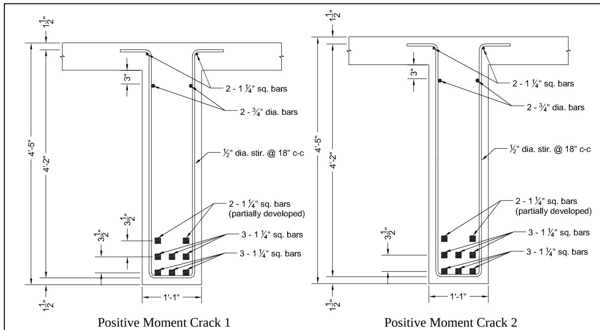
Figure B.3a: Beam Cross Sections at Crack Locations.
