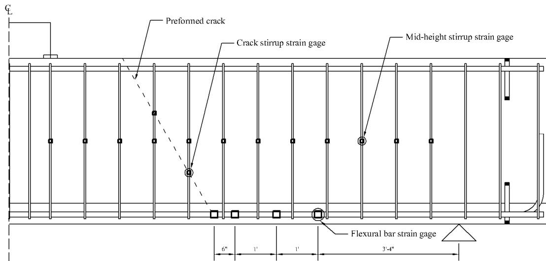
Figure 3.18: Specimen IT.60.Ld2(5+19) internal sensor array
