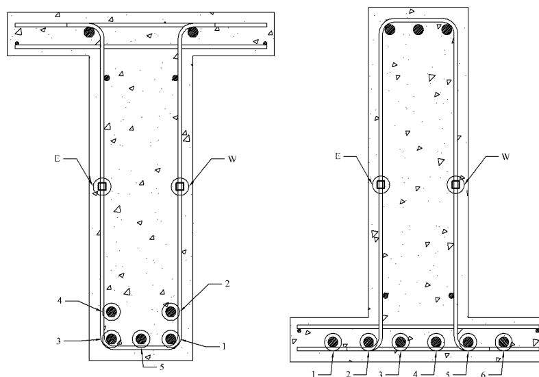
Figure A.3: Typical cross-section of specimens strain gage labeling convention
