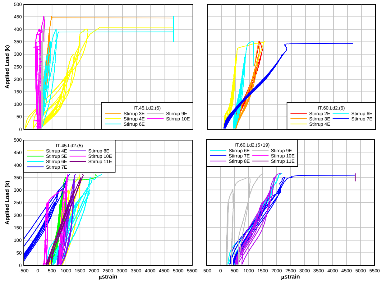
Figure A.24: Load – east mid-height stirrup stain plots for IT-beam specimens
