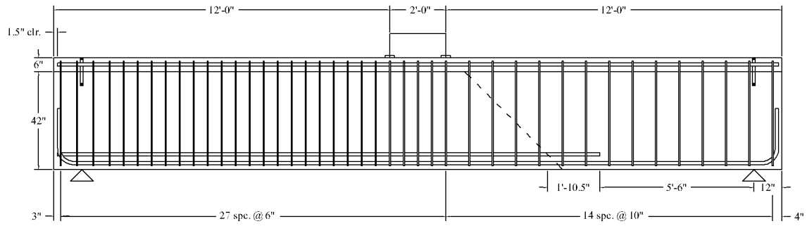
Figure 3.2: Elevation of specimens T.45.Ld3.(4) and T.45.Ld3.(5)
