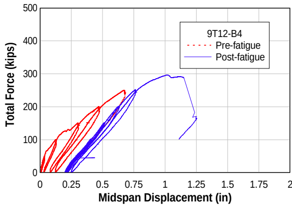
Figure 5.10: Specimen 9T12-B4 load-deflection plot and failure photo (Higgins, et al. 2004)
