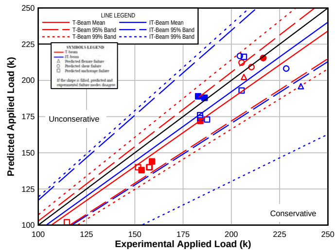
Figure 5.11: Macro analysis failure applied load predicted results bias analysis
