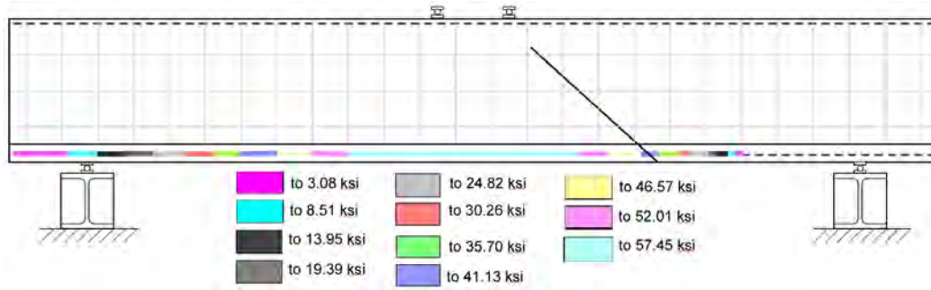
Figure 5.40: Specimen IT.45.Ld2.(5) predicted steel reinforcement stresses at failure
