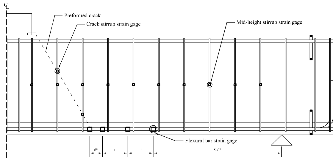
Figure 3.16: Specimen IT.60.Ld2 internal sensor array
