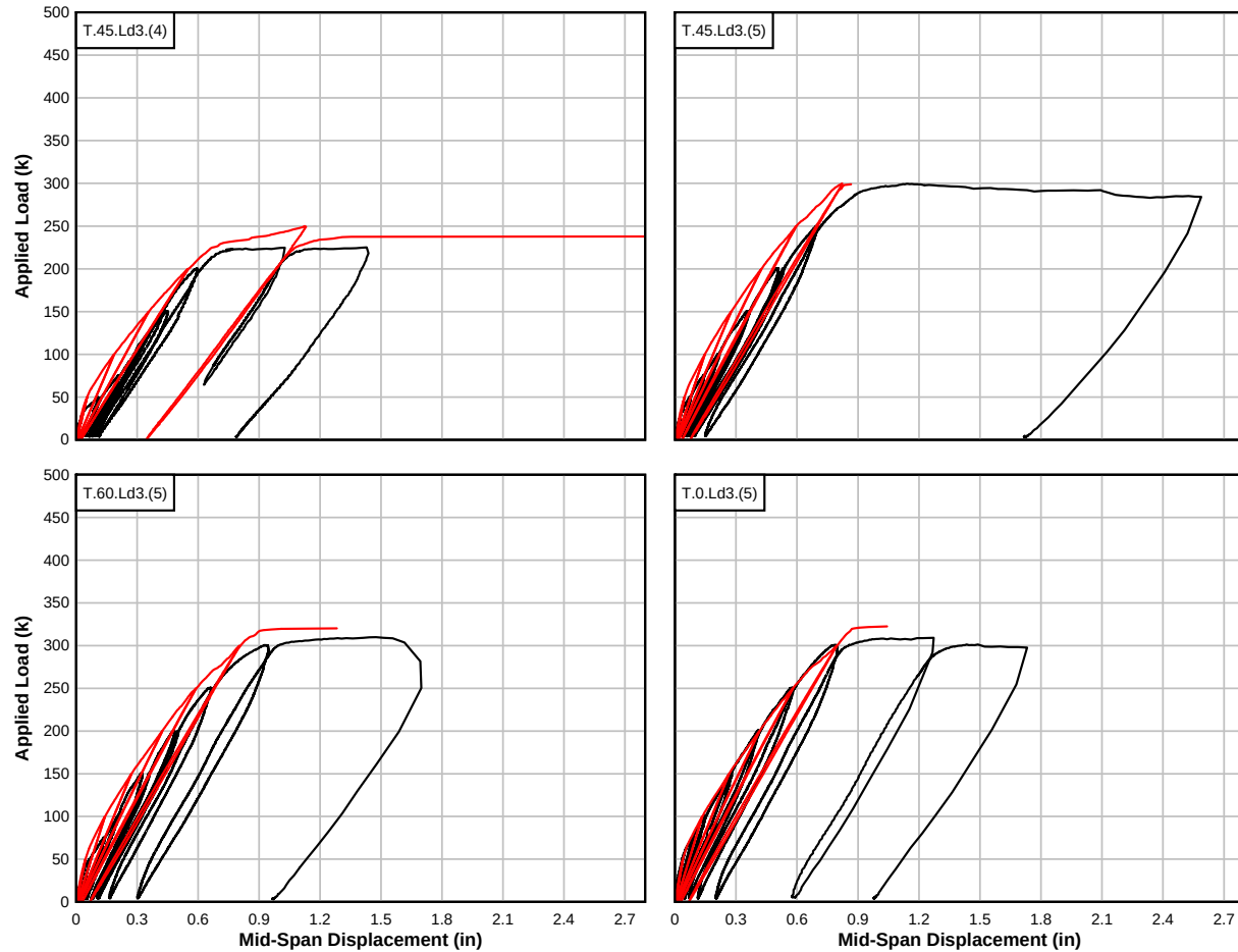
Figure 5.30: Predicted and experimental load-deformation of T-beam specimens, cyclic analysis
