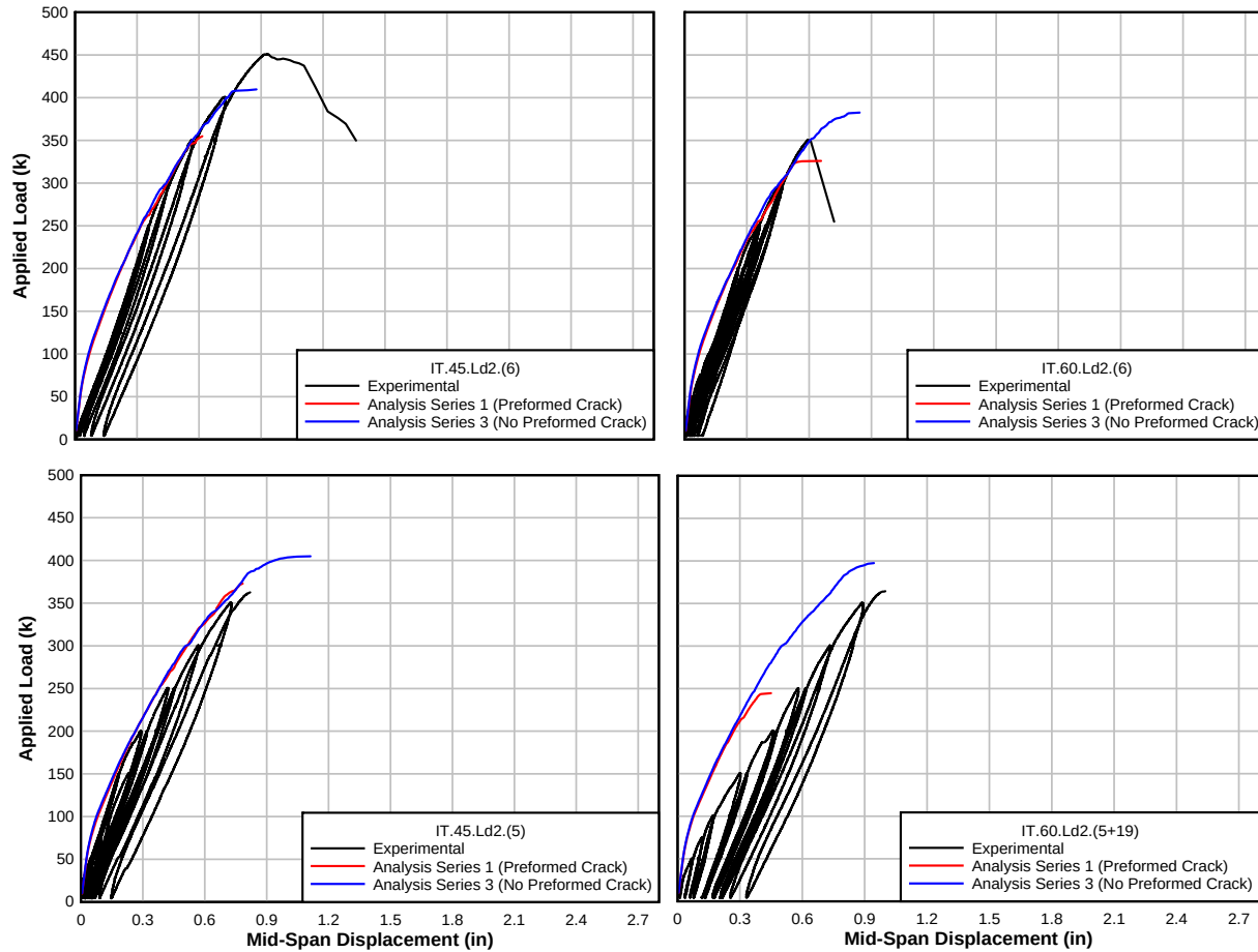
Figure 5.29: Predicted and experimental load-deformation of IT-beam specimens, monotonic analysis
