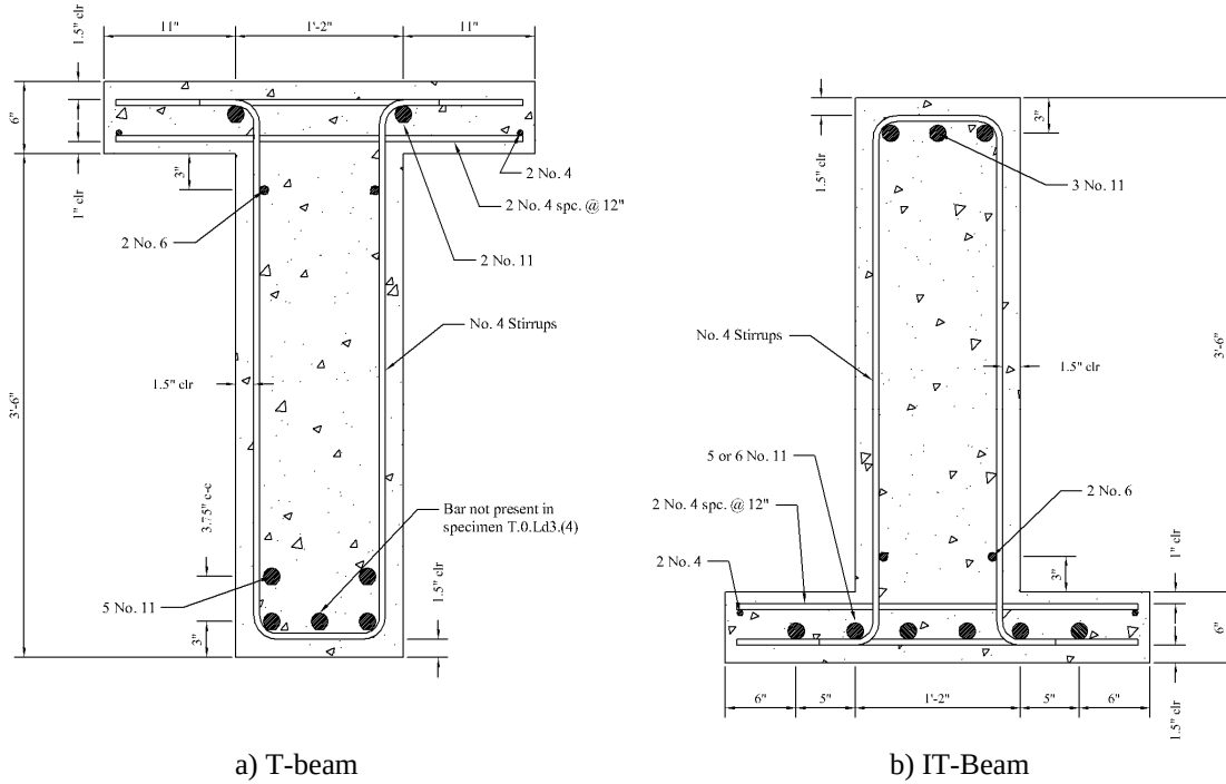
Figure 3.5: Typical specimen cross-sections
