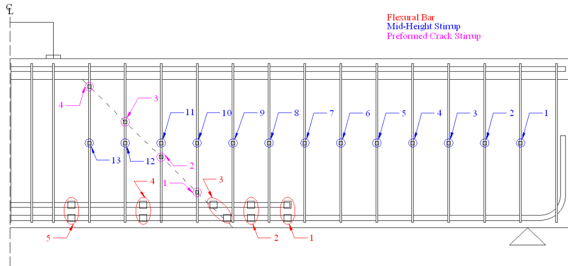
Figure A.2: Typical Specimen strain gage labeling convention
