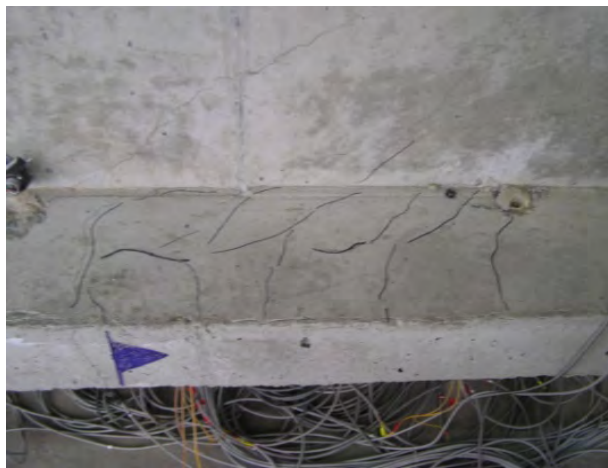
Figure C.1: Horizontal cracking along developing length of cutoff reinforcement in IT specimen
