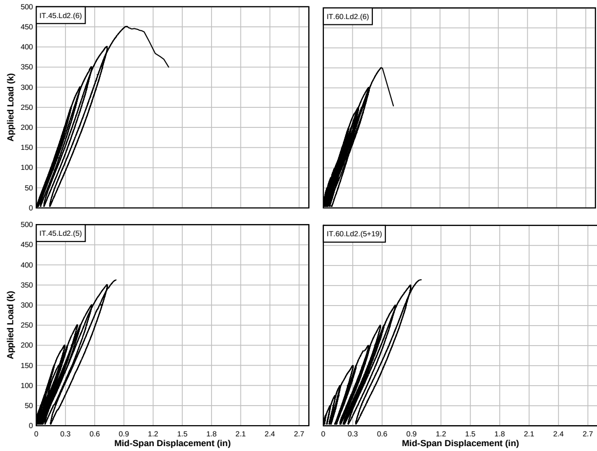
Figure A.5: Load – mid-span displacement plots for IT-beam specimens
