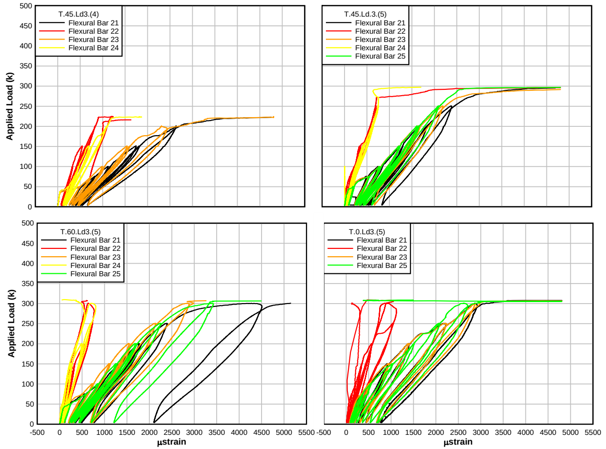
Figure A.14: Load – flexural bar location 2 strain plots for T-beam specimens
