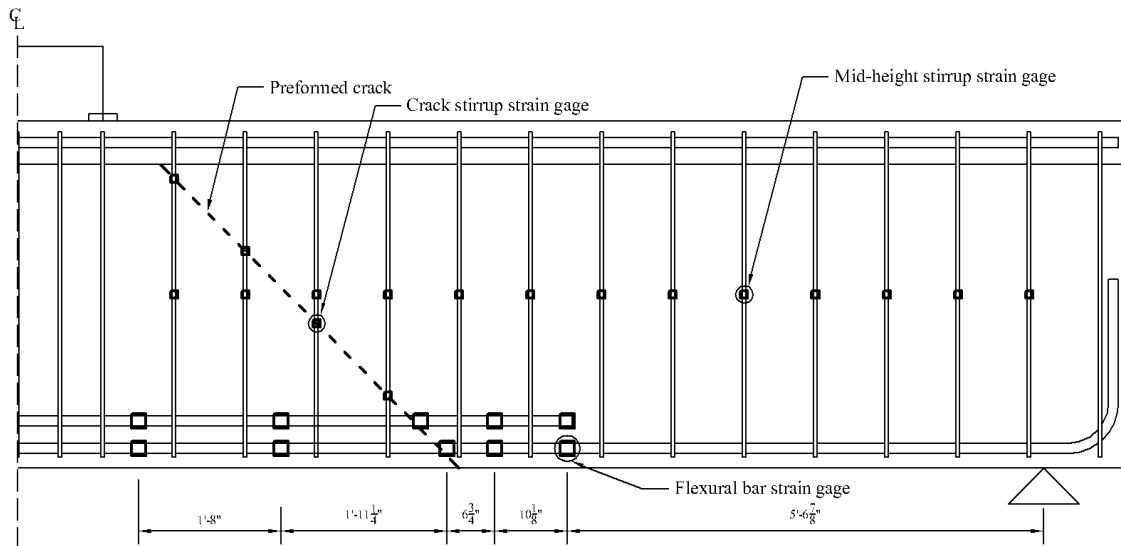
Figure 3.12: Specimens T.45.Ld3.(4) and T.45.Ld3.(5) internal sensor array
