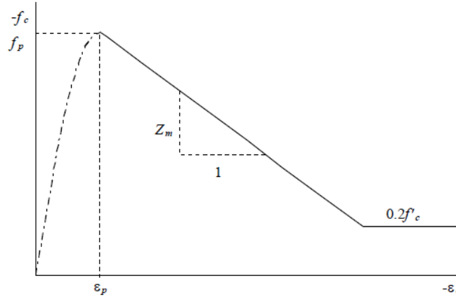
Figure D.2: Modified Park-Kent post-peak concrete compression response (Vecchio and Wong, 2002)
