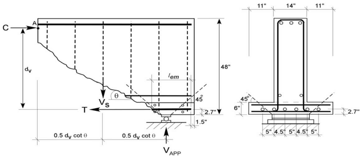
Figure 5.6: Effective region of confining stress due to supports (Higgins, et. al 2004)
