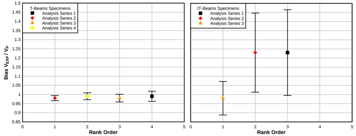
Figure 5.27: VecTor2 NLFEA ultimate shear strength prediction results
