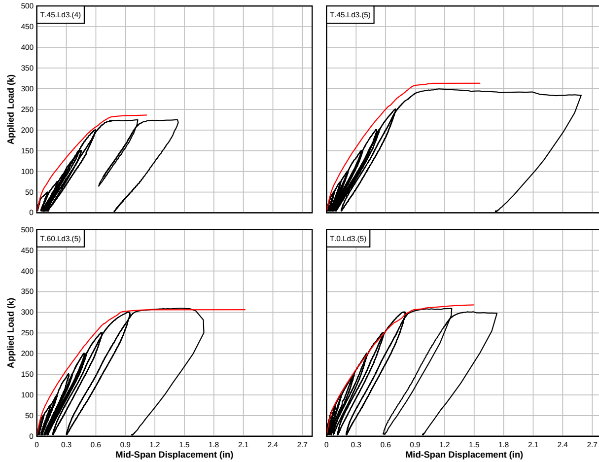
Figure 5.28: Predicted and experimental load-deformation of T-beam specimens, monotonic analysis
