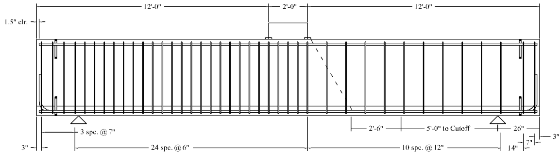
Figure 3.7: Elevation of specimen IT.60.Ld2
