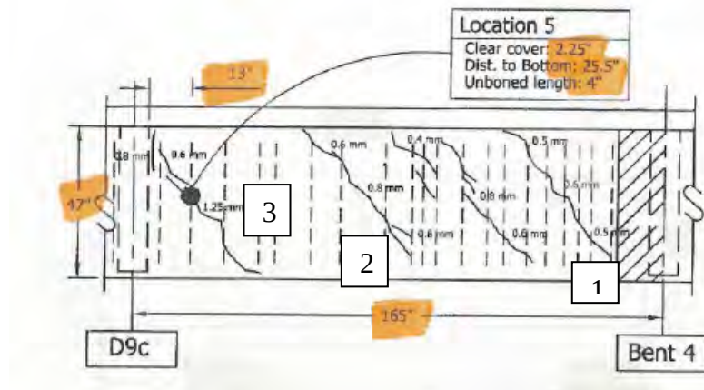
Figure B.2: Crack locations near Bent 4
