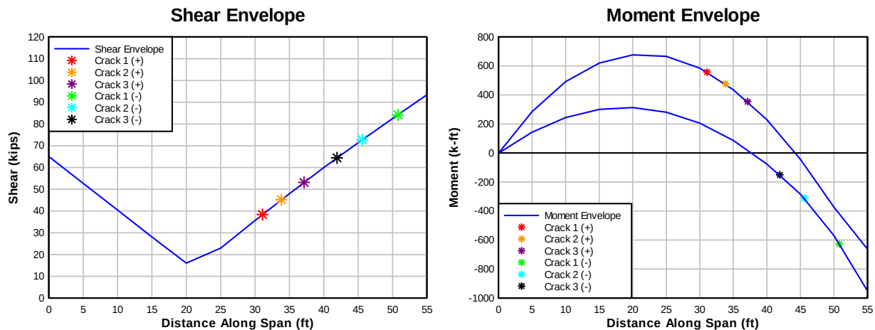
Figure B.4: Service I level shear and moment envelopes for WRB – Span 9 (similar curves developed for Strength I)
