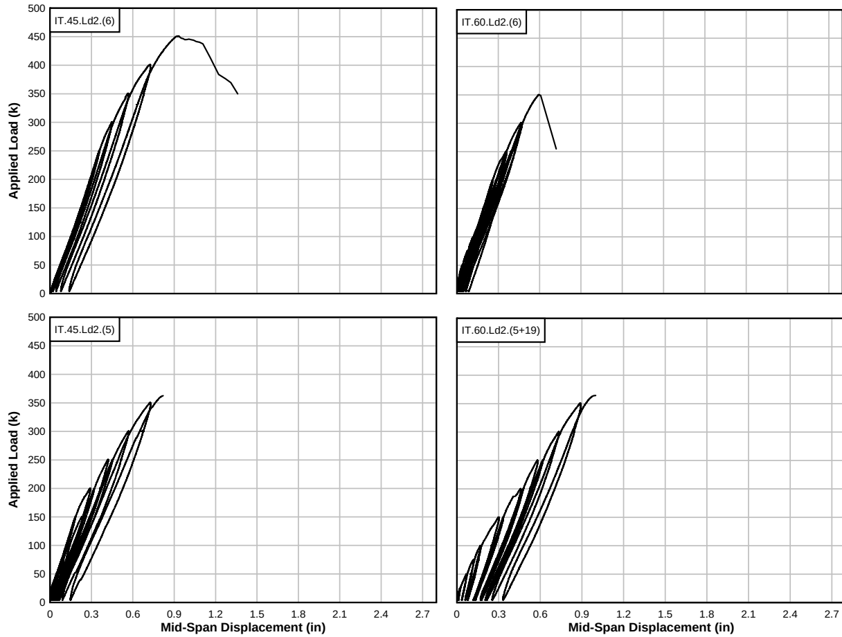
Figure 4.2: Load-displacement plots at mid-span for IT-beam specimens
