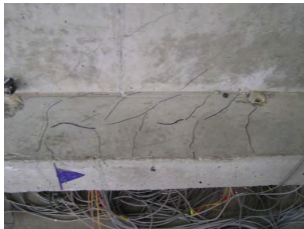
Figure 4.8: Typical anchorage cracking caused by slip of the cutoff bars in IT-beam specimens
