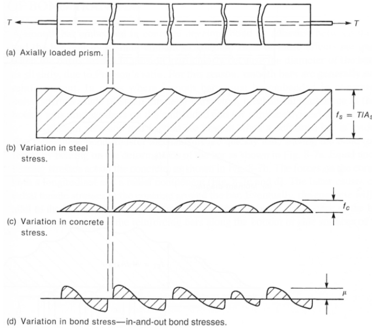
Figure 2.3: Bond stresses in a cracked prism (MacGregor and Wright 2005)
