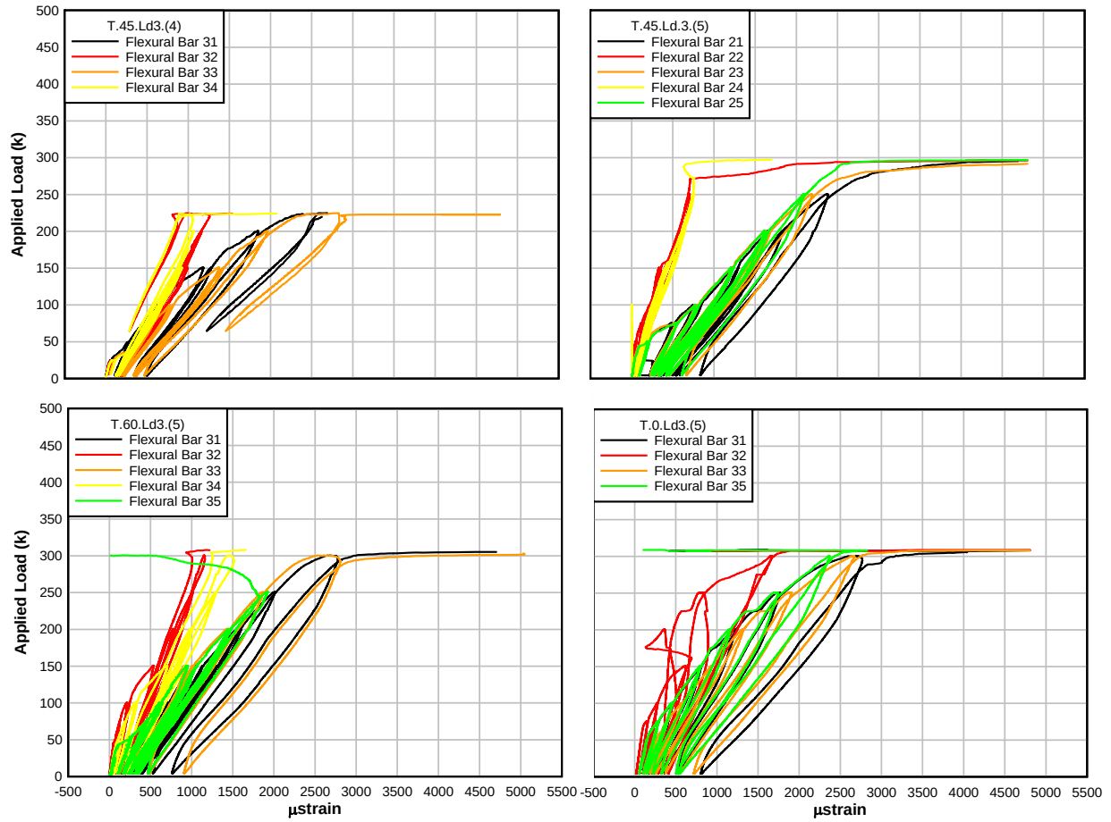
Figure A.16: Load – flexural bar location 3 strain plots for T-beam specimens
