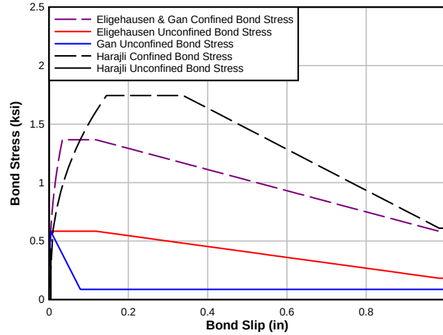
Figure 5.13: Eligehausen, Gan, and Harajli bond stress–slip response
