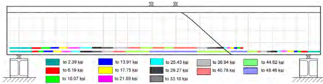
Figure 5.35: Specimen T.45.Ld3.(5) predicted steel reinforcement stresses at 234 kips
