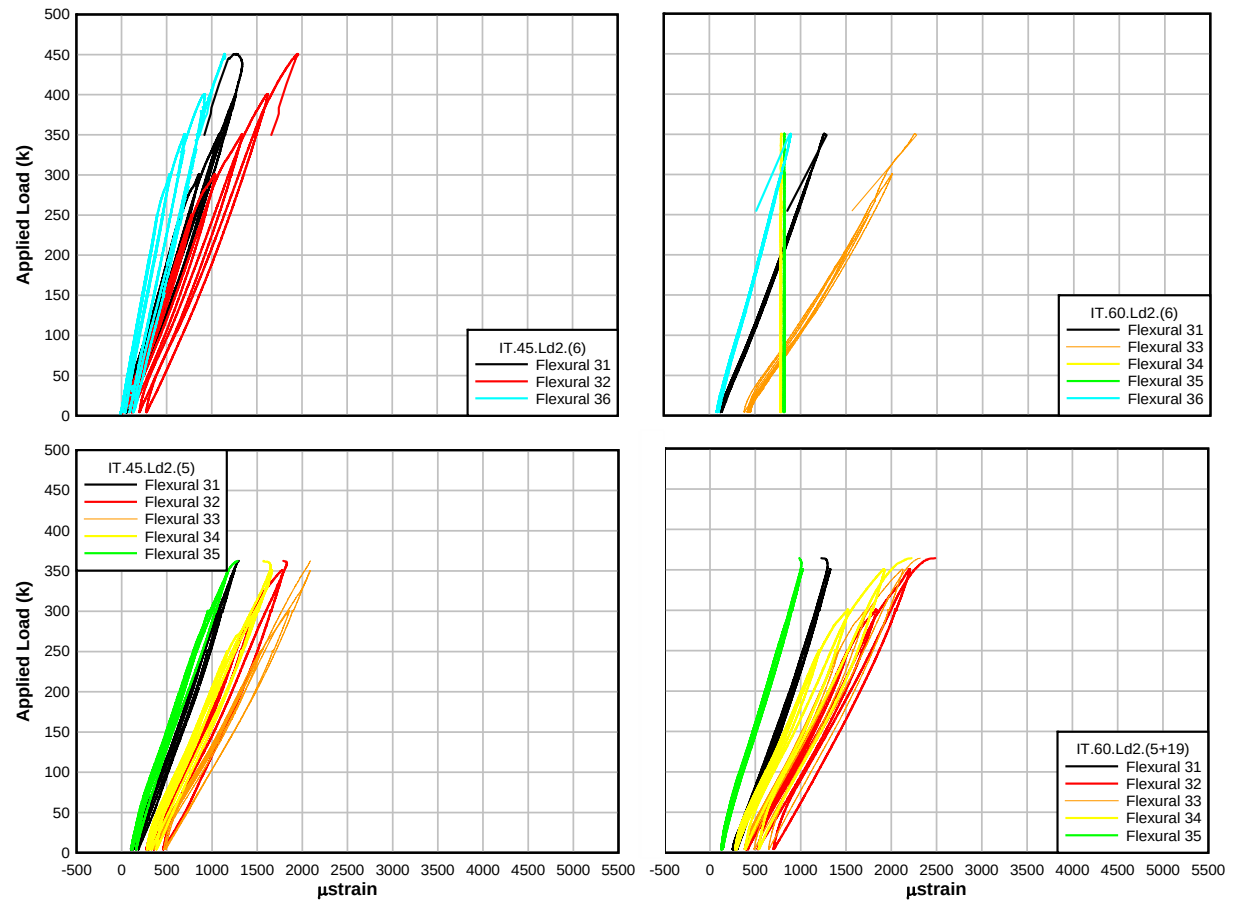
Figure A.17: Load – flexural bar location 3 strain plots for IT-beam specimens
