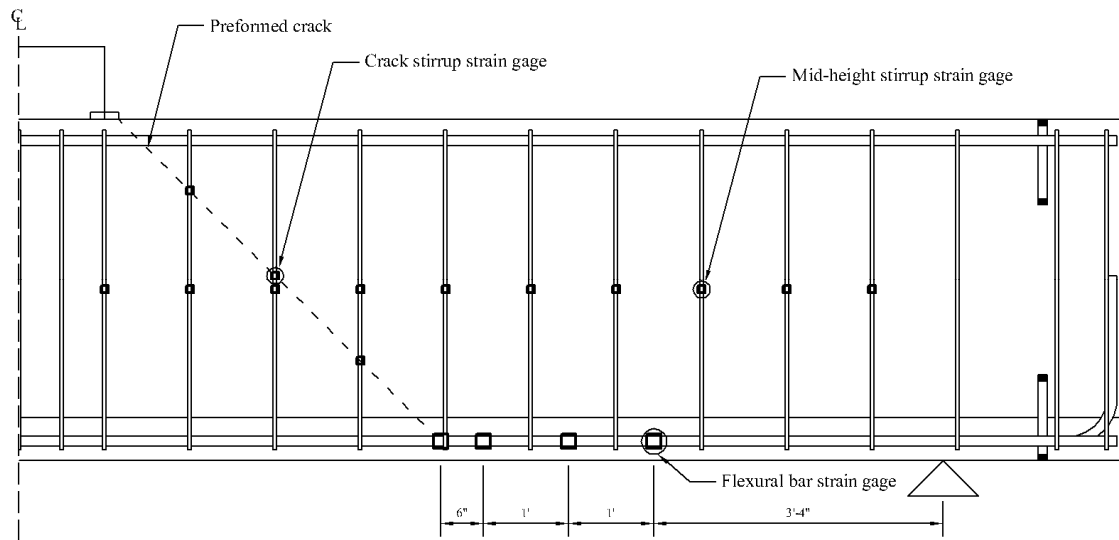
Figure 3.15: Specimen IT.45.Ld2 internal sensor array
