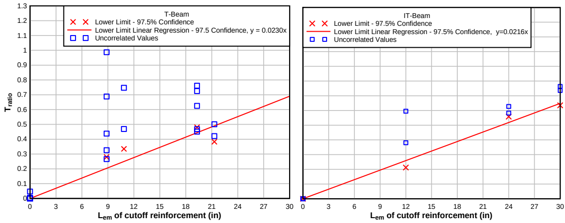
Figure 5.3: T_{ratio} analysis of the development of tension in cutoff reinforcement
