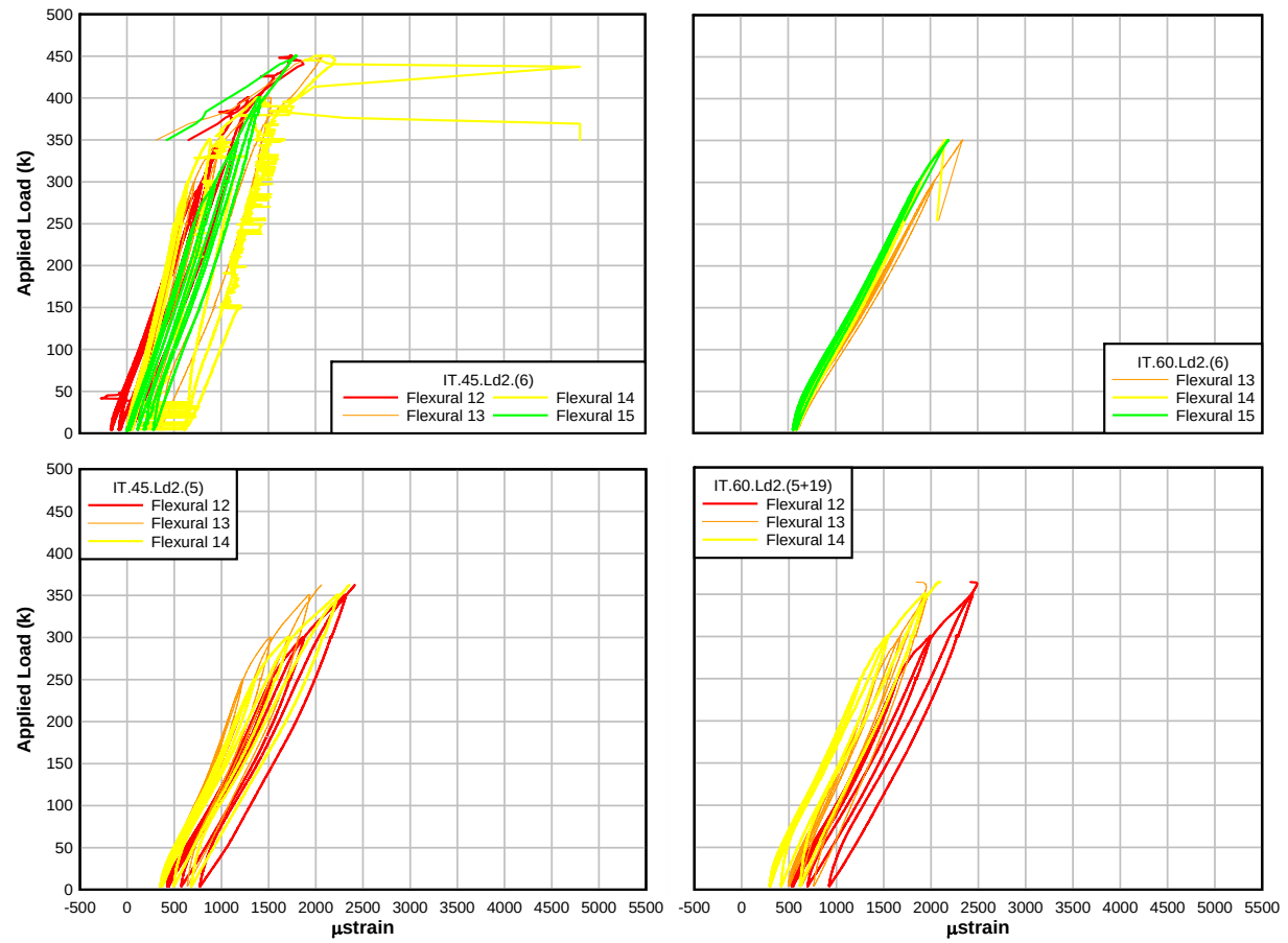
Figure A.13: Load – flexural bar location 1 strain plots for IT-beam specimens
