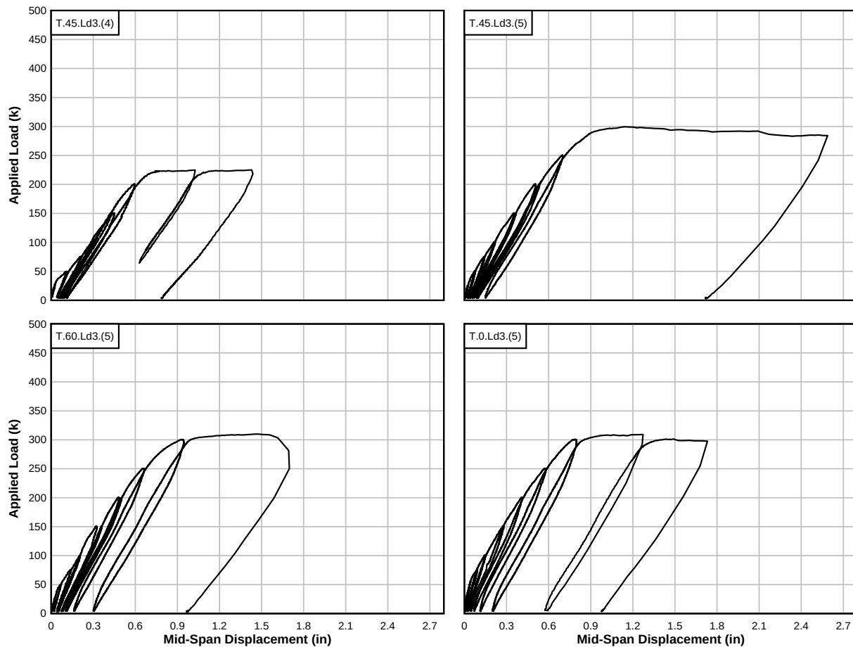
Figure 4.1: Load-displacement plots at mid-span for T-beam specimens
