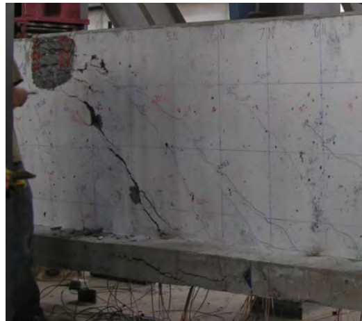
Figure C.3: Extremely wide horizontal cracking in IT specimen along developing length of cutoff bars
