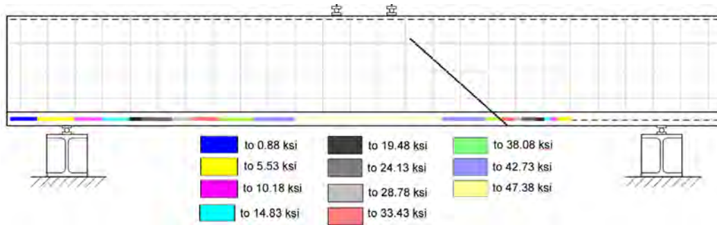
Figure 5.38: Specimen IT.45.Ld2.(6) predicted steel reinforcement stresses at failure
