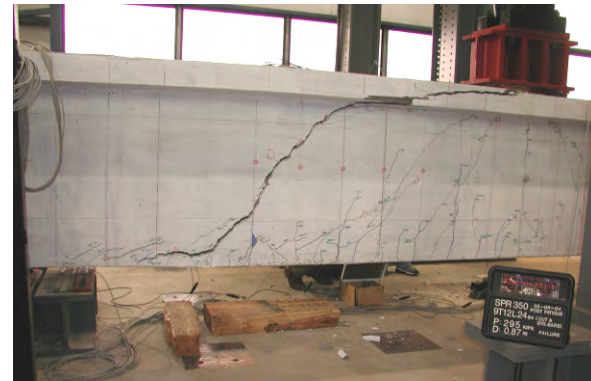
Figure 5.10: Specimen 9T12-B4 load-deflection plot and failure photo (Higgins, et al. 2004)
