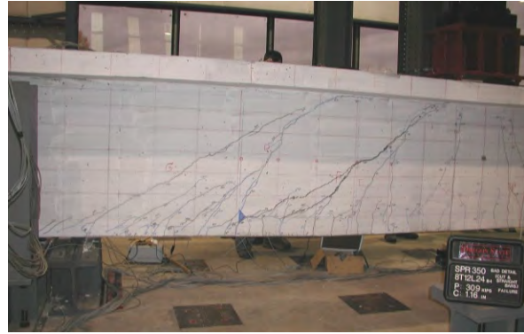
Figure 5.9: Specimen 8T12-B4 load-deflection plot and failure photo (Higgins, et al. 2004)
