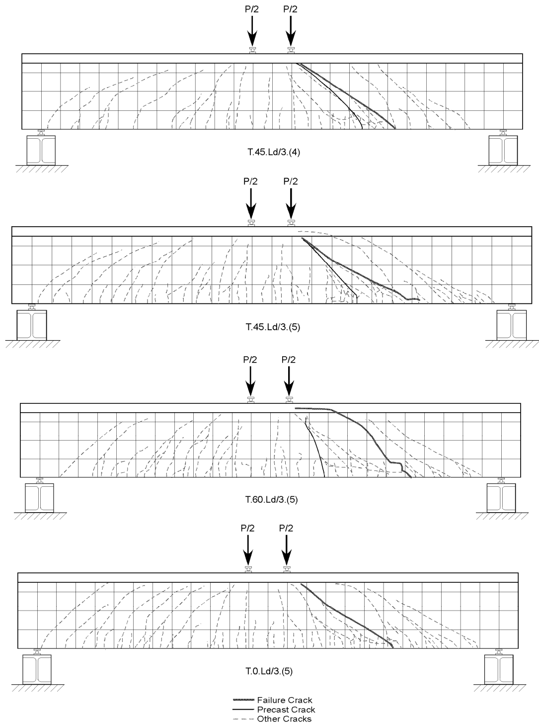
Figure 4.3: Failure crack maps for T-beam specimens
