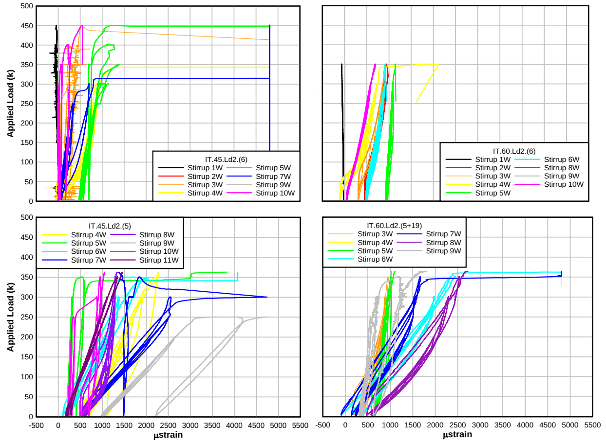
Figure A.22: Load – west mid-height stirrup strain plots for IT-beam specimens
