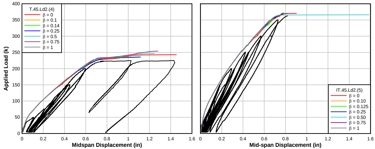
Figure 5.22: Predicted load-deformation response for different \beta values (specimen T.45.Ld3.(4))
