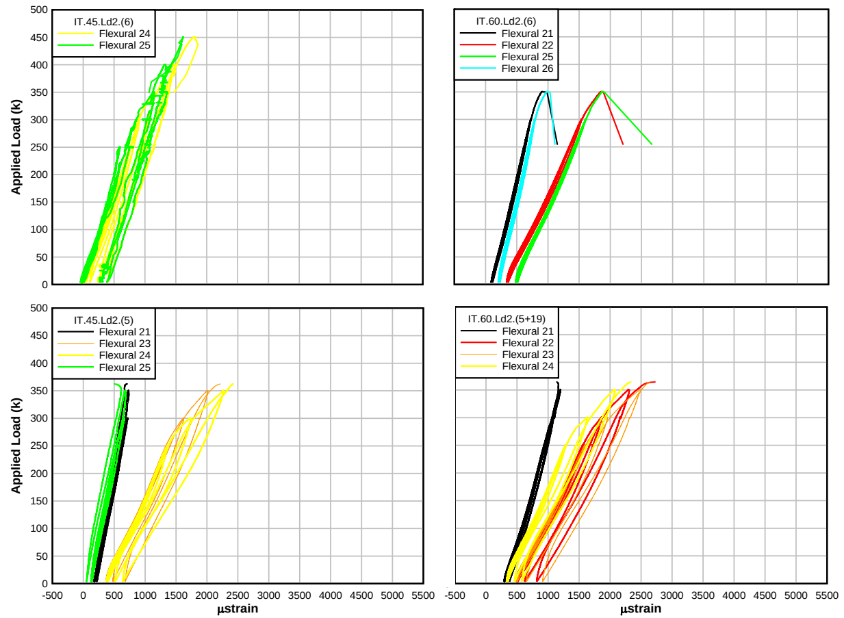
Figure A.15: Load – flexural bar location 2 strain plots for IT-beam specimens
