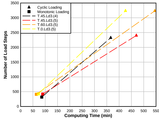
Figure 5.31: Computation time for monotonic and cyclic analyses
