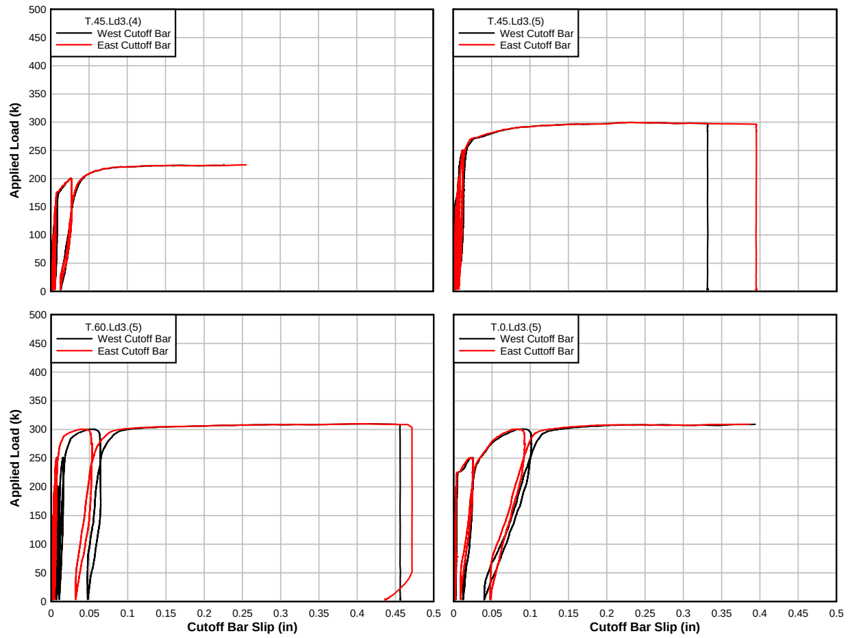
Figure 4.9: Load-cutoff bar slippage plots for T-beam specimens
