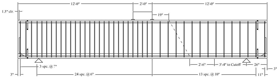
Figure 3.9: Elevation of specimen IT.60.Ld2(5+19)
