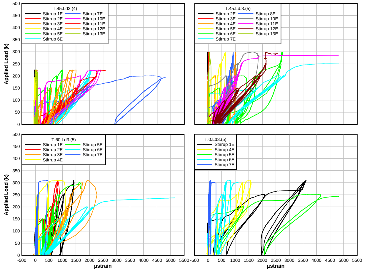
Figure A.23: Load – east mid-height stirrup stain plots for T-beam specimens
