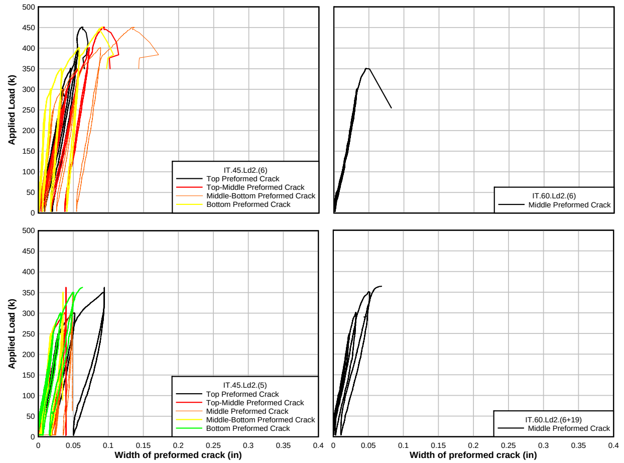
Figure A.9: Load – preformed crack width plots for IT-beam specimens
