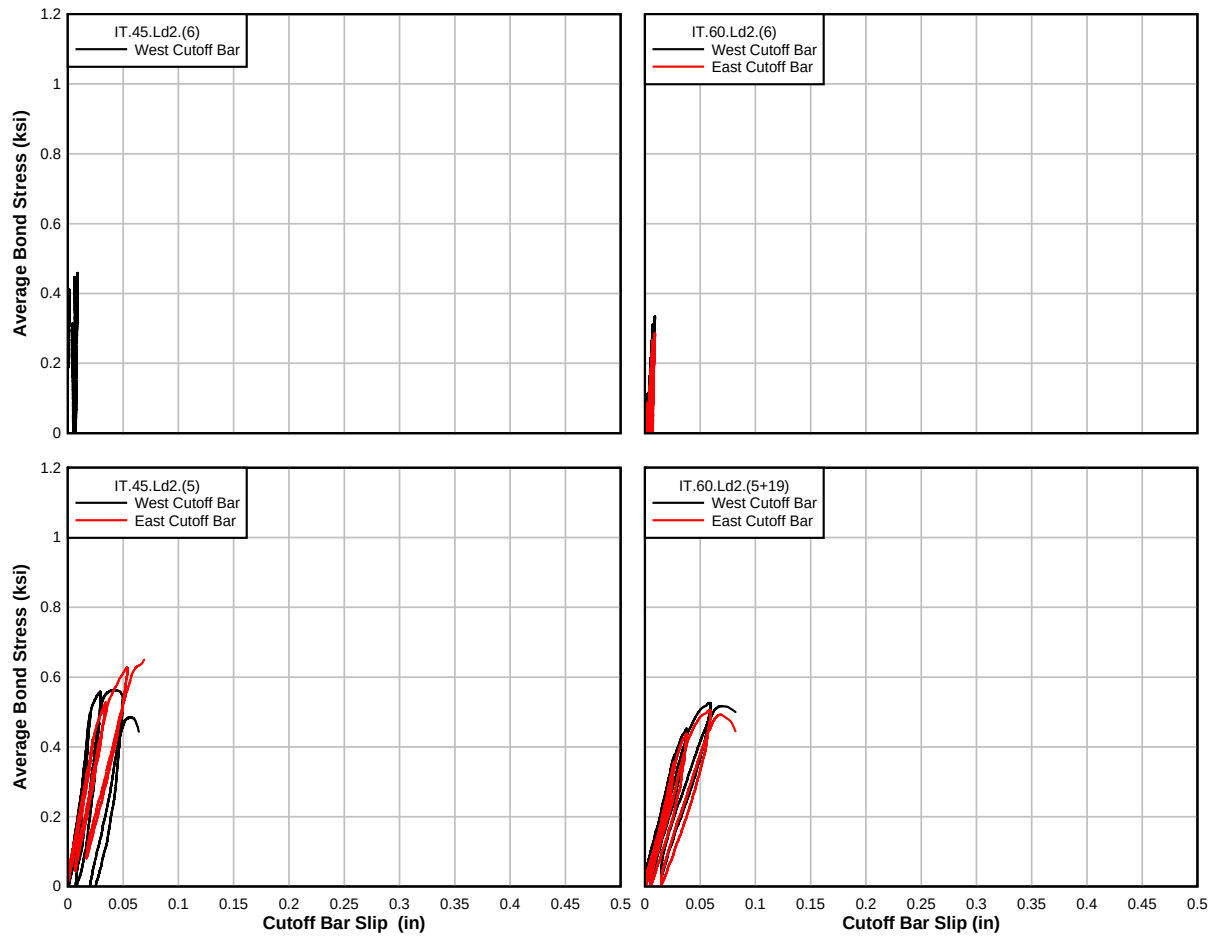
Figure 4.14: Bond stress – cutoff bar slip comparison for IT-beams
