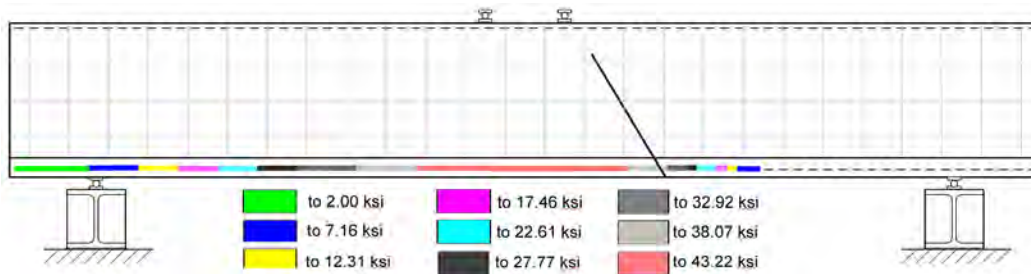
Figure 5.39: Specimen IT.60.Ld2.(6) predicted steel reinforcement stresses at failure
