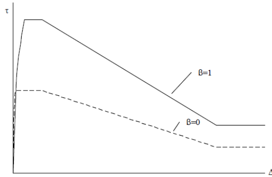
Figure D.7: Eligehausen bond stress-slip response (Vecchio and Wong, 2002)
