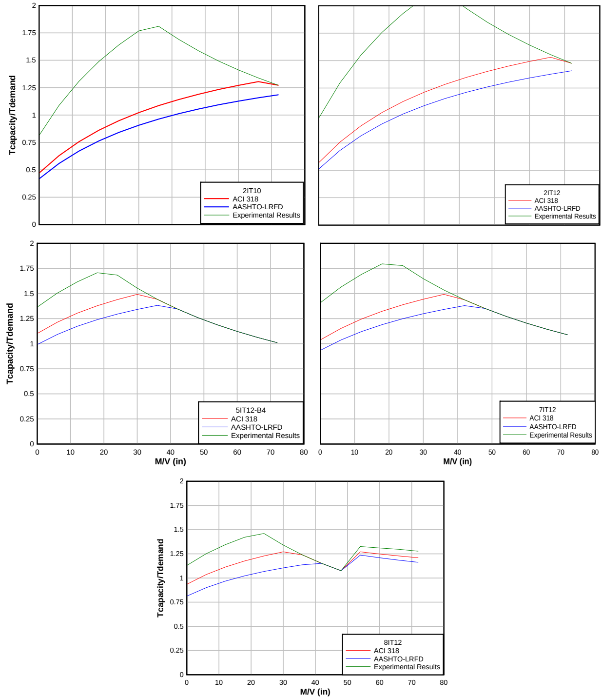
Figure 5.12: Tensile capacity - demand for each type of anchorage analysis using evaluation method two
