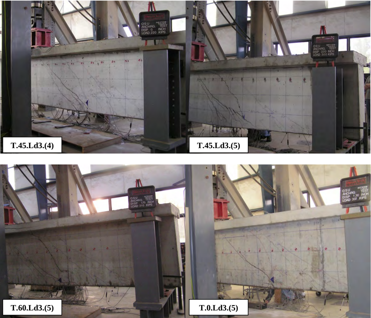
Figure 4.5: Digital photographs at failure of T-beam specimens
