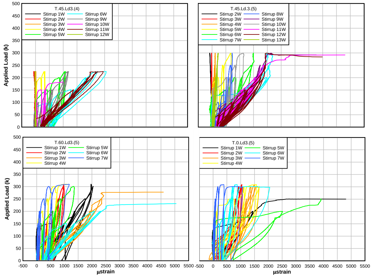
Figure A.21: Load – west mid-height stirrup strain plots for T-beam specimens
