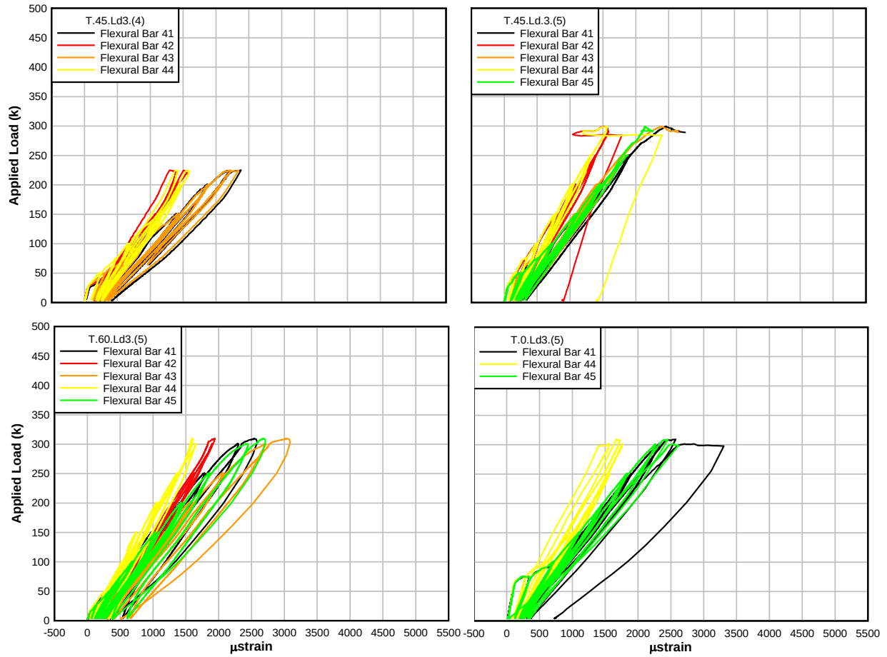
Figure A.18: Load – flexural bar location 4 strain plots for T-beam specimens
