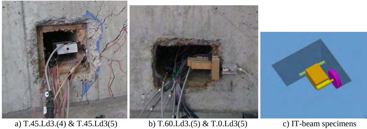
Figure 3.21: Typical anchorage slip sensor installation
