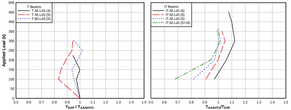
Figure 4.12: Comparison of predicted AASHTO-LRFD tensile demand to actual demand at increasing load steps
