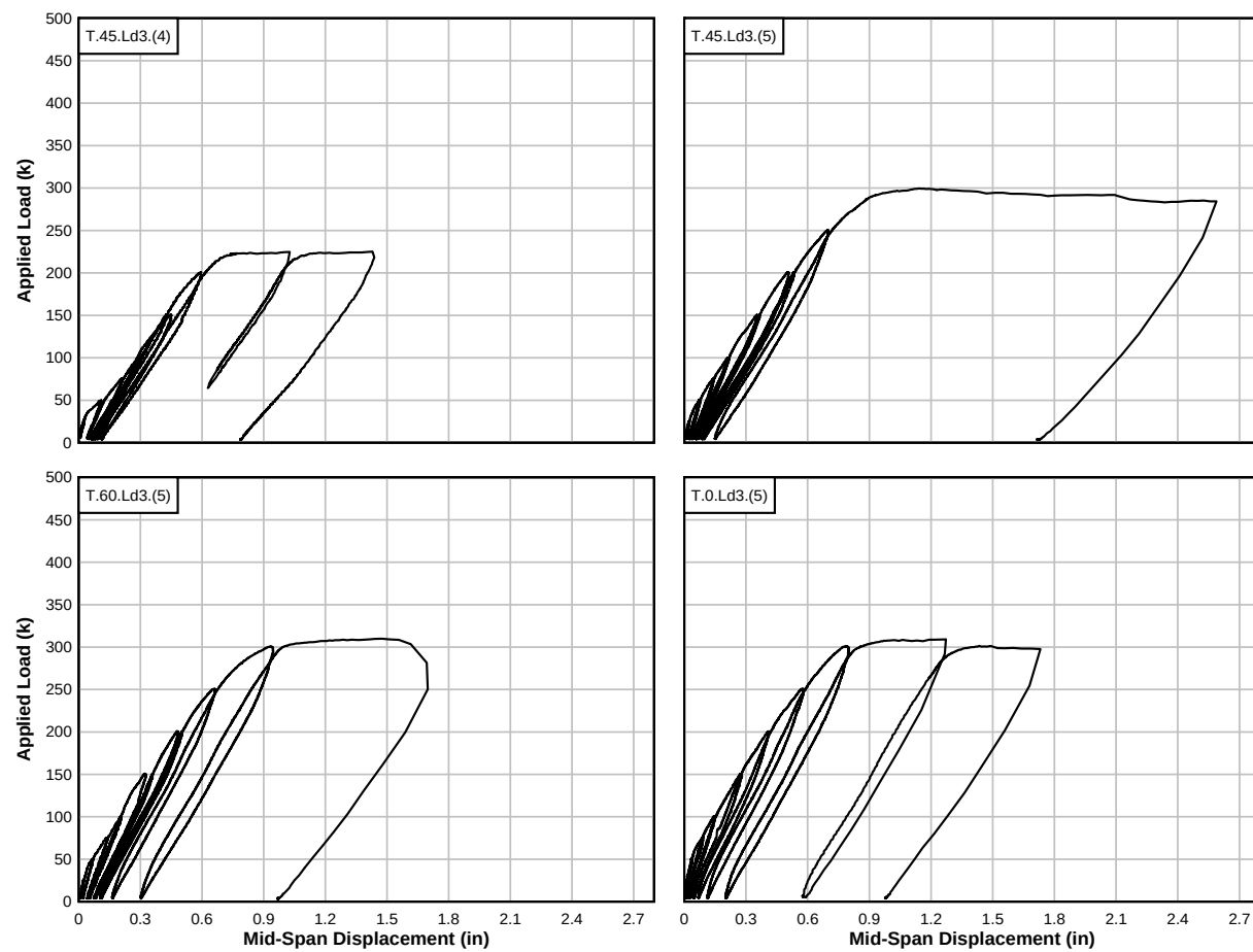
Figure A.4: Load – mid-span displacement plots for T-beam specimens
