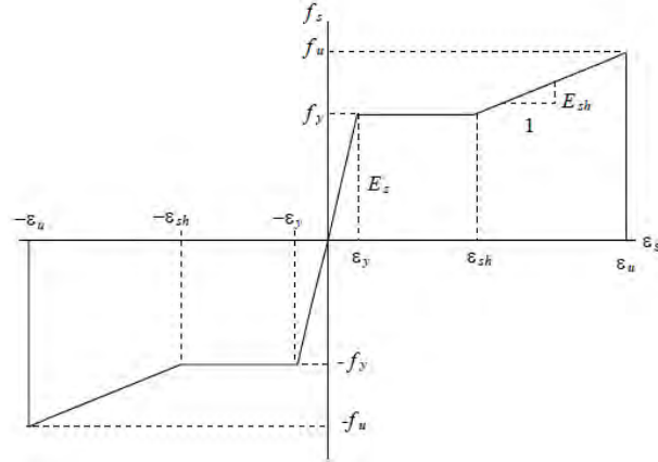
Figure D.6: Ductile steel reinforcement stress-strain response (Vecchio and Wong, 2002)
