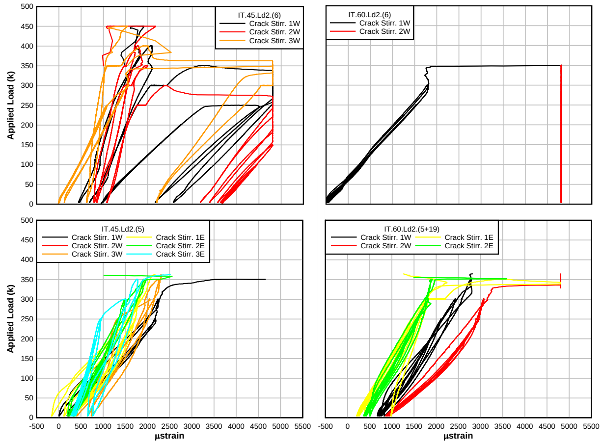
Figure A.26: Load – preformed crack stirrup stain plots for IT-beam specimens
