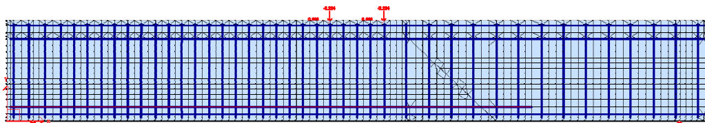
Figure 5.15: Specimen T.45.Ld3.(5) finite element model
