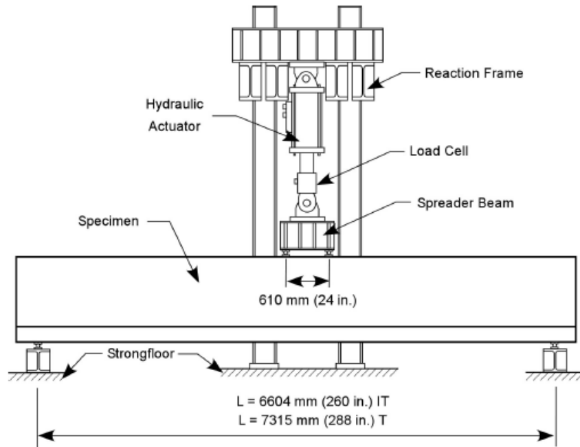
Figure 3.11: Four-point load configuration used for specimen testing
