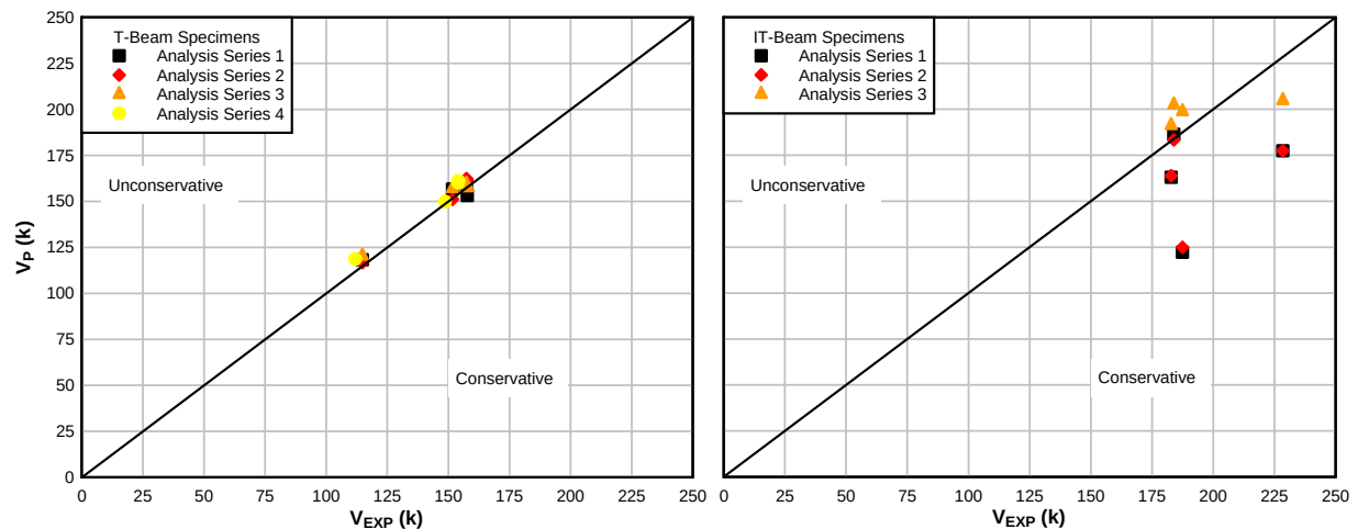
Figure 5.26: VecTor2 NLFEA ultimate shear strength prediction results
