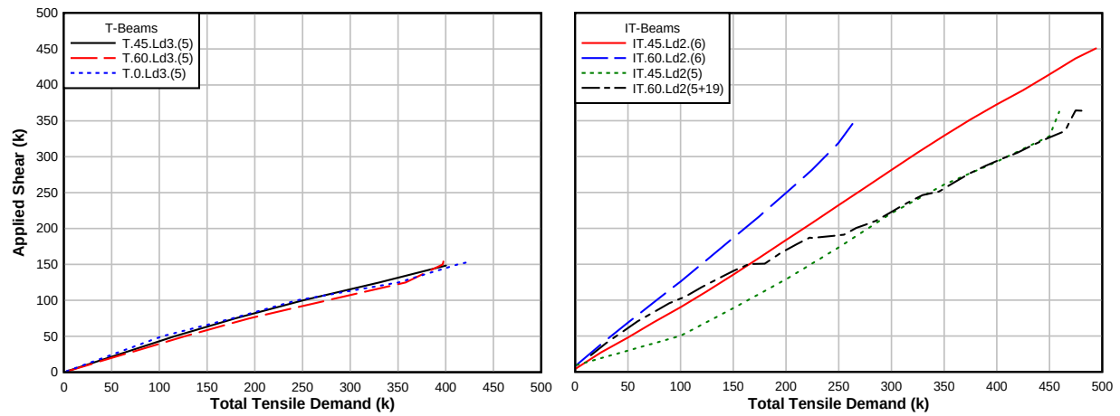
Figure 4.11: Average tensile demand at preformed diagonal crack location for T-beam specimens
