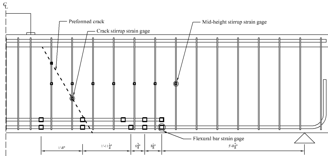
Figure 3.13: Specimen T.60.Ld3(5) internal sensor array
