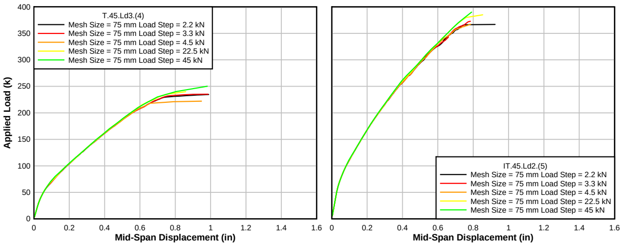
Figure 5.25: Predict load-deformation response for different load step sizes
