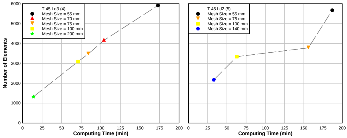
Figure 5.24: Computing time for different mesh sizes (specimen T.45.Ld3.(4))
