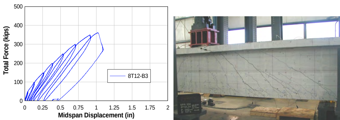
Figure 5.8: Specimen 8T12-B3 load-deflection plot and failure photo (Higgins, et al. 2004)
