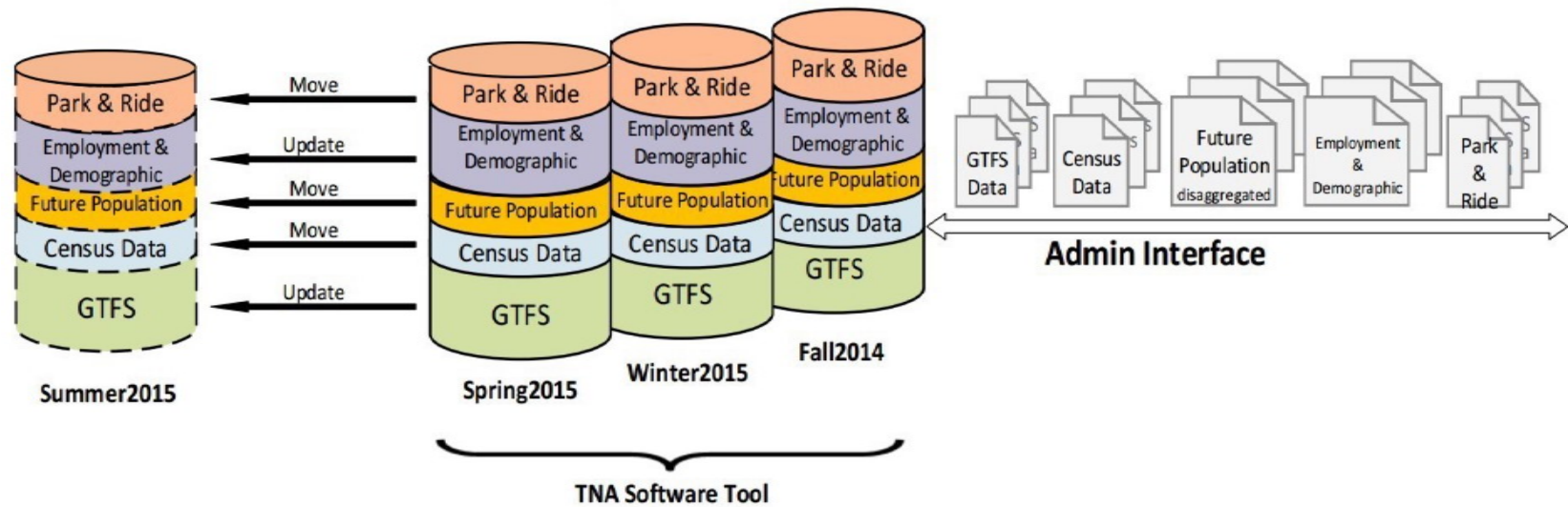
Figure 3.1: Data sources and the structure of the PostgreSQL relational databases supporting the TNA software tool
