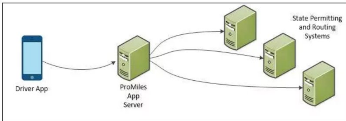
Figure 8.1: ProMiles Architecture
