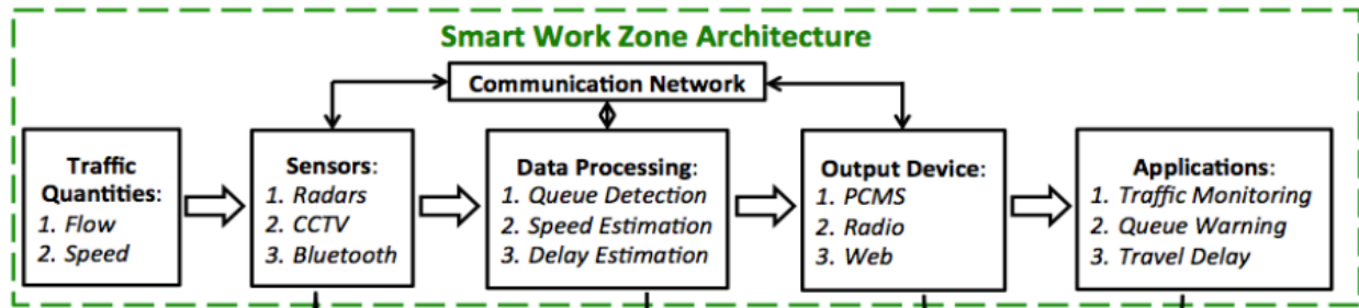
Figure 2.1: Smart Work Zone Overview (Li et al., 2016)
