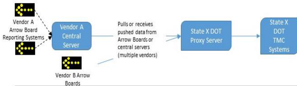
Figure 2.4: Arrow Board Reporting Systems (ACC, 2017a)
