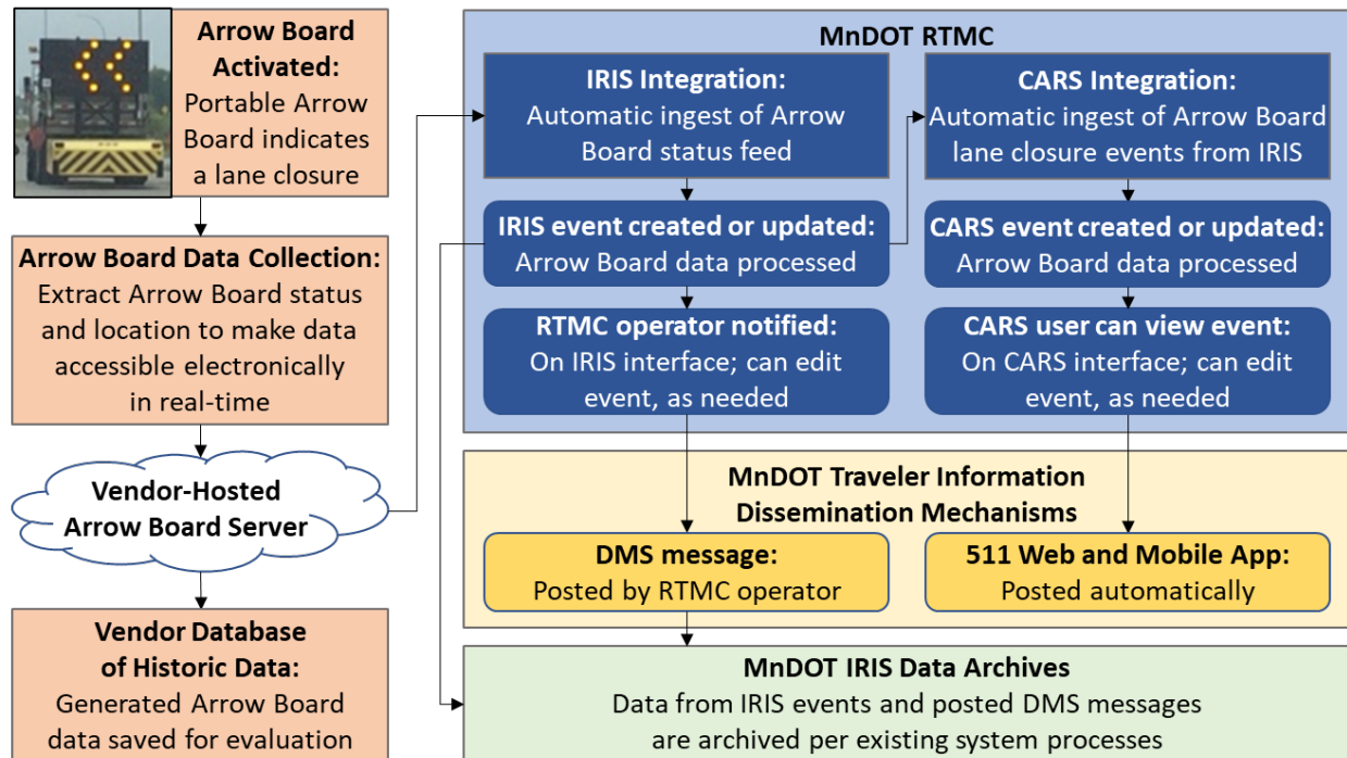
Figure 2.7: Minnesota SAB project system data transmission pipeline
