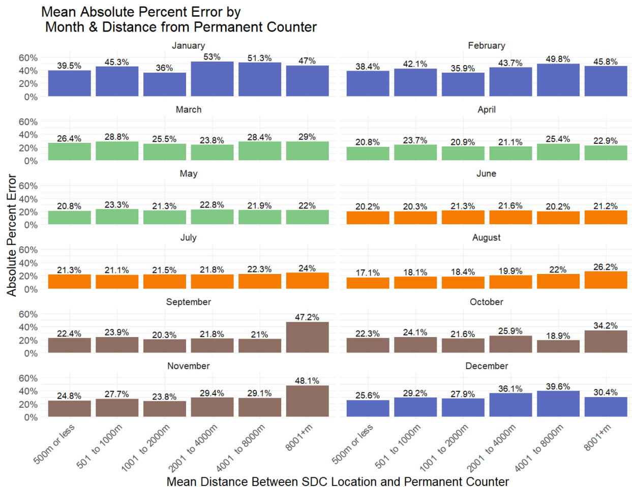
Figure 3.16: Mean Average Error from Annual Factoring Method Testing
