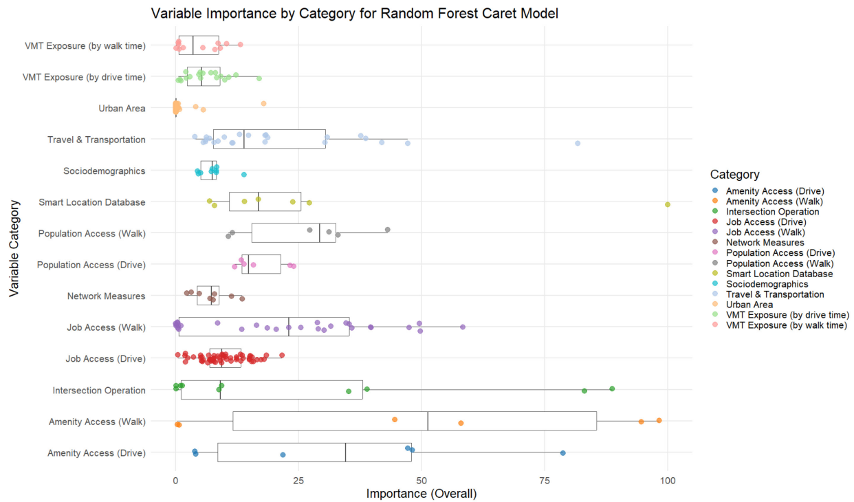
Figure 3.25: Variable Importance by Category for Random Forest Caret Model
