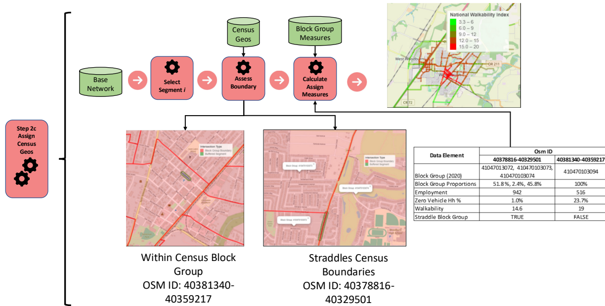
Figure 3.5: Step 2c – Process Example for Assigning Census Boundaries to Segments
