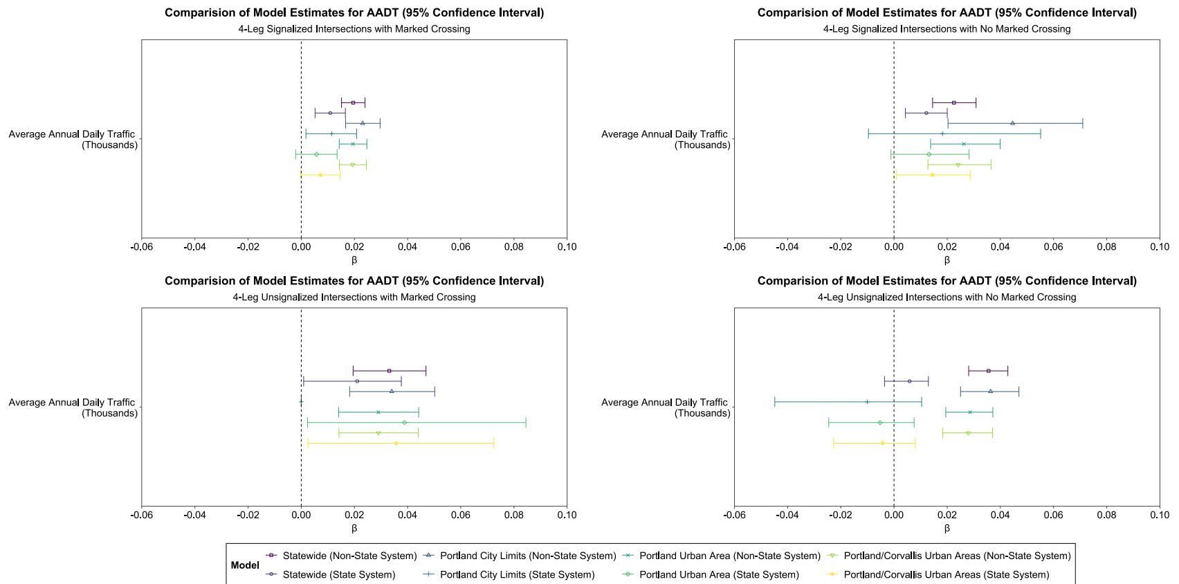
Figure 4.17: Comparison of Model Estimates for AADT Between 4-Leg Intersection Models
