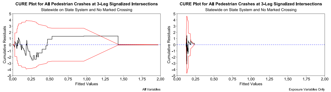
Figure A.21: Comparison of CURE Plots Between Full Model and Exposure-Only Model at 3-Leg Signalized Intersections, Statewide, on State System, and No Marked Crossing
