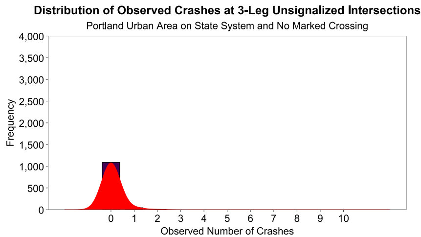
Figure D.15: Distribution of Observed Crashes at 3-Leg Unsignalized Intersections on State System with No Marked Crossing
