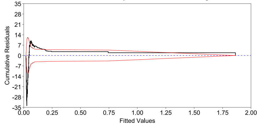
CURE Plot for All Pedestrian Crashes at 3-Leg Unsignalized Intersections Portland Urban Area on State System and No Marked Crossing
