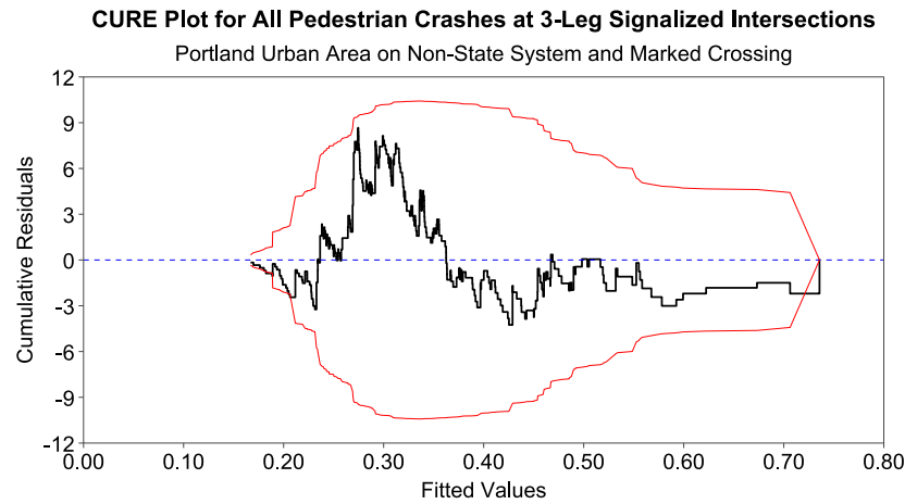
Figure 4.10: CURE Plots for 3-Leg Signalized Intersections and Marked Crossing (a) Statewide, (b) Portland City Limits, (c) Portland Urban Area, and (d) Portland/Corvallis Urban Areas on Non-State System
