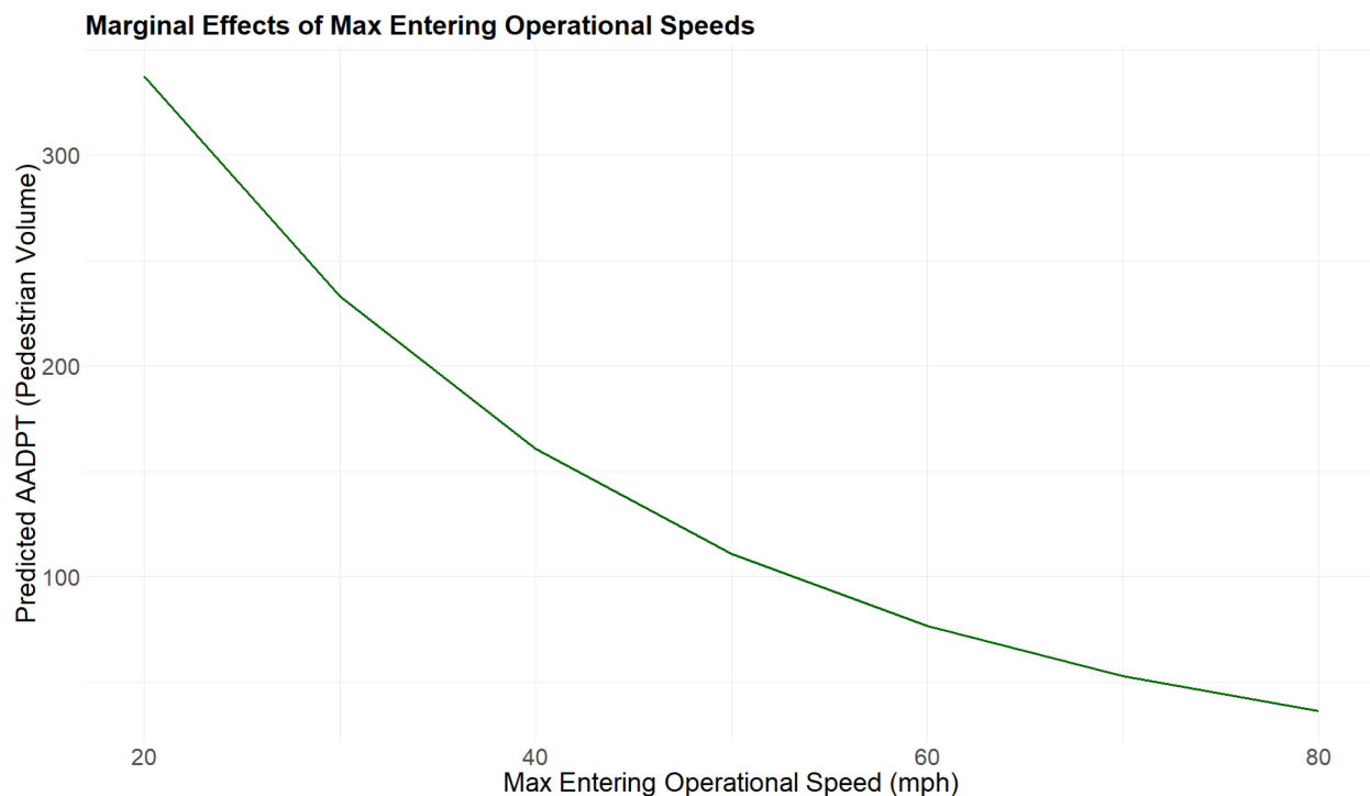
Figure 3.19: Max Operational Speed Marginal Effects on AADPT
