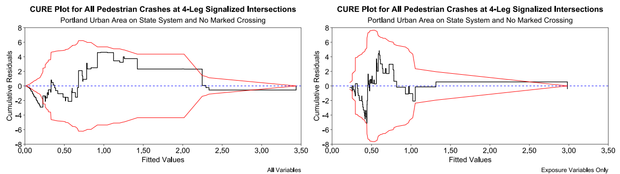
Figure A. 12: Comparison of CURE Plots Between Full Model and Exposure-Only Model at 4-Leg Signalized Intersections, Portland Urban Area, on State System, and No Marked Crossing
