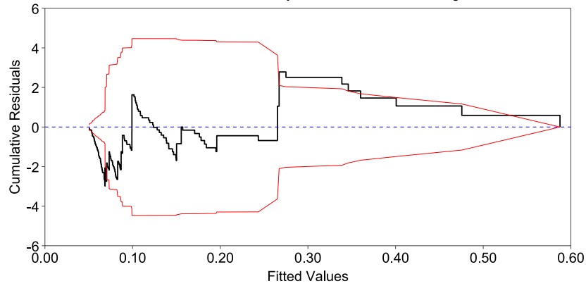
CURE Plot for All Pedestrian Crashes at 3-Leg Unsignalized Intersections
