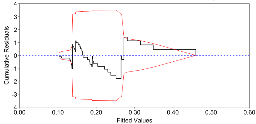
Figure 4.13: CURE Plots for 3-Leg Unsignalized Intersections and Marked Crossing (a) Statewide, (b) Portland City Limits, (c) Portland Urban Area, and (d) Portland/Corvallis Urban Areas on State System
