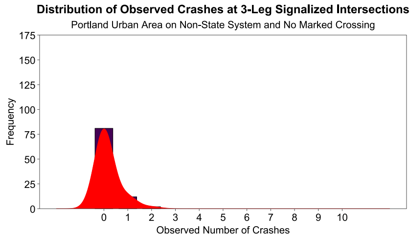
Figure D.12: Distribution of Observed Crashes at 3-Leg Signalized Intersections on Non-State System with No Marked Crossing
