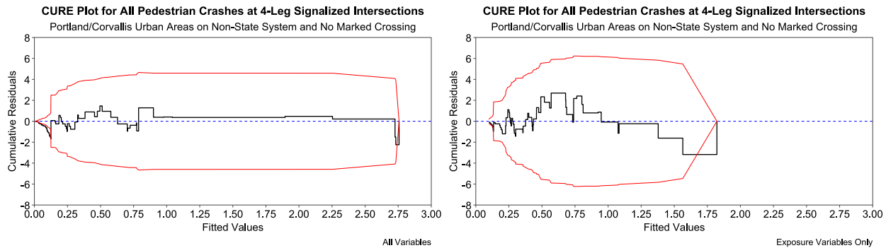
Figure A.14: Comparison of CURE Plots Between Full Model and Exposure-Only Model at 4-Leg Signalized Intersections, Portland/Corvallis Urban Areas, on Non-State System, and No Marked Crossing
