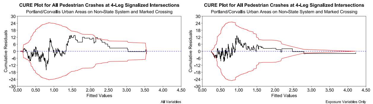
Figure A.8: Comparison of CURE Plots Between Full Model and Exposure-Only Model at 4-Leg Signalized Intersections, Portland/Corvallis Urban Areas, on Non-State System, and Marked Crossing
