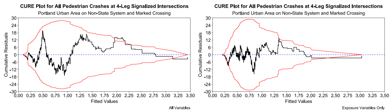
Figure A.6: Comparison of CURE Plots Between Full Model and Exposure-Only Model at 4-Leg Signalized Intersections, Portland Urban Area, on Non-State System, and Marked Crossing
