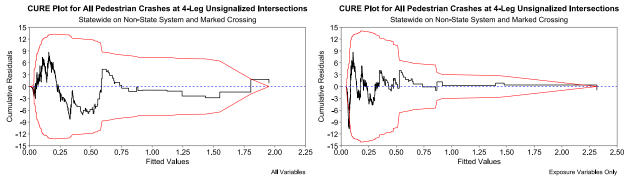
Figure A. 16: Comparison of CURE Plots Between Full Model and Exposure-Only Model at 4-Leg Unsignalized Intersections, Statewide, on Non-State System, and Marked Crossing
