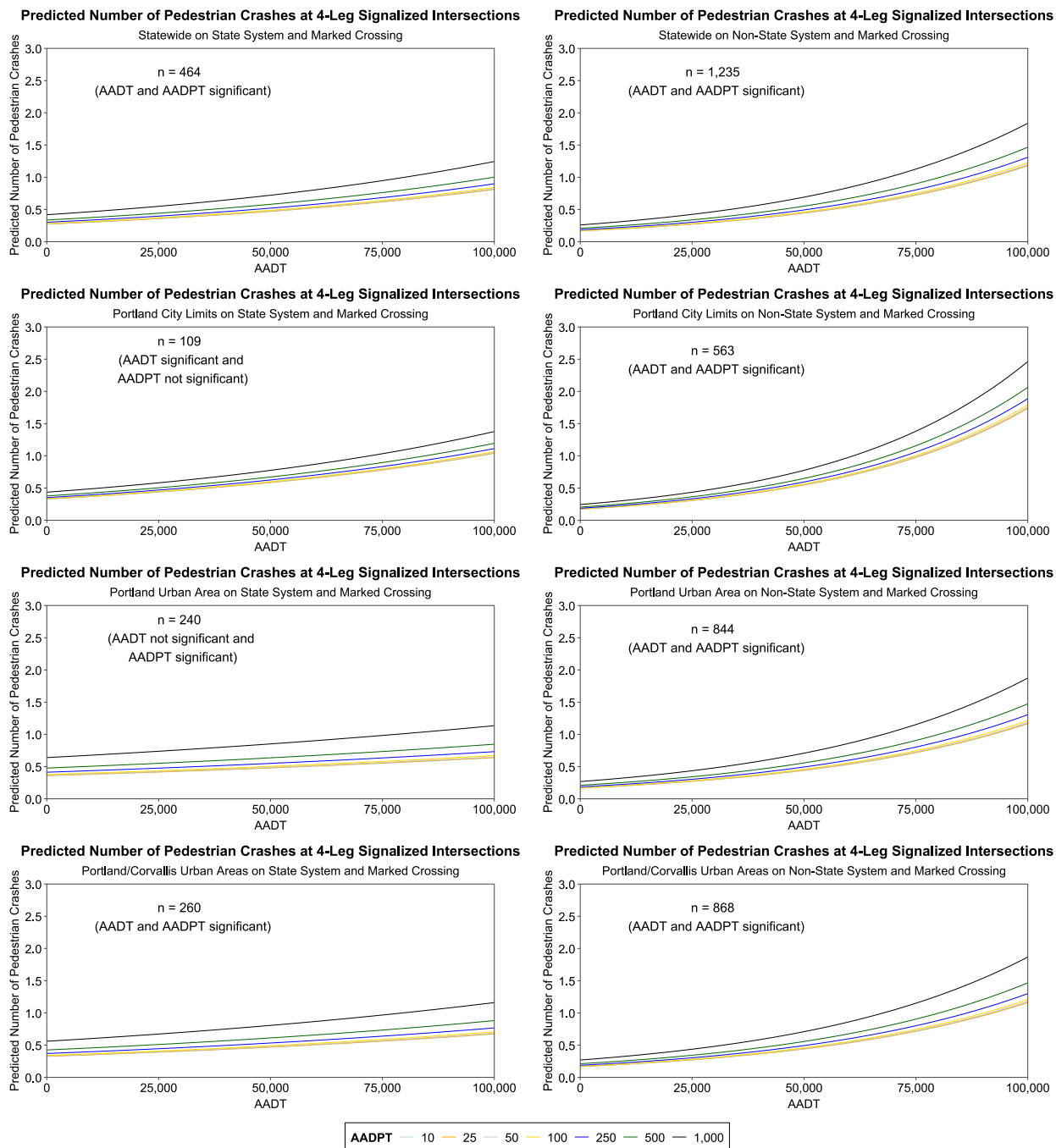
Figure 4.19: Predicted Number of Pedestrian Crashes at 4-Leg Signalized Intersections with Marked Crossing
