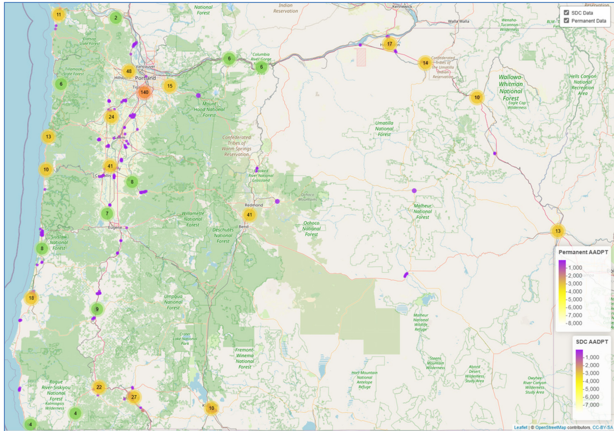
Figure 3.17: Statewide Locations of SDC and Permanent Count Locations
