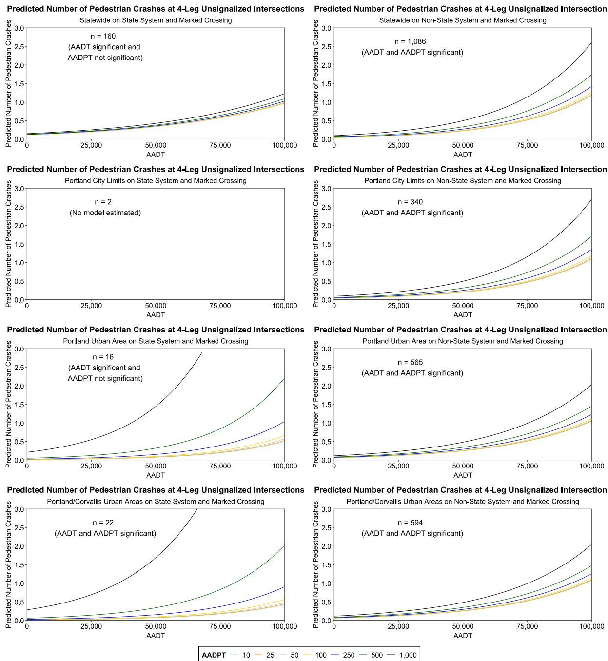
Figure 4.21: Predicted Number of Pedestrian Crashes at 4-Leg Unsignalized Intersections with Marked Crossing
