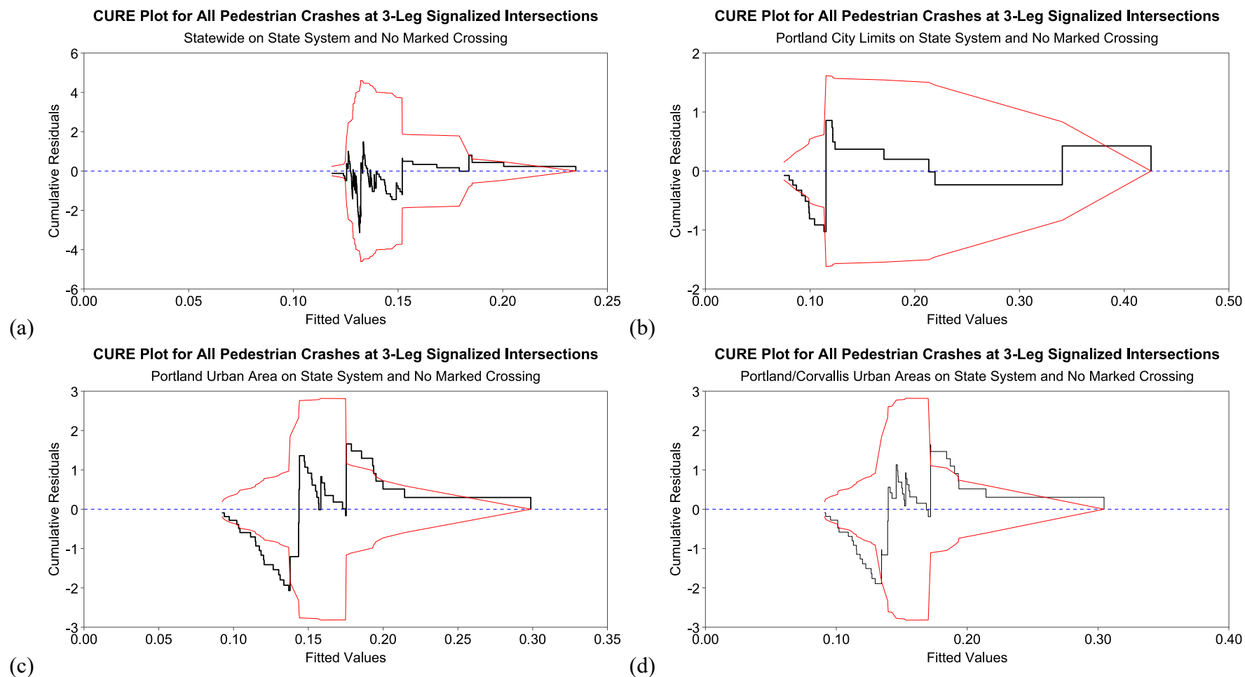
Figure 4.11: CURE Plots for 3-Leg Signalized Intersections and No Marked Crossing (a) Statewide, (b) Portland City Limits, (c) Portland Urban Area, and (d) Portland/Corvallis Urban Areas on State System
