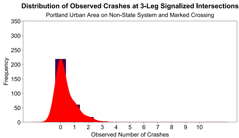
Figure D.10: Distribution of Observed Crashes at 3-Leg Signalized Intersections on Non-State System with Marked Crossing
