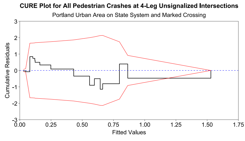
Figure 4.5: CURE Plots for 4-Leg Unsignalized Intersections and Marked Crossing (a) Statewide, (b) Portland Urban Area, and (c) Portland/Corvallis Urban Areas on State System
