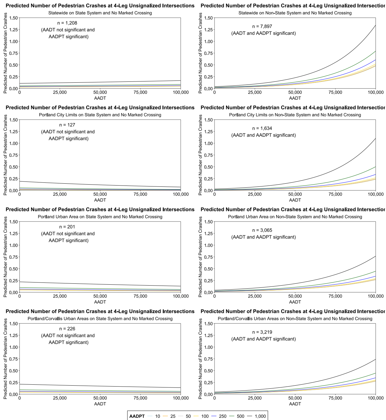
Figure 4.22: Predicted Number of Pedestrian Crashes at 4-Leg Unsignalized Intersections with No Marked Crossing
