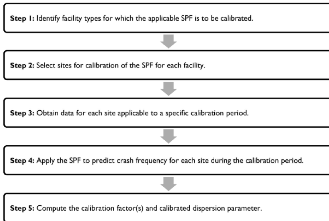
Figure 2.2 Calibration Process proposed in Lyon et al., 2016 (p. 4)
