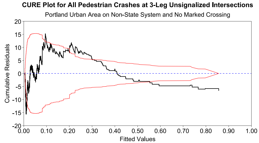
Figure 4.16: CURE Plots for 3-Leg Unsignalized Intersections and No Marked Crossing (a) Statewide, (b) Portland City Limits, (c) Portland Urban Area, and (d) Portland/Corvallis Urban Areas on Non-State System
