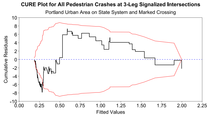
Figure 4.9: CURE Plots for 3-Leg Signalized Intersections and Marked Crossing (a) Statewide, (b) Portland City Limits, (c) Portland Urban Area, and (d) Portland/Corvallis Urban Areas on State System
