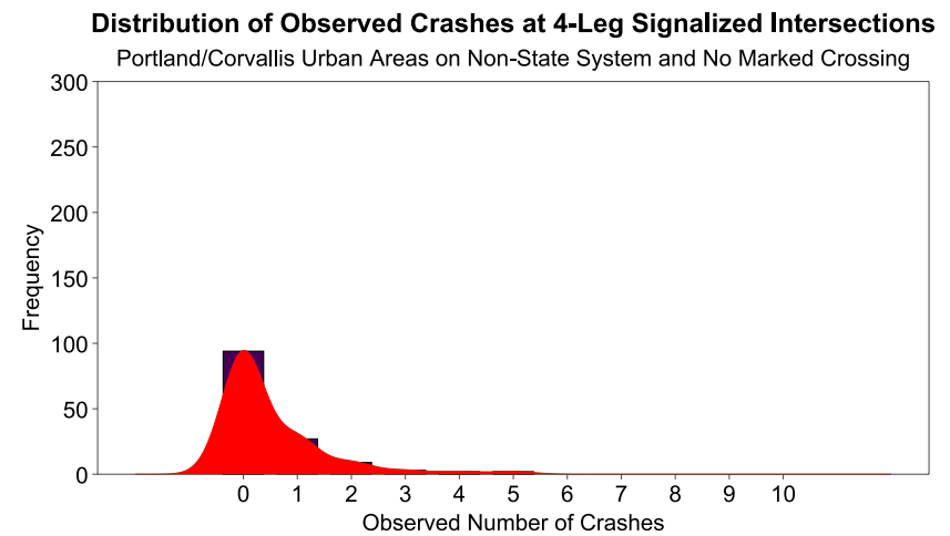
Figure D.4: Distribution of Observed Crashes at 4-Leg Signalized Intersections on Non-State System with No Marked Crossing
