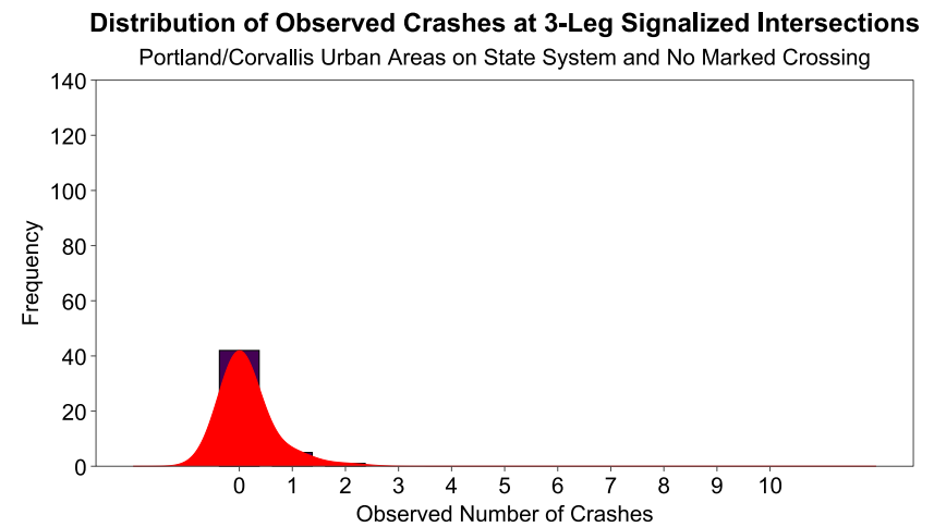
Figure D.11: Distribution of Observed Crashes at 3-Leg Signalized Intersections on State System with No Marked Crossing
