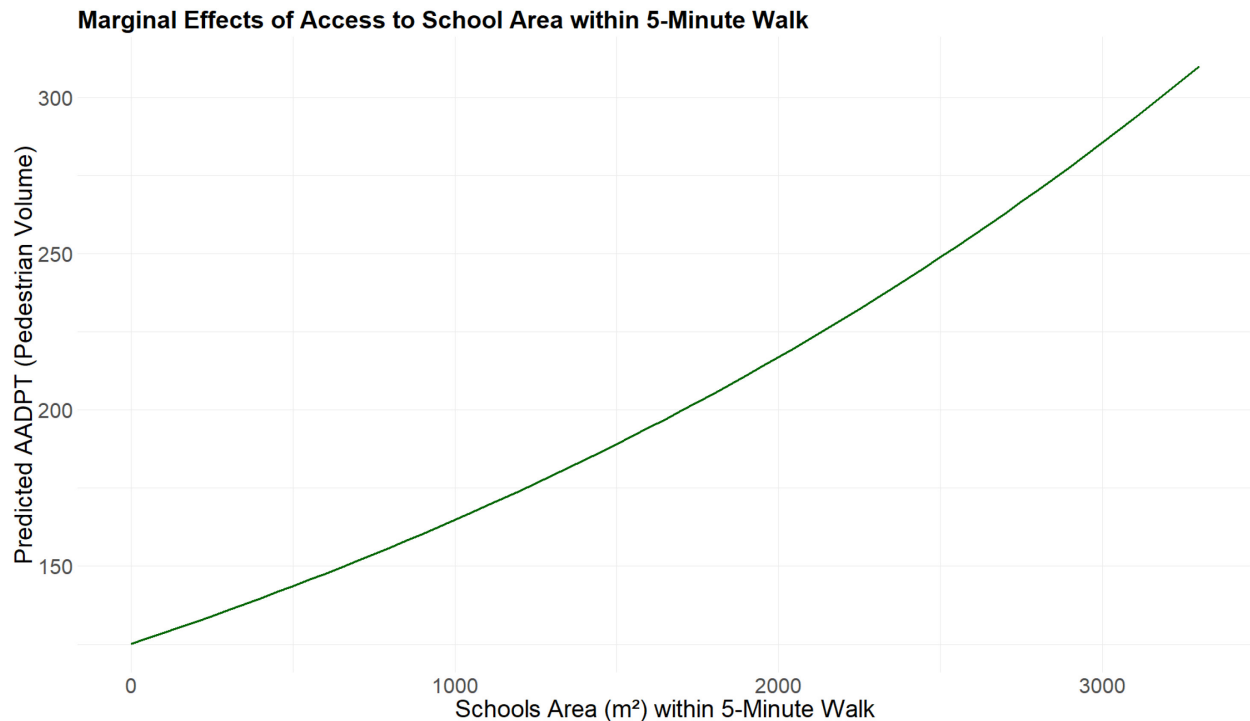
Figure 3.20: Access to School Area (m 2 ) Marginal Effects on AADPT
