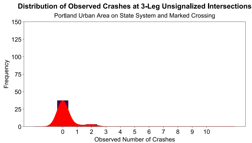
Figure D.13: Distribution of Observed Crashes at 3-Leg Unsignalized Intersections on State System with Marked Crossing
