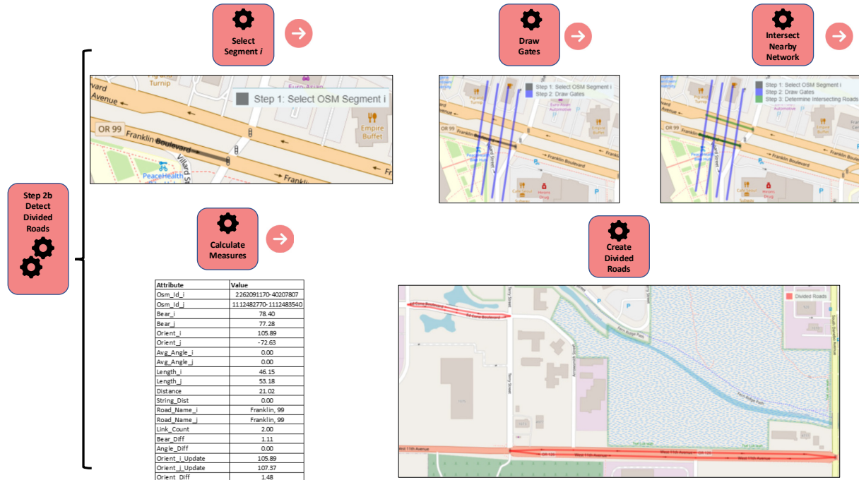
Figure 3.4: Step 2b – Workflow for Detecting Divided Roads in Base Network data
