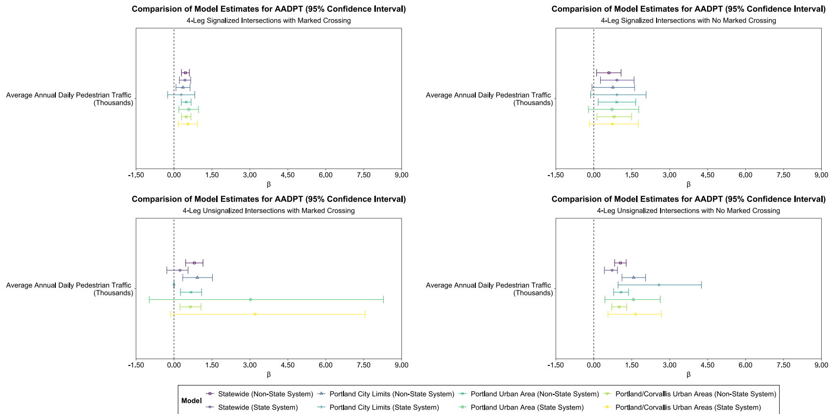
Figure 4.18: Comparison of Model Estimates for AADPT Between 4-Leg Intersection Models
