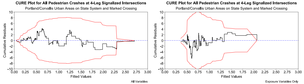
Figure A.7: Comparison of CURE Plots Between Full Model and Exposure-Only Model at 4-Leg Signalized Intersections, Portland/Corvallis Urban Areas, on State System, and Marked Crossing
