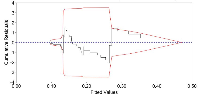
Figure 4.13: CURE Plots for 3-Leg Unsignalized Intersections and Marked Crossing (a) Statewide, (b) Portland City Limits, (c) Portland Urban Area, and (d) Portland/Corvallis Urban Areas on State System
