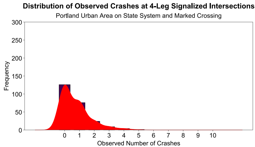
Figure D.1: Distribution of Observed Crashes at 4-Leg Signalized Intersections on State System with Marked Crossing
