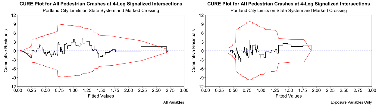
Figure A.3: Comparison of CURE Plots Between Full Model and Exposure-Only Model at 4-Leg Signalized Intersections, Portland City Limits, on State System, and Marked Crossing
