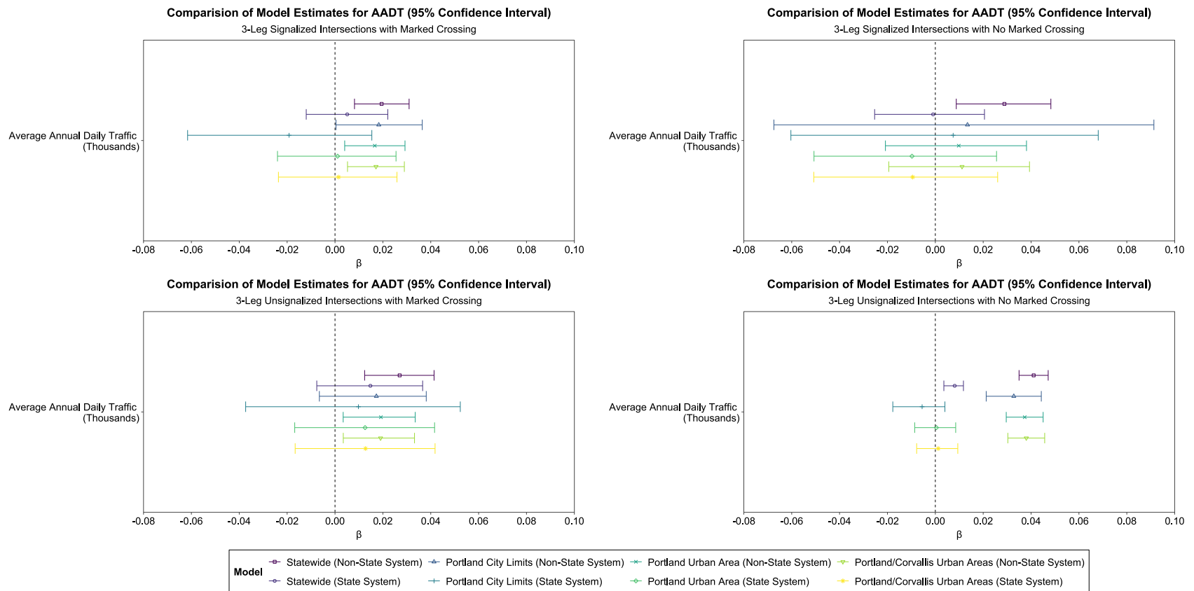
Figure 4.23: Comparison of Model Estimates for AADT Between 3-Leg Intersection Models
