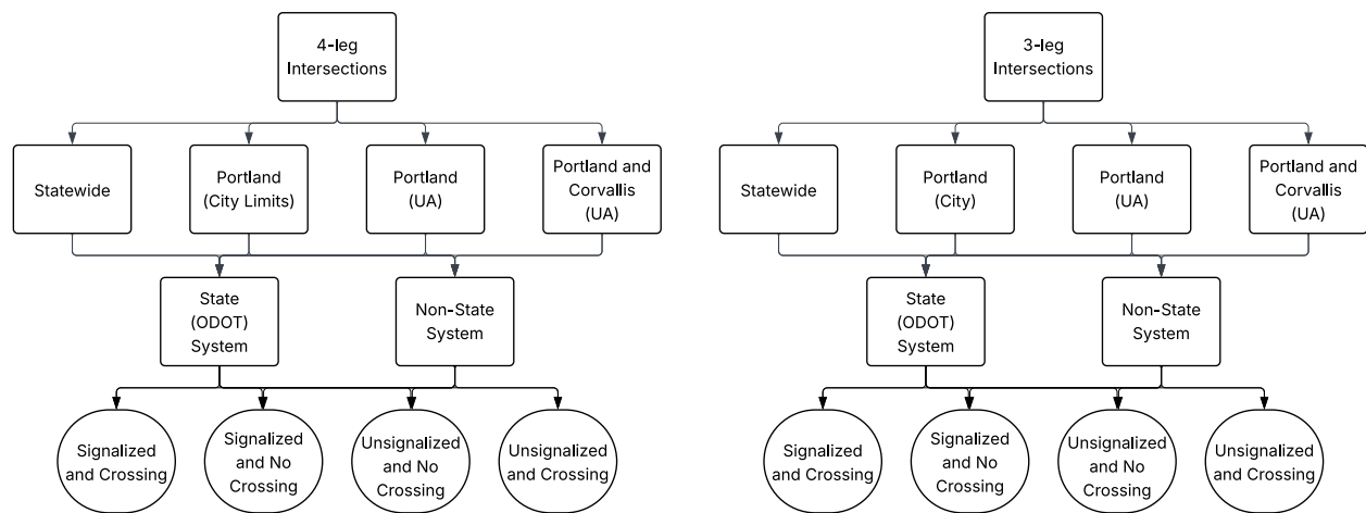
Figure 4.1: Pedestrian Crash Frequency Model Workflow
