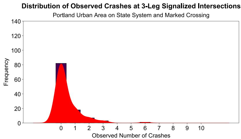
Figure D.9: Distribution of Observed Crashes at 3-Leg Signalized Intersections on State System with Marked Crossing
