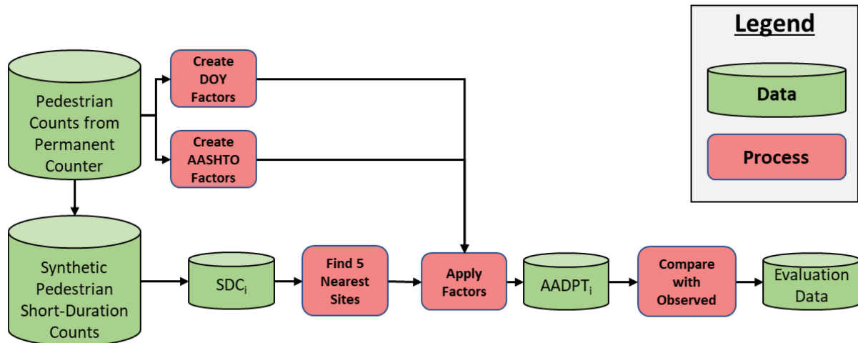
Figure 3.14: Annual Factoring Method Testing Flowchart
