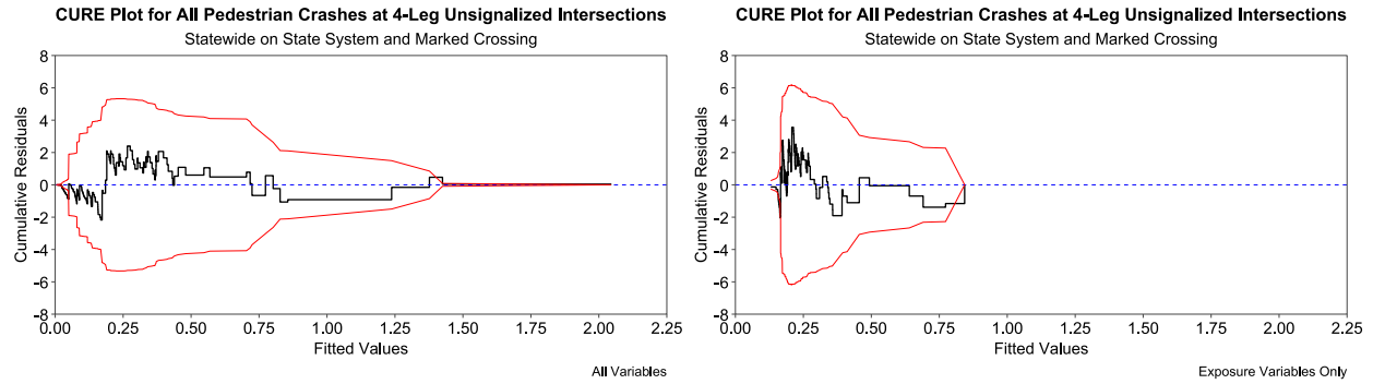
Figure A.15: Comparison of CURE Plots Between Full Model and Exposure-Only Model at 4-Leg Unsignalized Intersections, Statewide, on State System, and Marked Crossing
