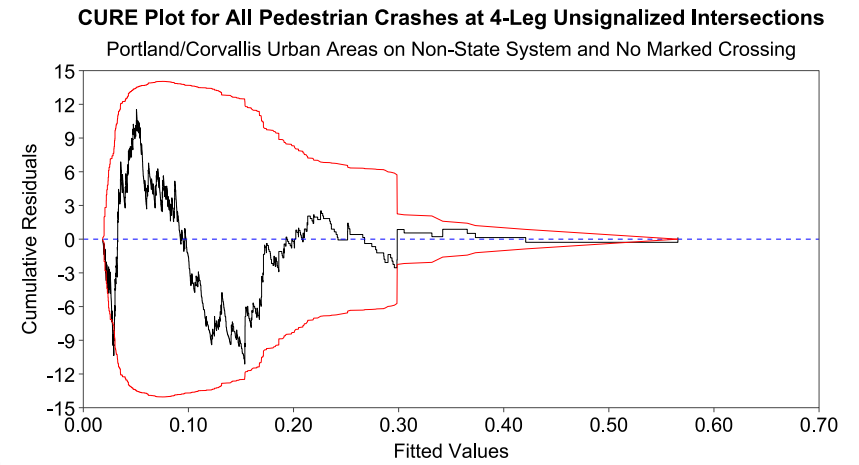
Figure 4.8: CURE Plots for 4-Leg Unsignalized Intersections and No Marked Crossing (a) Statewide, (b) Portland City Limits, (c) Portland Urban Area, and (d) Portland/Corvallis Urban Areas on Non-State System
