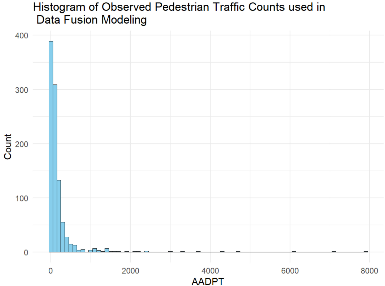
Figure 3.18: Distribution of AADPT Measures
