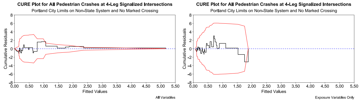
Figure A.11: Comparison of CURE Plots Between Full Model and Exposure-Only Model at 4-Leg Signalized Intersections, Portland City Limits, on Non-State System, and No Marked Crossing
