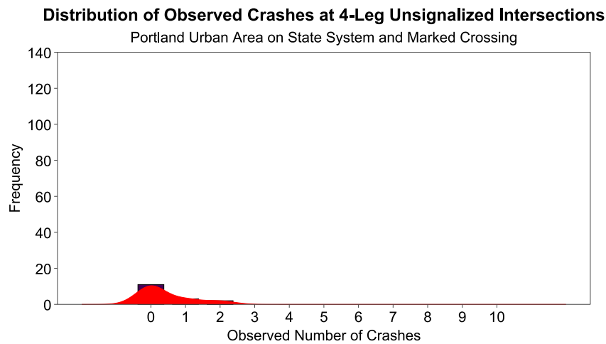
Figure D.5: Distribution of Observed Crashes at 4-Leg Unsignalized Intersections on State System with Marked Crossing
