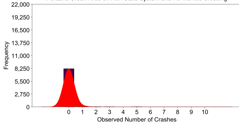
Figure D.16: Distribution of Observed Crashes at 3-Leg Unsignalized Intersections on Non-State System with No Marked Crossing
