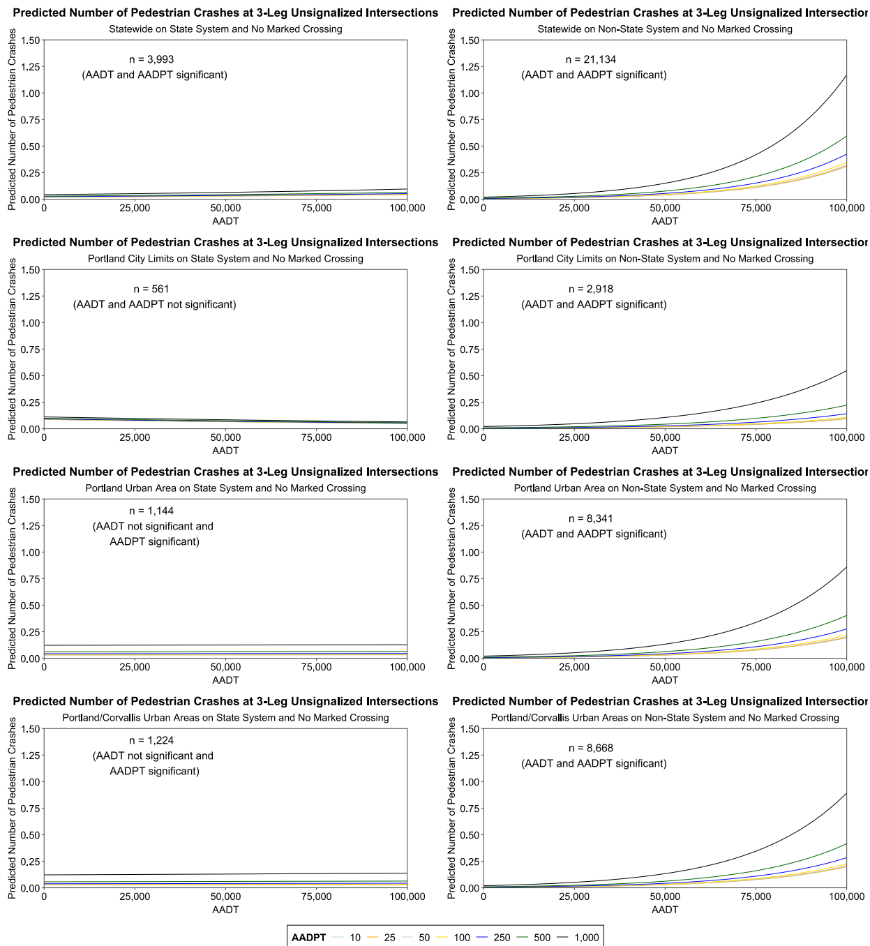
Figure 4.28: Predicted Number of Pedestrian Crashes at 3-Leg Unsignalized Intersections with No Marked Crossing
