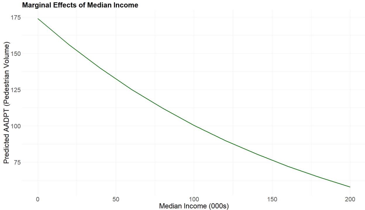
Figure 3.21: Median Income Marginal Effects on AADPT
