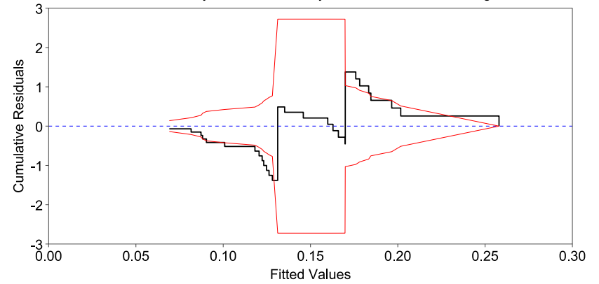
CURE Plot for All Pedestrian Crashes at 3-Leg Unsignalized Intersections
