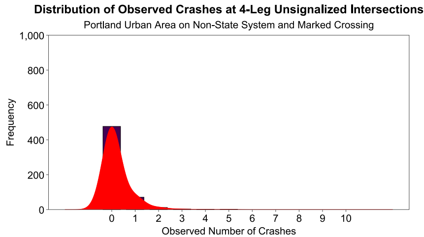
Figure D.6: Distribution of Observed Crashes at 4-Leg Unsignalized Intersections on Non-State System with Marked Crossing
