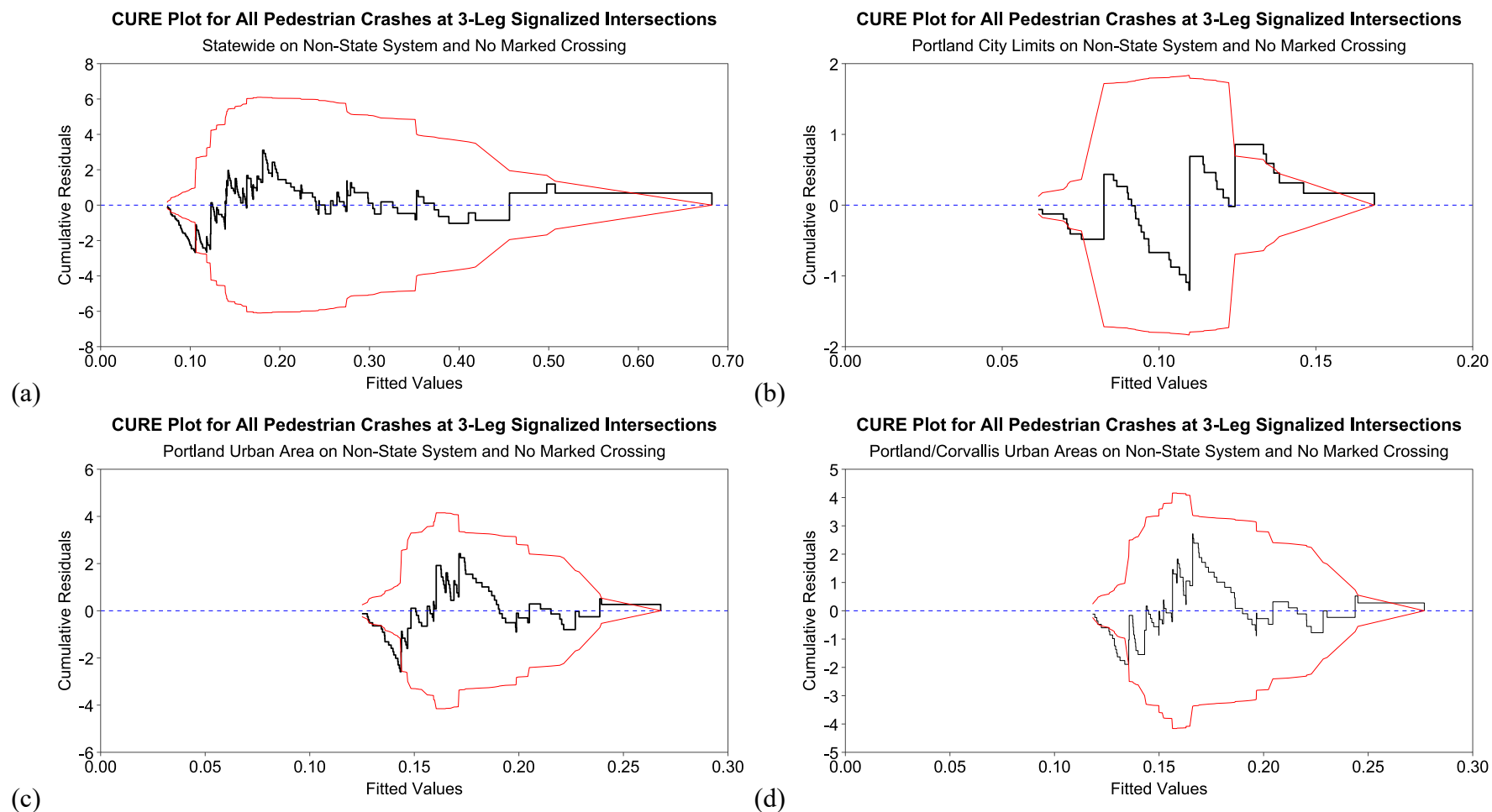
Figure 4.12: CURE Plots for 3-Leg Signalized Intersections and No Marked Crossing (a) Statewide, (b) Portland City Limits, (c) Portland Urban Area, and (d) Portland/Corvallis Urban Areas on Non-State System
