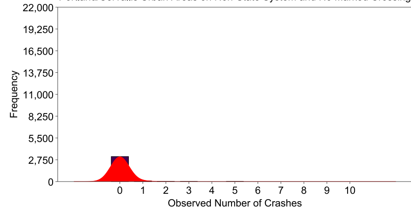
Figure D.16: Distribution of Observed Crashes at 3-Leg Unsignalized Intersections on Non-State System with No Marked Crossing
