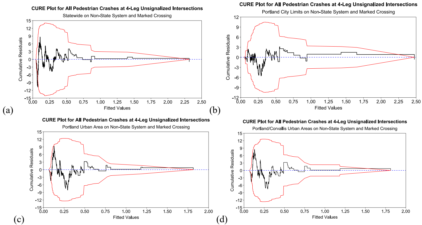
Figure 4.6: CURE Plots for 4-Leg Unsignalized Intersections and Marked Crossing (a) Statewide, (b) Portland City Limits, (c) Portland Urban Area, and (d) Portland/Corvallis Urban Areas on Non-State System
