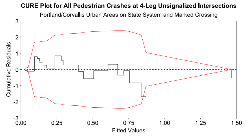
Figure 4.5: CURE Plots for 4-Leg Unsignalized Intersections and Marked Crossing (a) Statewide, (b) Portland Urban Area, and (c) Portland/Corvallis Urban Areas on State System
