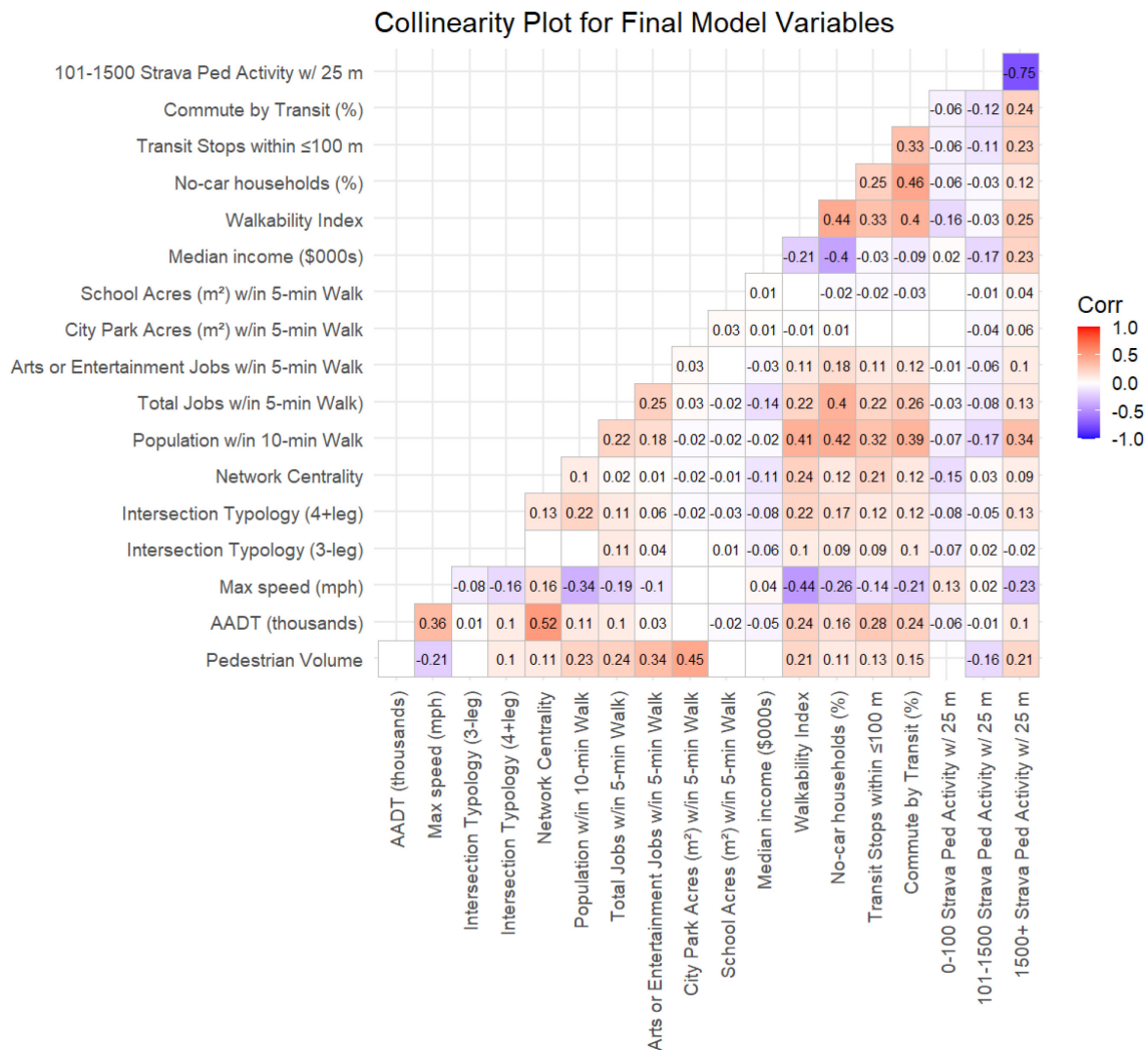
Figure 3.22: Collinearity Plot for Final Model Variables
