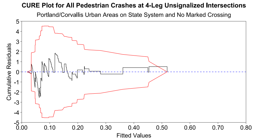
Figure 4.7: CURE Plots for 4-Leg Unsignalized Intersections and No Marked Crossing (a) Statewide, (b) Portland City Limits, (c) Portland Urban Area, and (d) Portland/Corvallis Urban Areas on State System
