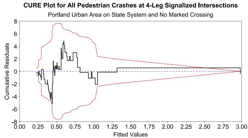
Figure 4.3: CURE Plots for 4-Leg Signalized Intersections and No Marked Crossing (a) Statewide, (b) Portland City Limits, (c) Portland Urban Area, and (d) Portland/Corvallis Urban Areas on State System
