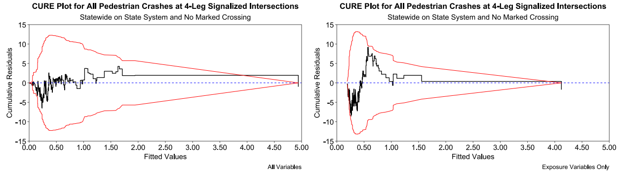
Figure A.9: Comparison of CURE Plots Between Full Model and Exposure-Only Model at 4-Leg Signalized Intersections, Statewide, on State System, and No Marked Crossing
