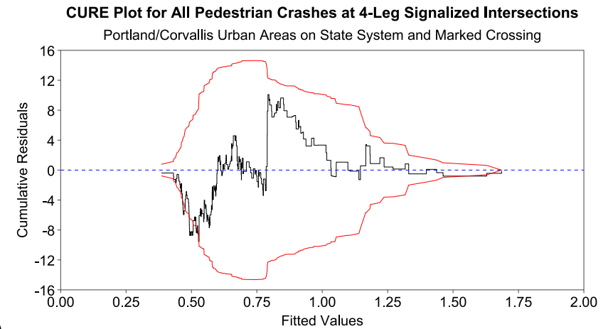
Figure 4.1: CURE Plots for 4-Leg Signalized Intersections and Marked Crossing (a) Statewide, (b) Portland City Limits, (c) Portland Urban Area, and (d) Portland/Corvallis Urban Areas on State System
