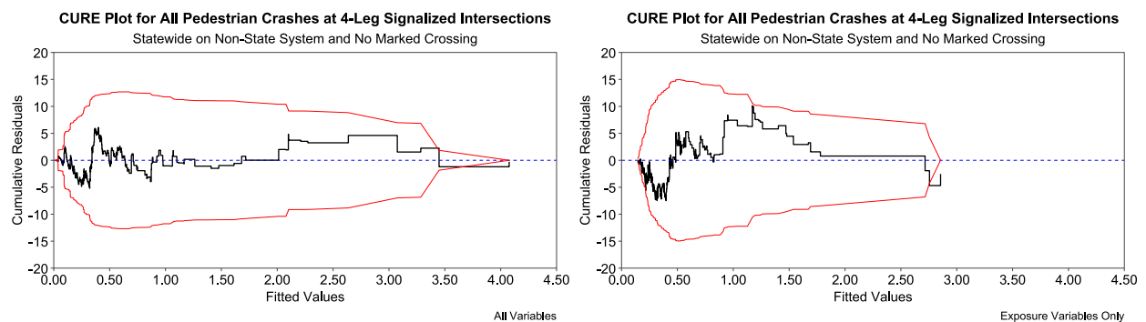
Figure A.10: Comparison of CURE Plots Between Full Model and Exposure-Only Model at 4-Leg Signalized Intersections, Statewide, on Non-State System, and No Marked Crossing
