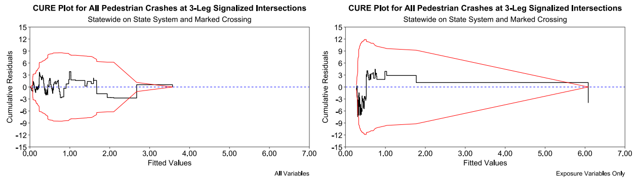
Figure A.17: Comparison of CURE Plots Between Full Model and Exposure-Only Model at 3-Leg Signalized Intersections, Statewide, on State System, and Marked Crossing
