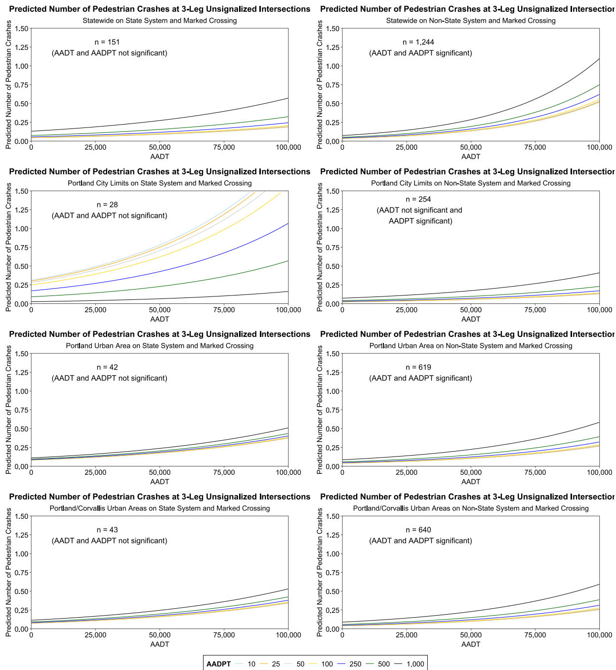
Figure 4.27: Predicted Number of Pedestrian Crashes at 3-Leg Unsignalized Intersections with Marked Crossing
