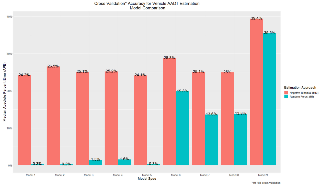
Figure 3.6: Median Absolute Percent Error from 10-fold Cross-Validation for AADT Data Fusion Model
