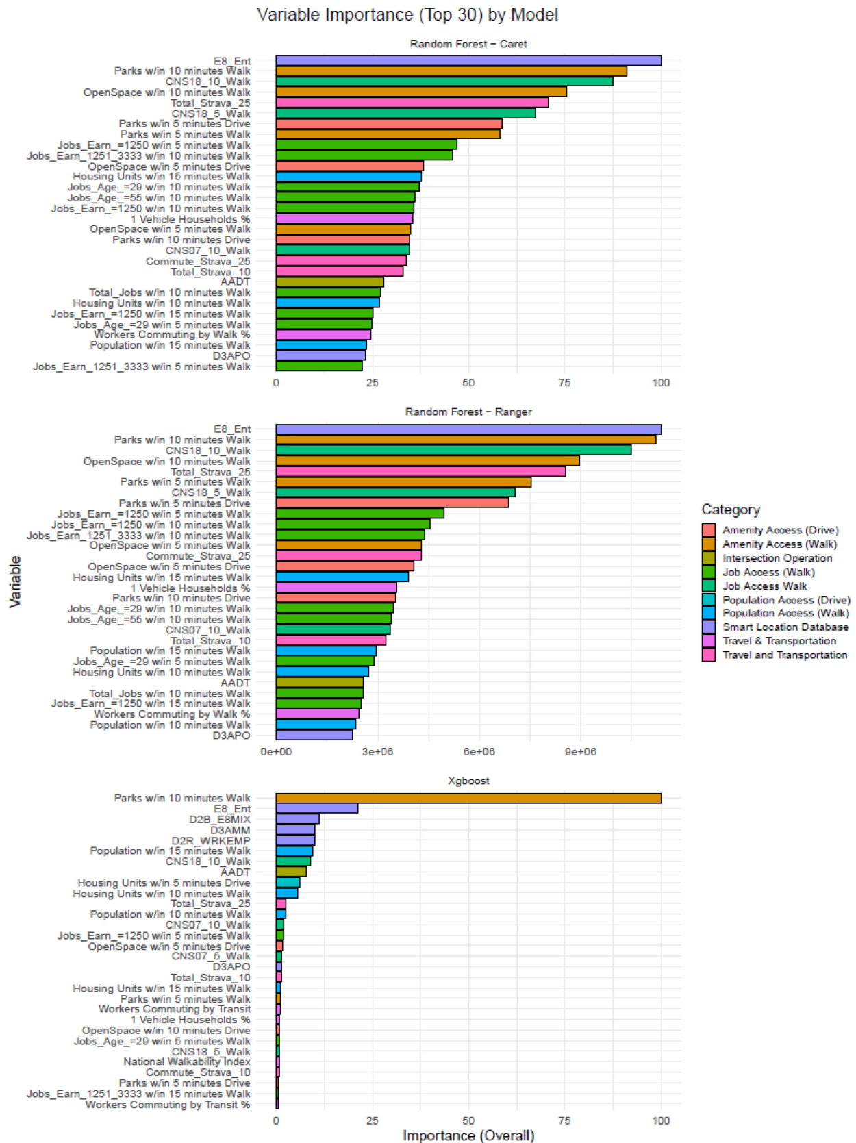
Figure 3.24: Variable Importance (Top 30) by Model
