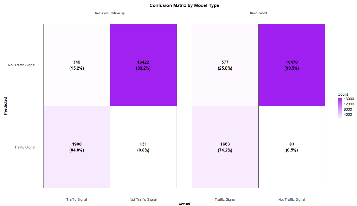
Figure 3.12: Confusion matrix from 10-fold cross validation of recursive partitioning model
