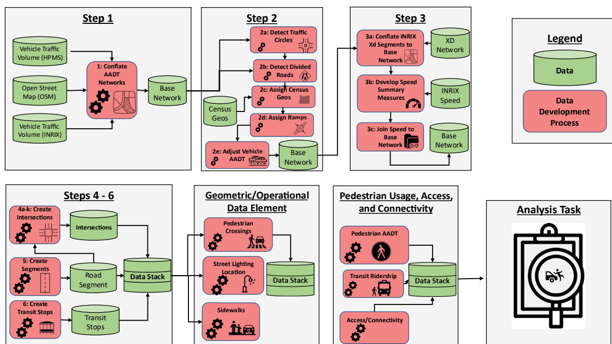
Figure 3.1: Data Development Flow Chart
