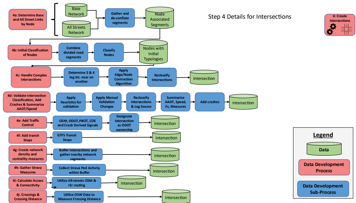
Figure 3.7: Intersection Data Development Processes and Sub-Processes
