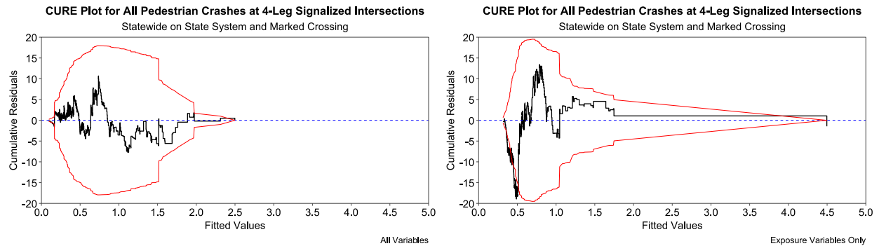
Figure A.1: Comparison of CURE Plots Between Full Model and Exposure-Only Model at 4-Leg Signalized Intersections, Statewide, on State System, and Marked Crossing
