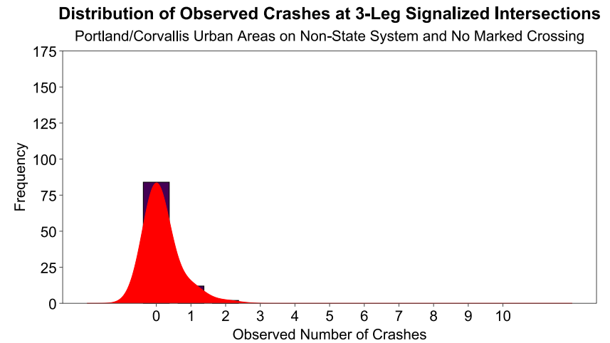
Figure D.12: Distribution of Observed Crashes at 3-Leg Signalized Intersections on Non-State System with No Marked Crossing
