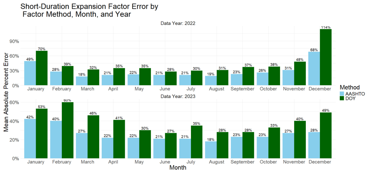
Figure 3.15: Mean Average Error from Annual Factoring Method Testing
