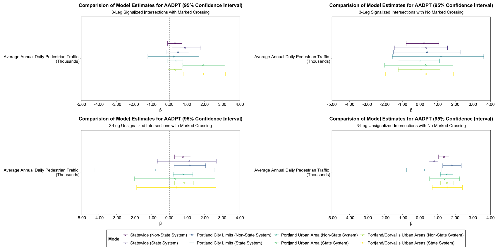
Figure 4.24: Comparison of Model Estimates for AADPT Between 3-Leg Intersection Models
