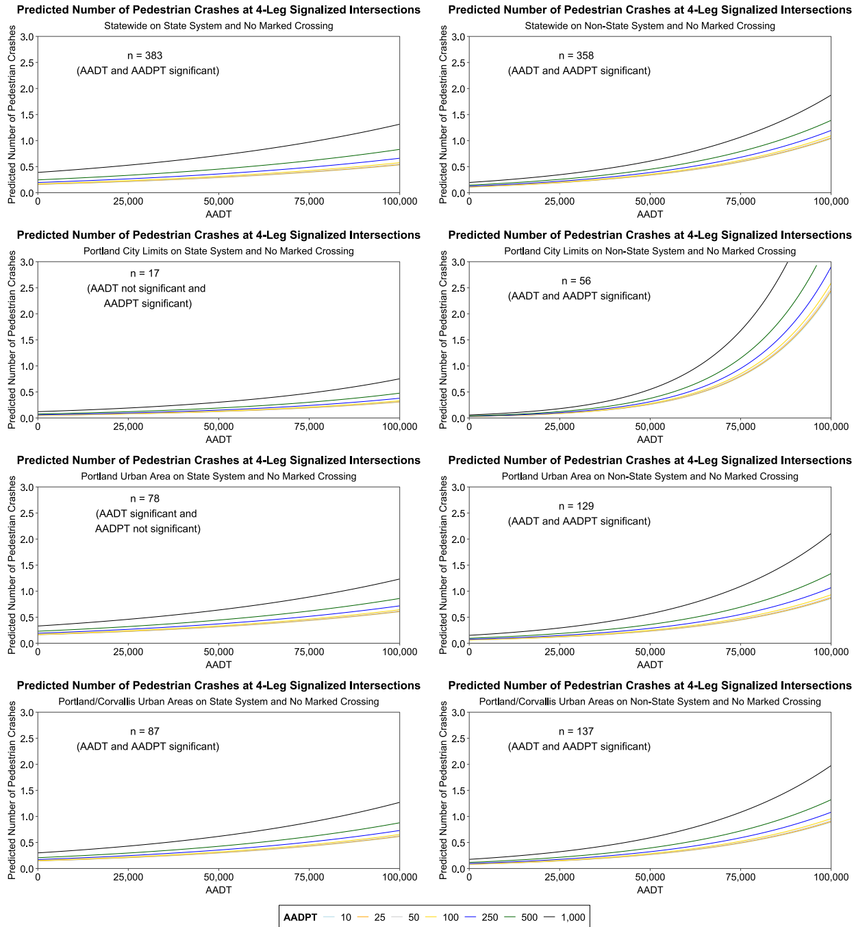
Figure 4.20: Predicted Number of Pedestrian Crashes at 4-Leg Signalized Intersections with No Marked Crossing
