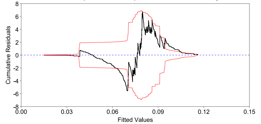
CURE Plot for All Pedestrian Crashes at 3-Leg Unsignalized Intersections Portland/Corvallis Urban Areas on State System and No Marked Crossing
