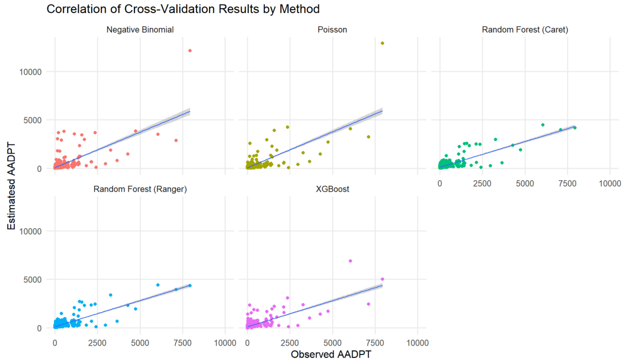
Figure 3.23: Correlation of Cross-Validation Results by Method
