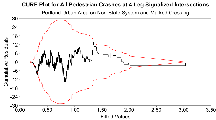
Figure 4.2: CURE Plots for 4-Leg Signalized Intersections and Marked Crossing (a) Statewide, (b) Portland City Limits, (c) Portland Urban Area, and (d) Portland/Corvallis Urban Areas on Non-State System
