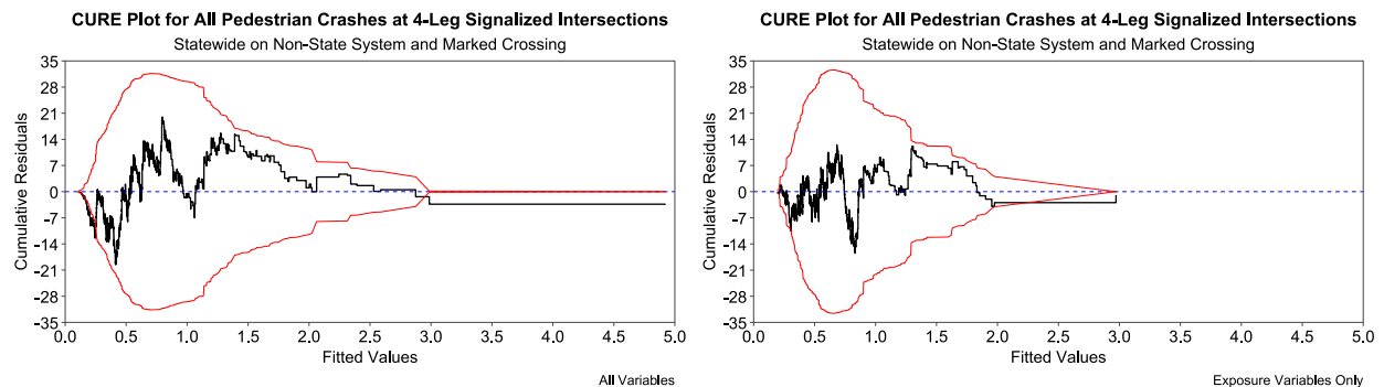
Figure A.2: Comparison of CURE Plots Between Full Model and Exposure-Only Model at 4-Leg Signalized Intersections, Statewide, on Non-State System, and Marked Crossing
