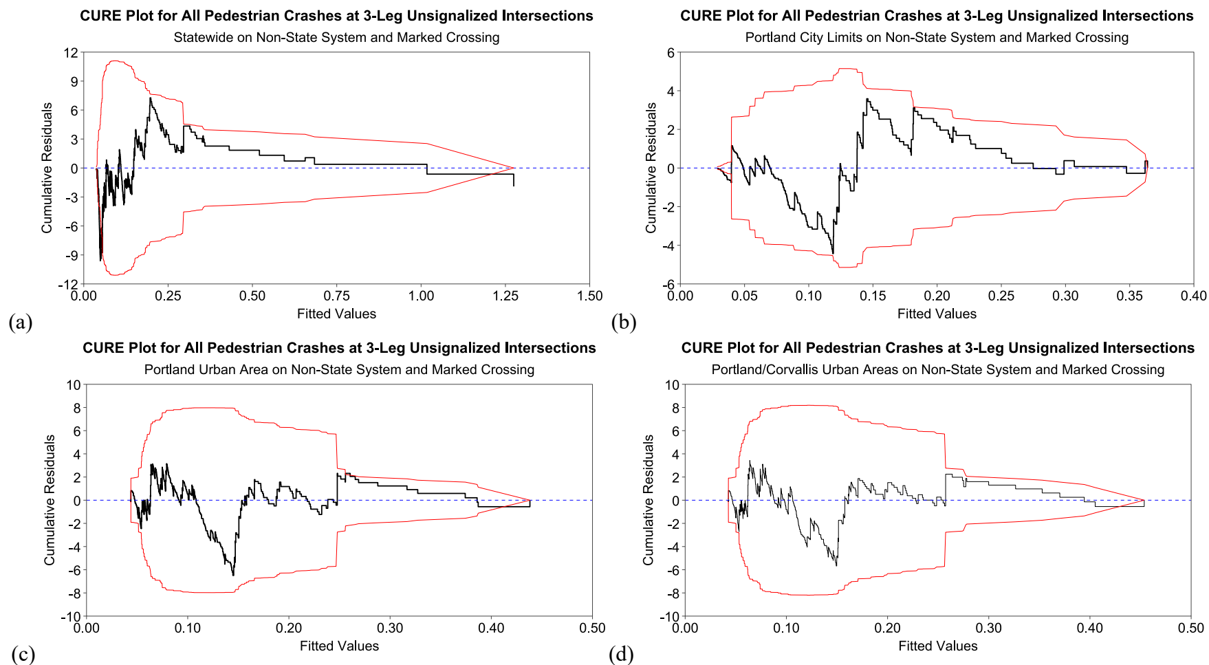
Figure 4.14: CURE Plots for 3-Leg Unsignalized Intersections and Marked Crossing (a) Statewide, (b) Portland City Limits, (c) Portland Urban Area, and (d) Portland/Corvallis Urban Areas on Non-State System
