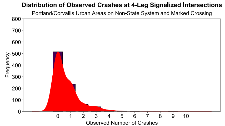
Figure D.2: Distribution of Observed Crashes at 4-Leg Signalized Intersections on Non-State System with Marked Crossing
