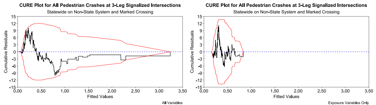
Figure A.18: Comparison of CURE Plots Between Full Model and Exposure-Only Model at 3-Leg Signalized Intersections, Statewide, on Non-State System, and Marked Crossing
