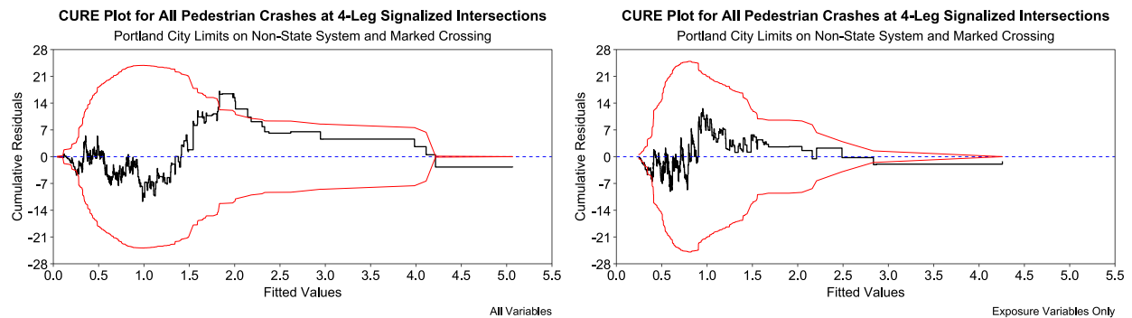
Figure A.4: Comparison of CURE Plots Between Full Model and Exposure-Only Model at 4-Leg Signalized Intersections, Portland City Limits, on Non-State System, and Marked Crossing
