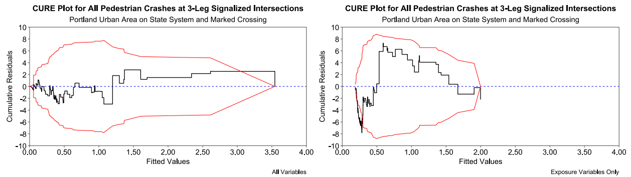
Figure A. 19: Comparison of CURE Plots Between Full Model and Exposure-Only Model at 3-Leg Signalized Intersections, Portland Urban Area, on State System, and Marked Crossing
