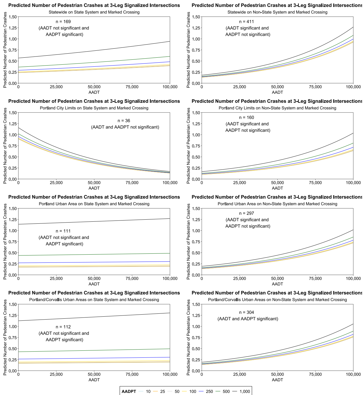
Figure 4.25: Predicted Number of Pedestrian Crashes at 3-Leg Signalized Intersections with Marked Crossing
