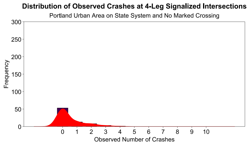
Figure D.3: Distribution of Observed Crashes at 4-Leg Signalized Intersections on State System with No Marked Crossing
