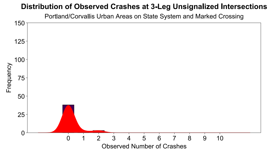
Figure D.13: Distribution of Observed Crashes at 3-Leg Unsignalized Intersections on State System with Marked Crossing
