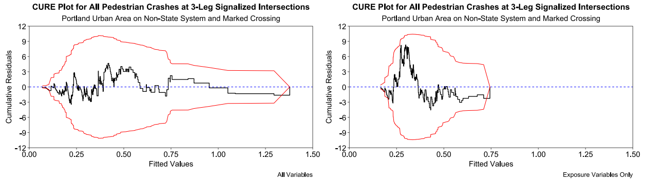
Figure A.20: Comparison of CURE Plots Between Full Model and Exposure-Only Model at 3-Leg Signalized Intersections, Portland Urban Area, on Non-State System, and Marked Crossing
