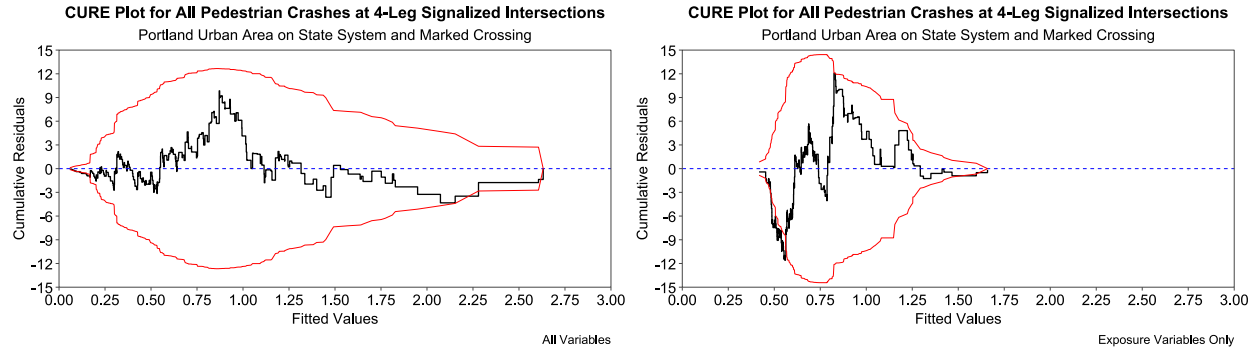
Figure A.5: Comparison of CURE Plots Between Full Model and Exposure-Only Model at 4-Leg Signalized Intersections, Portland Urban Area, on State System, and Marked Crossing
