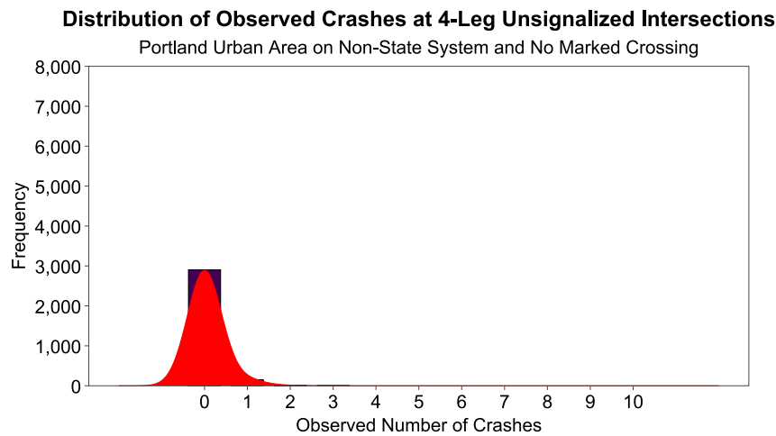
Figure D.8: Distribution of Observed Crashes at 4-Leg Unsignalized Intersections on Non-State System with No Marked Crossing
