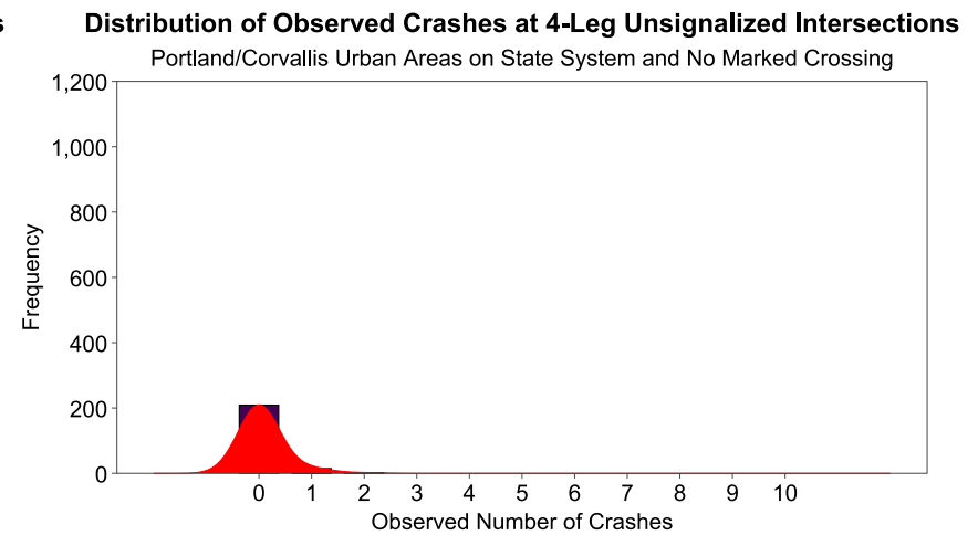
Figure D.7: Distribution of Observed Crashes at 4-Leg Unsignalized Intersections on State System with No Marked Crossing
