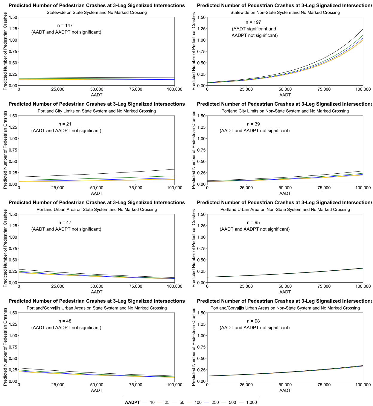
Figure 4.26: Predicted Number of Pedestrian Crashes at 3-Leg Signalized Intersections with No Marked Crossing
