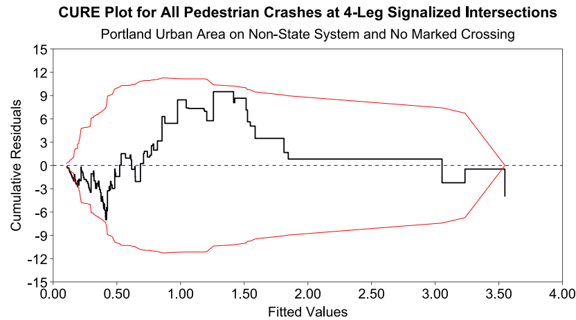
Figure 4.4: CURE Plots for 4-Leg Signalized Intersections and No Marked Crossing (a) Statewide, (b) Portland City Limits, (c) Portland Urban Area, and (d) Portland/Corvallis Urban Areas on Non-State System
