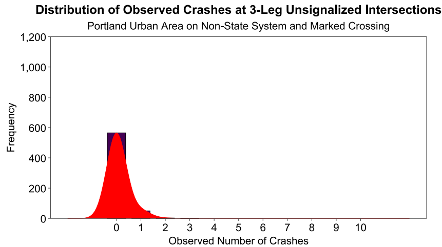
Figure D.14: Distribution of Observed Crashes at 3-Leg Unsignalized Intersections on Non-State System with Marked Crossing
