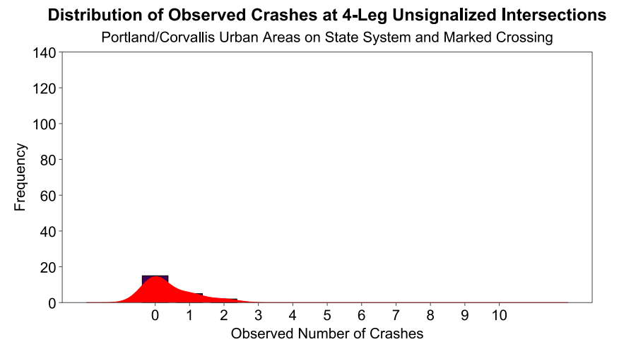
Figure D.5: Distribution of Observed Crashes at 4-Leg Unsignalized Intersections on State System with Marked Crossing
