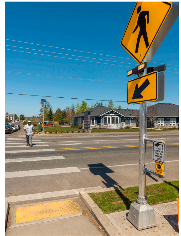
Example of a completed Rectangular Rapid Flashing Beacon (RRFB) crossing, creating a safer and more visible pedestrian crossing along a busy corridor.
