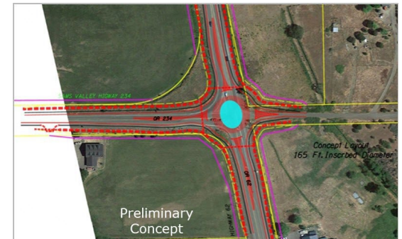
Preliminary concept of OR 62_234 roundabout
