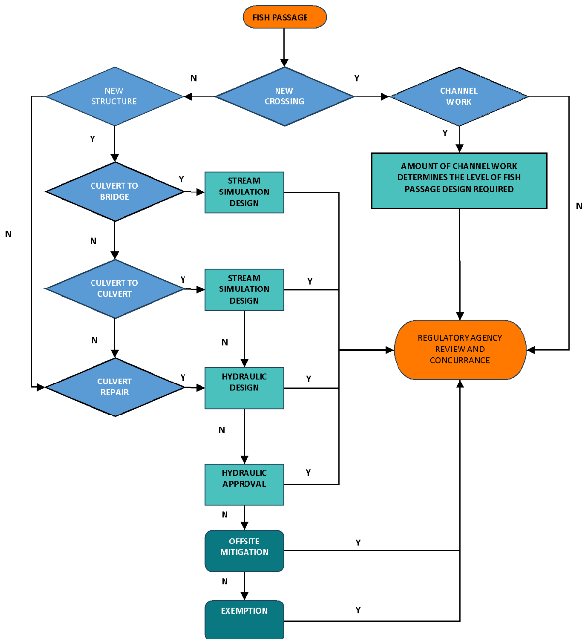
Figure 9.1-1: Fish Passage Project Flow Chart
