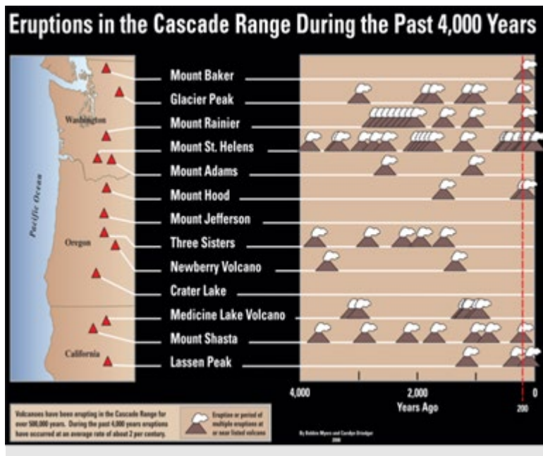
Figure 3.3.9-2: Eruptions in the Cascade Range During the Past 4,000 Years
