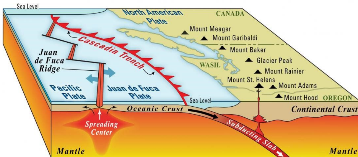
Figure 3.3.9-1: Generalized Subduction Zone Setting.
