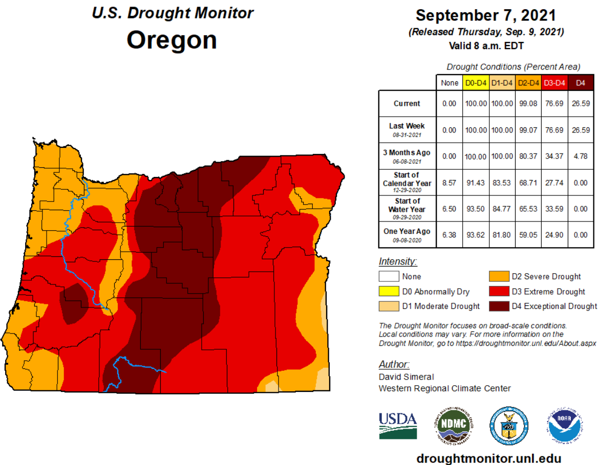
Figure 3.3.2-3 September 7, 2021 U.S. Drought Monitor Report for Oregon
