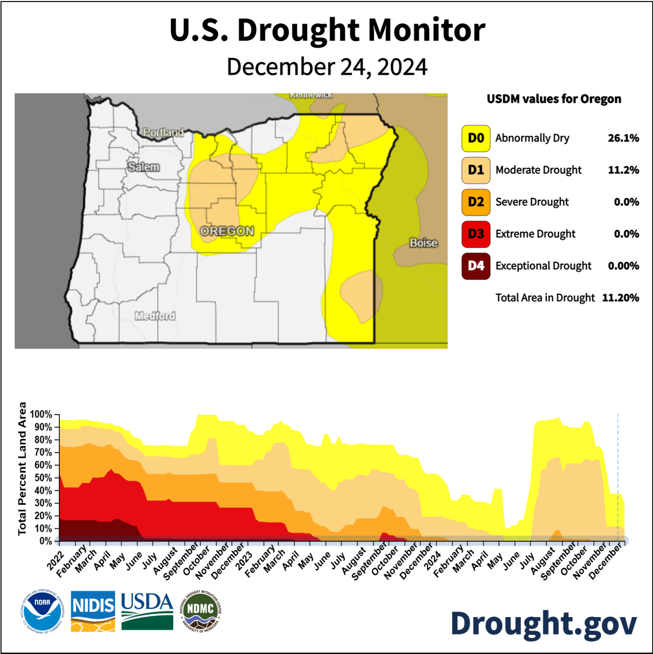
Figure 3.3.2-4 December 24, 2024 U.S. Drought Monitor Report for Oregon.
