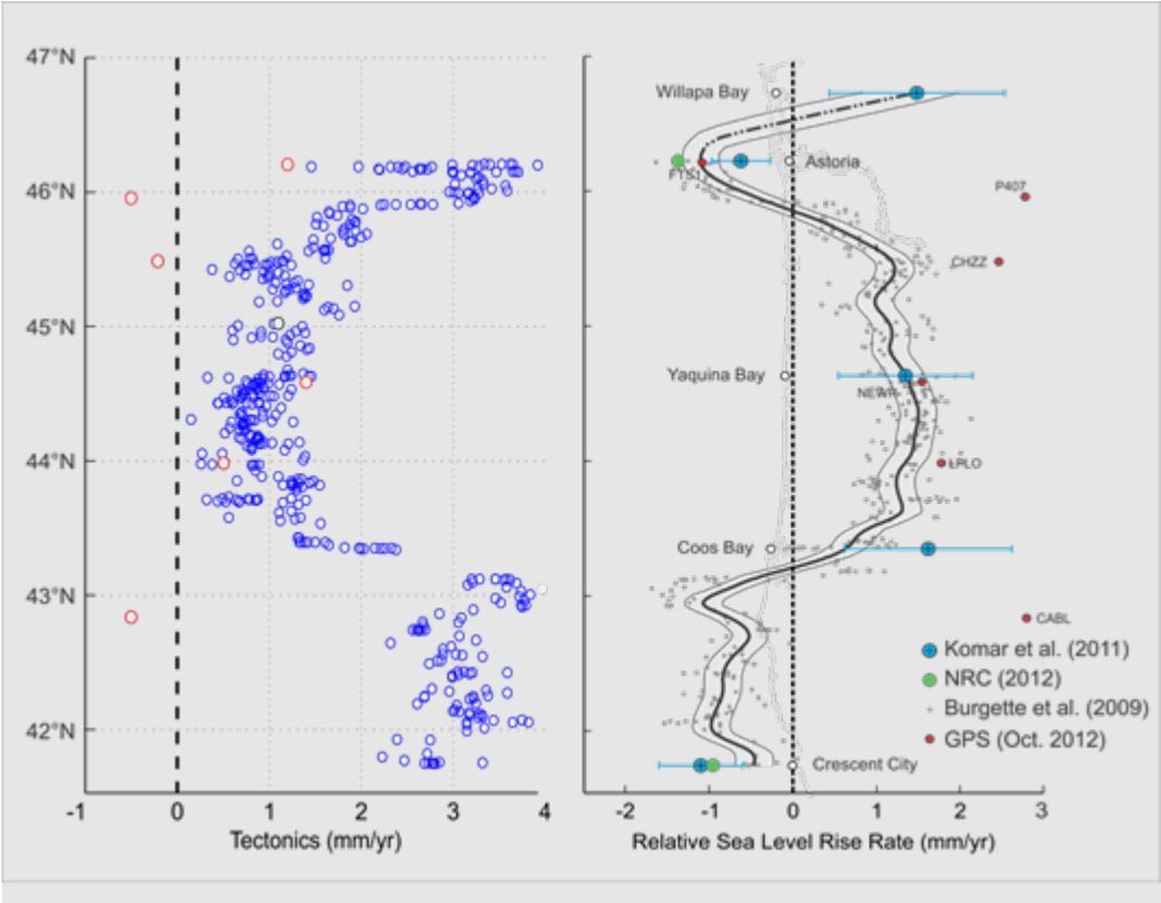
Figure 3.3.1-11: Coast Variations in Rates of Tectonic Uplift, and Relative Sea Level Trends for the Oregon Coast
