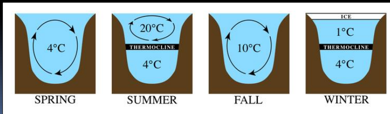
Seasonal Lake Turnover
