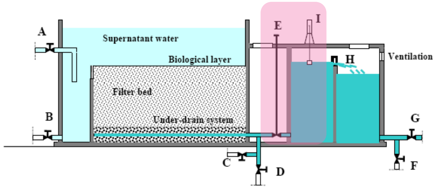
Basic components of an outlet controlled slow sand filter
