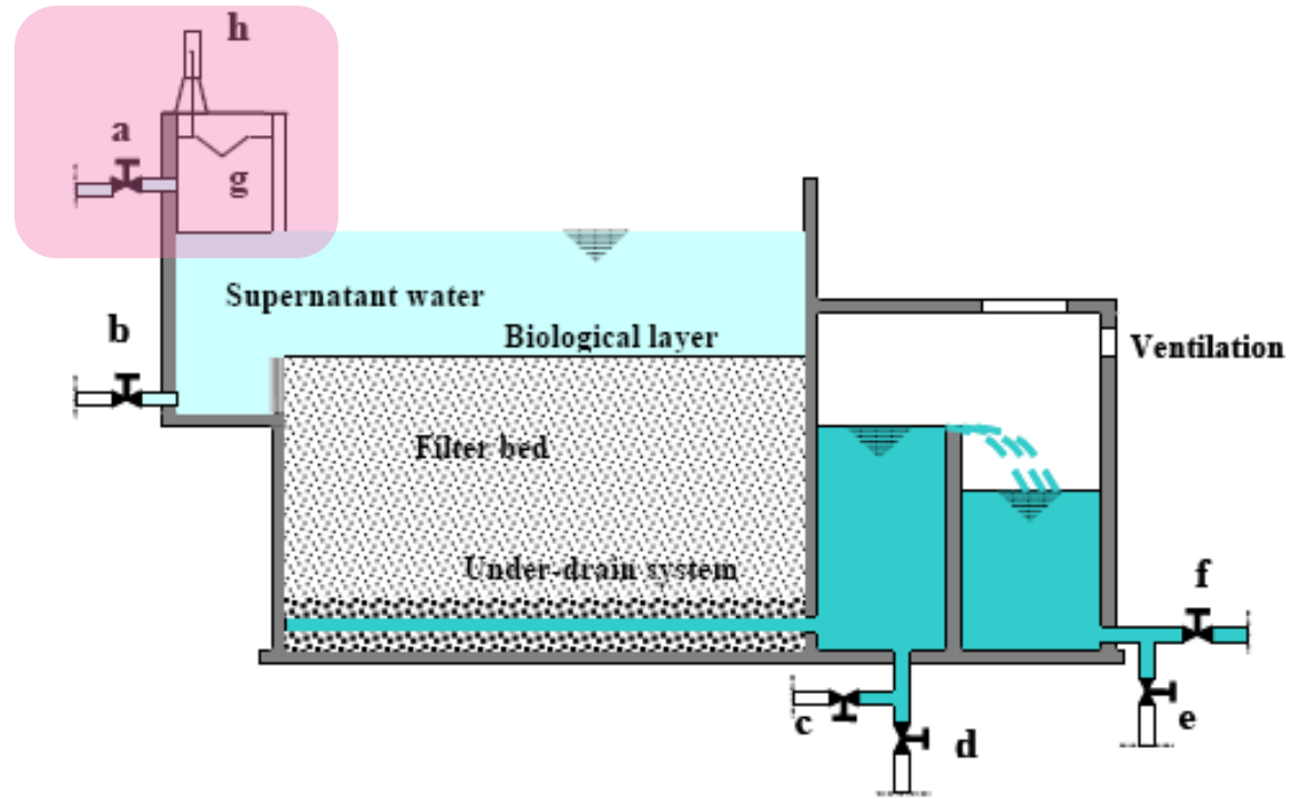
Basic components of an inlet controlled slow sand filter
