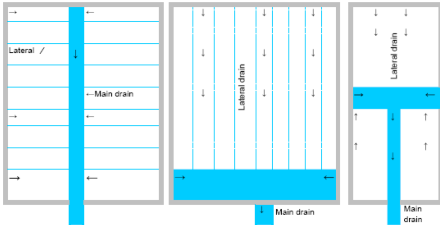
Figure 10: Common arrangements for the main drain of a slow sand filter
