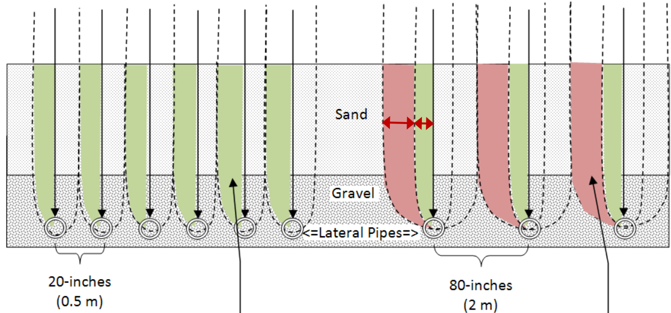
Streamlines with 20-in lateral spacing (shorter & more uniform flow paths)
