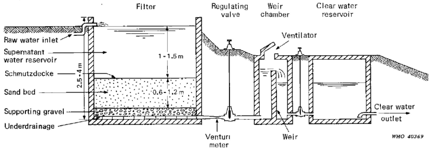
FIG. 1. DIAGRAM OF A SLOW SAND FILTER
