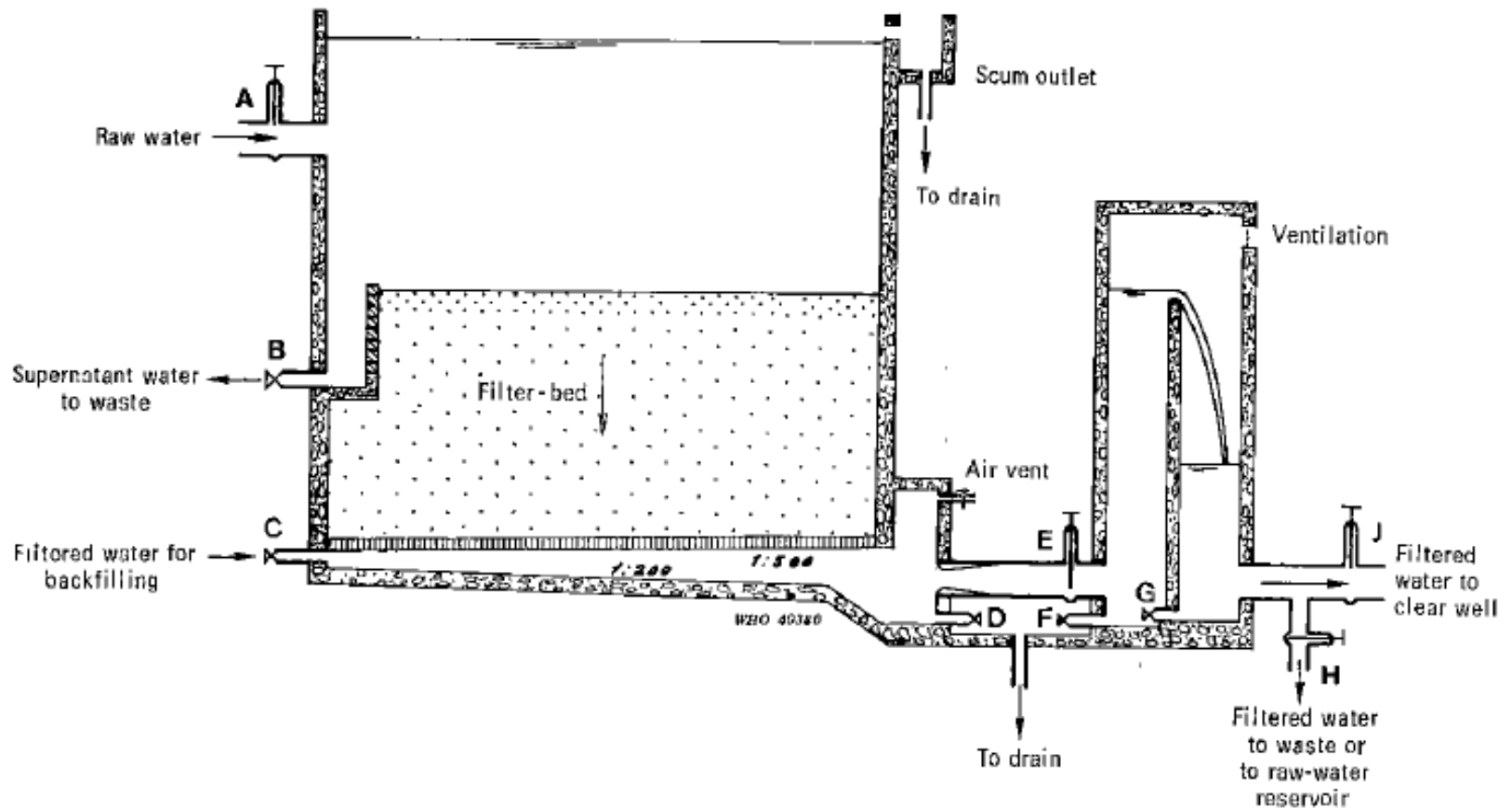
FIG. 18. DIAGRAM OF A SLOW FILTER, SHOWING CONTROL VALVES
