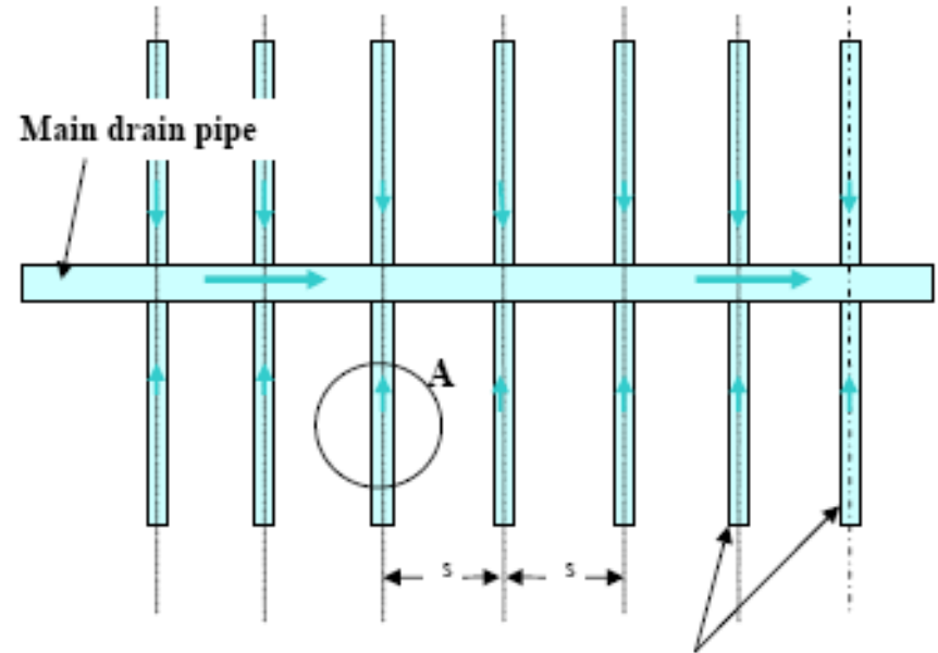
Lateral pipes
