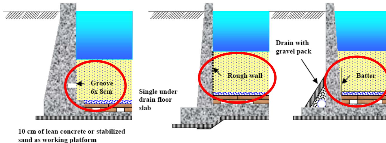
Figure 12: Method of preventing the short circuiting of the filter bed along the vertical wall (WHO)
