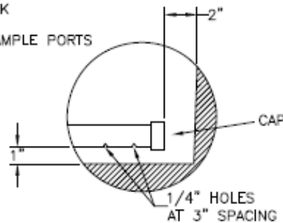
UNDER DRAIN DETAIL
