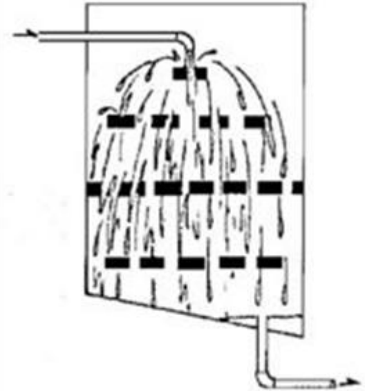
Fig 2: Wooden trays brake water up into droplets
