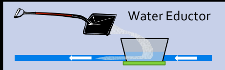
FIG. 32. HYDRAULIC SAND EJECTOR
