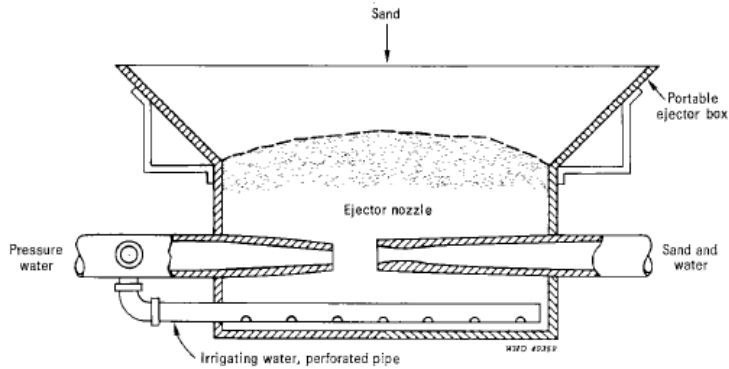
FIG. 32. HYDRAULIC SAND EJECTOR
