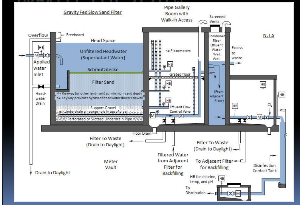
Gravity Fed system
