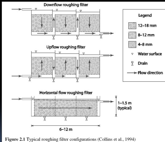
Figure 2.1 Typical roughing filter configurations (Collins et al., 1994)
