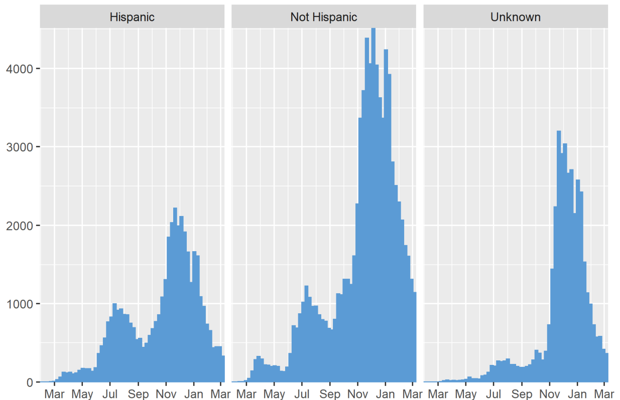
Figure 20. All COVID-19 cases by ethnicity (counts) and week of onset
